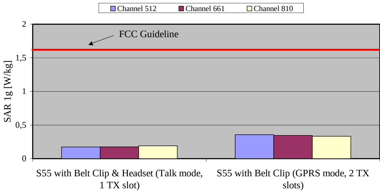
Fig. 9: The measured SAR values in body-worn configuration for the Siemens S55 for PCS 1900 in comparison to the FCC exposure limit. With Headset for Talk mode (1 TX slot) and without Headset for GPRS mode (2 TX slots). Since the GPRS software was not available during the SAR test, the measured values were multiplied by two to get this values. For the measurements the Belt Clip which dictates the closest spacing to the body was used.
