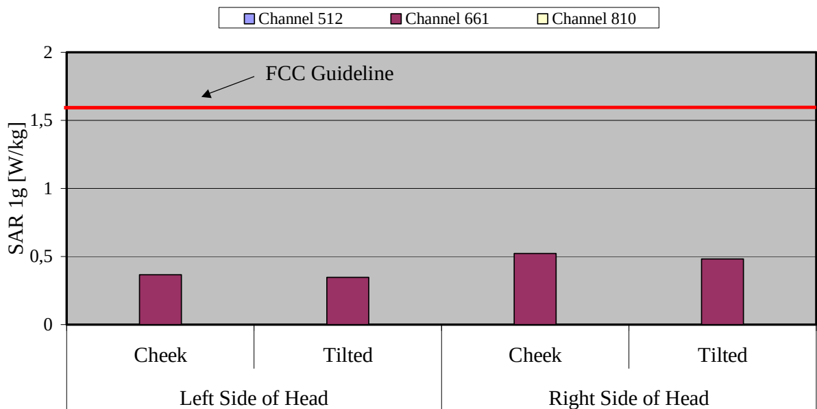
Fig. 8: The measured head phantom SAR values for the Siemens S55 with QuickPic Camera for PCS 1900 in comparison to the FCC exposure limit
