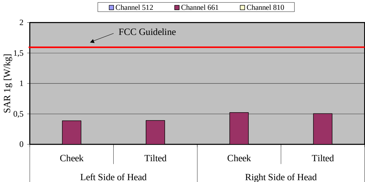
Fig. 7: The measured head phantom SAR values for the Siemens S55 for PCS 1900 in comparison to the FCC exposure limit.
