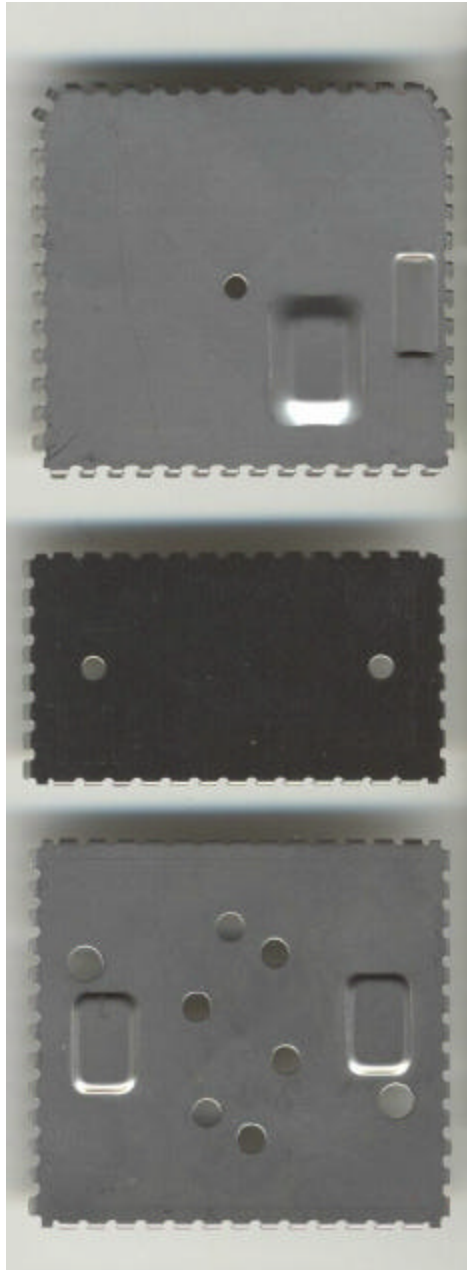
S46: Main Board (side 2) shielding
