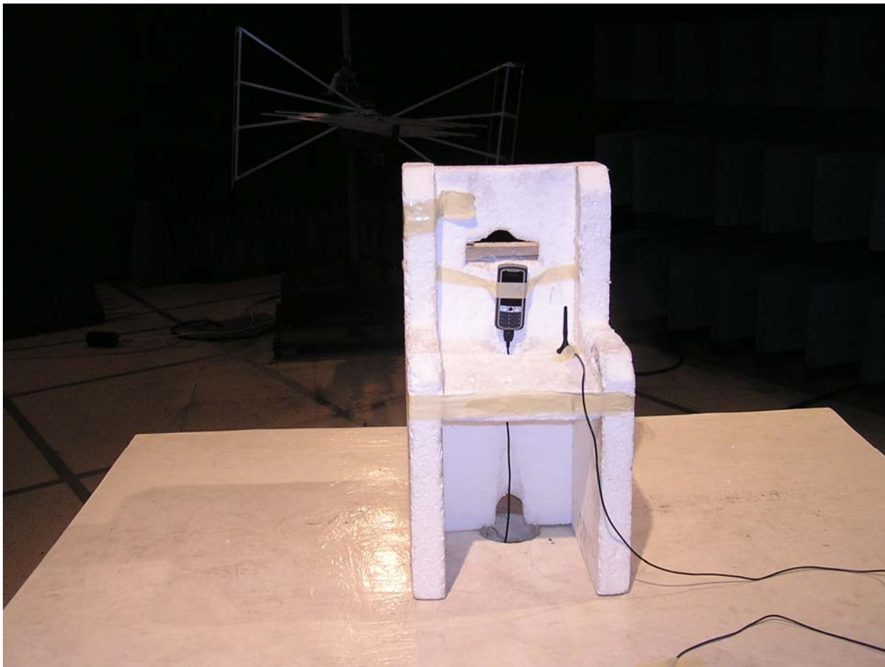
RADIATED EMISSIONS
