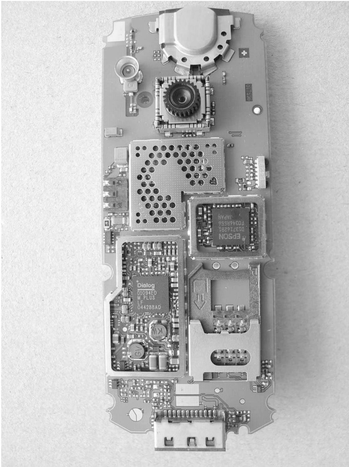
ME75 Back view repair lid mounted
