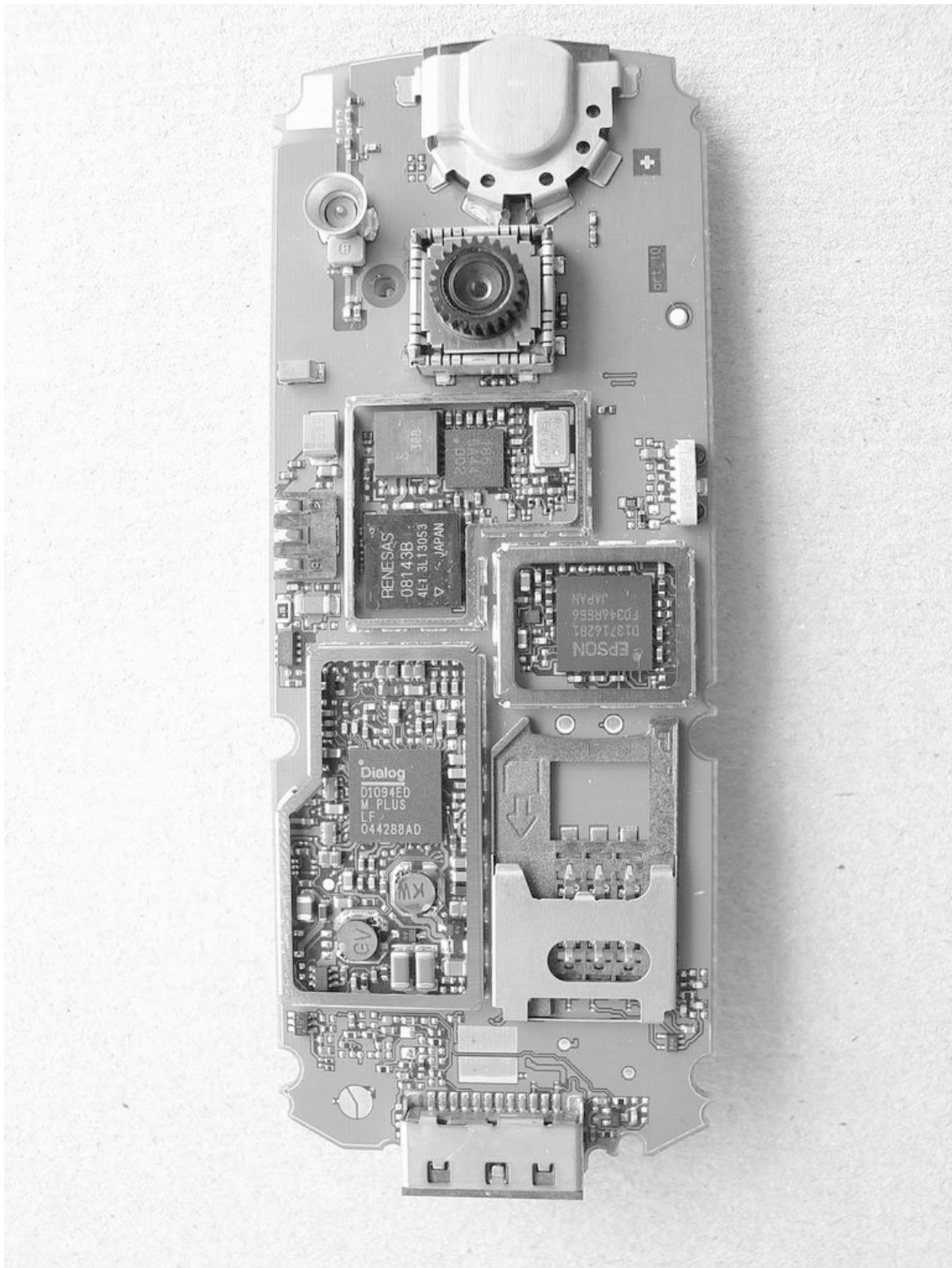
ME75 PCB Back View Shields Removed
