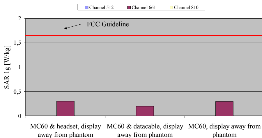
Fig. 9: The measured SAR values in body-worn configuration (GPRS mode) for the Siemens MC60 distance for PCS 1900 in comparison to the FCC exposure limit.
