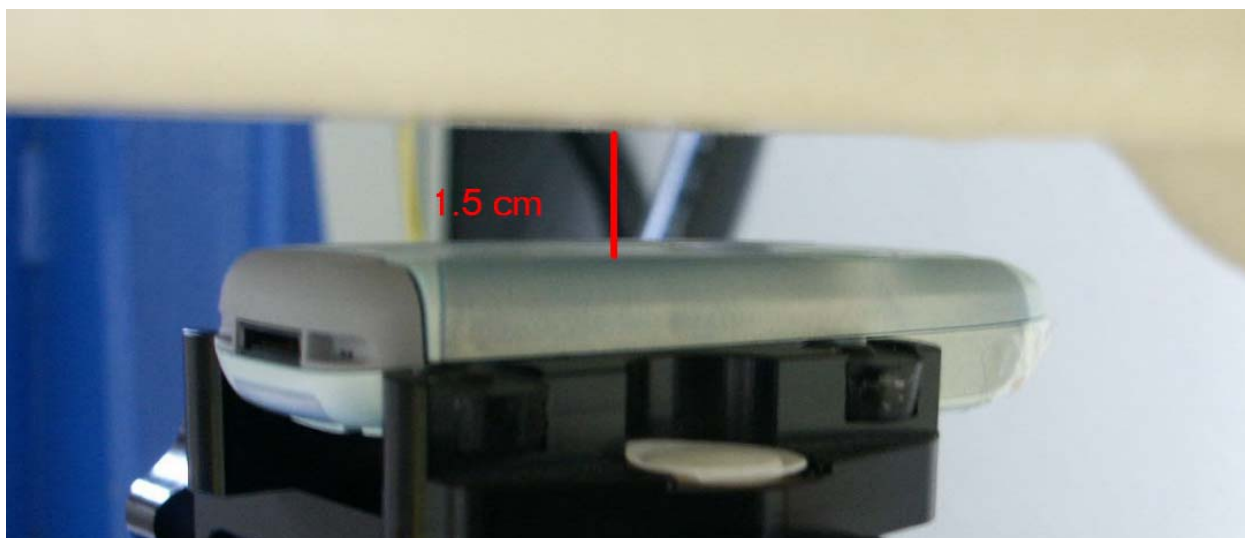
Fig. 24: Body worn configuration, (1 TX slot).
