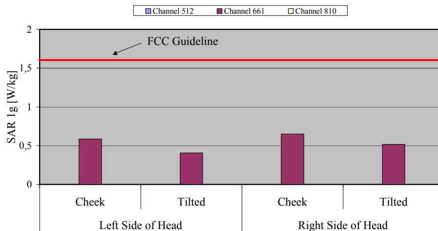
Fig. 8: The measured head phantom SAR values for the Siemens MC60 for PCS 1900 in comparison to the FCC exposure limit.
