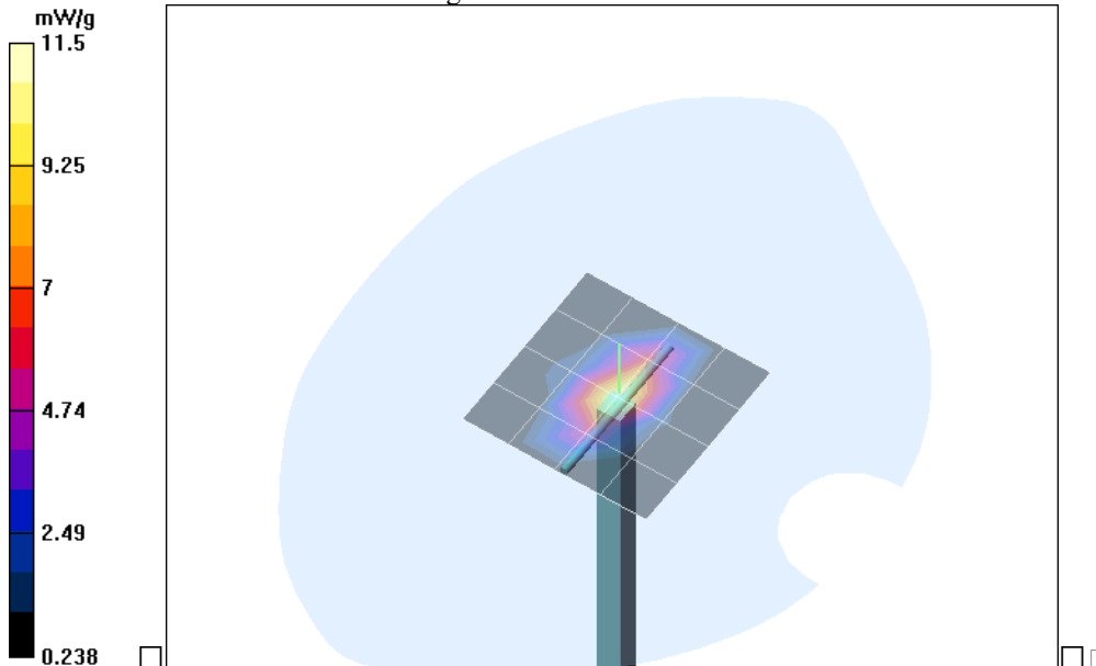
Fig. 11: Validation measurement 1900 MHz body (23.07.2003), coarse grid. Ambient Temperature: 21.3° C, Liquid Temperature: 20.3° C.
