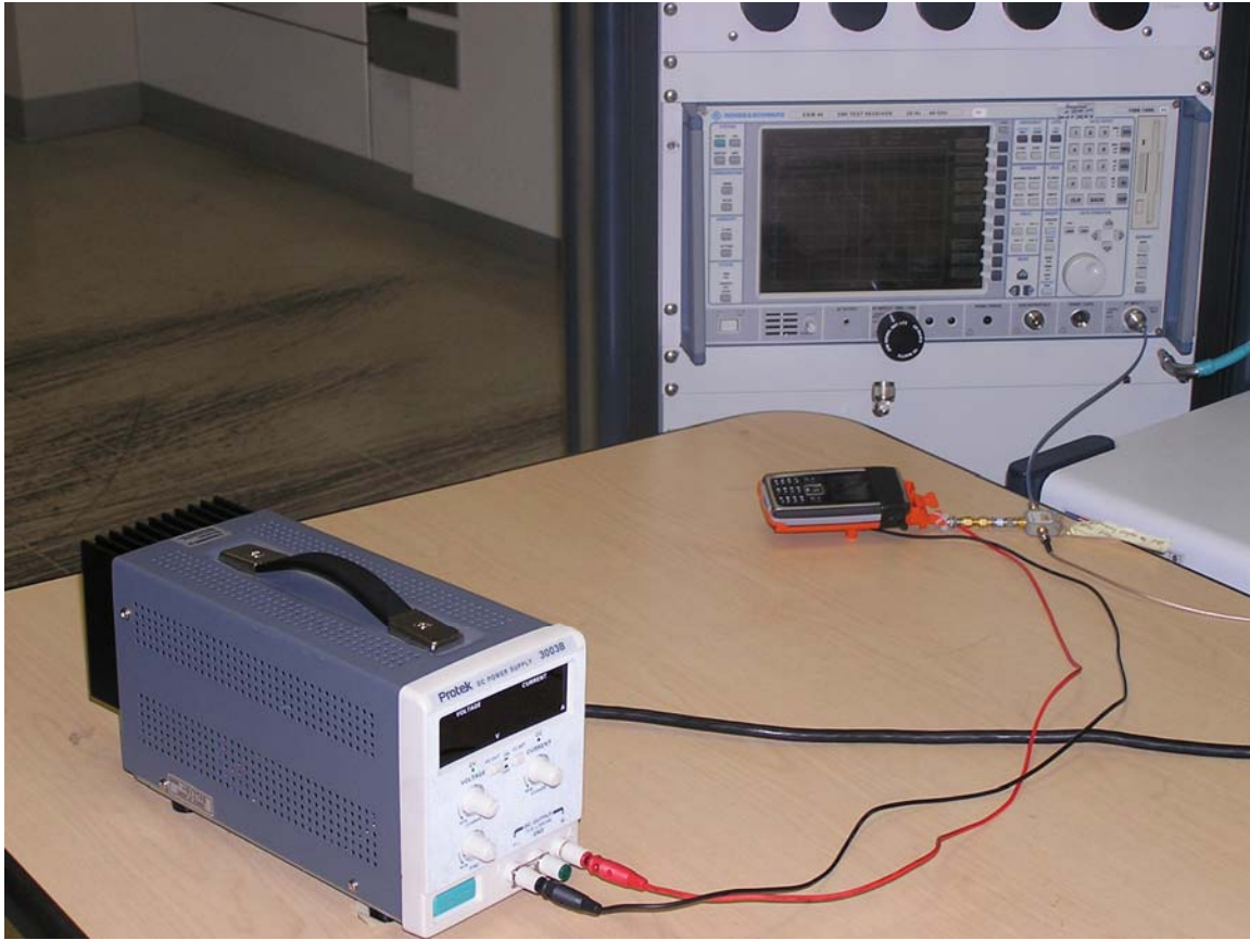
Test setup – Conducted measurements for GSM
