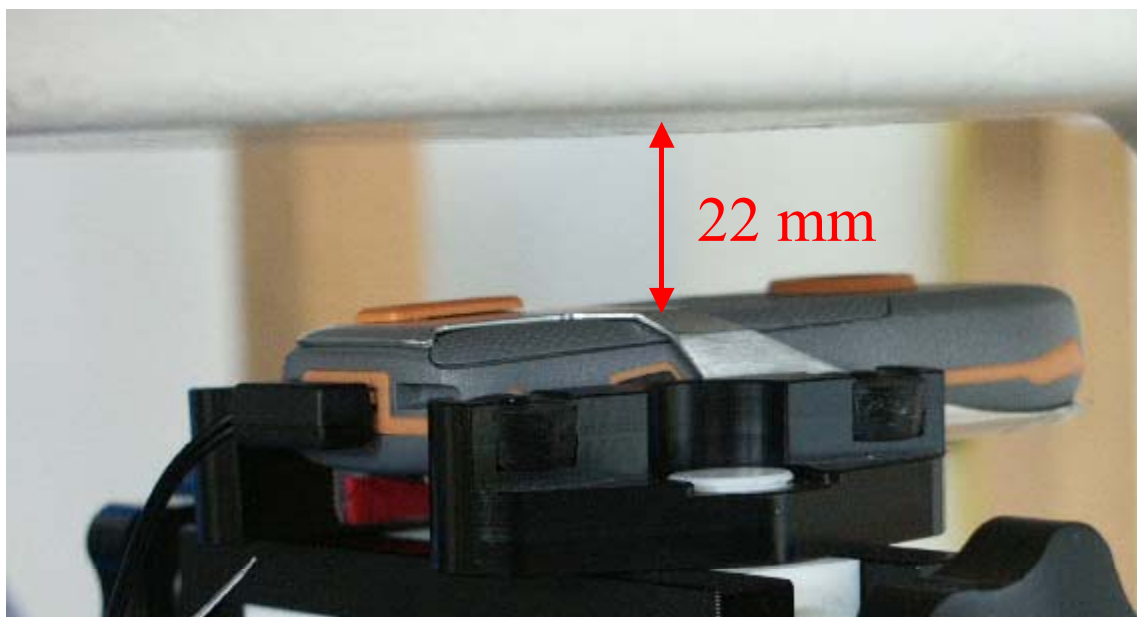
Fig. 27: Body worn configuration, GSM mode (1 TX slot) with headset, antenna towards the phantom.
