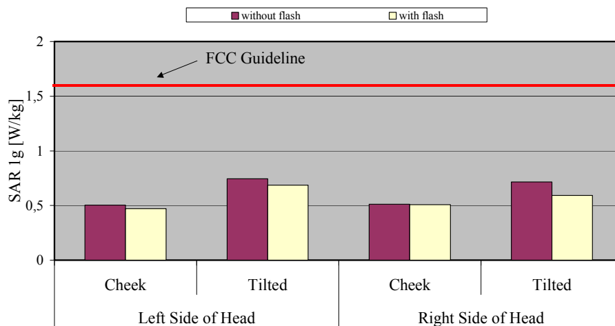
Fig. 8: The measured head phantom SAR values for the Siemens M65 without and with flash for PCS 1900 in comparison to the FCC exposure limit.
