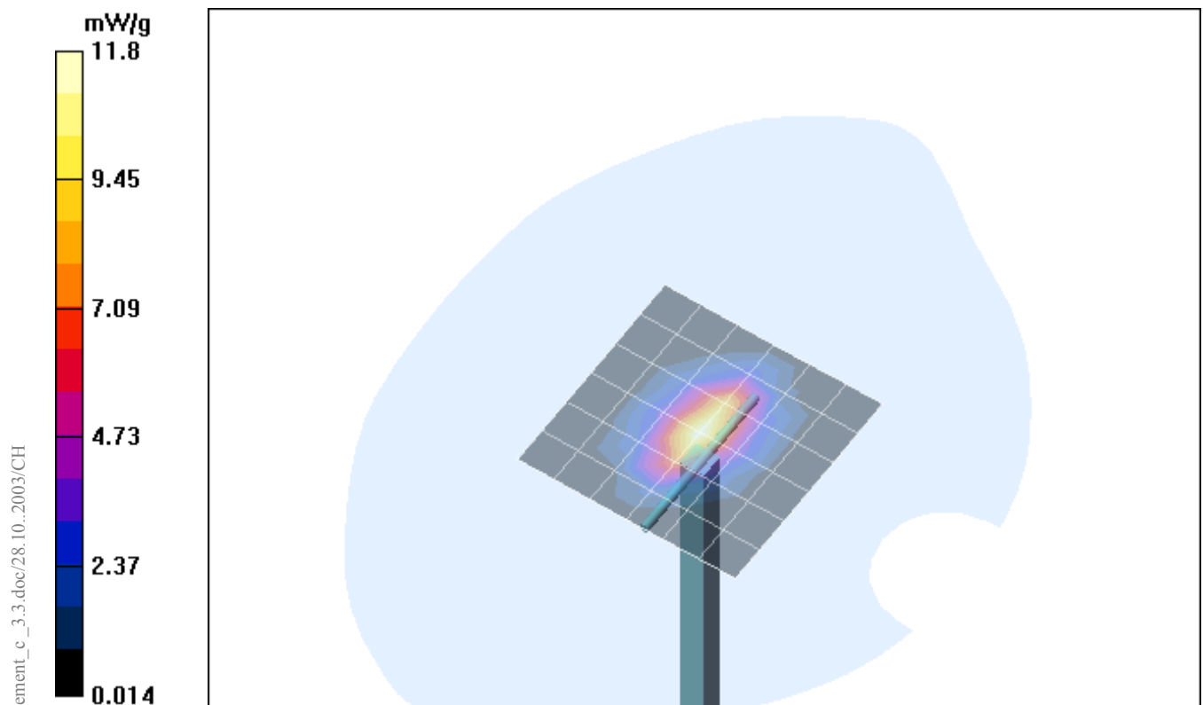
Fig. 10: Validation measurement 1900 MHz Head (March 24, 2004), coarse grid. Ambient Temperature: 21.0° C, Liquid Temperature: 20.0 C.
