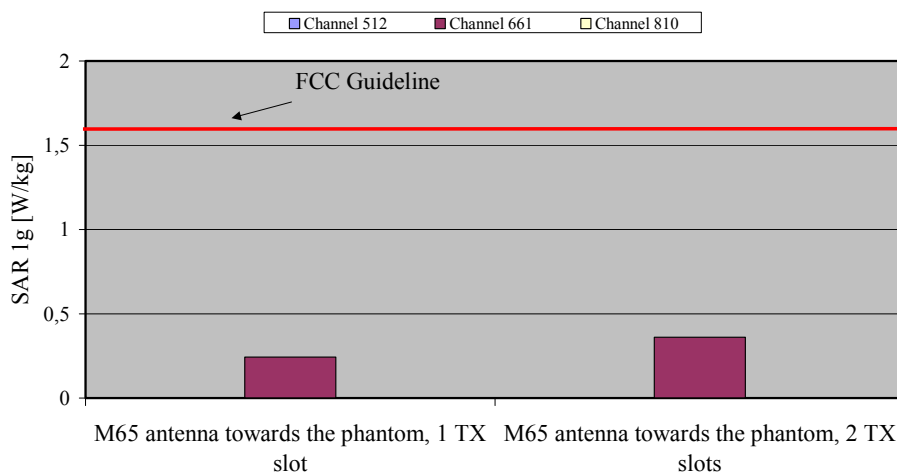
Fig. 9: The measured SAR values in body-worn configuration for the Siemens M65 for PCS 1900 (1 TX and 2 TX slots, gap = 2.2 cm) in comparison to the FCC exposure limit.
