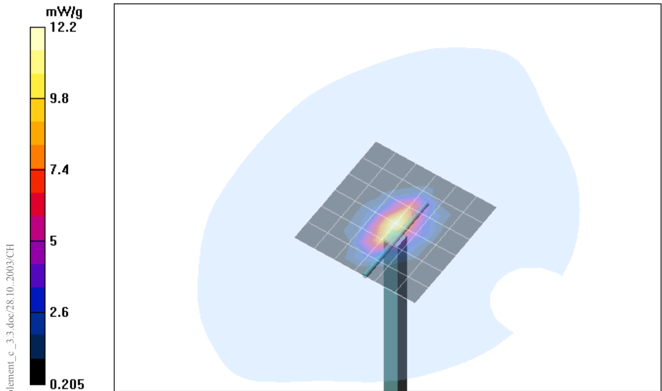
Fig. 11: Validation measurement 1900 MHz body (March 25, 2004), coarse grid. Ambient Temperature: 20.8° C, Liquid Temperature: 20.0° C.
