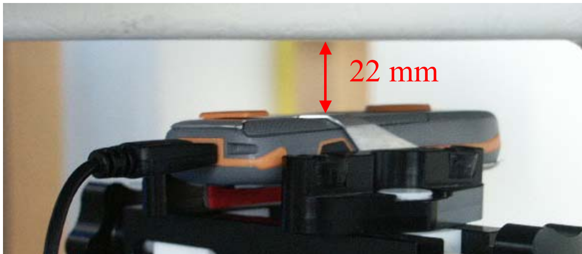
Fig. 26: Body worn configuration, GPRS mode (2 TX slots) with data cable, antenna towards the phantom.
