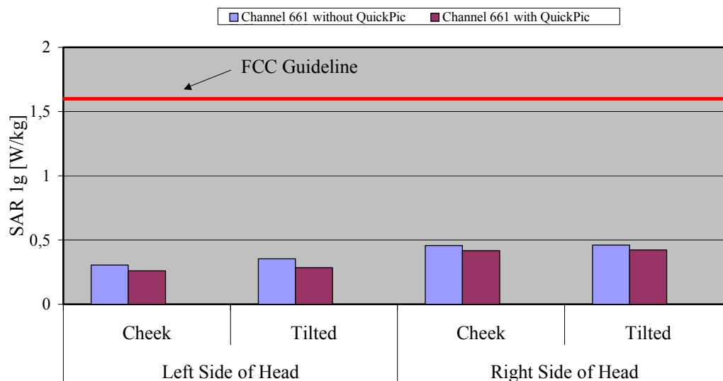
Fig. 10: The measured head phantom SAR values for the Siemens M56 for PCS 1900 in comparison to the FCC exposure limit.
