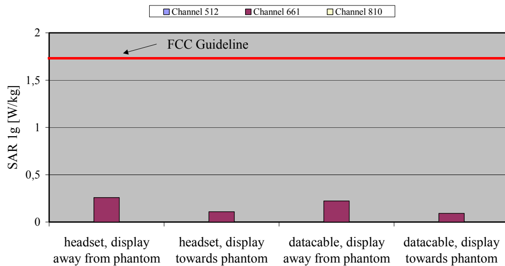
Fig. 12: The measured SAR values in body-worn configuration for the Siemens M56 for PCS 1900 in comparison to the FCC exposure limit.
