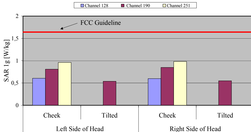
Fig. 8: The measured head phantom SAR values for the Siemens M56 without QuickPic camera for GSM 850 in comparison to the FCC exposure limit.
