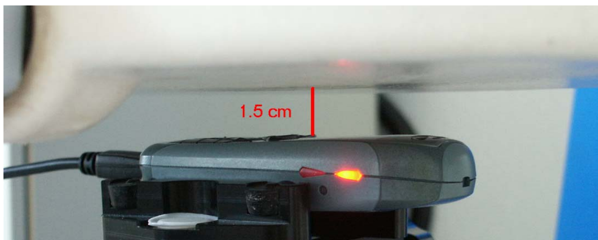
Fig. 33: Body worn configuration, GPRS mode (1 TX slot) with datacable, display towards the phantom.
