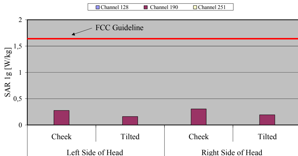
Fig. 9: The measured head phantom SAR values for the Siemens M56 with QuickPic camera for GSM 850 in comparison to the FCC exposure limit.
