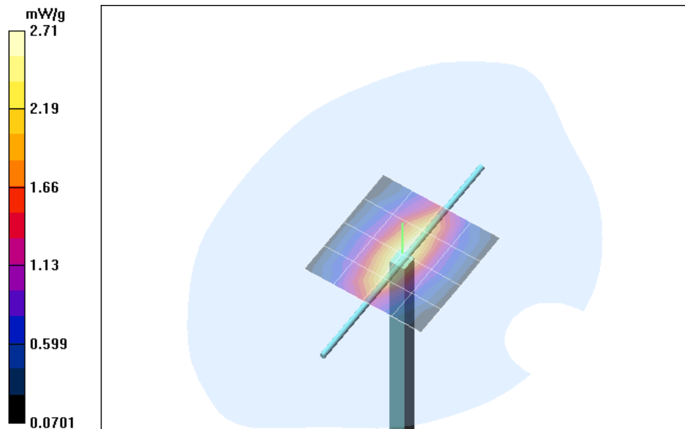
Fig. 14: Validation measurement 850 MHz body (16.07.2003), coarse grid. Ambient Temperature: 32.2° C, Liquid Temperature: 20.9° C.
