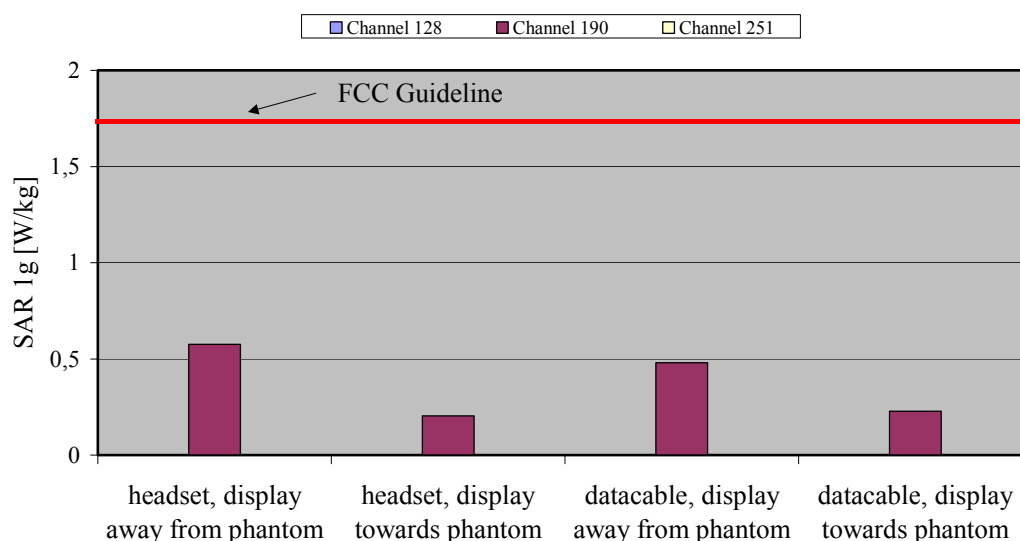
Fig. 11: The measured SAR values in body-worn configuration for the Siemens M56 for GSM 850 in comparison to the FCC exposure limit.
