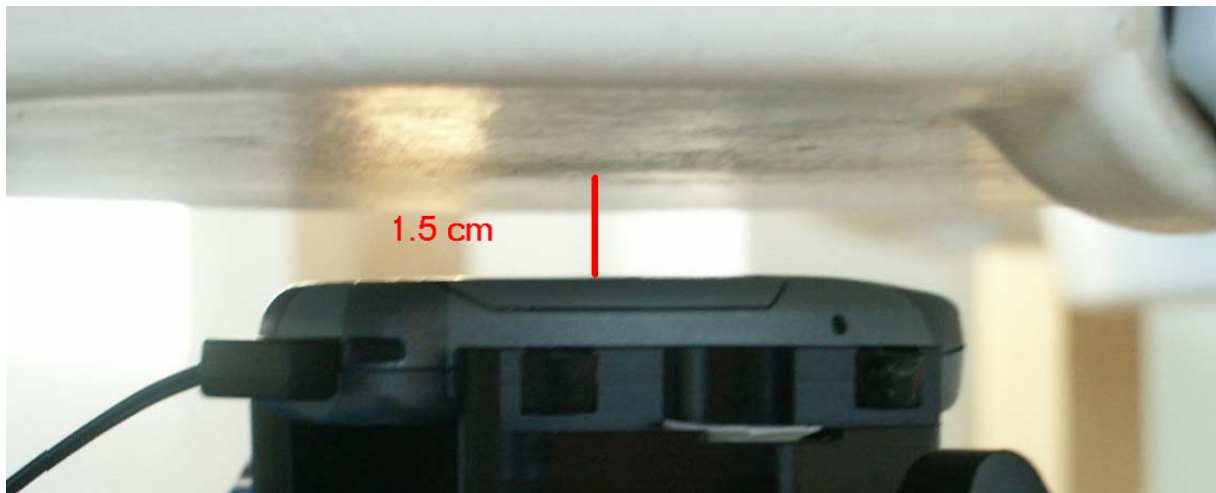
Fig. 30: Body worn configuration, GSM mode (1 TX slot) with headset, display away from phantom.
