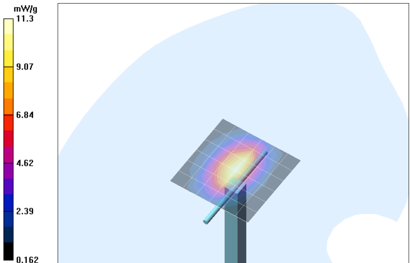
Fig. 10: Validation measurement 1900 MHz Head (March 07, 2006), coarse grid. Ambient Temperature: 22.0° C, Liquid Temperature: 21.0° C.
