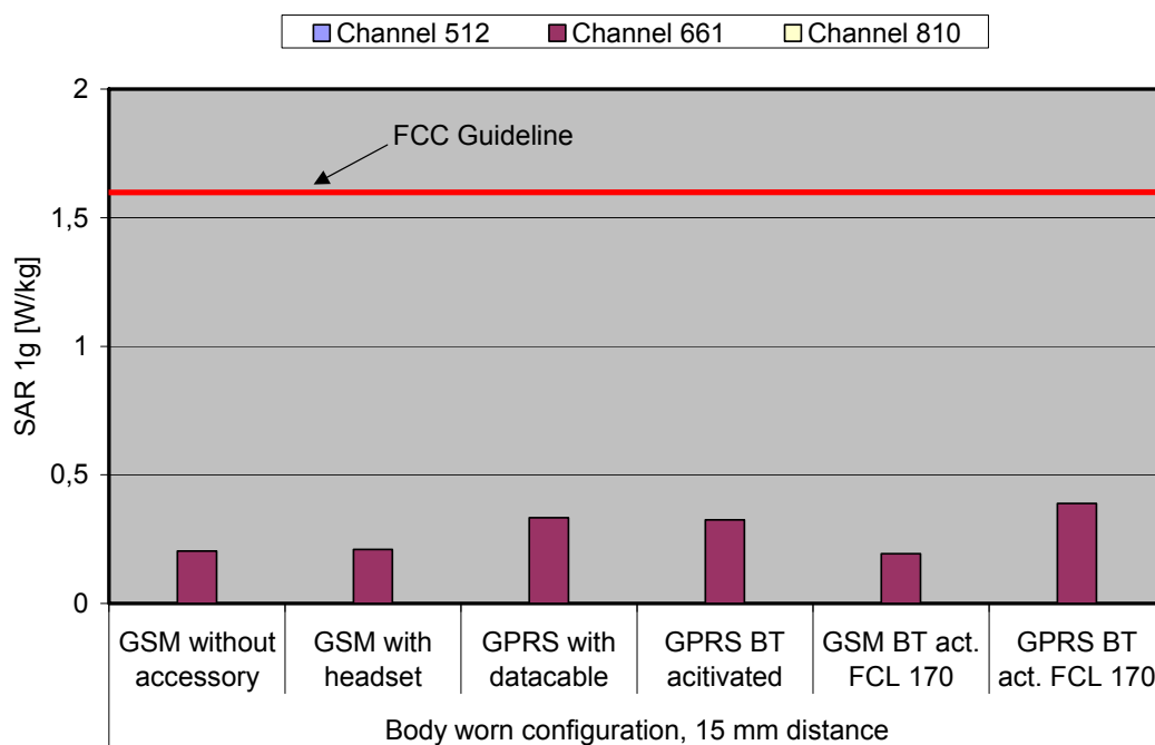
Fig. 9: The measured SAR values in body-worn configuration for the BenQ Siemens EL71 for PCS 1900 in comparison to the FCC exposure limit.
