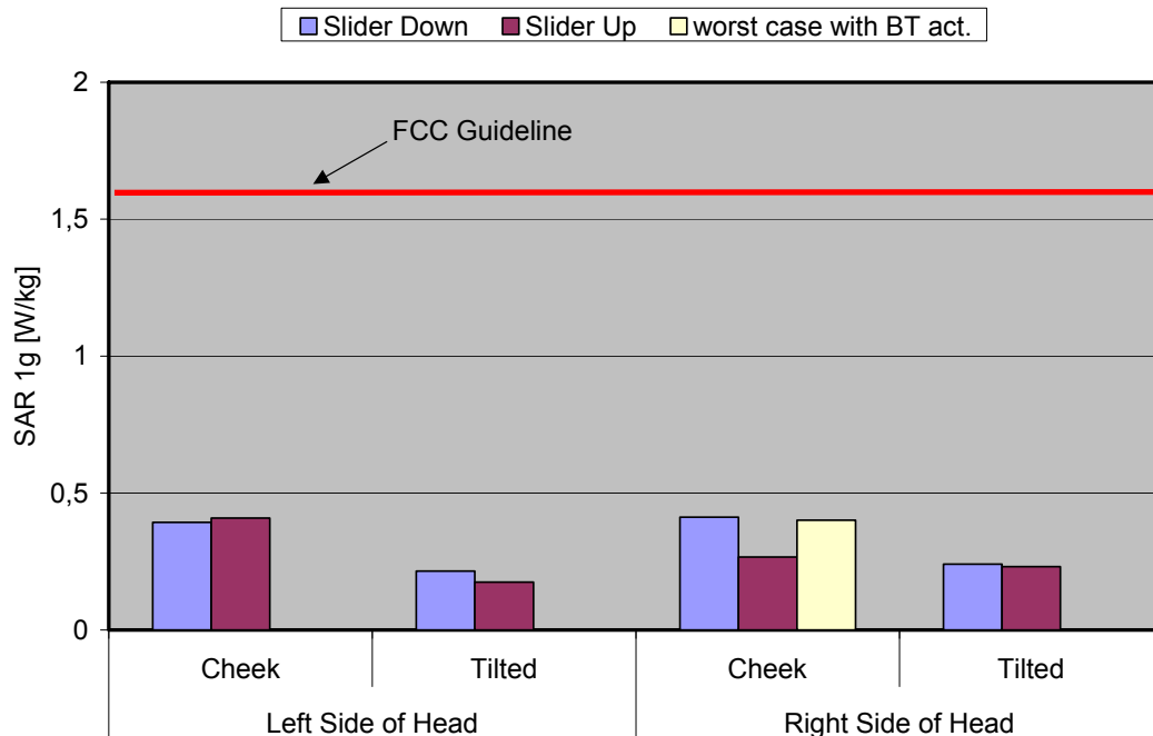
Fig. 8: The measured head phantom SAR values for the BenQ Siemens EL71 for PCS 1900 in comparison to the FCC exposure limit.
