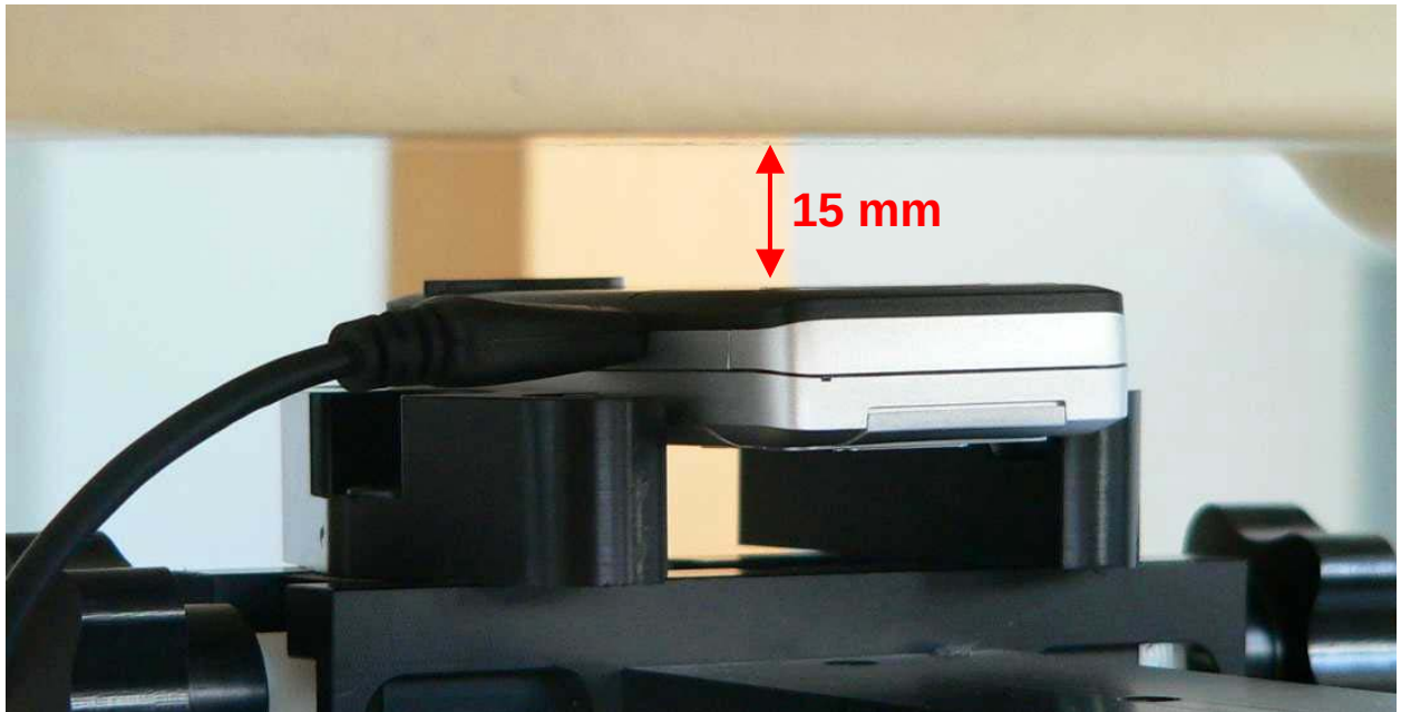
Fig. 32: Body worn configuration BenQ Siemens EL71, GPRS (Class 10), with data cable, antenna towards the phantom, gap= 15 mm.
