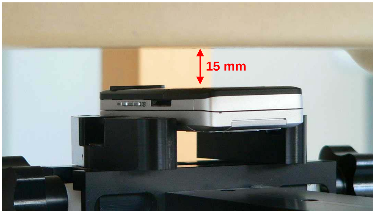
Fig. 30: Body worn configuration BenQ Siemens EL71, GSM mode without accessory, GPRS (Class 10) with BT activated, antenna towards the phantom, gap= 15 mm.
