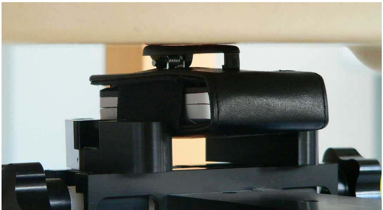
Fig. 33: Body worn configuration BenQ Siemens EL71, GSM and GPRS (Class 10), with leather case FCL-170 and BT activated , antenna towards the phantom.
