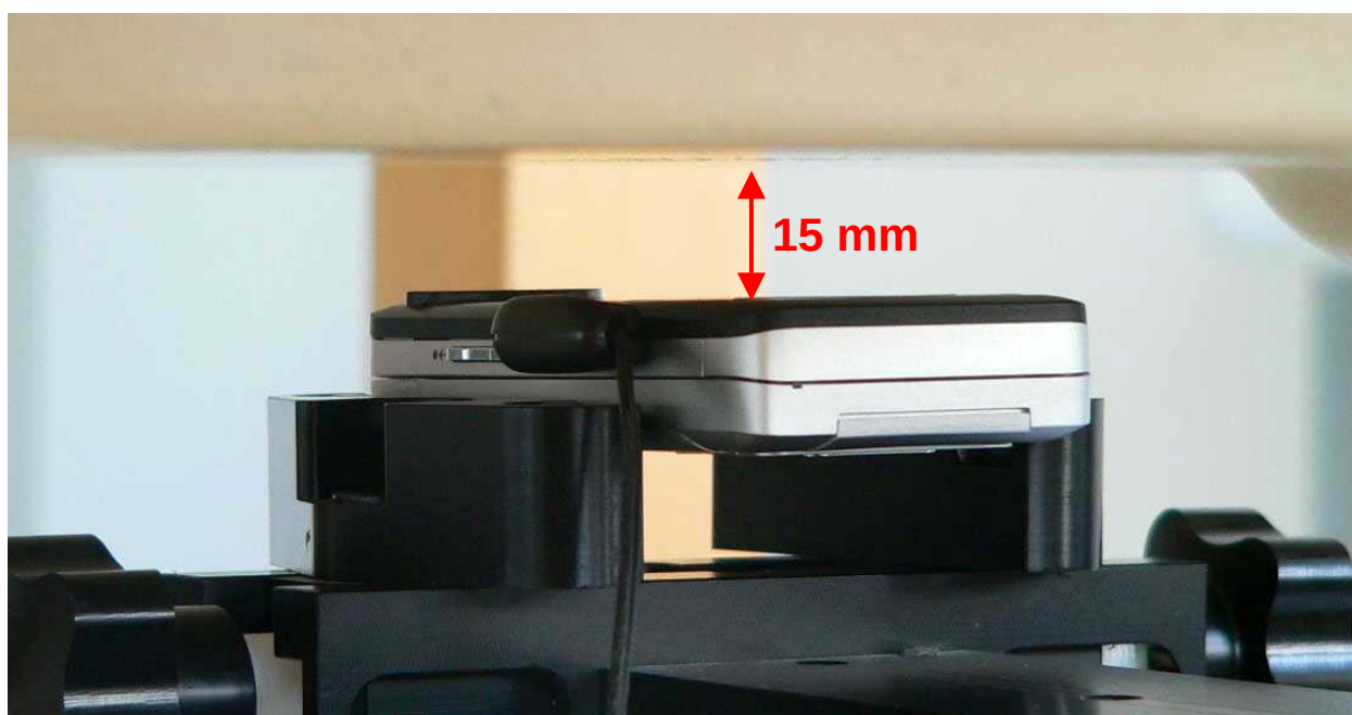
Fig. 31: Body worn configuration BenQ Siemens EL71, GSM mode with headset, antenna towards the phantom, gap= 15 mm.
