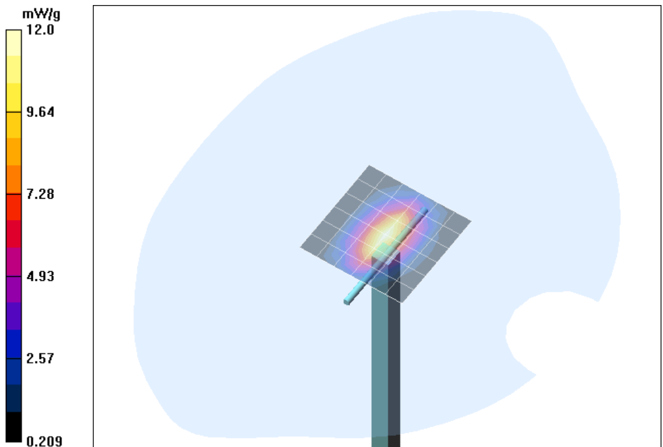
Fig. 11: Validation measurement 1900 MHz body (March 10, 2006), coarse grid. Ambient Temperature: 22.0° C, Liquid Temperature: 21.0° C.
