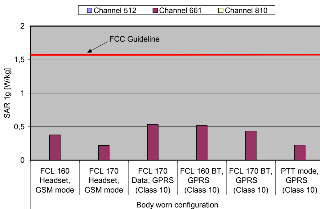
Fig. 9: The measured SAR values in body-worn configuration for the BenQ Siemens EF81 for PCS 1900 in comparison to the FCC exposure limit.
