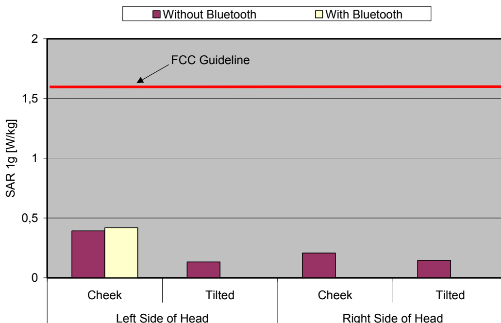
Fig. 8: The measured head phantom SAR values for the BenQ Siemens EF81 for PCS 1900 in comparison to the FCC exposure limit.
