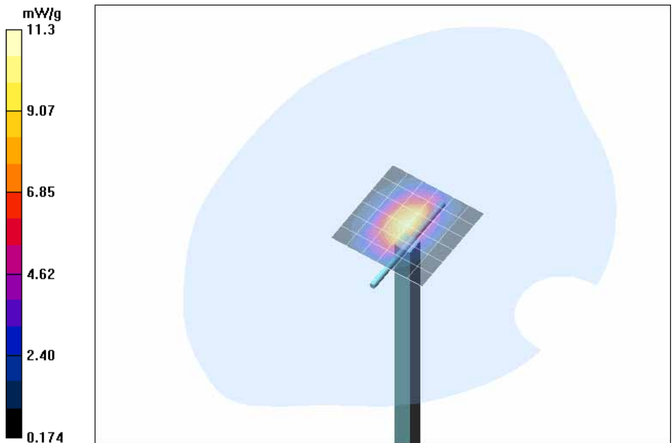
Fig. 10: Validation measurement 1900 MHz Head (January 06, 2006), coarse grid. Ambient Temperature: 21.1° C, Liquid Temperature: 20.5° C.
