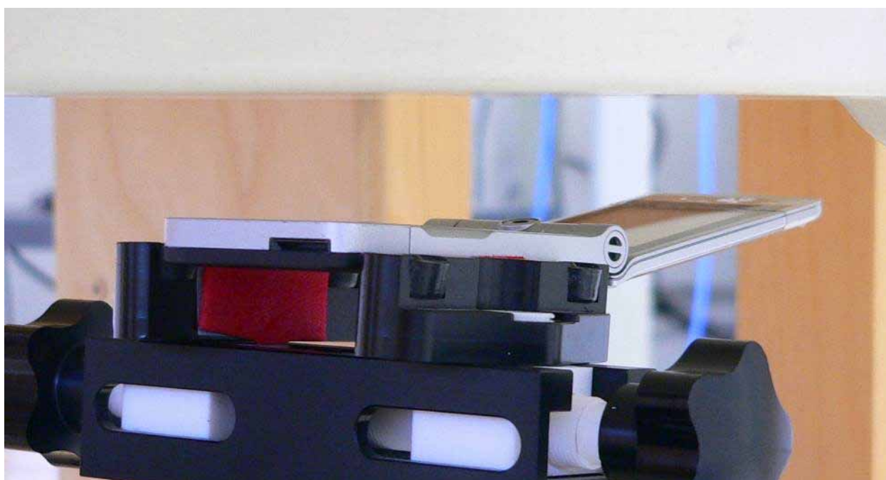
Fig. 27: Body worn configuration, PTT mode (Class 10), display towards the phantom.
