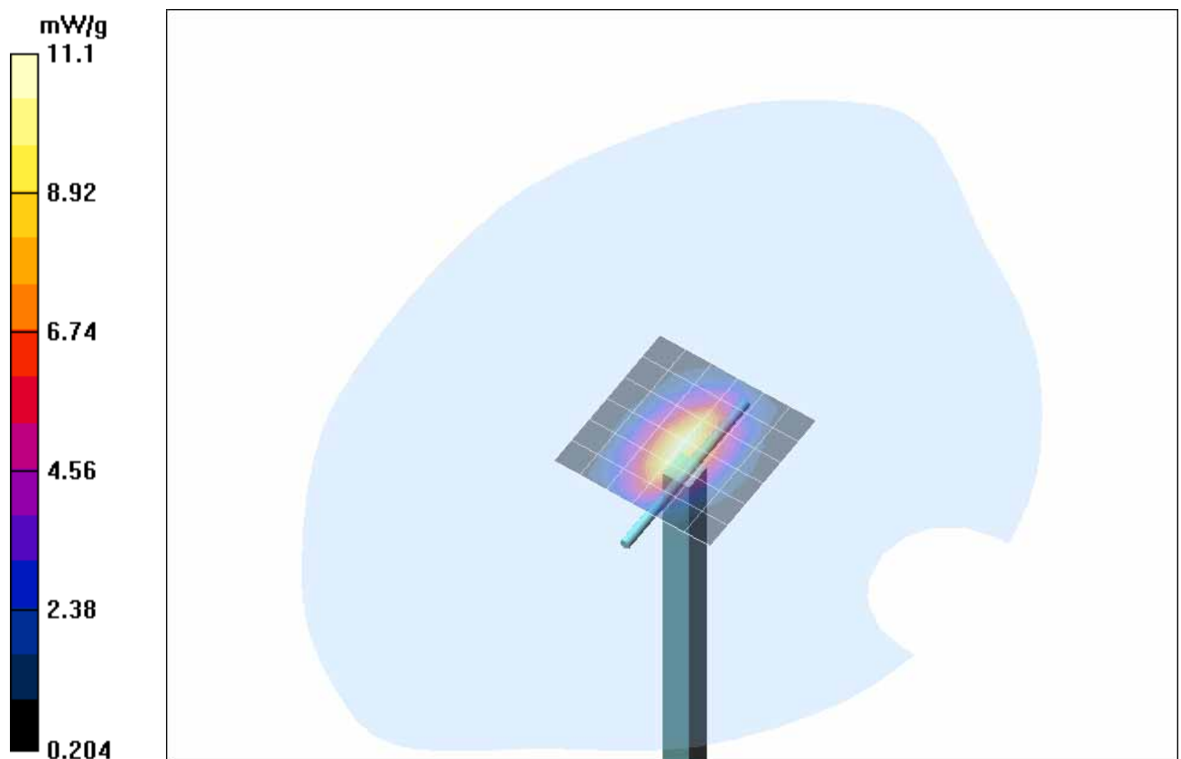
Fig. 11: Validation measurement 1900 MHz body (January 10, 2006), coarse grid. Ambient Temperature: 21.0° C, Liquid Temperature: 20.5° C.
