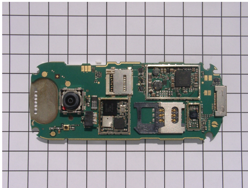
Main PCB, camera side, shielding removed 1 cm Grid
