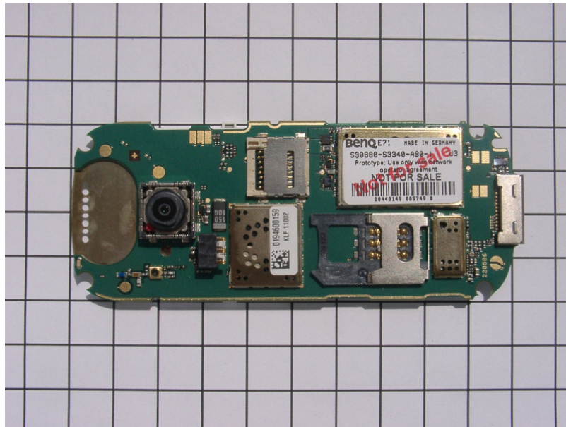
Main PCB, camera side, with shielding 1 cm Grid
