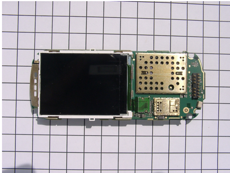
Main PCB, display side, with shielding 1 cm Grid
