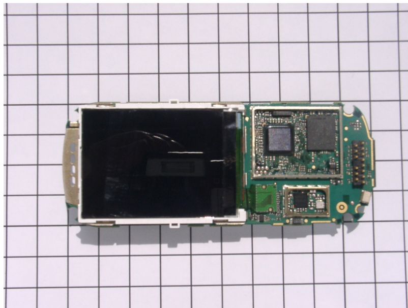
Main PCB, display side, shielding removed 1 cm Grid
