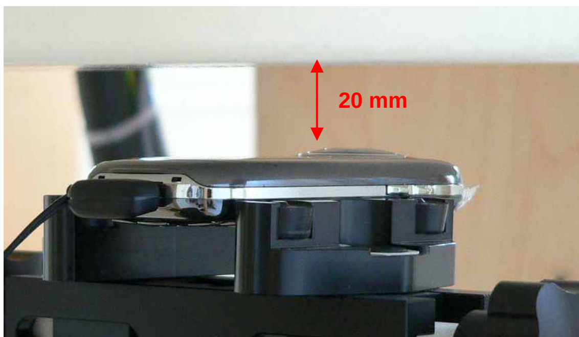
Fig. 25: Body worn configuration BenQ Siemens E71, GSM mode with headset, antenna towards the phantom, gap = 20 mm.
