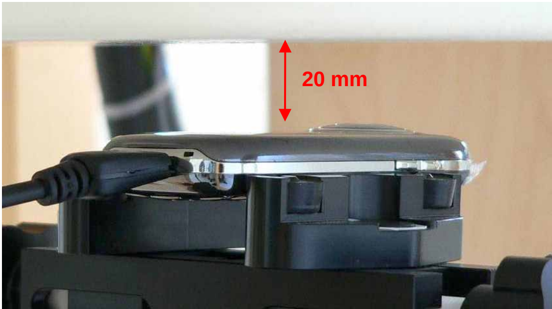
Fig. 26: Body worn configuration BenQ Siemens E71, GPRS (Class 10), with data cable, antenna towards the phantom, gap = 20 mm.
