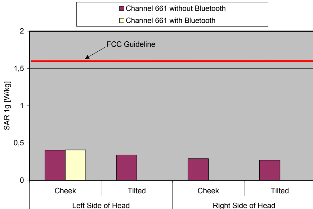
Fig. 8: The measured head phantom SAR values for the BenQ Siemens E71 for PCS 1900 in comparison to the FCC exposure limit.
