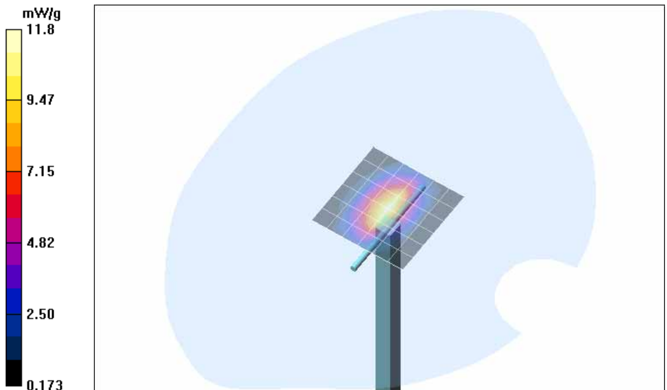
Fig. 11: Validation measurement 1900 MHz body (July 18, 2006), coarse grid. Ambient Temperature: 22.3° C, Liquid Temperature: 21.6° C.
