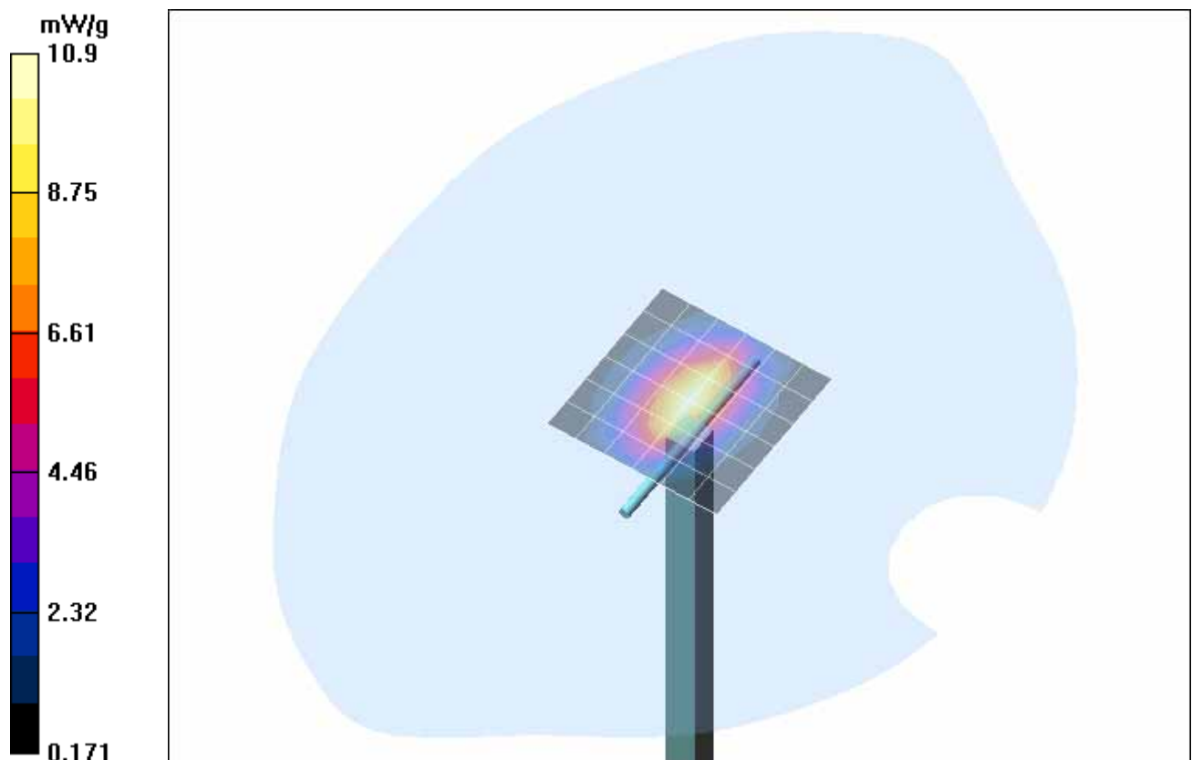
Fig. 10: Validation measurement 1900 MHz Head (July 18, 2006), coarse grid. Ambient Temperature: 22.1° C, Liquid Temperature: 21.3° C.
