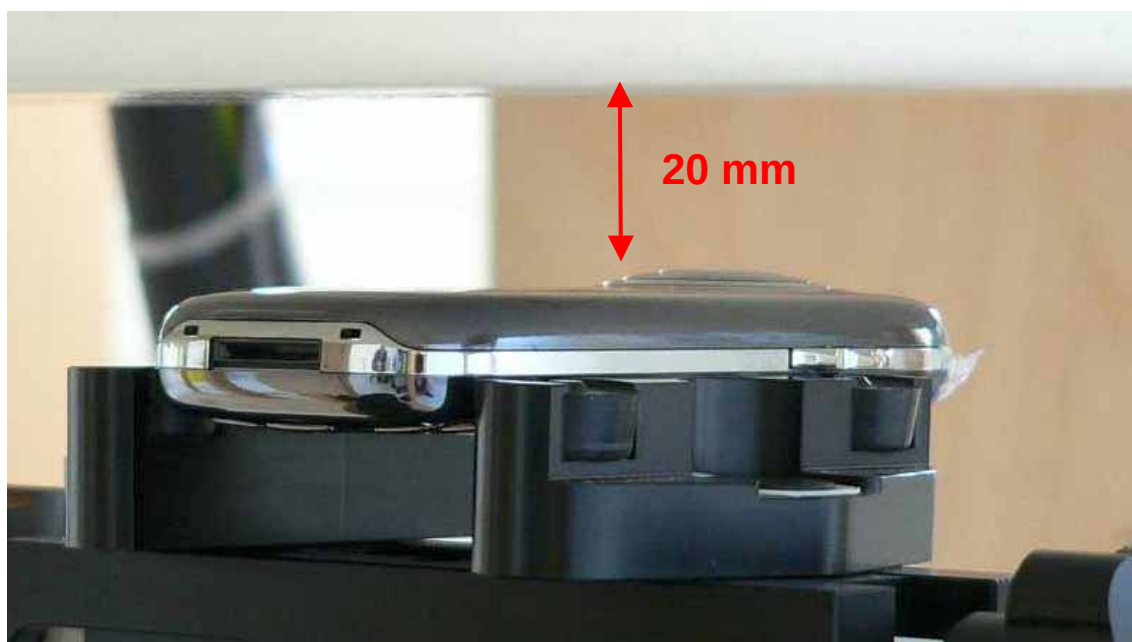
Fig. 24: Body worn configuration BenQ Siemens E71, GSM mode without accessory, with and without Bluetooth activated, antenna towards the phantom, gap = 20 mm.
