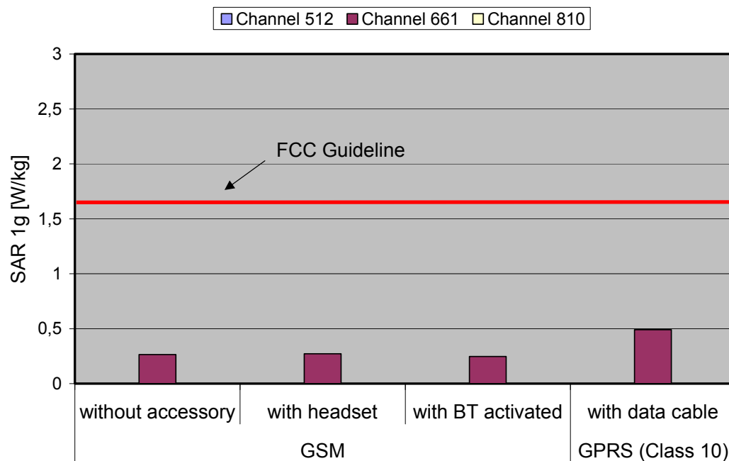
Fig. 8: The measured head phantom SAR values for the BenQ Siemens E71 for PCS 1900 in comparison to the FCC exposure limit.
