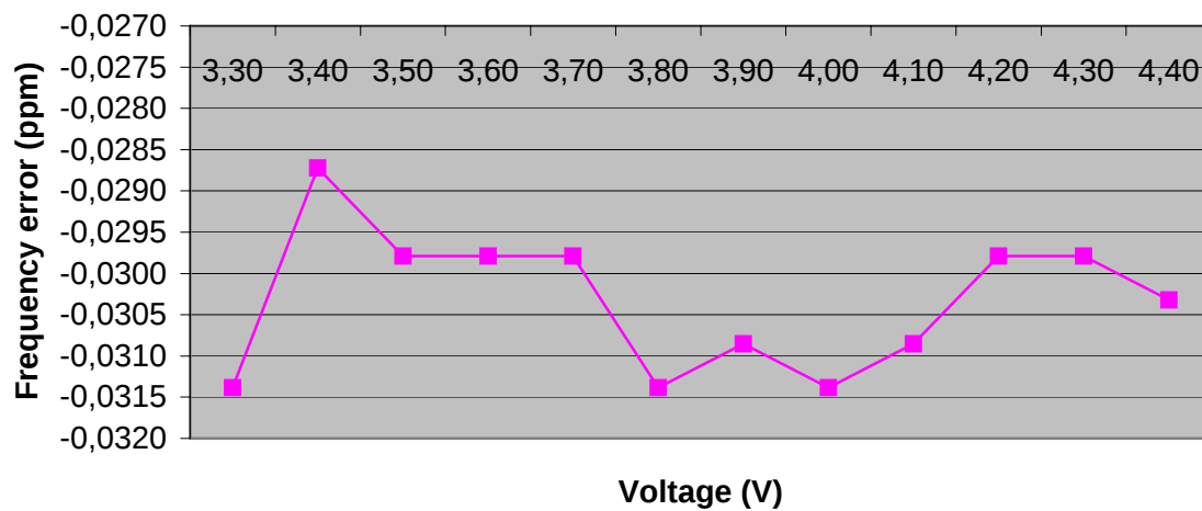
Frequency Error vs. Voltage
