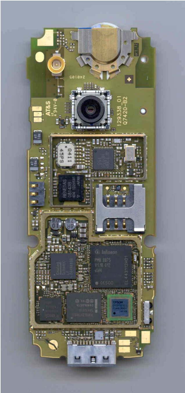
CX75 PCB Back View Shields Removed
