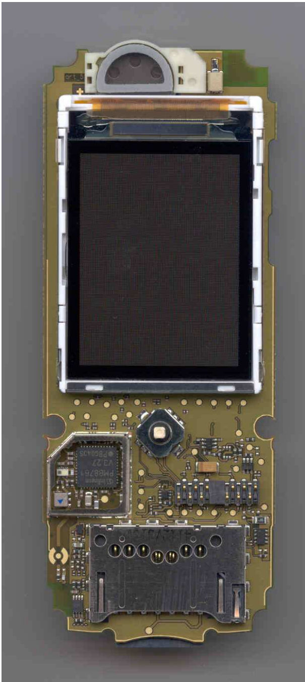
CX75 PCB Front View Shields Removed
