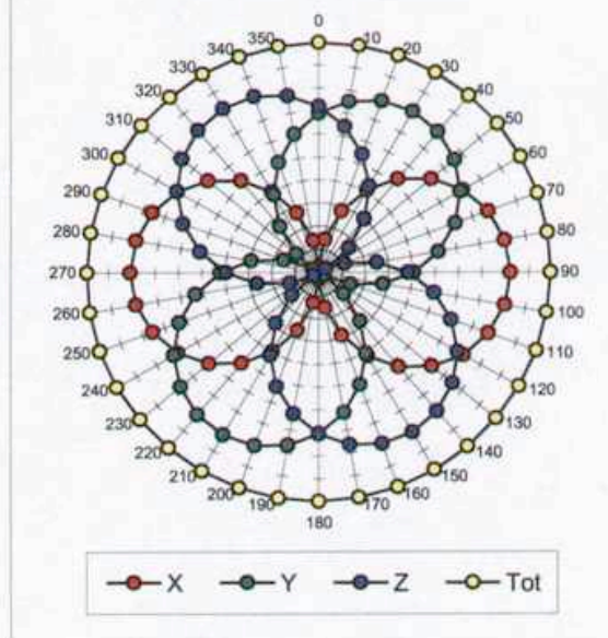
f = 1800 MHz, WG R22
