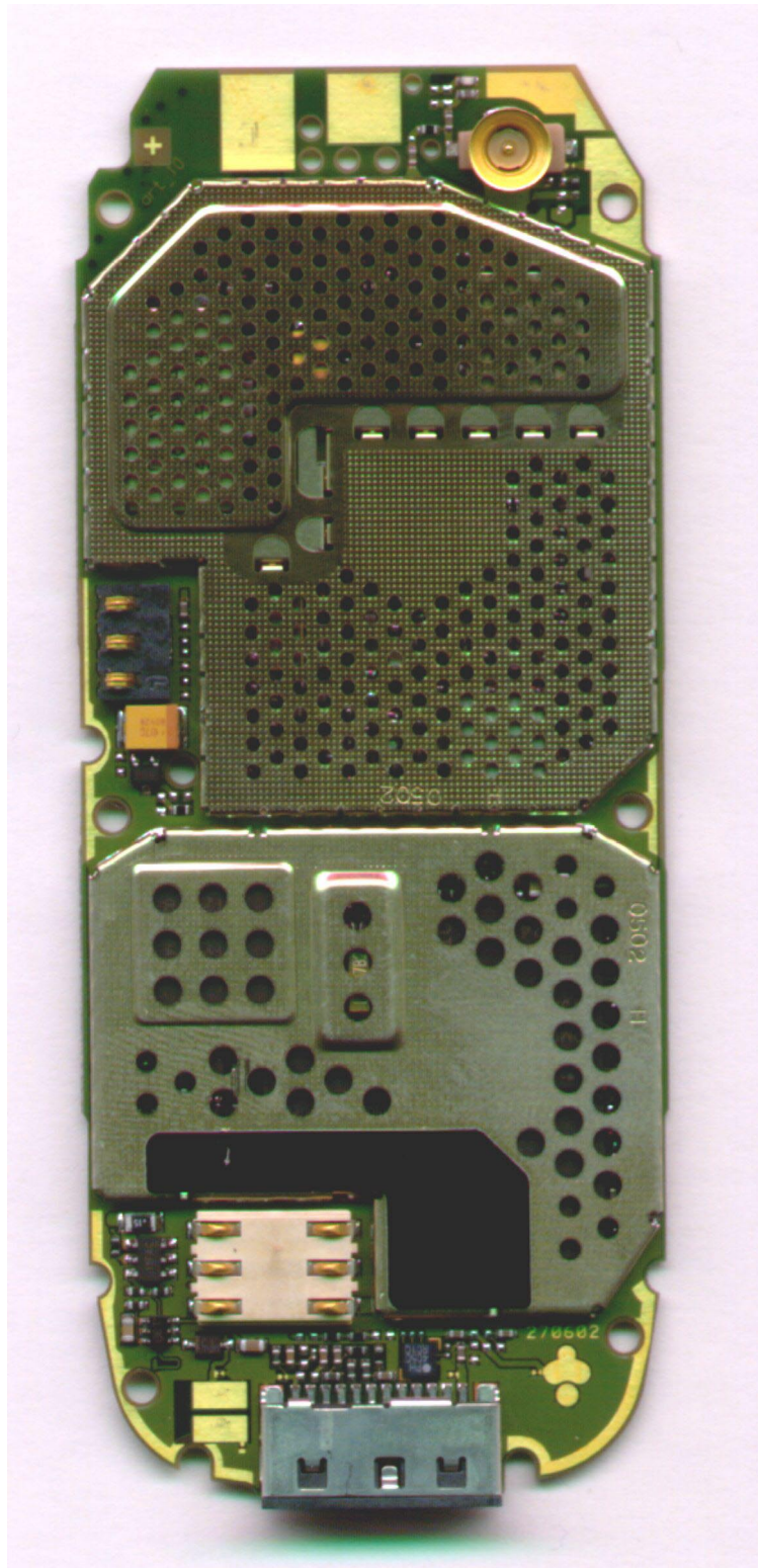
C56 Board with shielding, side 2
