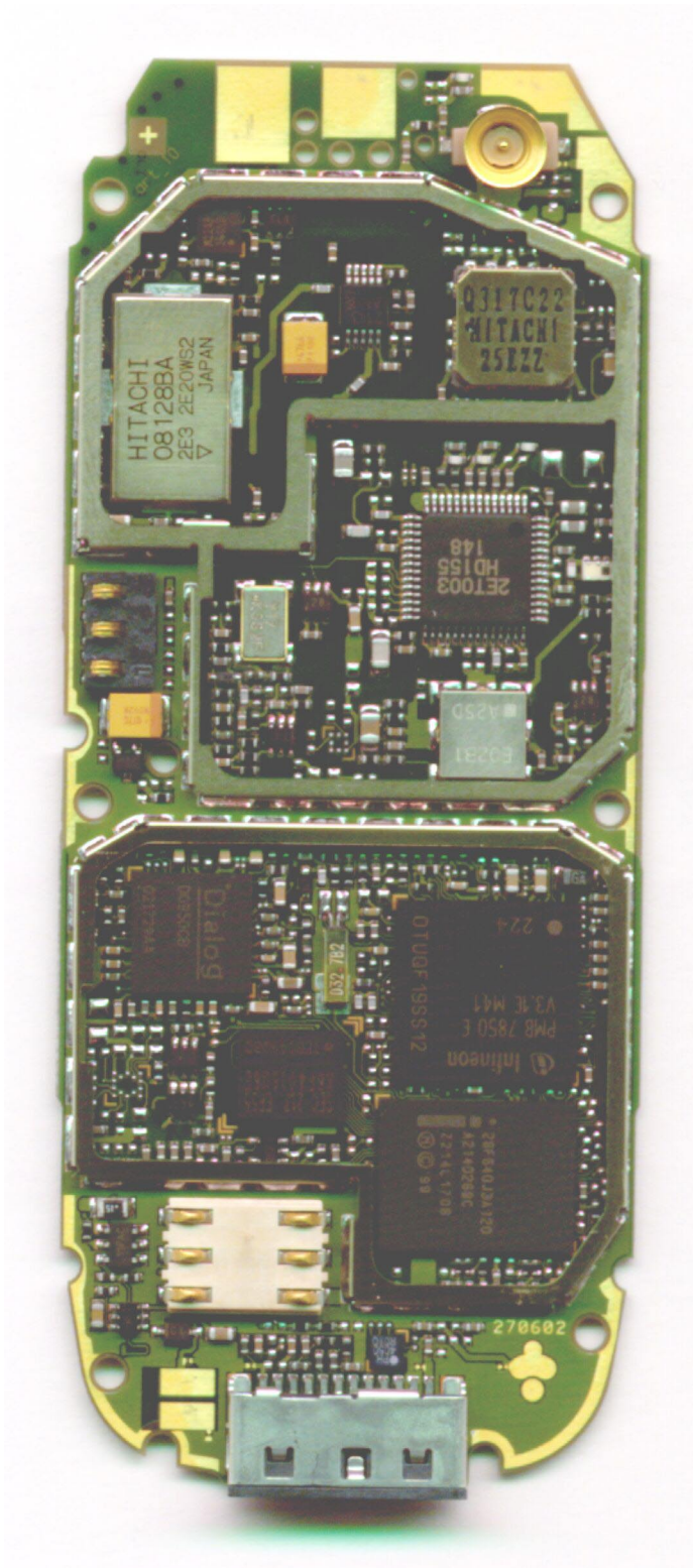
C56 Board without shielding, side 2
