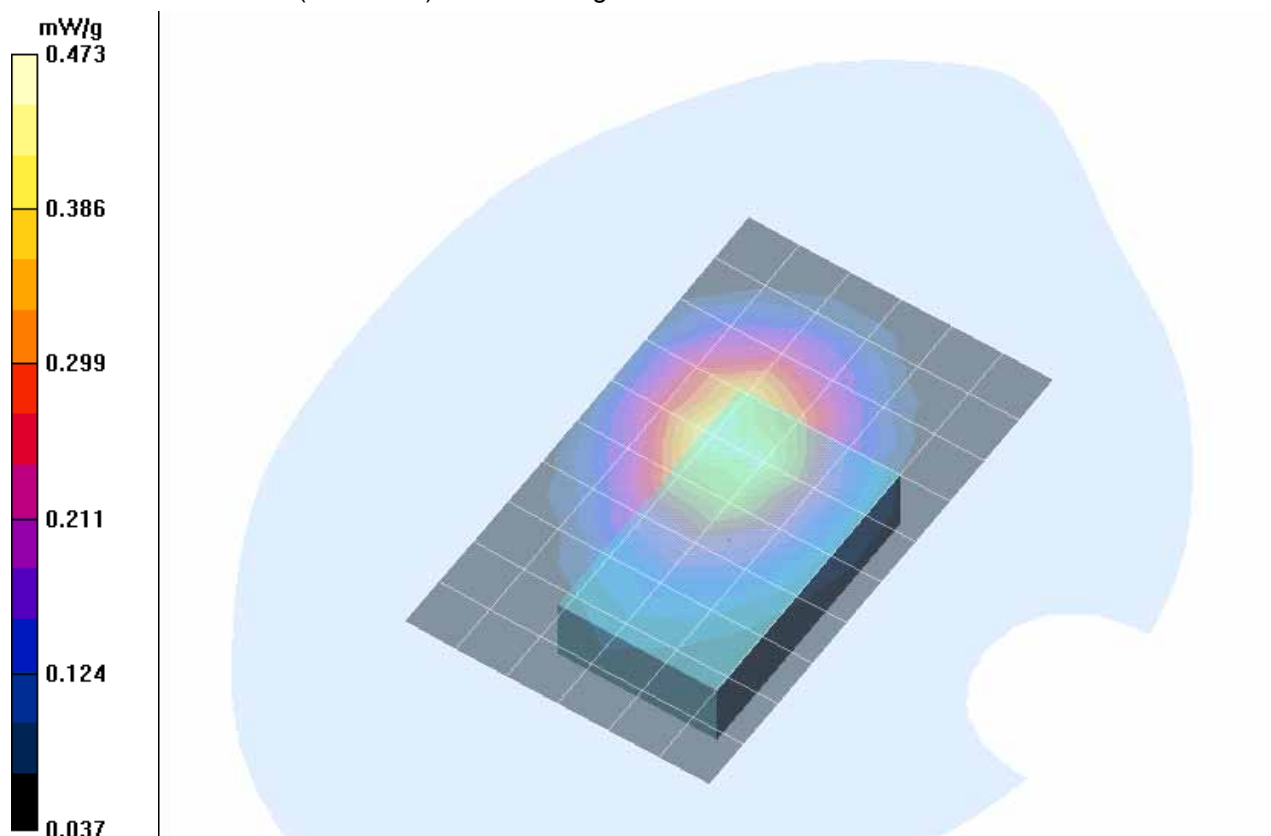
Fig. 28: SAR distribution for GPRS 850, channel 190, body worn configuration, antenna towards the phantom, with data cable, 15 mm distance (August 22, 2005; Ambient Temperature: 22.3° C; Liquid Temperature: 21.3° C).
