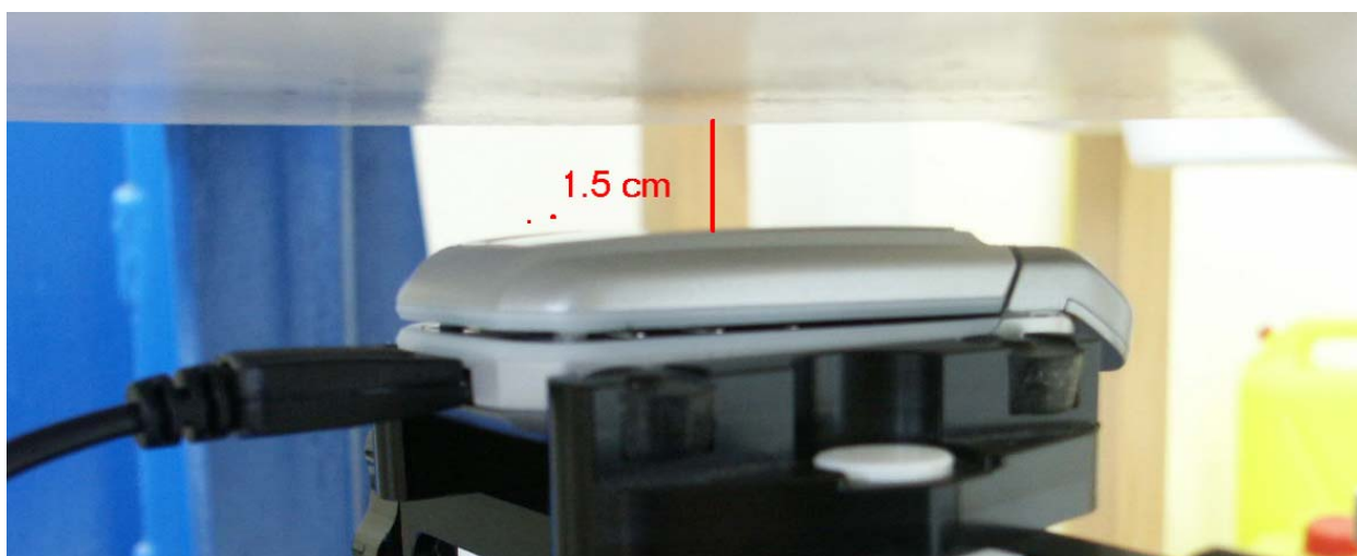
Fig. 28: Body worn configuration, GPRS mode (2 TX slots) with datacable, battery towards the ground.
