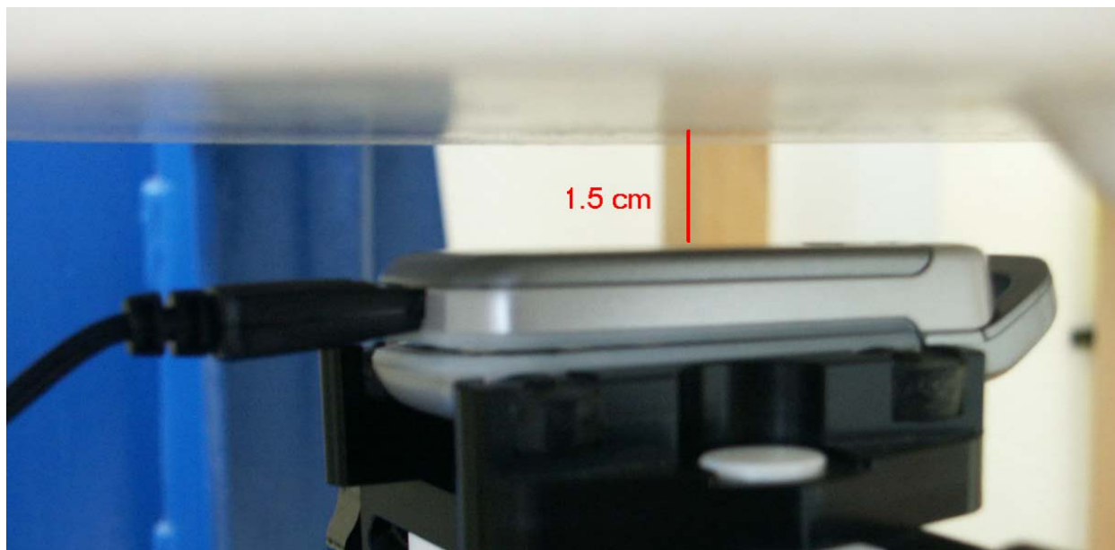
Fig. 27: Body worn configuration, GPRS mode (2 TX slots) with datacable, battery towards the phantom.
