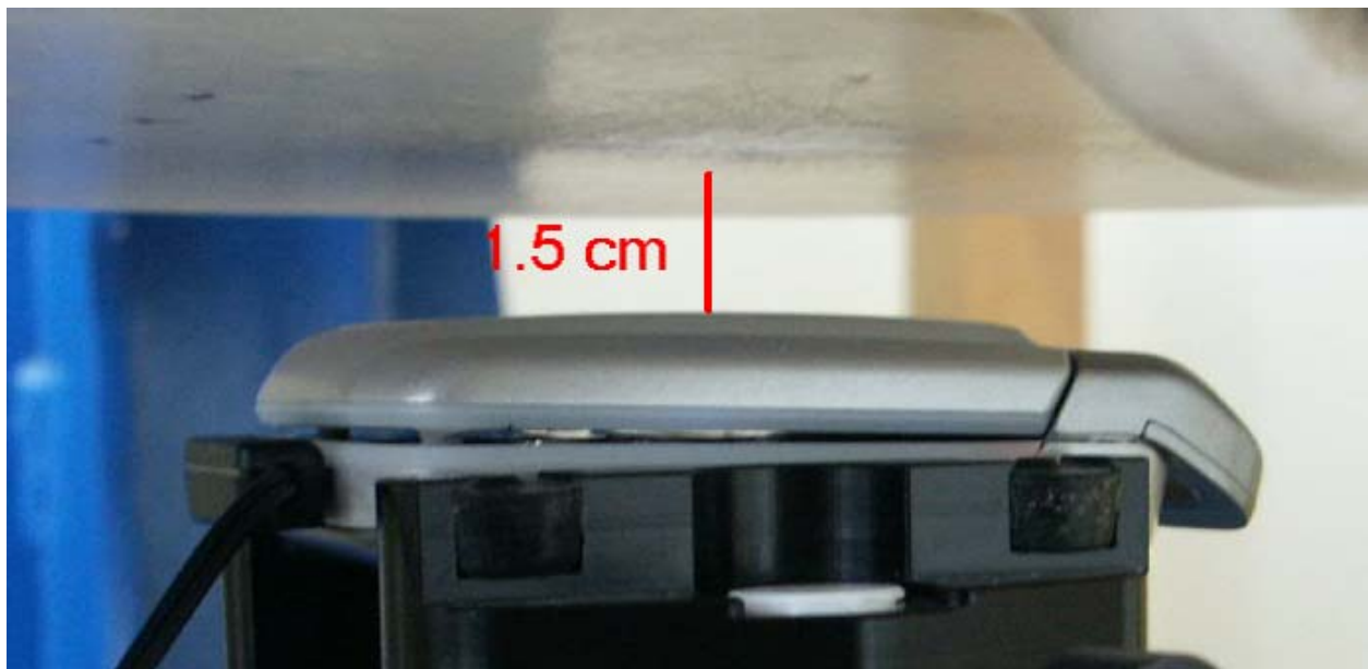
Fig. 30: Body worn configuration, GSM mode (1 TX slot) with headset, battery towards the ground.
