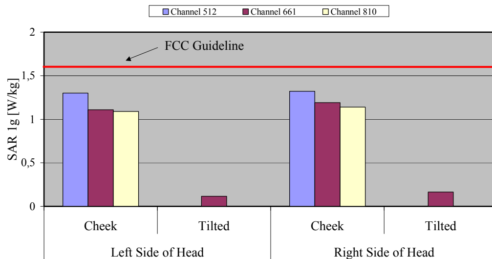
Fig. 9: The measured head phantom SAR values for the Siemens CF62 with camera for PCS 1900 in comparison to the FCC exposure limit.
