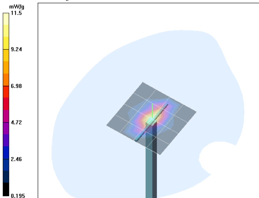
Fig. 11: Validation measurement 1900 MHz Head (February 10, 2004), coarse grid. Ambient Temperature: 19.8° C, Liquid Temperature: 19.5° C.
