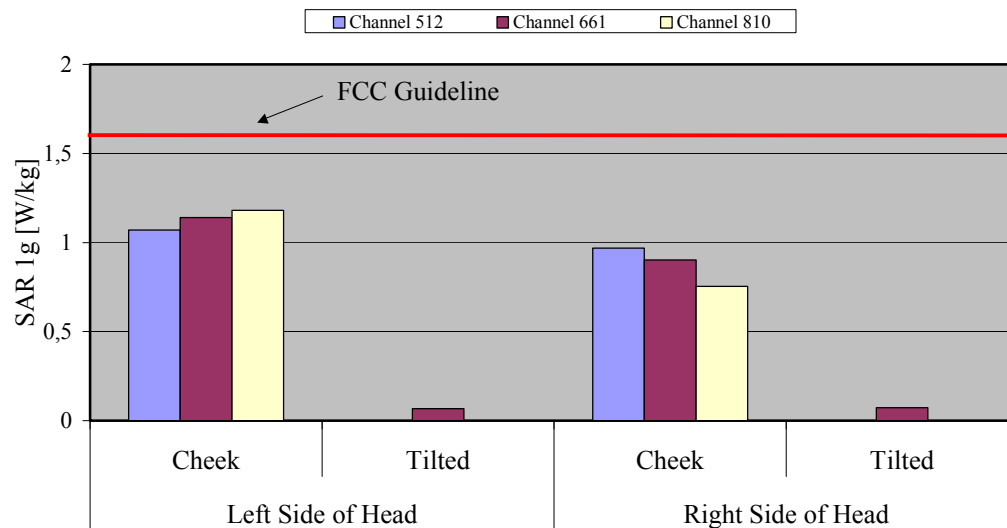
Fig. 8: The measured head phantom SAR values for the Siemens CF62 without camera for PCS 1900 in comparison to the FCC exposure limit.
