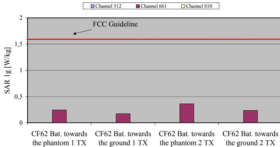
Fig. 10: The measured SAR values in body-worn configuration for the Siemens CF62 for PCS 1900 (1 TX and 2 TX slots, gap = 1.5 cm) in comparison to the FCC exposure limit.
