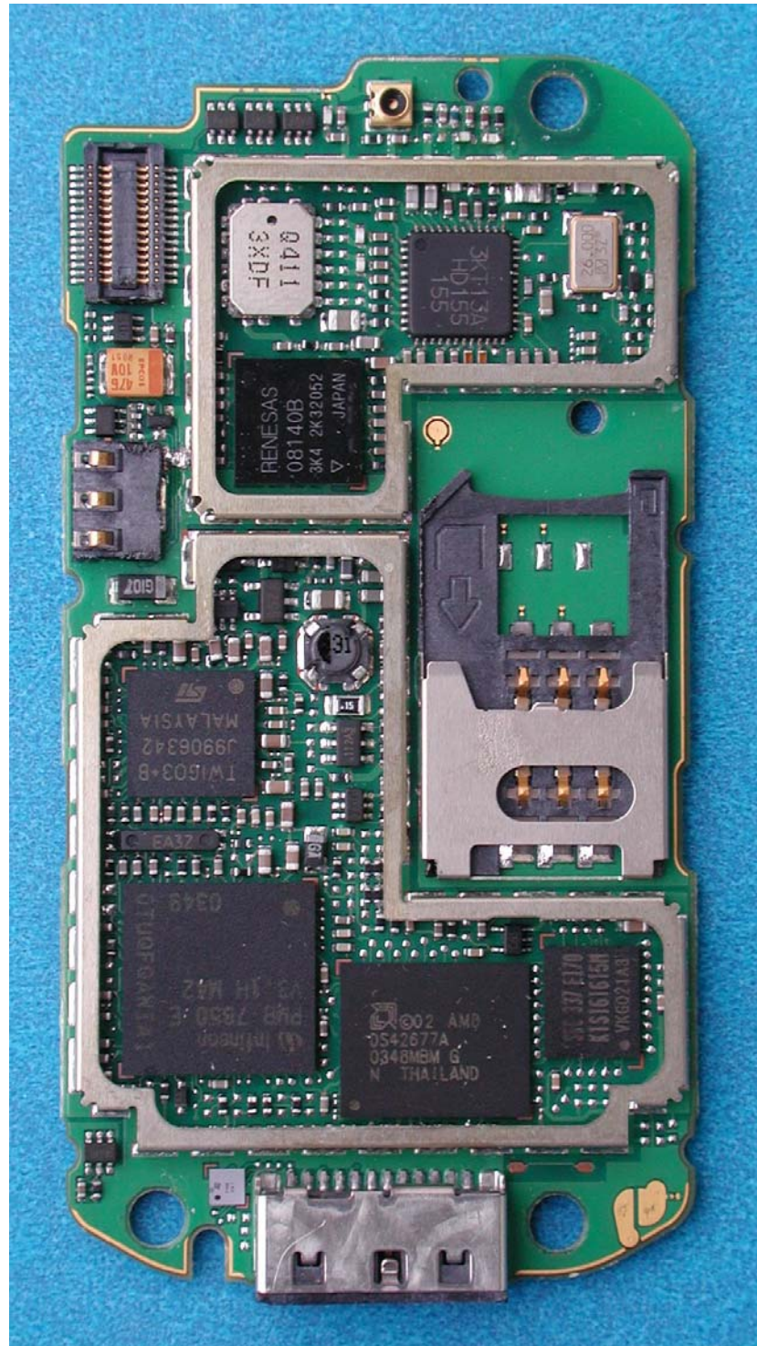
CF62 PCB Rear View Shields Removed
