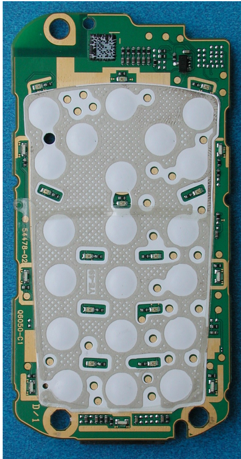
CF62 PCB Front View Keypad Removed
