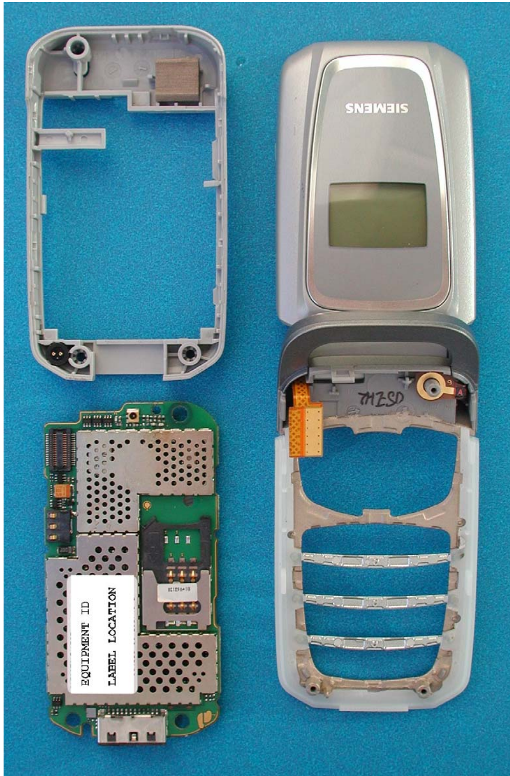
CF62 Disassembly
