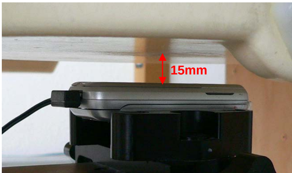
Fig. 34: Body worn configuration, GSM with headset, slider down, antenna towards the phantom, 15mm distance.
