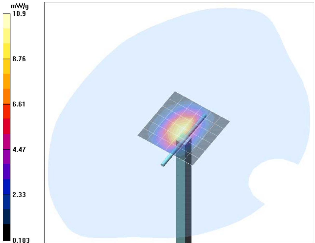
Fig. 11: Validation measurement 1900 MHz Head (August 08, 2005), coarse grid. Ambient Temperature: 22.0° C, Liquid Temperature: 21.0° C.
