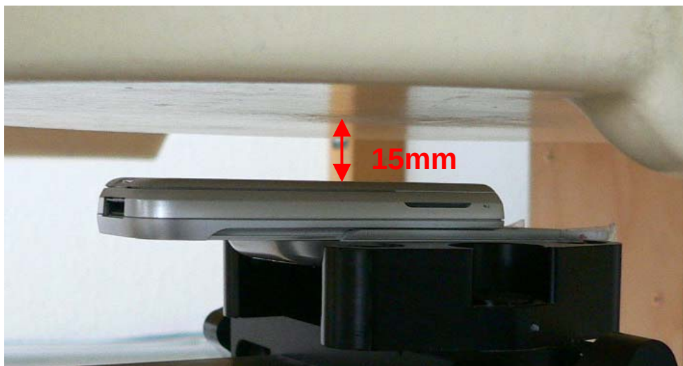
Fig. 30: Body worn configuration, GSM without accessory, slider up, antenna towards the phantom, 15mm distance.
