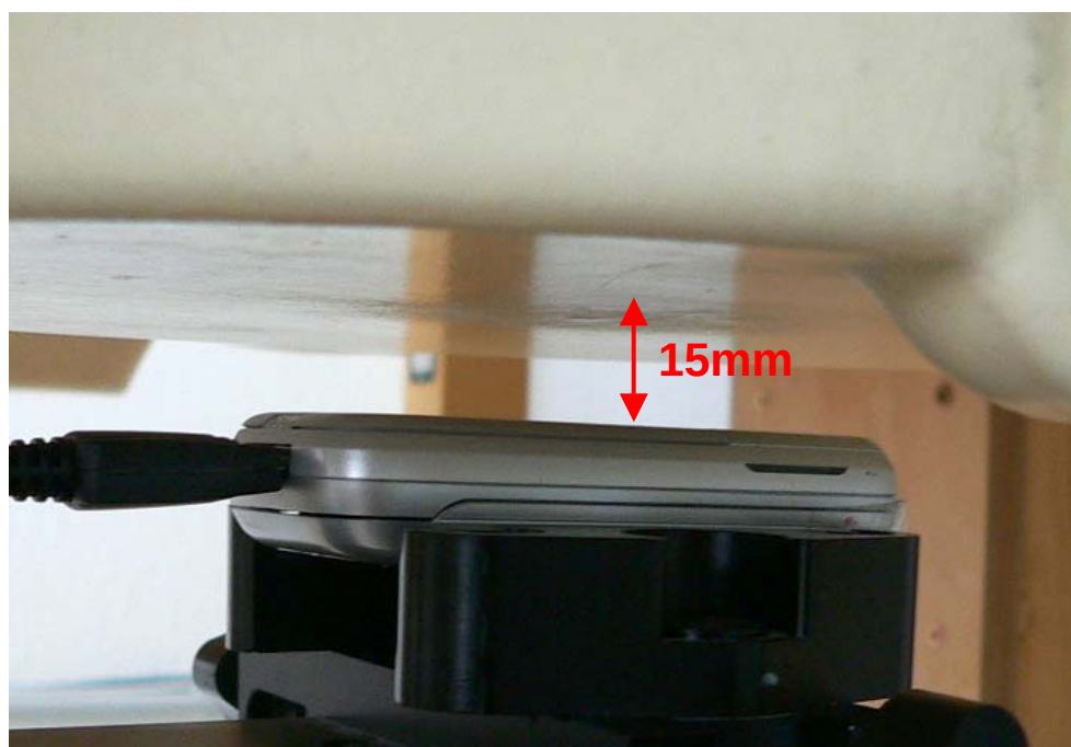
Fig. 35: Body worn configuration, GPRS (Class 8) with data cable, slider down, antenna towards the phantom, 15mm distance.
