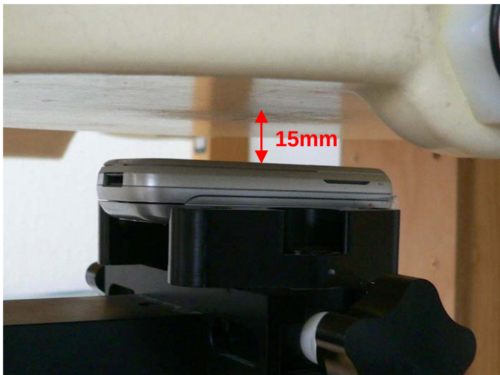
Fig. 33: Body worn configuration, GSM without accessory, slider down, antenna towards the phantom, 15mm distance.
