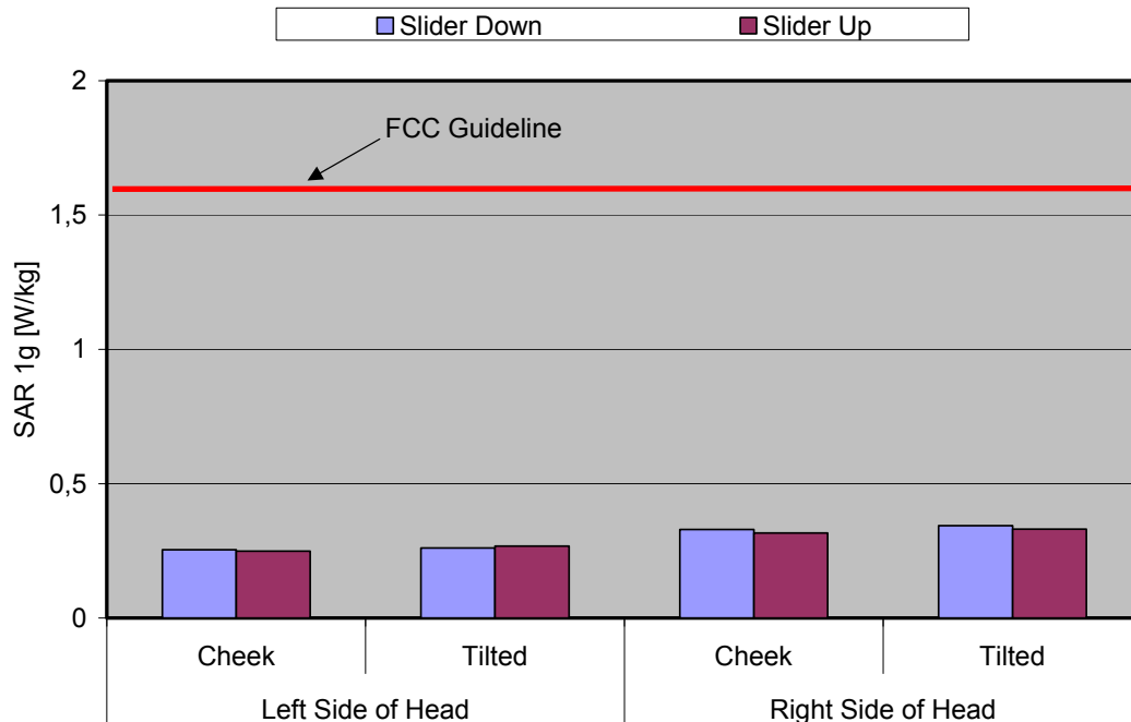
Fig. 8: The measured head phantom SAR values for the Siemens CF110 for PCS 1900 in comparison to the FCC exposure limit.
