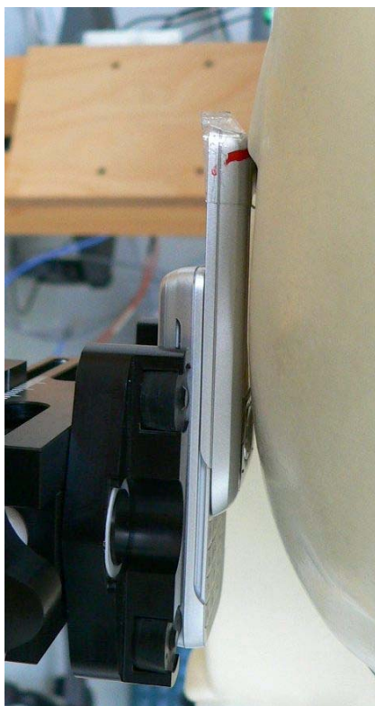
Fig. 24: Cheek position, right side, slider up.
