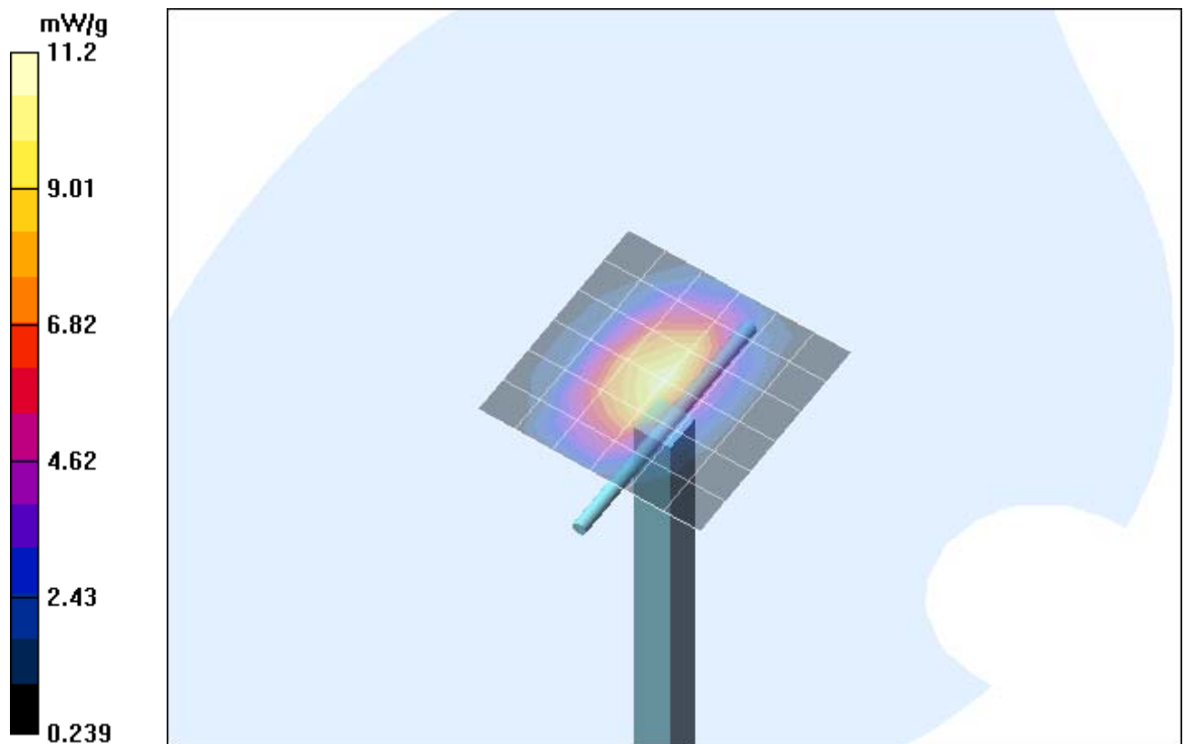
Fig. 12: Validation measurement 1900 MHz body (August 19, 2005), coarse grid. Ambient Temperature: 22.0° C, Liquid Temperature: 21.0° C.
