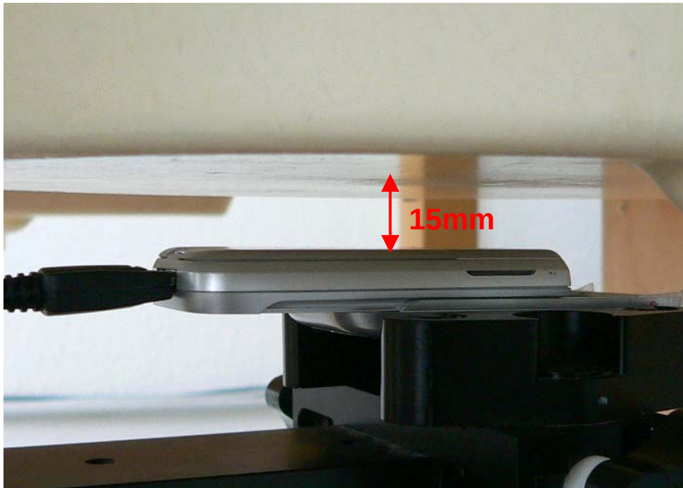
Fig. 32: Body worn configuration, GPRS (Class 8) with data cable, slider up, antenna towards the phantom, 15mm distance.
