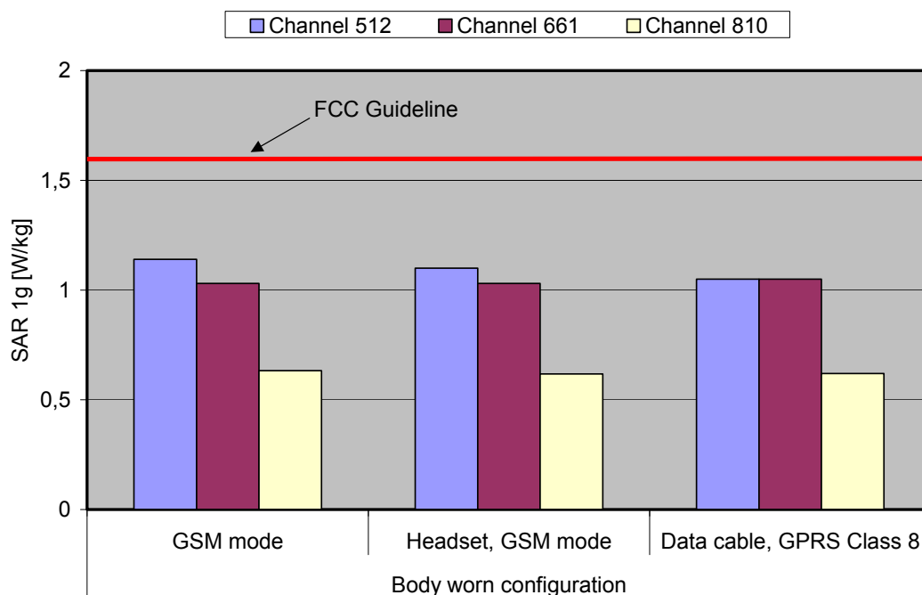
Fig. 10: The measured SAR values in body-worn configuration for the Siemens CF110 slider down for PCS 1900 in comparison to the FCC exposure limit.
