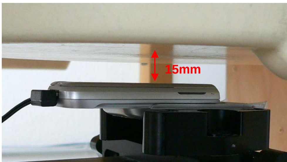
Fig. 31: Body worn configuration, GSM with headset, slider up, antenna towards the phantom, 15mm distance.
