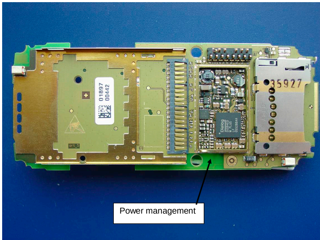
Disassemble Step 5: Front Side of main PCB
