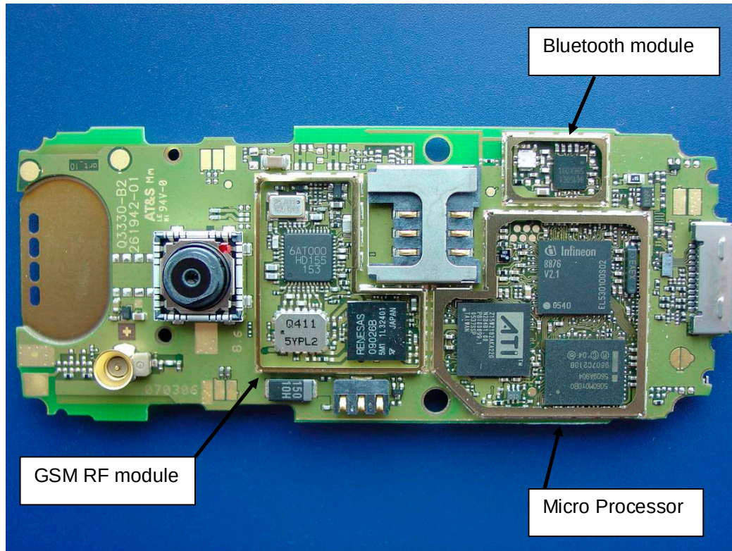
Disassemble Step 6: Back Side of main PCB
