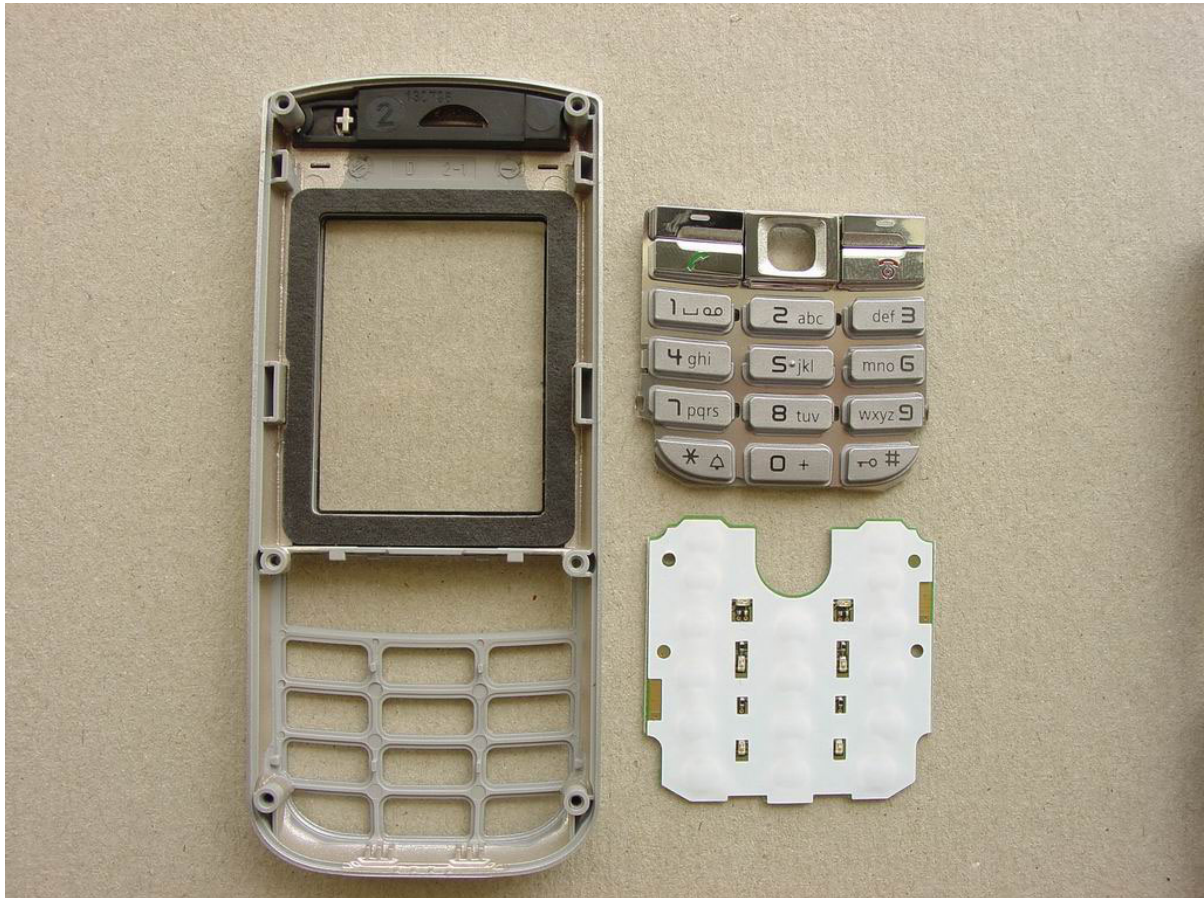
C75 Disassembly Step 4
