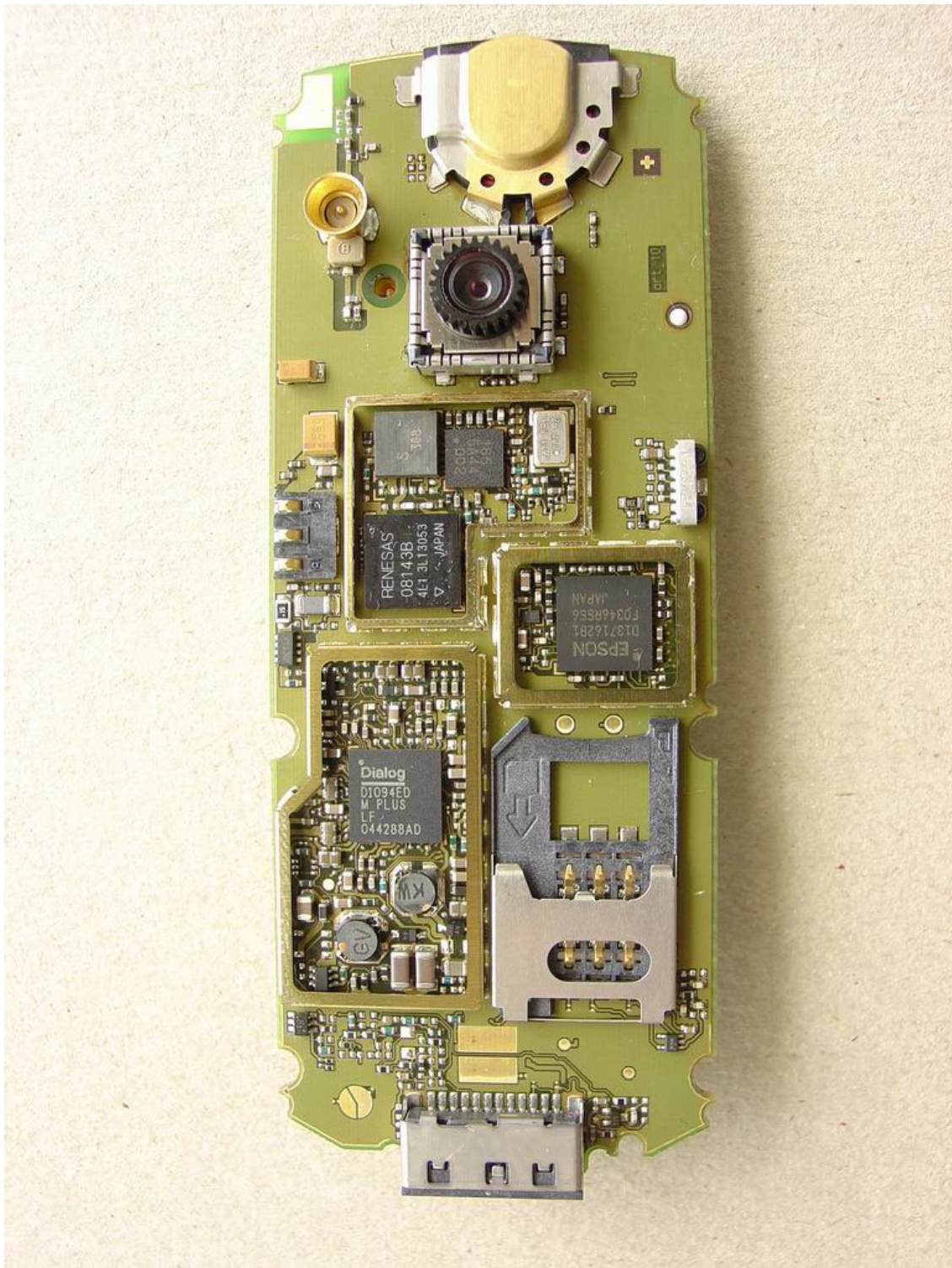
C75 PCB Back View Shields Removed
