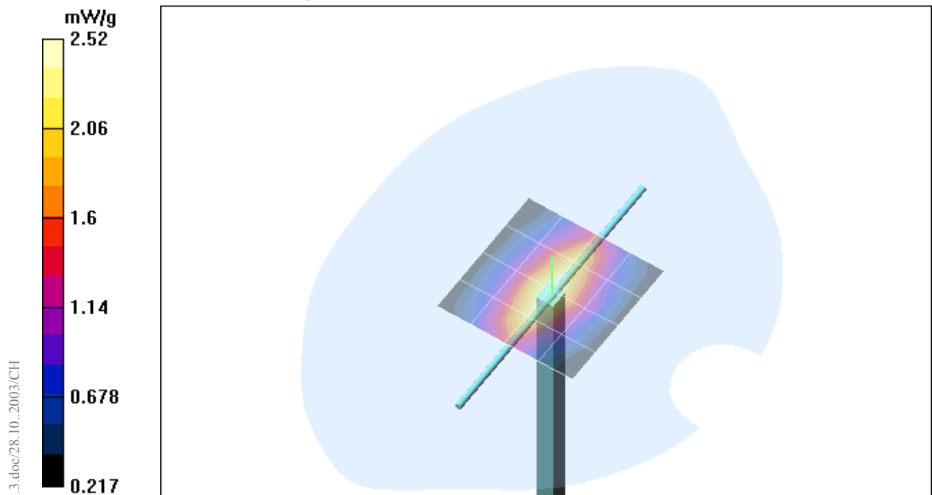
Fig. 13: Validation measurement 850 MHz head (November 21, 2003), coarse grid. Ambient Temperature: 20.8° C, Liquid Temperature: 19.7° C.
