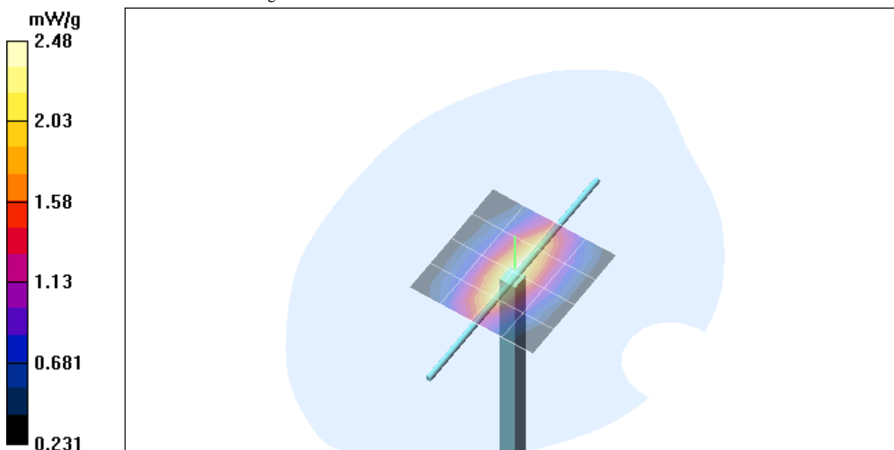
Fig. 14: Validation measurement 850 MHz body (November 17, 2003), coarse grid. Ambient Temperature: 20.9° C, Liquid Temperature: 19.9° C.
