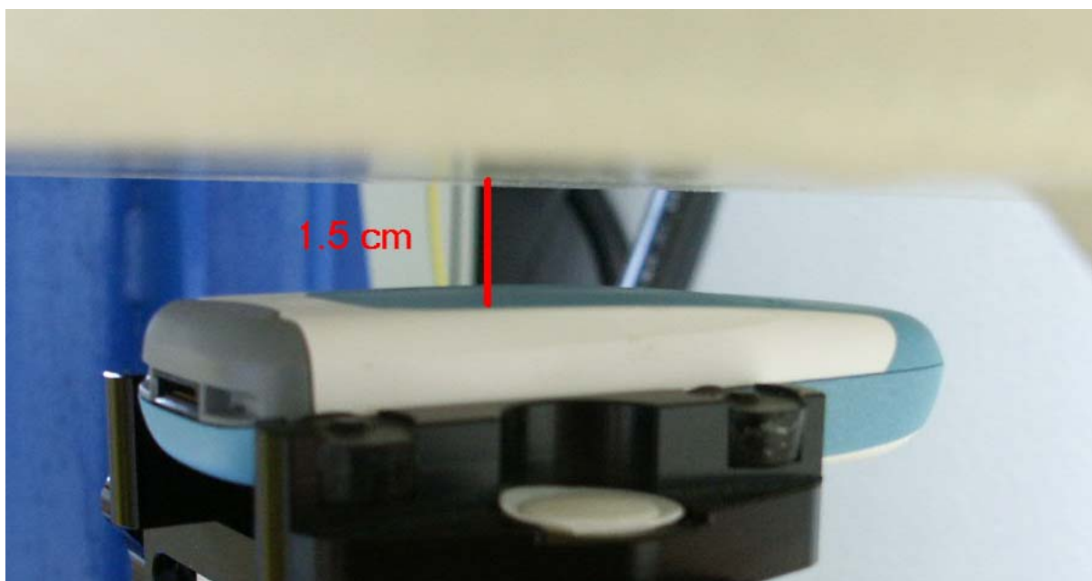
Fig. 32: Body worn configuration, (1 TX slot), display away from phantom.
