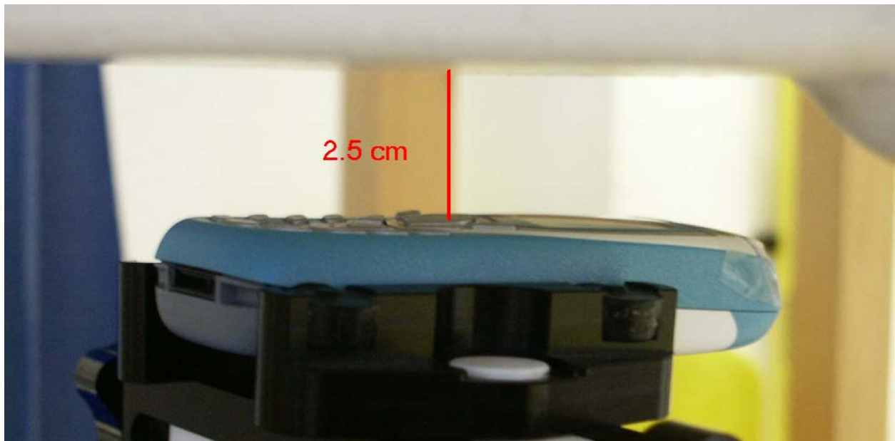
Fig. 33: Push-to-talk function, (1 TX slot), display towards the phantom.
