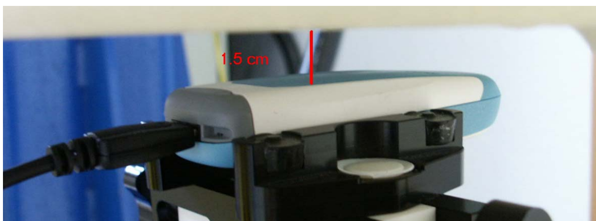
Fig. 31: Body worn configuration, GPRS mode (1 TX slot) with datacable, display away from phantom.
