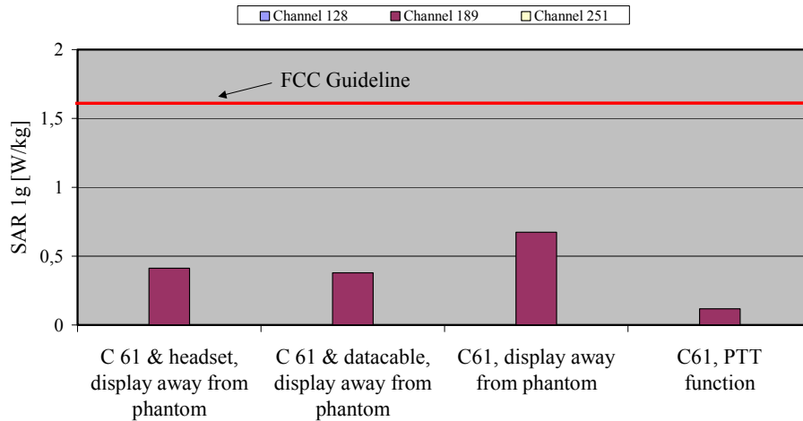
Fig. 11: The measured SAR values in body-worn configuration for the Siemens C61 for GSM 850 in comparison to the FCC exposure limit.
