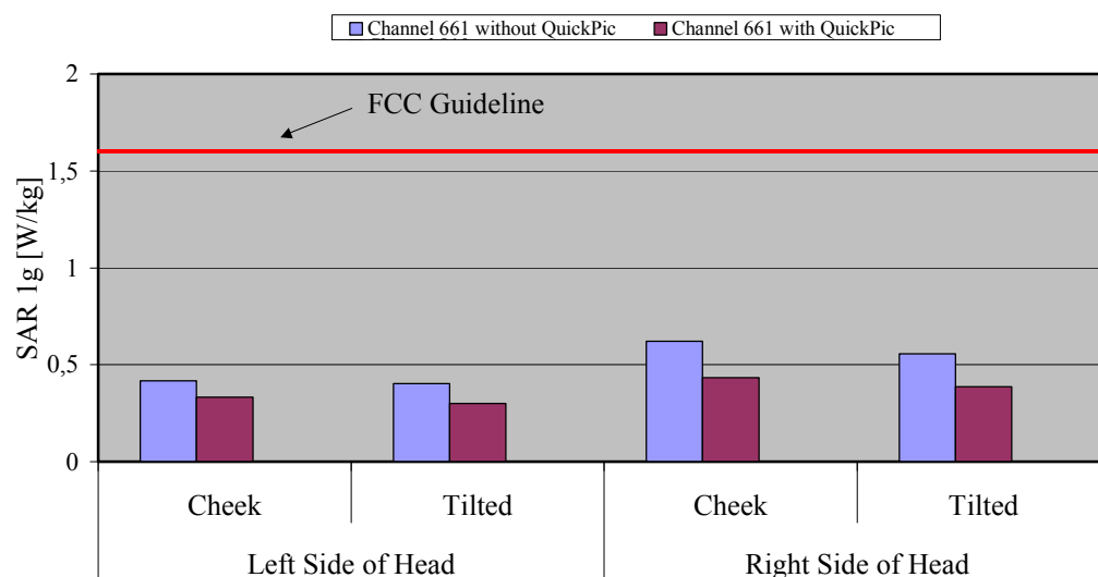
Fig. 10: The measured head phantom SAR values for the Siemens C61 for PCS 1900 in comparison to the FCC exposure limit.
