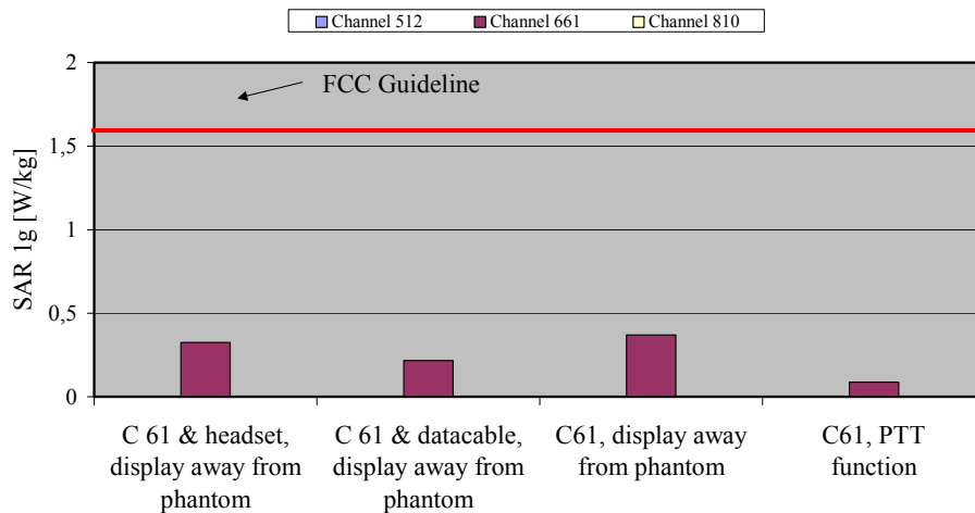
Fig. 12: The measured SAR values in body-worn configuration for the Siemens C61 for PCS 1900 in comparison to the FCC exposure limit.
