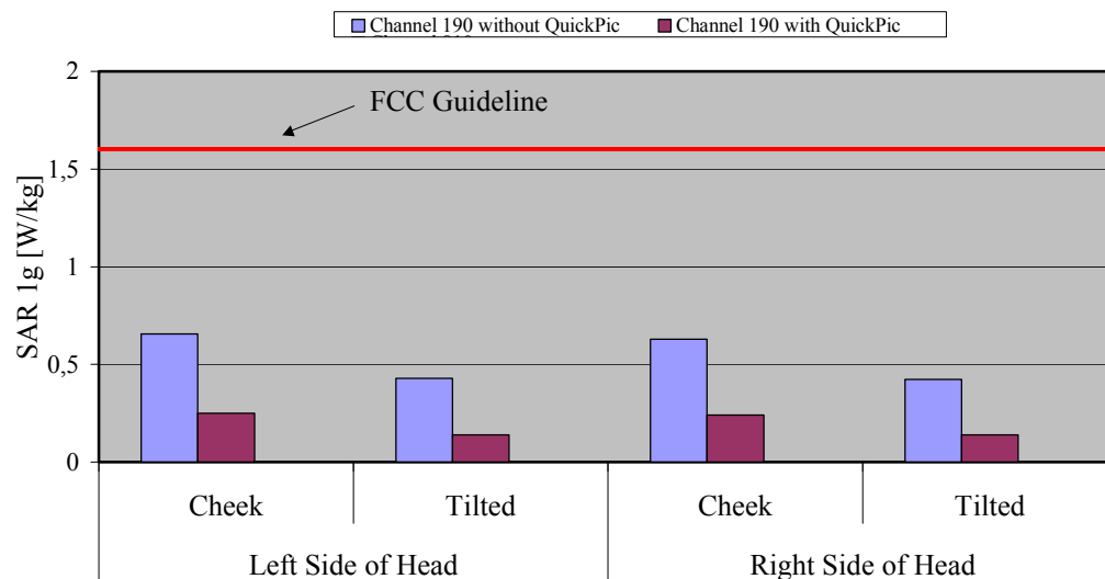
Fig. 9: The measured head phantom SAR values for the Siemens C61 for GSM 850 in comparison to the FCC exposure limit.
