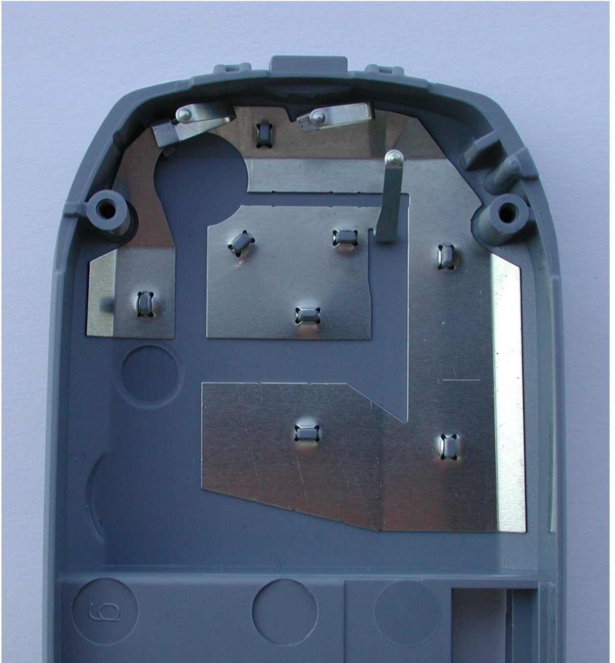
C61 GSM Dual-band Antenna
