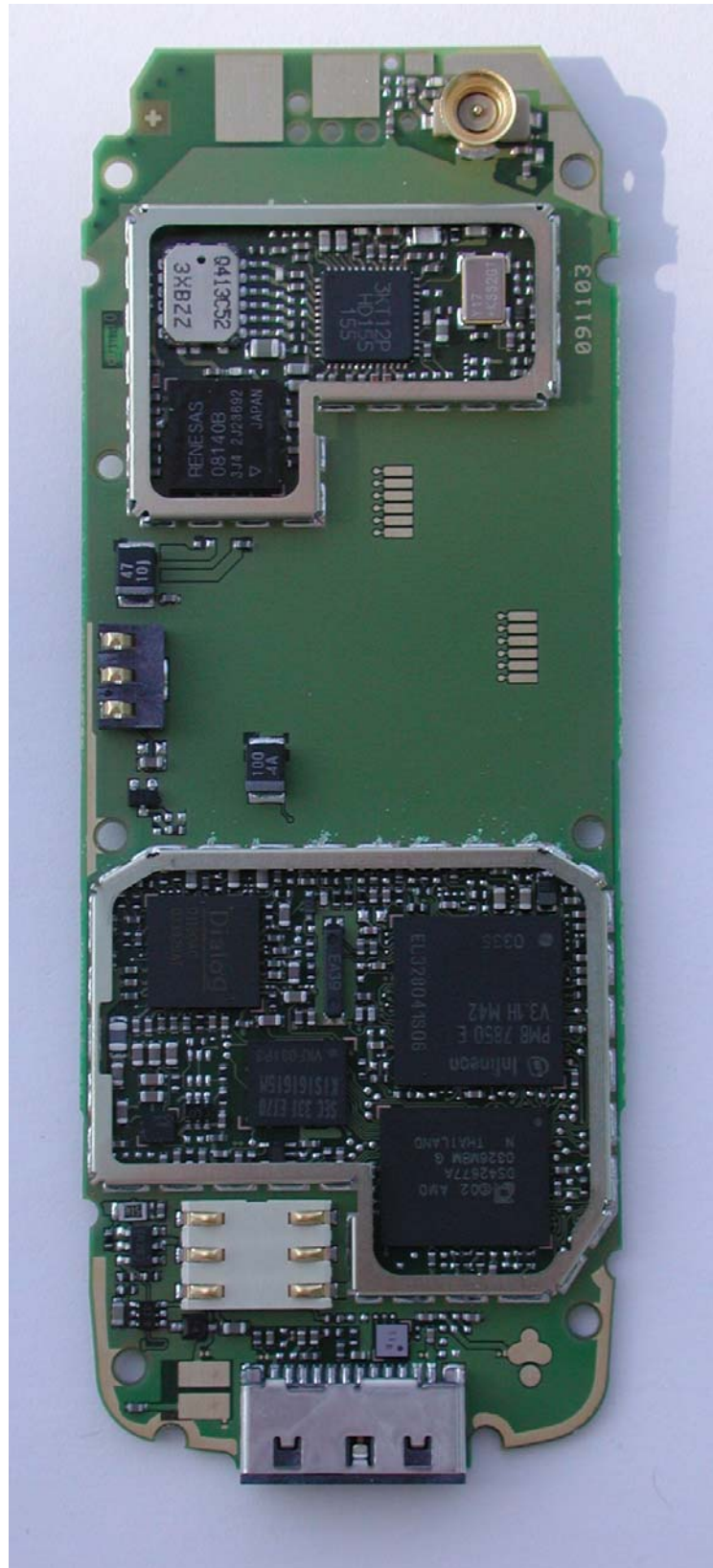
C61 Board without shield
