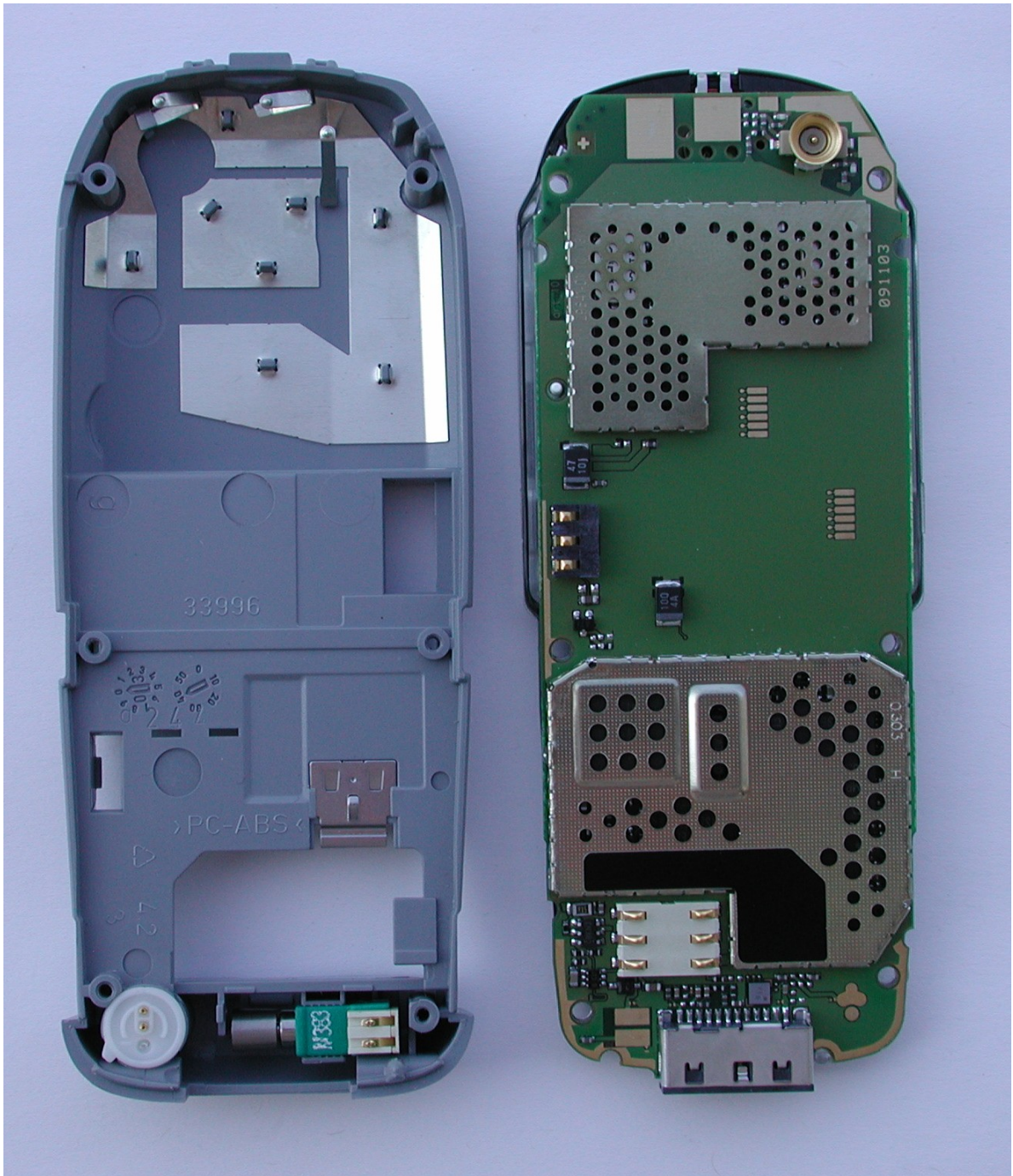
C61 Disassembly step 2
