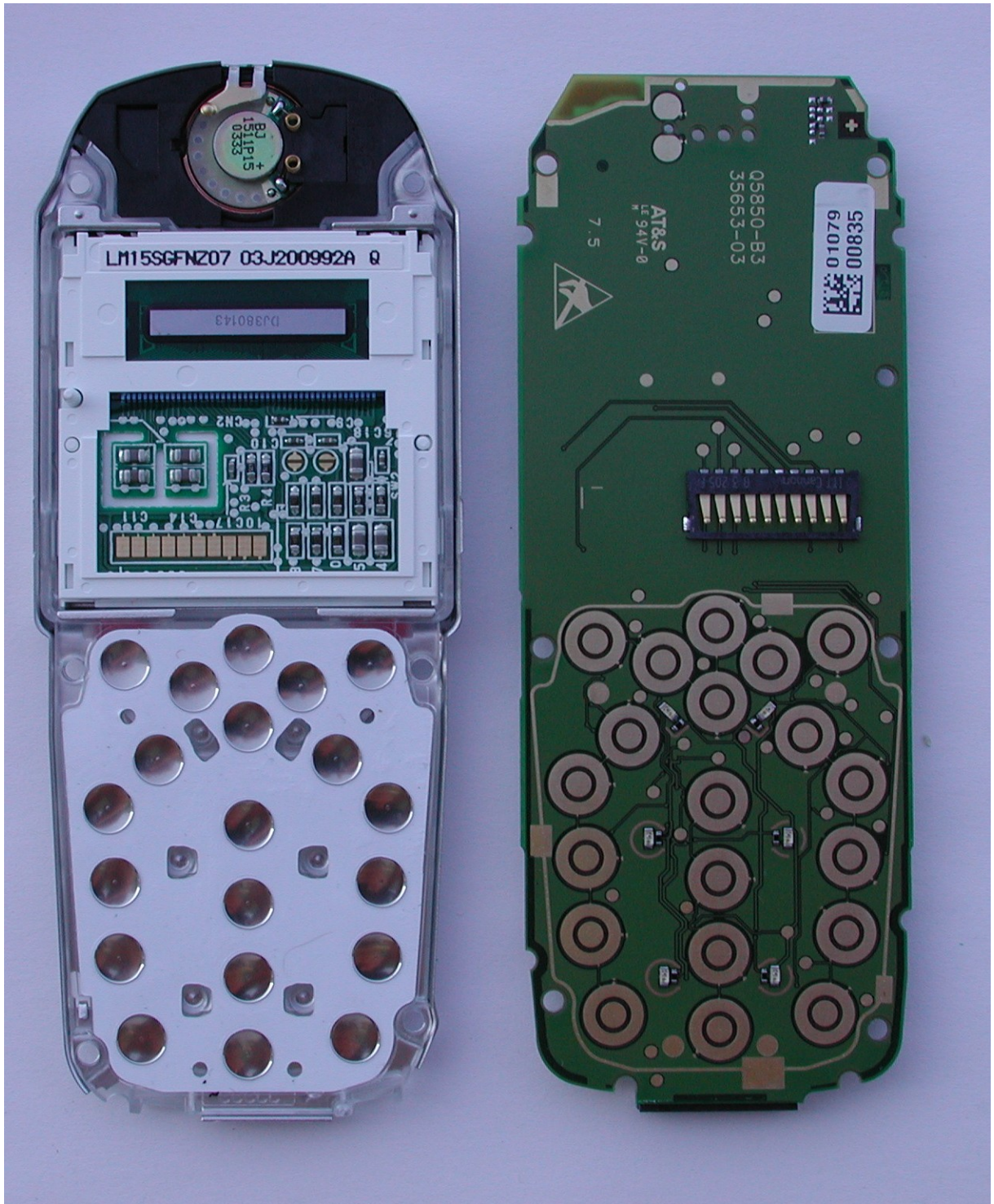
C61 Disassembly step 3
