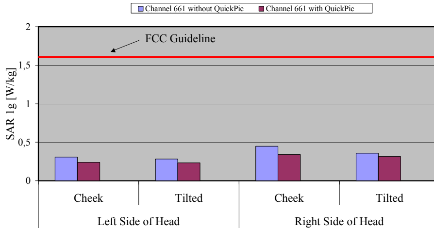
Fig. 9: The measured head phantom SAR values for the Siemens C60 for PCS 1900 in comparison to the FCC exposure limit.
