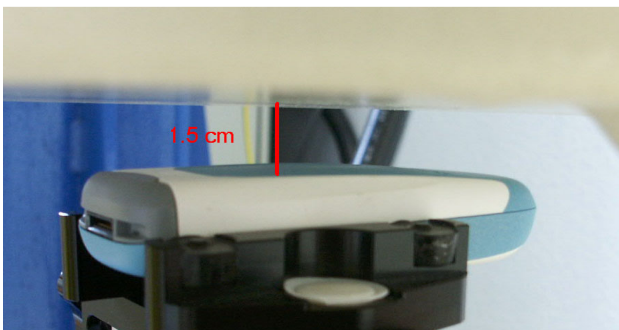
Fig. 29: Body worn configuration, (1 TX slot), display away from phantom.
