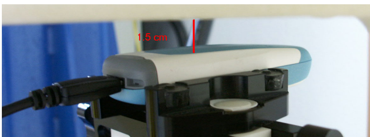
Fig. 28: Body worn configuration, GPRS mode (1 TX slot) with datacable, display away from phantom.
