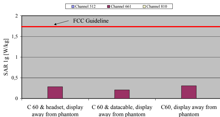
Fig. 10: The measured SAR values in body-worn configuration for the Siemens C60 for PCS 1900 in comparison to the FCC exposure limit.
