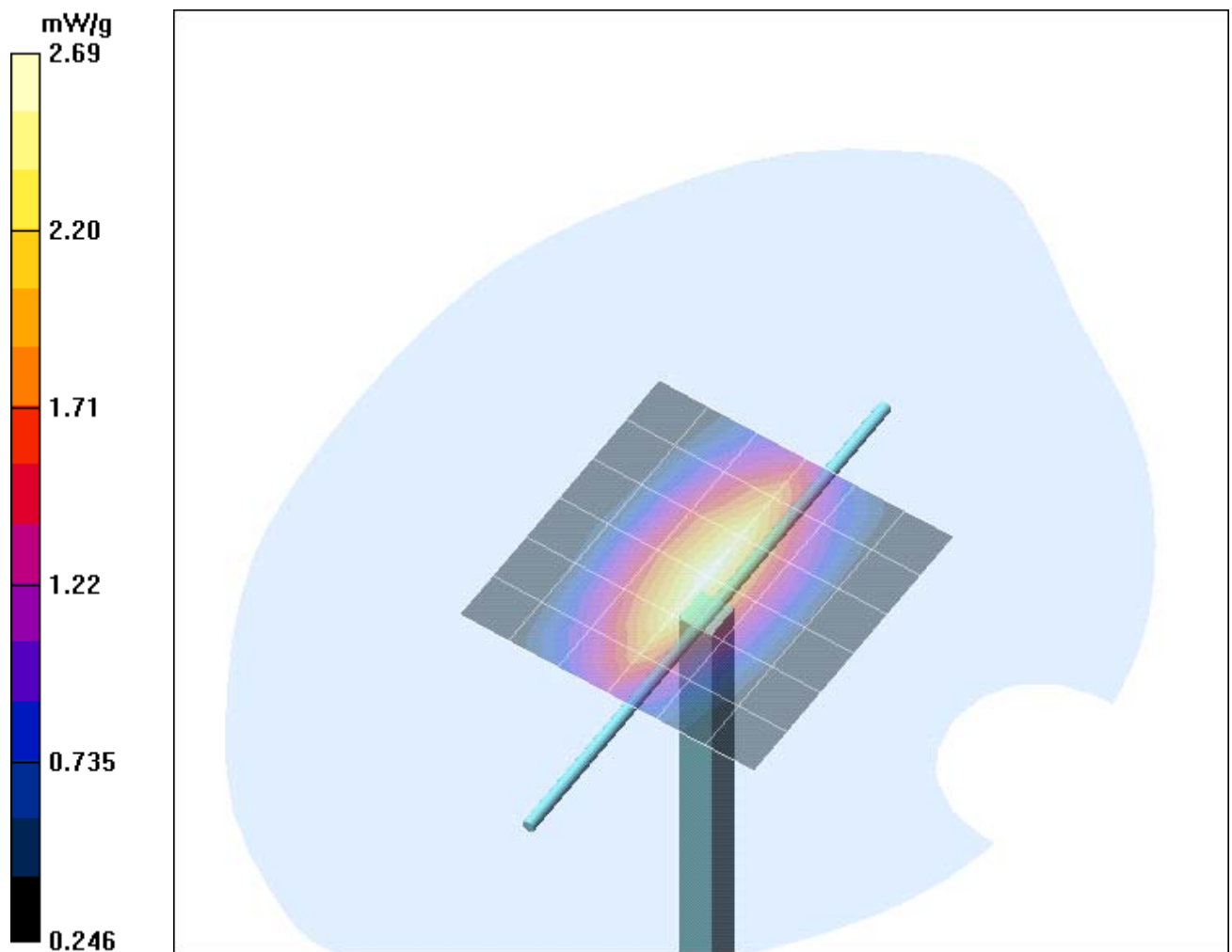
Fig. 13: Validation measurement 835 MHz Body (August 04, 2005), coarse grid. Ambient Temperature: 22.0° C, Liquid Temperature: 21.0° C.
