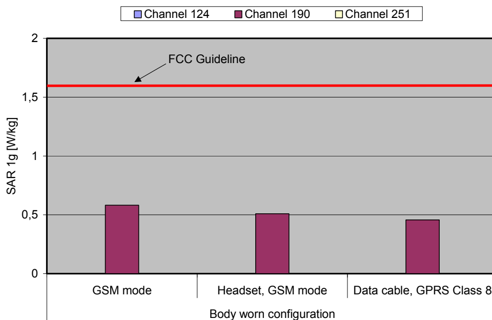
Fig. 10: The measured SAR values in body-worn configuration for the Siemens AX76 for GSM 850 in comparison to the FCC exposure limit.
