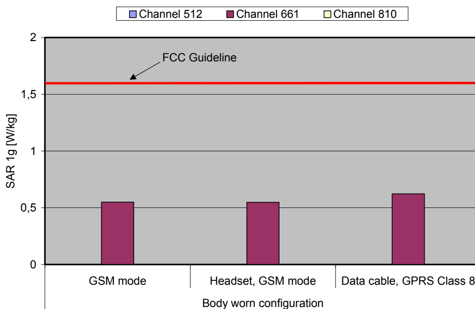
Fig. 11: The measured SAR values in body-worn configuration for the Siemens AX76 for PCS 1900 in comparison to the FCC exposure limit.
