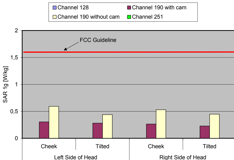
Fig. 8: The measured head phantom SAR values for the Siemens AX76 for GSM 850 in comparison to the FCC exposure limit.
