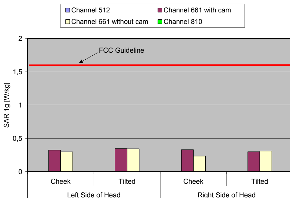
Fig. 9: The measured head phantom SAR values for the Siemens AX76 for PCS 1900 in comparison to the FCC exposure limit.
