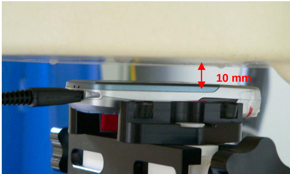
Fig. 38: Body worn configuration, GPRS mode (Class 8) with data cable, antenna towards the phantom (10 mm distance).
