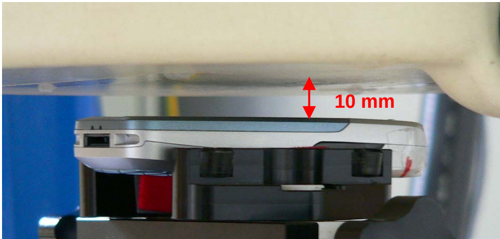
Fig. 36: Body worn configuration, GSM mode without accessory, antenna towards the phantom (10 mm distance).
