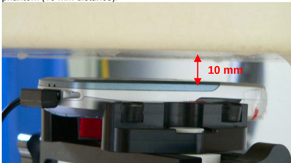
Fig. 37: Body worn configuration, GSM mode with headset, antenna towards the phantom (10 mm distance).
