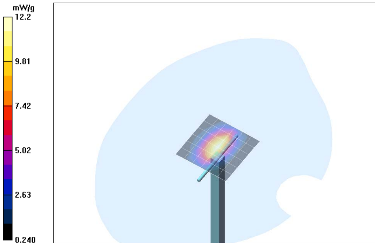
Fig. 15: Validation measurement 1900 MHz Body (August 03, 2005), coarse grid. Ambient Temperature: 22.0° C, Liquid Temperature: 21.0° C.
