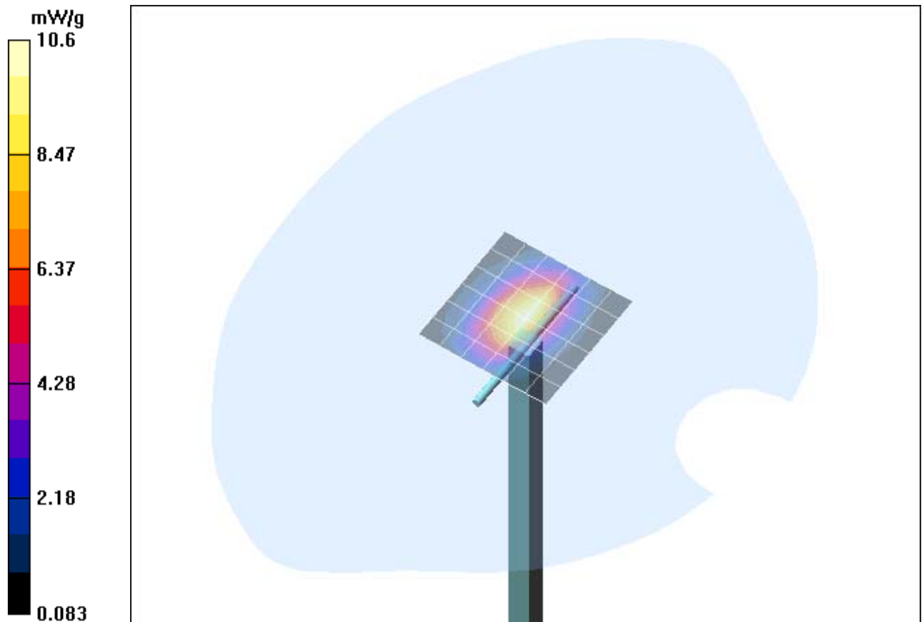
Fig. 14: Validation measurement 1900 MHz Head (August 01, 2005), coarse grid. Ambient Temperature: 22.0° C, Liquid Temperature: 21.5° C.
