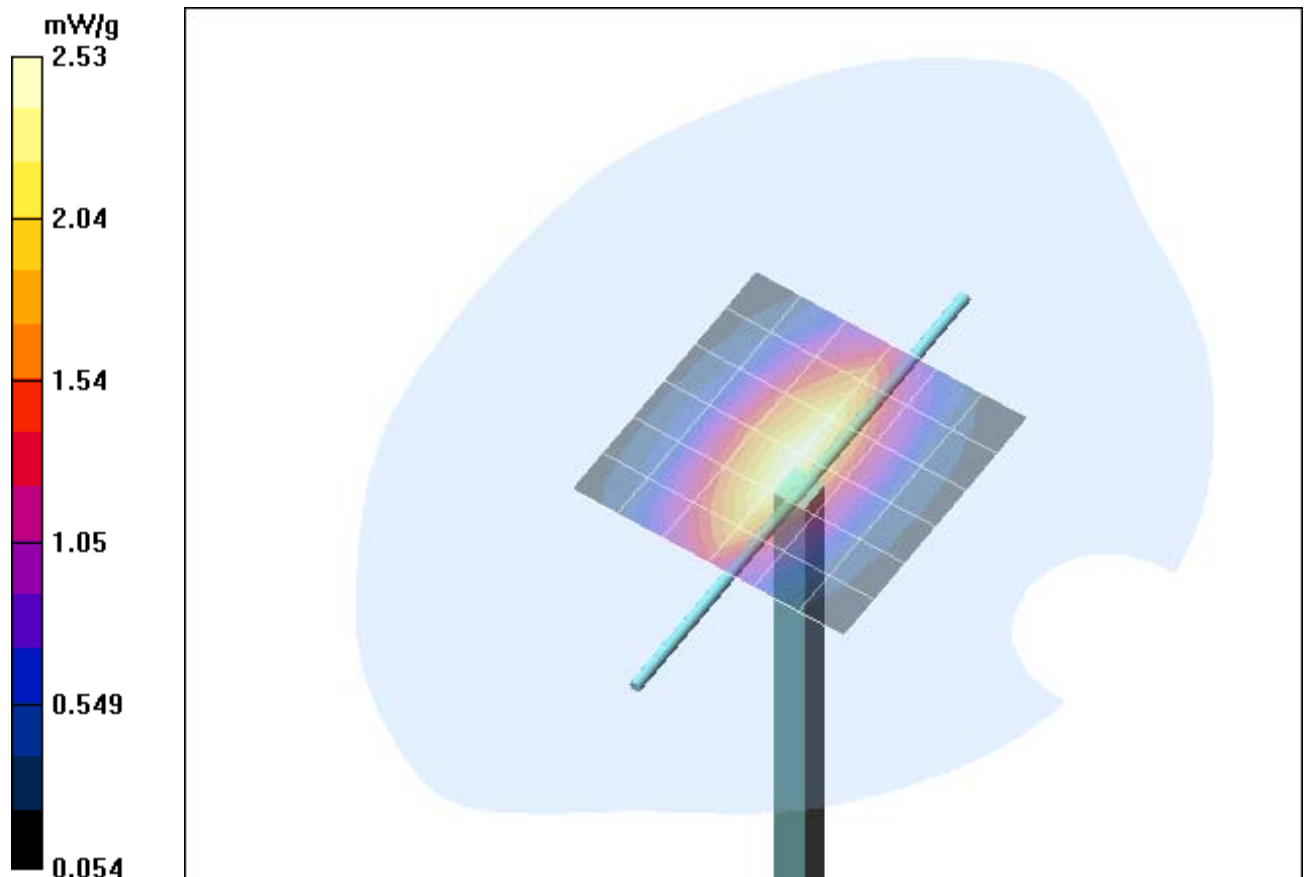
Fig. 12: Validation measurement 835 MHz Head (August 02, 2005), coarse grid. Ambient Temperature: 22.0° C, Liquid Temperature: 21.5° C.
