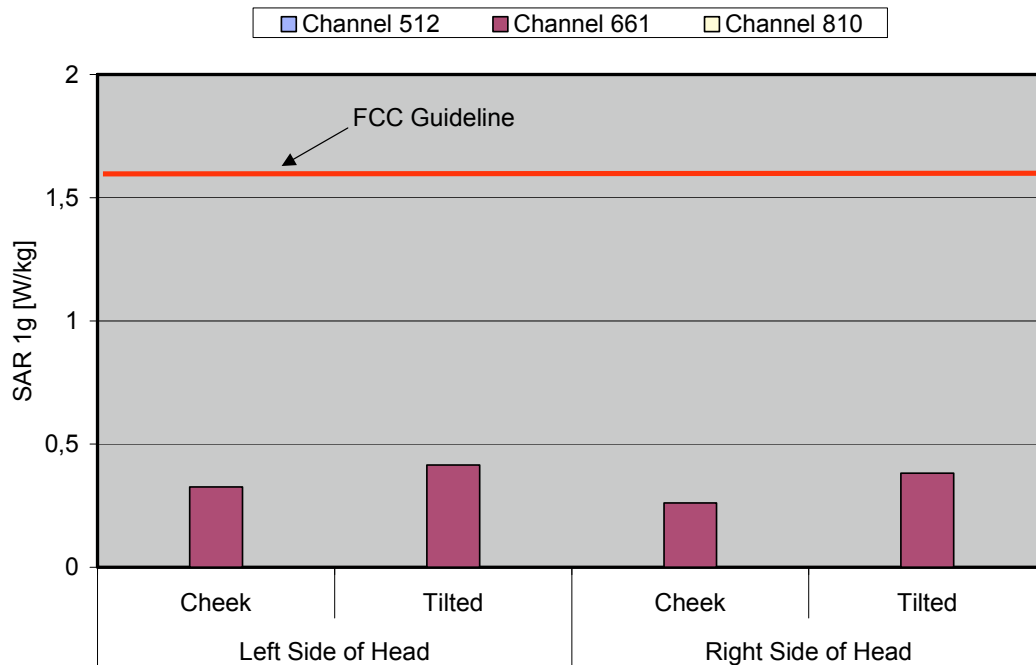
Fig. 8: The measured head phantom SAR values for the Siemens AX75 for PCS 1900 in comparison to the FCC exposure limit.
