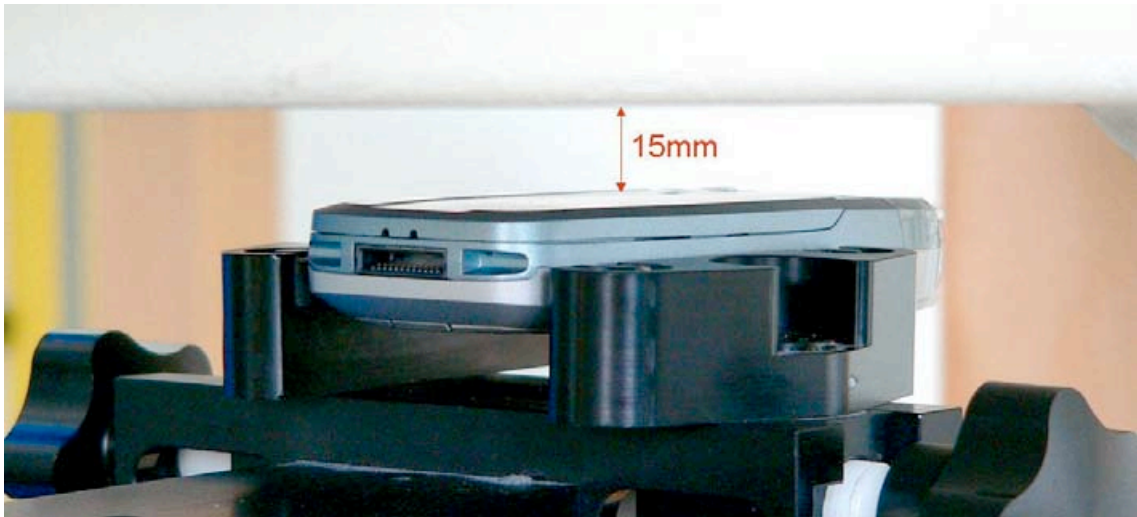
Fig. 25: Body worn configuration, GSM, antenna towards the phantom.
