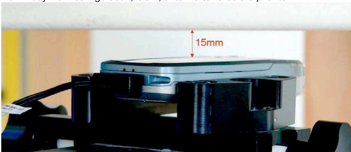
Fig. 26: Body worn configuration, GSM with headset, antenna towards the phantom.
