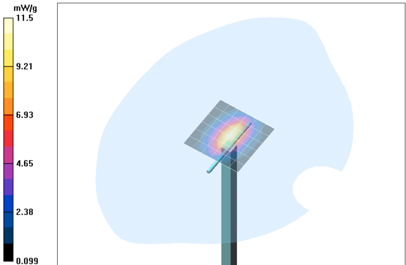
Fig. 11: Validation measurement 1900 MHz Head (May 13, 2005), coarse grid. Ambient Temperature: 21.1° C, Liquid Temperature: 20.6° C.
