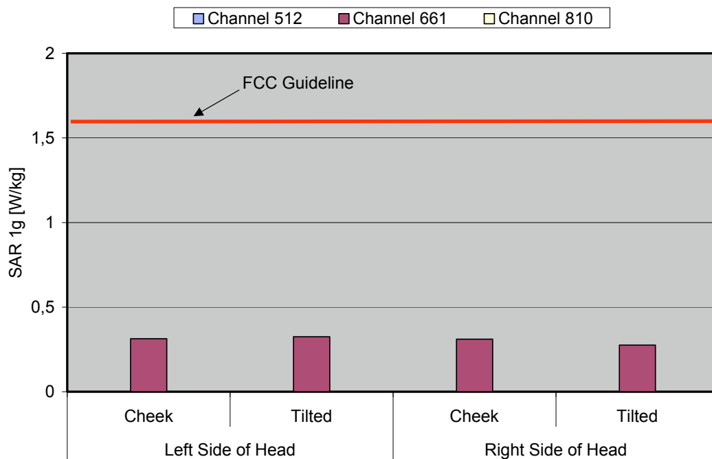
Fig. 9: The measured head phantom SAR values for the Siemens AX75 with Camera for PCS 1900 in comparison to the FCC exposure limit.
