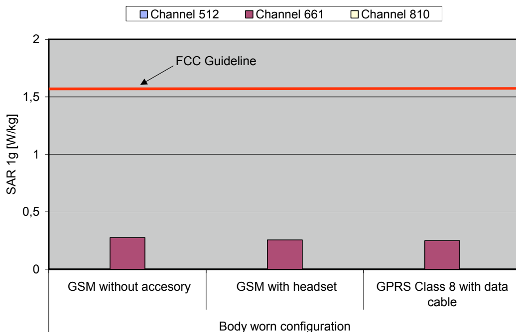
Fig. 10: The measured SAR values in body-worn configuration for the Siemens AX75 for PCS 1900 in comparison to the FCC exposure limit.
