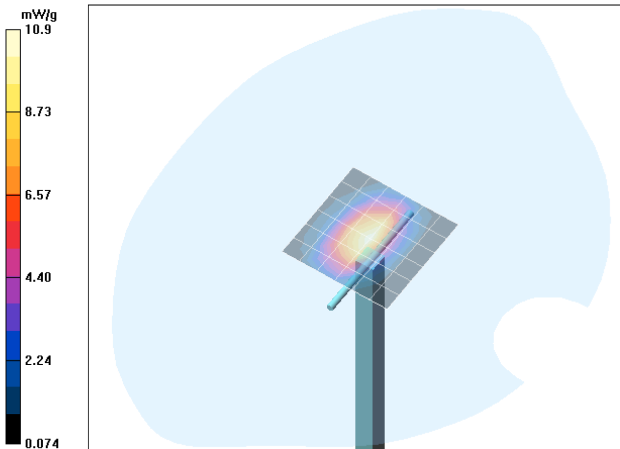
Fig. 12: Validation measurement 1900 MHz body (May 20, 2005), coarse grid. Ambient Temperature: 21.3° C, Liquid Temperature: 20.7° C.
