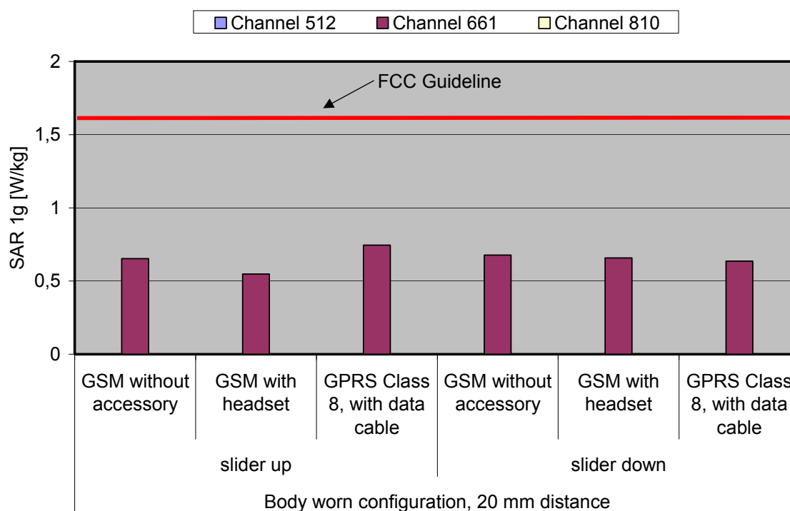
Fig. 11: The measured SAR values in body-worn configuration for the BenQ Siemens AL21a for PCS 1900 in comparison to the FCC exposure limit.
