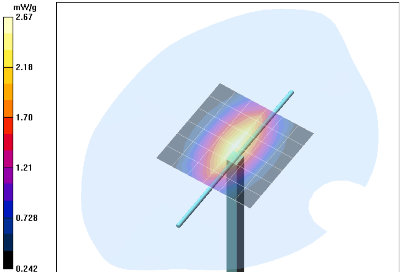
Fig. 12: Validation measurement 835 MHz Head (March 24, 2006), coarse grid. Ambient Temperature: 22.0° C, Liquid Temperature: 21.0° C.
