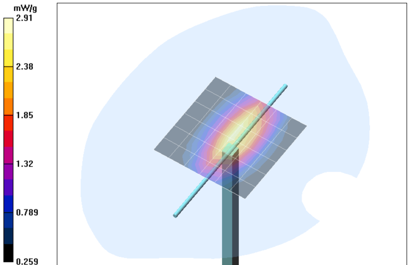
Fig. 13: Validation measurement 835 MHz Body (March 24, 2006), coarse grid. Ambient Temperature: 22.0° C, Liquid Temperature: 21.0° C.
