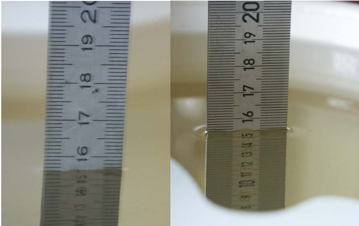
Fig. 40: Liquid depth for GSM 850 head and body measurements.
