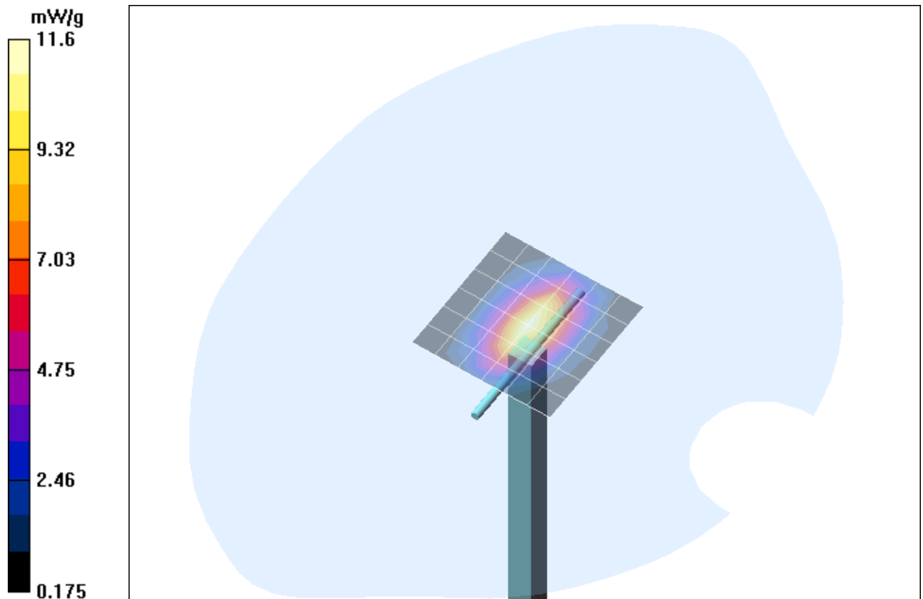
Fig. 15: Validation measurement 1900 MHz Body (March 27, 2006), coarse grid. Ambient Temperature: 22.0° C, Liquid Temperature: 21.0° C.
