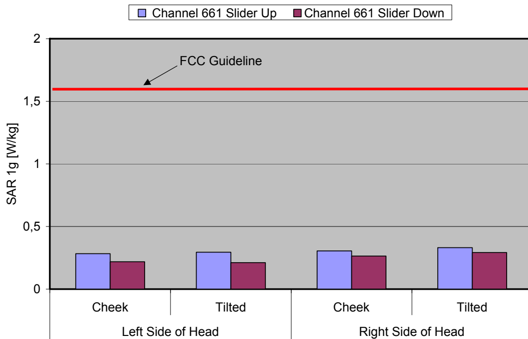
Fig. 9: The measured head phantom SAR values for the BenQ Siemens AL21a for PCS 1900 in comparison to the FCC exposure limit.
