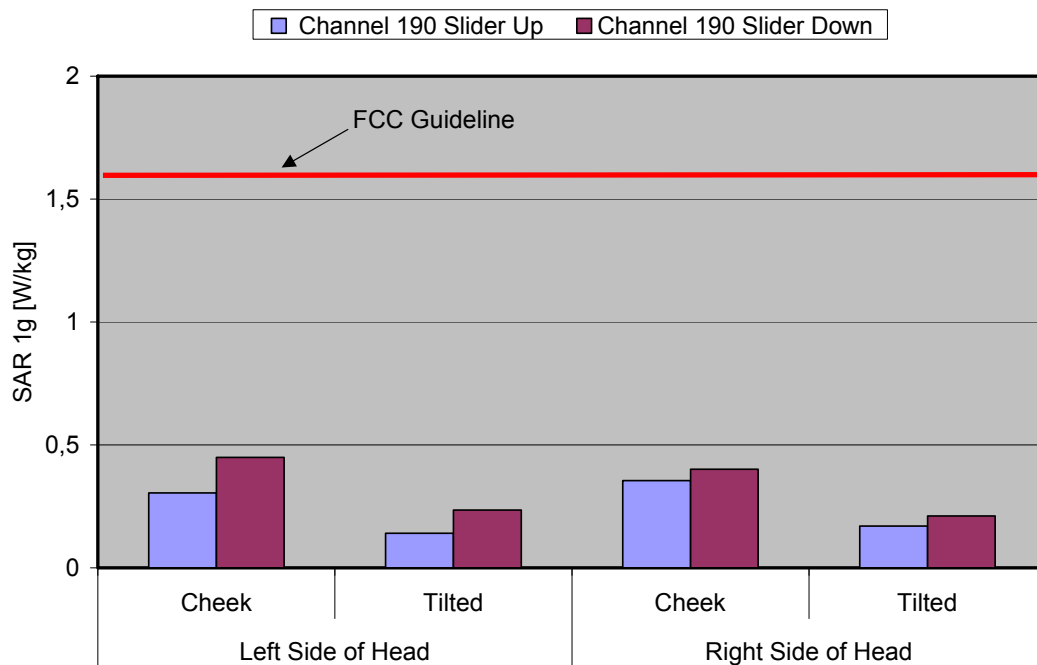
Fig. 8: The measured head phantom SAR values for the BenQ Siemens AL21a for GSM 850 in comparison to the FCC exposure limit.
