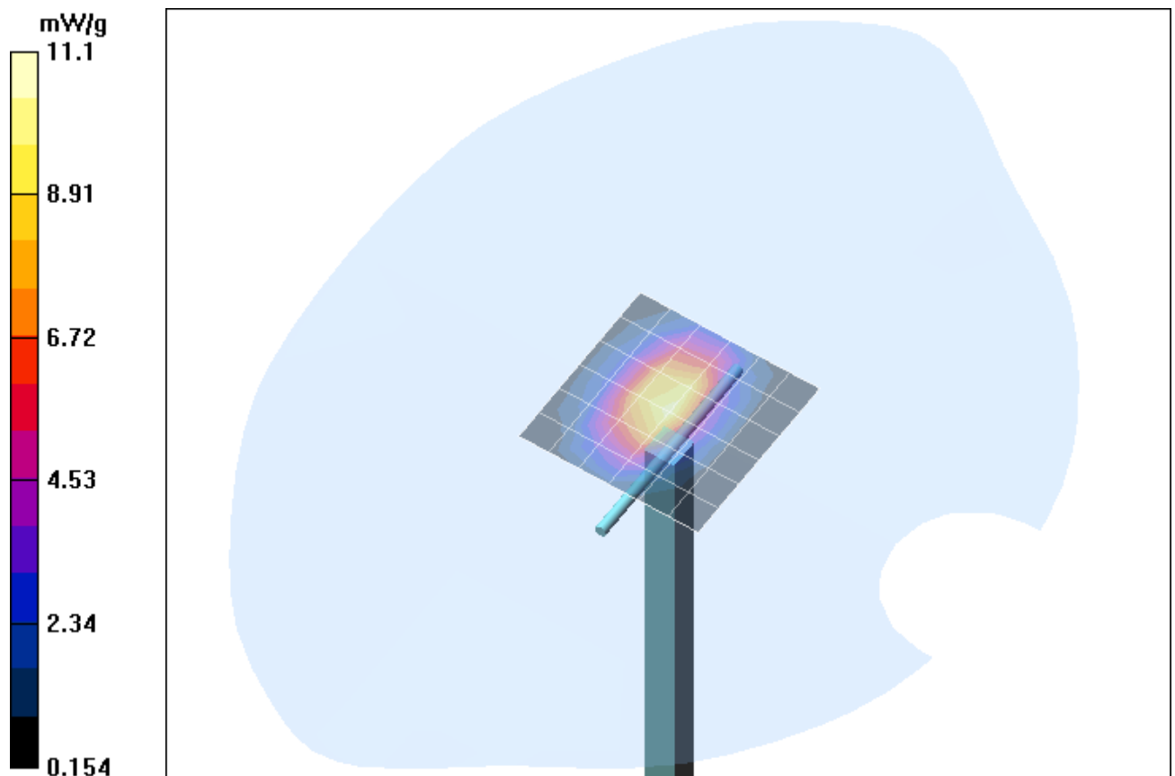
Fig. 14: Validation measurement 1900 MHz Head (March 22, 2006), coarse grid. Ambient Temperature: 22.0° C, Liquid Temperature: 21.0° C.
