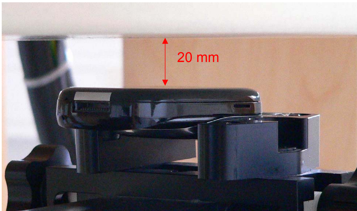
Fig. 34: Body worn configuration, GSM without accessory, slider up, antenna towards the phantom.
