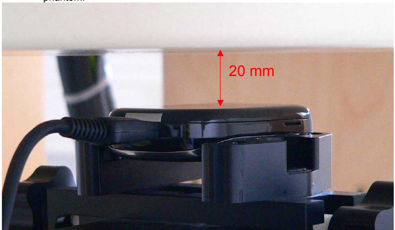
Fig. 39: Body worn configuration, GPRS (Class 8) with data cable, slider down, antenna towards the phantom.
