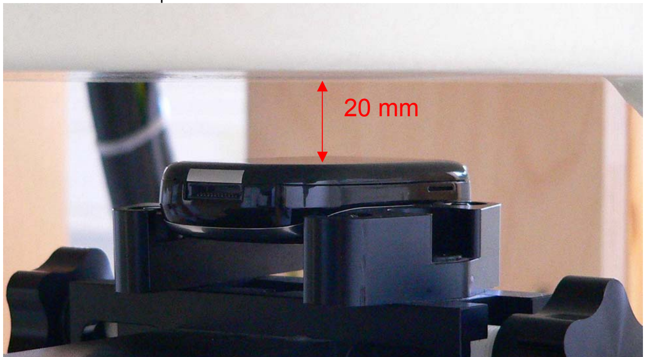
Fig. 37: Body worn configuration, GSM without accessory, slider down, antenna towards the phantom
