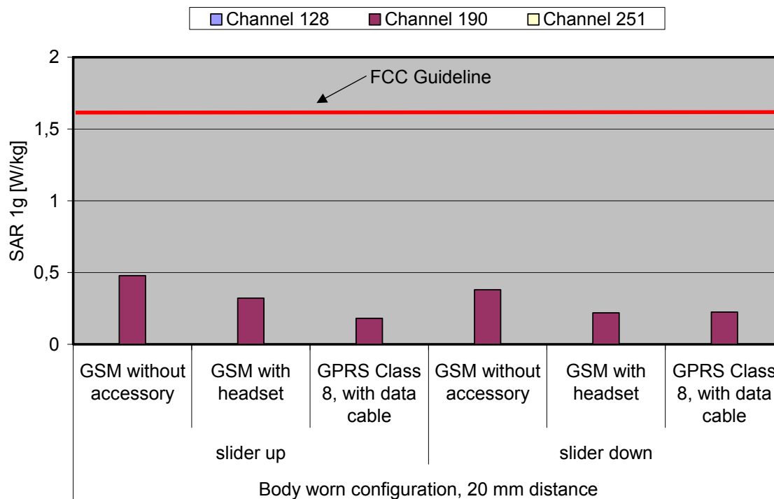
Fig. 10: The measured SAR values in body-worn configuration for the BenQ Siemens AL21a for GSM 850 in comparison to the FCC exposure limit.
