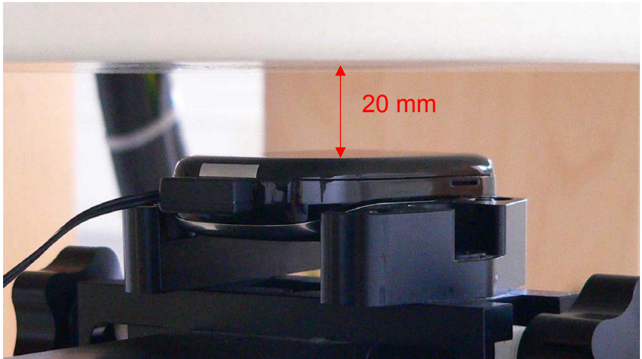
Fig. 38: Body worn configuration, GSM with headset, slider down, antenna towards the phantom.
