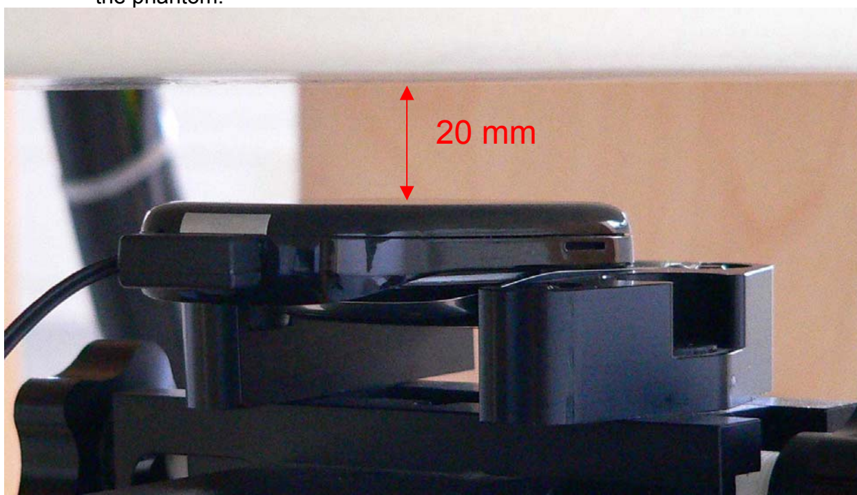
Fig. 35: Body worn configuration, GSM with headset, slider up, antenna towards the phantom
