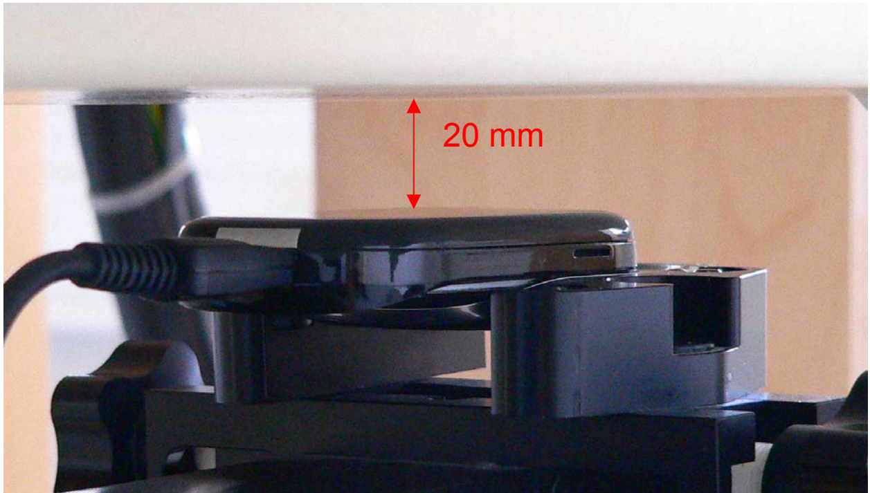
Fig. 36: Body worn configuration, GPRS (Class 8) with data cable, slider up, antenna towards the phantom.
