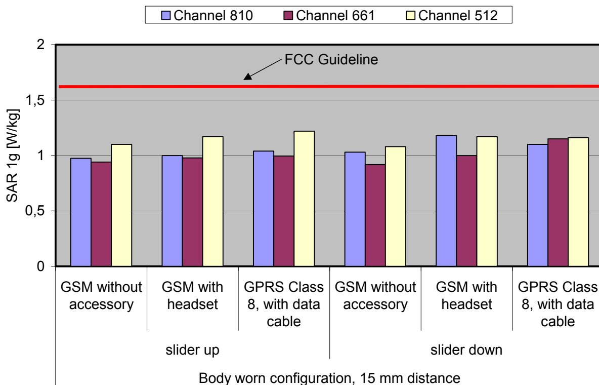
Fig. 10: The measured SAR values in body-worn configuration for the BenQ AL21 for PCS 1900 in comparison to the FCC exposure limit.
