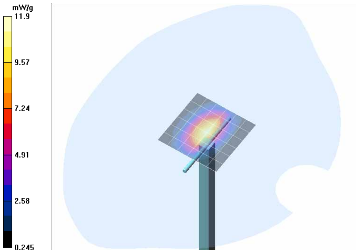
Fig. 12: Validation measurement 1900 MHz body (February 10, 2006), coarse grid. Ambient Temperature: 21.4° C, Liquid Temperature: 20.6° C.
