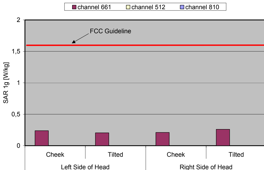
Fig. 8: The measured head phantom SAR values for the BenQ AL21 with slider up for PCS 1900 in comparison to the FCC exposure limit.
