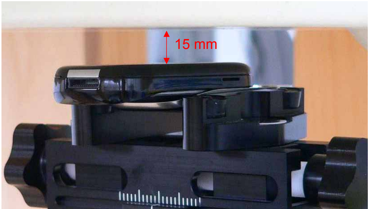
Fig. 30: Body worn configuration, GSM without accessory, antenna towards the phantom.
