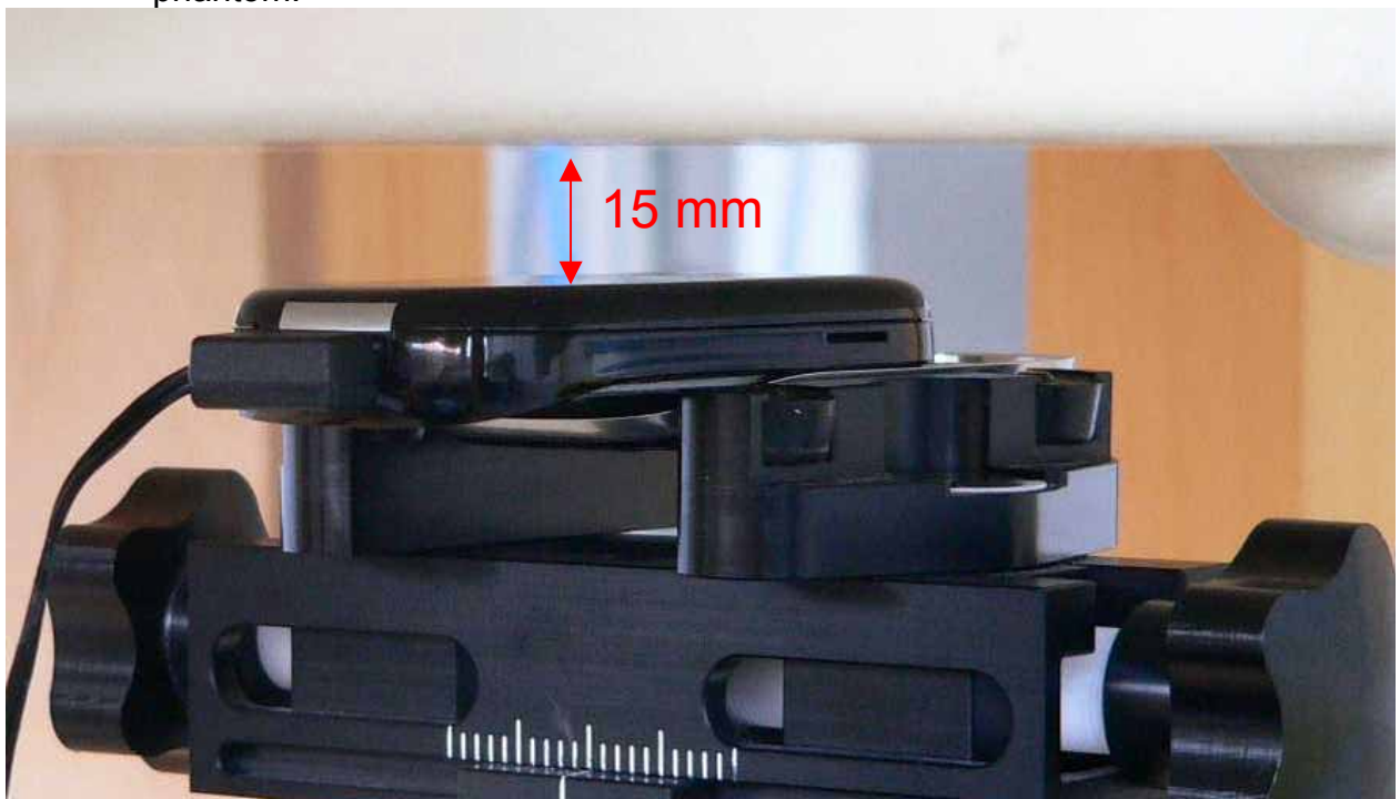
Fig. 31: Body worn configuration, GSM with headset, antenna towards the phantom
