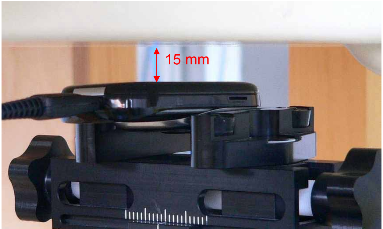
Fig. 32: Body worn configuration, GPRS (Class 8) with data cable, antenna towards the phantom.
