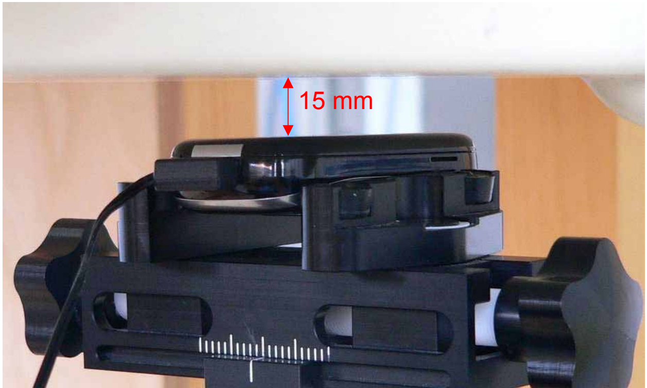
Fig. 34: Body worn configuration, GSM without accessory, antenna towards the phantom.
