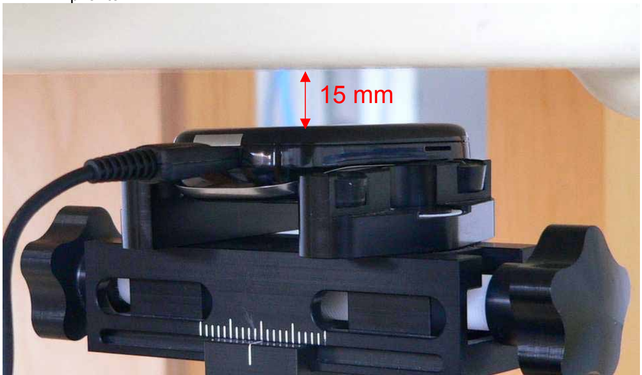
Fig. 35: Body worn configuration, GPRS (Class 8) with data cable, antenna towards the phantom.
