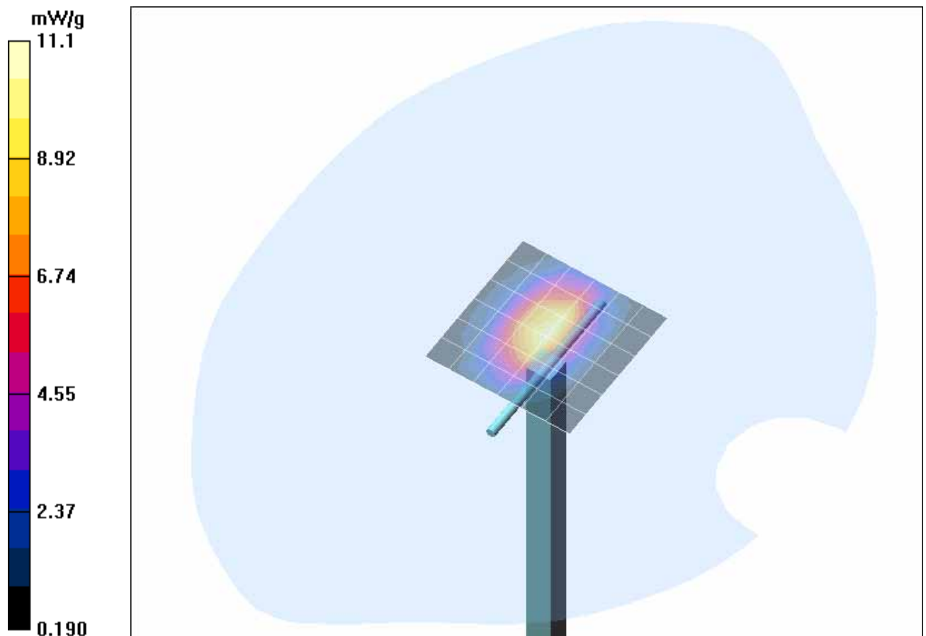
Fig. 11: Validation measurement 1900 MHz Head (February 08, 2006), coarse grid. Ambient Temperature: 21.7° C, Liquid Temperature: 20.9° C.
