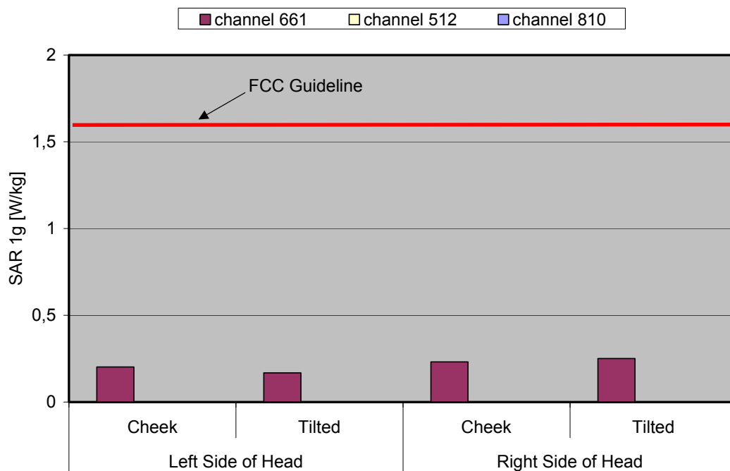
Fig. 9: The measured head phantom SAR values for the BenQ AL21 with slider down for PCS 1900 in comparison to the FCC exposure limit.
