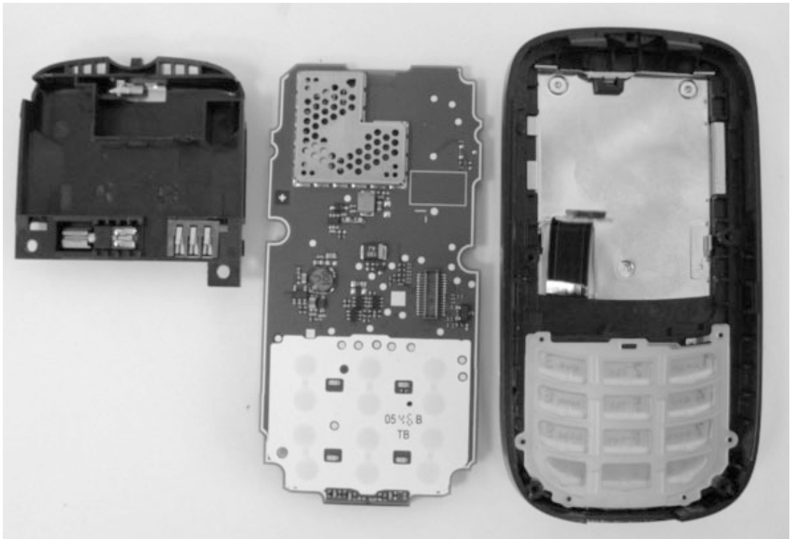
AL21 Disassembly Step 2
