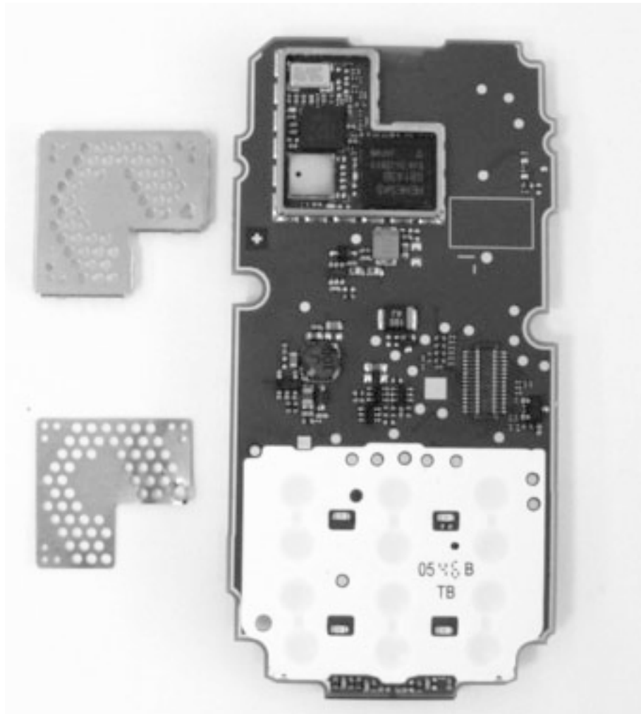
AL21 Front view RF
