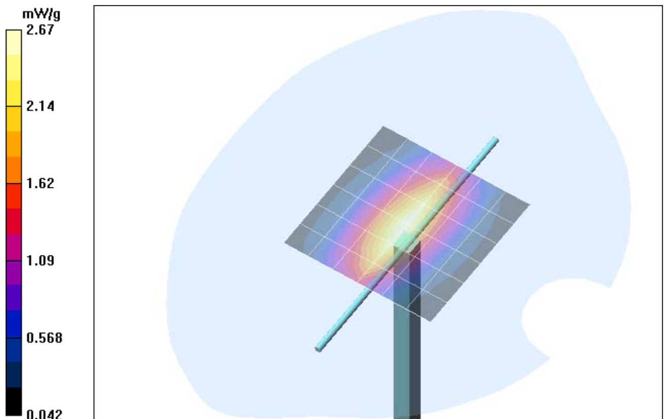
Fig. 13: Validation measurement 835 MHz Body (June 23, 2005), coarse grid. Ambient Temperature: 22.1° C, Liquid Temperature: 22.0° C.
