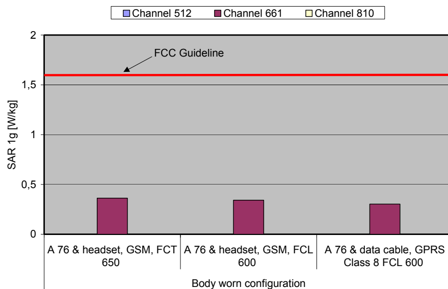
Fig. 11: The measured SAR values in body-worn configuration for the Siemens A76 for PCS 1900 in comparison to the FCC exposure limit.
