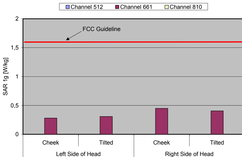
Fig. 9: The measured head phantom SAR values for the Siemens A76 for PCS 1900 in comparison to the FCC exposure limit.
