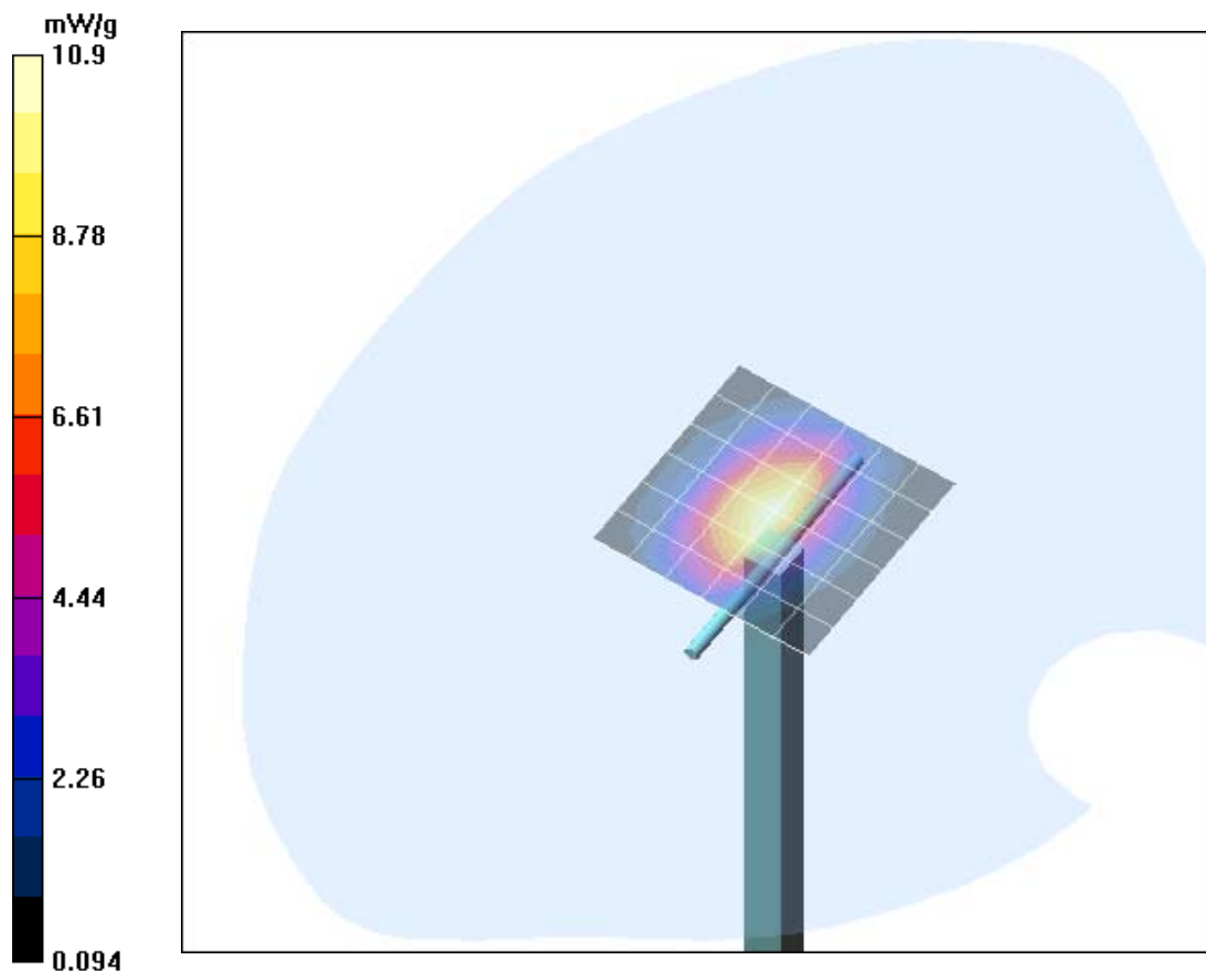
Fig. 14: Validation measurement 1900 MHz Head (June 27, 2005), coarse grid. Ambient Temperature: 22.0° C, Liquid Temperature: 21.0° C.
