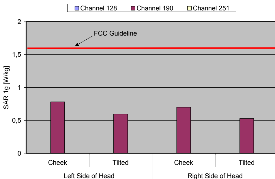
Fig. 8: The measured head phantom SAR values for the Siemens A76 for GSM 850 in comparison to the FCC exposure limit.
