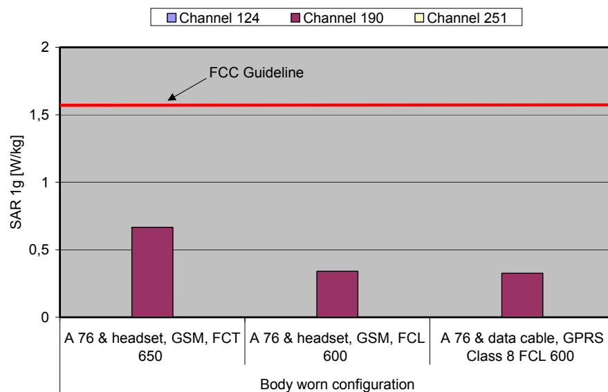
Fig. 10: The measured SAR values in body-worn configuration for the Siemens A76 for GSM 850 in comparison to the FCC exposure limit.
