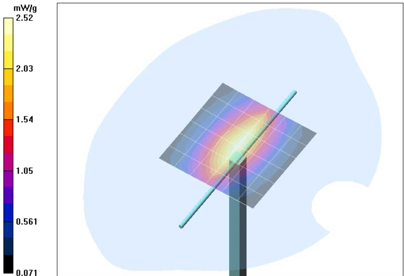
Fig. 12: Validation measurement 835 MHz Head (June 24, 2005), coarse grid. Ambient Temperature: 22.0° C, Liquid Temperature: 21.8° C.
