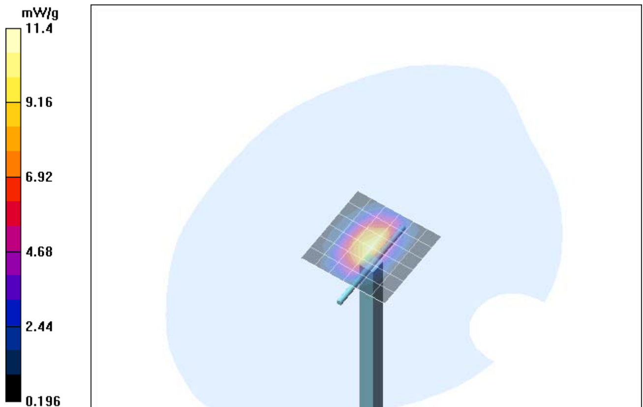
Fig. 15: Validation measurement 1900 MHz Body (June 21, 2005), coarse grid. Ambient Temperature: 22.0° C, Liquid Temperature: 21.0° C.
