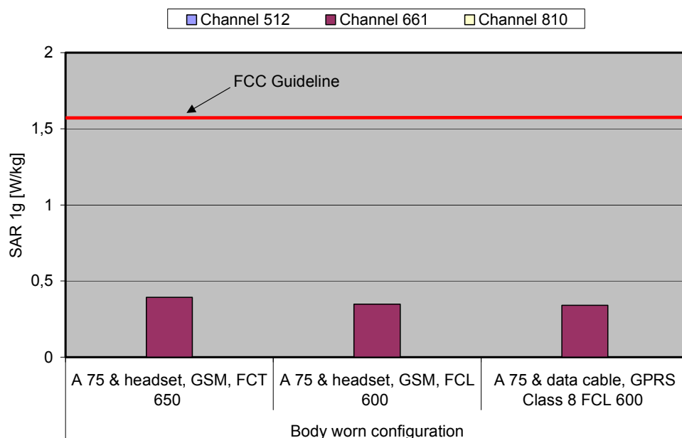
Fig. 9: The measured SAR values in body-worn configuration for the Siemens A75 for PCS 1900 in comparison to the FCC exposure limit.
