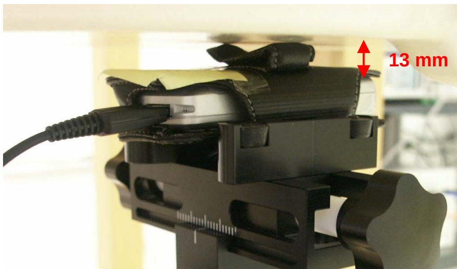
Fig. 23: Body worn configuration, GPRS mode (Class 8) with data cable, antenna towards the phantom and FCL 600 carry case.
