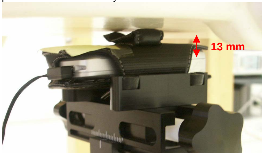
Fig. 22: Body worn configuration, GSM mode with headset, antenna towards the phantom and FCL 600 carry case.
