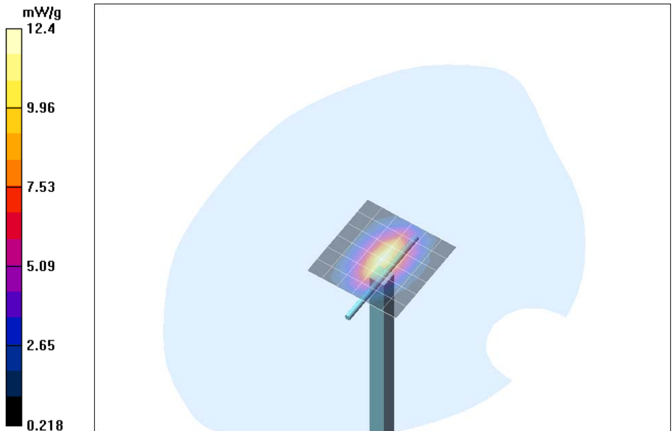
Fig. 11: Validation measurement 1900 MHz body (March 17, 2005), coarse grid. Ambient Temperature: 22.0° C, Liquid Temperature: 21.0° C.
