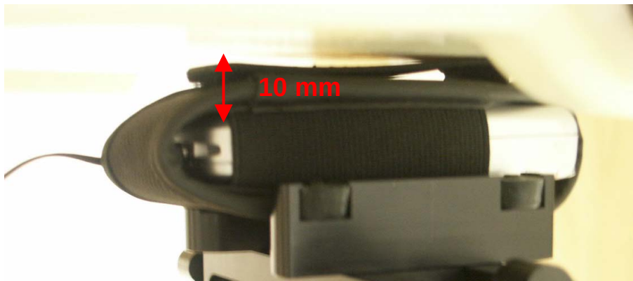
Fig. 21: Body worn configuration, GSM mode with headset, antenna towards the phantom and FCT 650 carry case.
