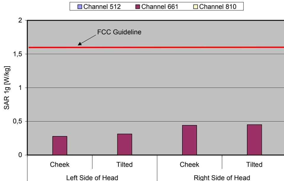
Fig. 8: The measured head phantom SAR values for the Siemens A75 for PCS 1900 in comparison to the FCC exposure limit.
