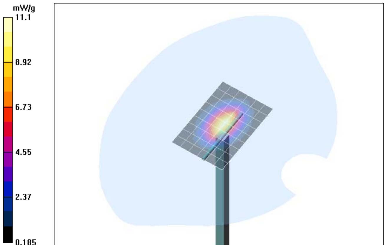
Fig. 10: Validation measurement 1900 MHz Head (March 16, 2005), coarse grid. Ambient Temperature: 22.0° C, Liquid Temperature: 21.0° C.
