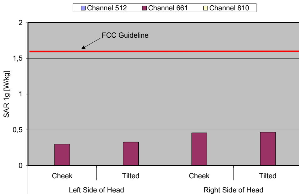
Fig. 9: The measured head phantom SAR values for the Siemens A71 for PCS 1900 in comparison to the FCC exposure limit.
