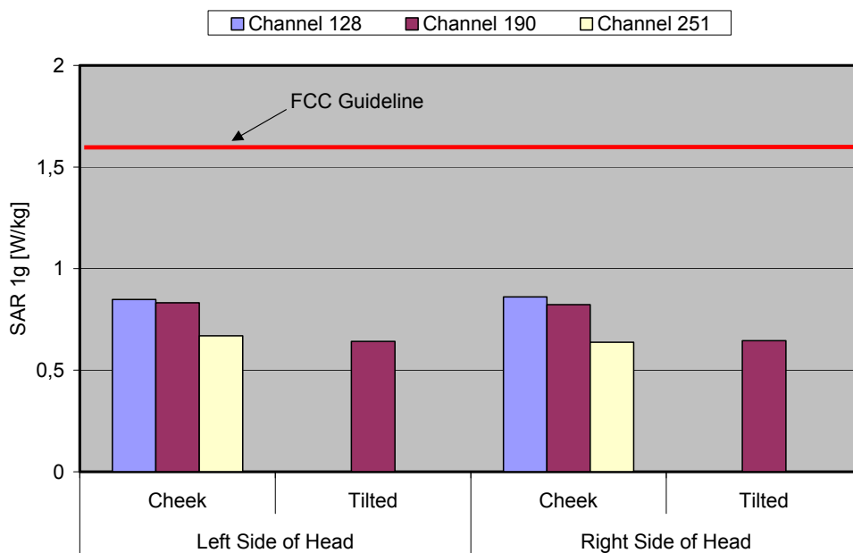
Fig. 8: The measured head phantom SAR values for the Siemens A71 for GSM 850 in comparison to the FCC exposure limit.
