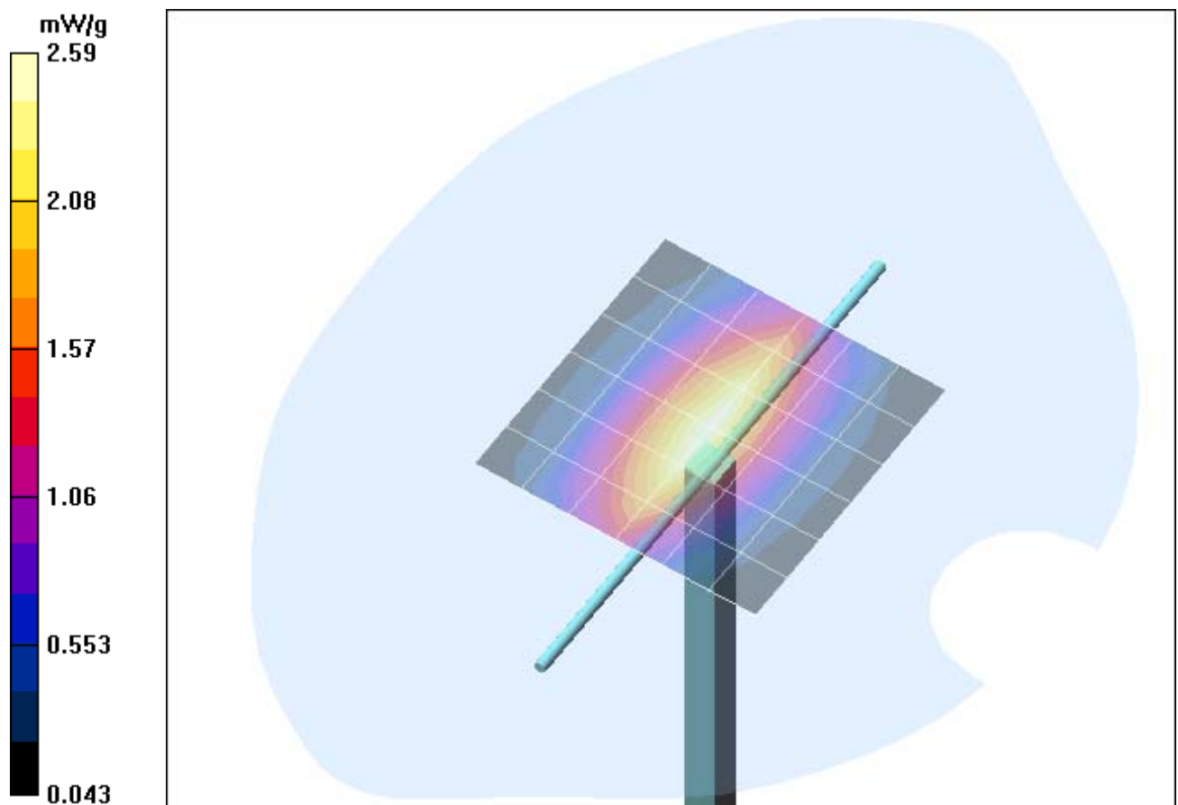
Fig. 13: Validation measurement 835 MHz Body (July 05, 2005), coarse grid. Ambient Temperature: 22.5° C, Liquid Temperature: 21.9° C.
