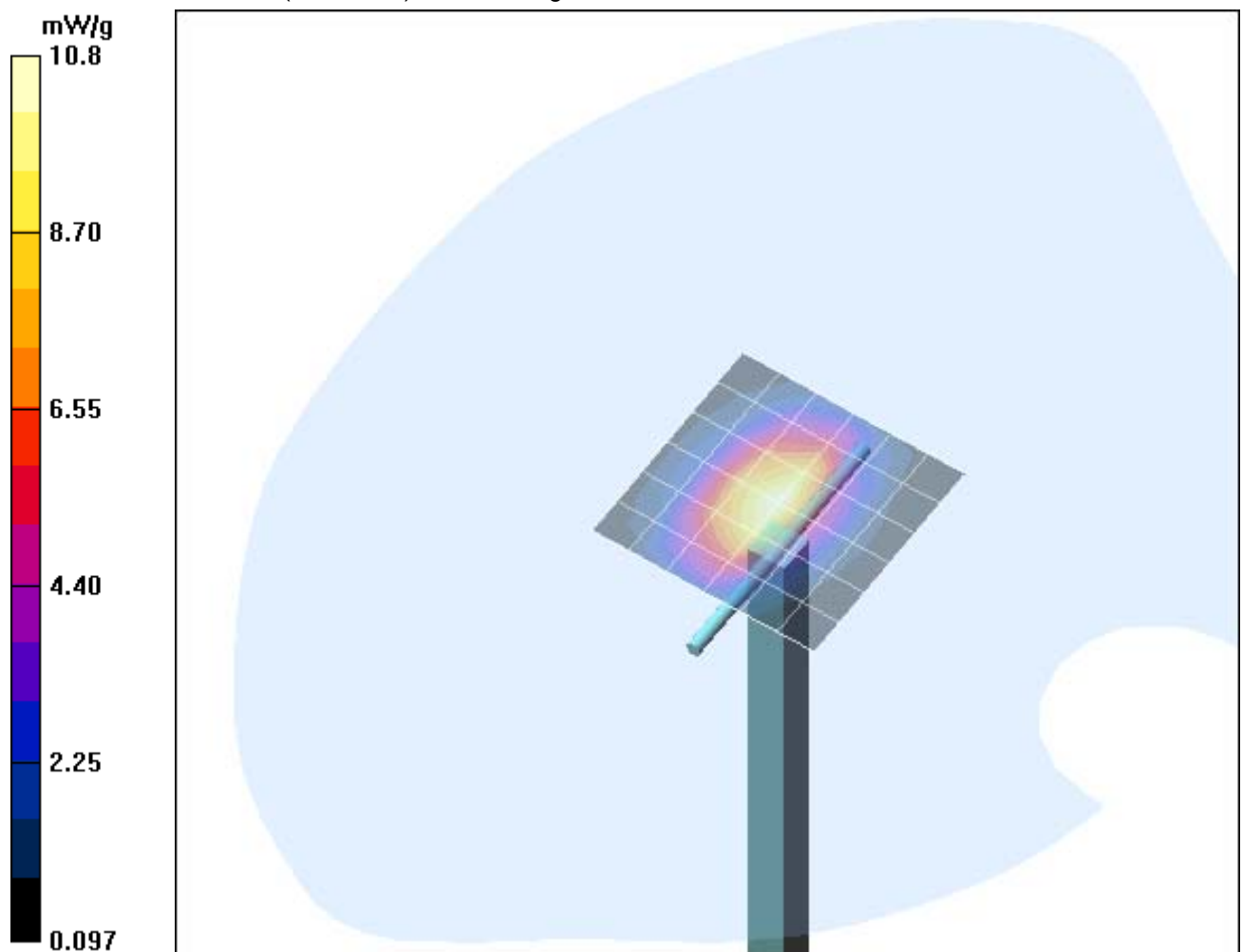
Fig. 14: Validation measurement 1900 MHz Head (July 04, 2005), coarse grid.
