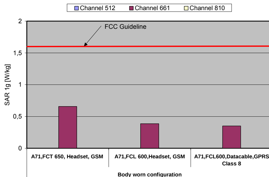
Fig. 11: The measured SAR values in body-worn configuration for the Siemens A71 for PCS 1900 in comparison to the FCC exposure limit.
