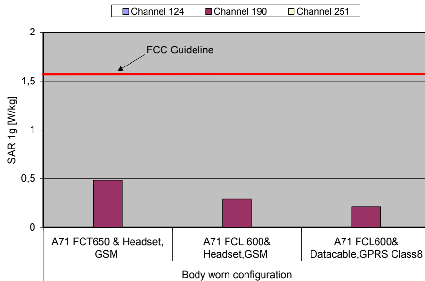
Fig. 10: The measured SAR values in body-worn configuration for the Siemens A71 for GSM 850 in comparison to the FCC exposure limit.
