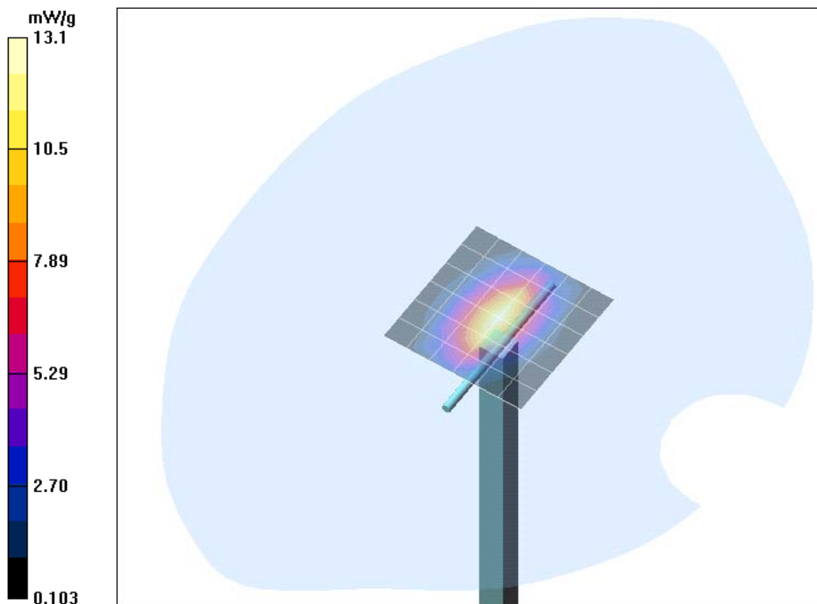
Fig. 15: Validation measurement 1900 MHz Body (July 07, 2005), coarse grid. Ambient Temperature: 22.0° C, Liquid Temperature: 21.0° C.
