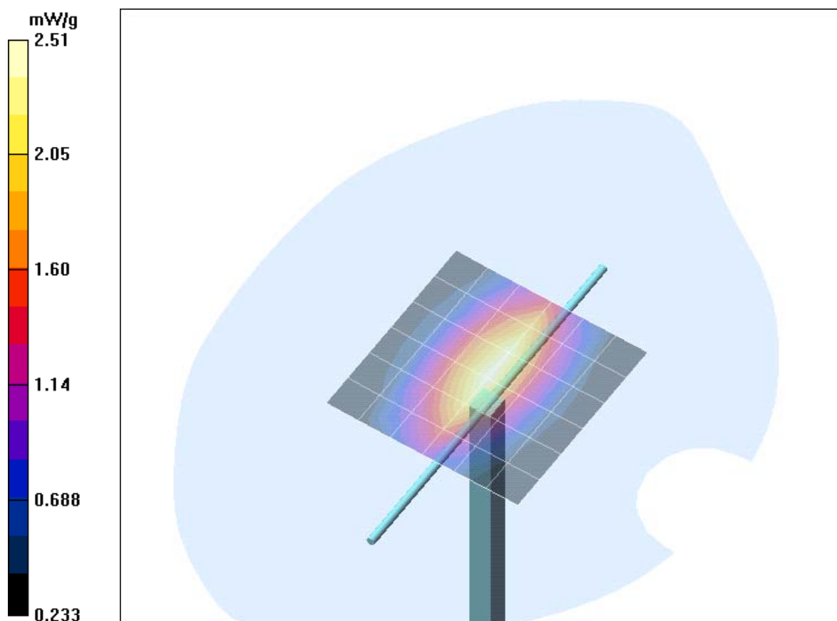
Fig. 12: Validation measurement 835 MHz Head (July 01, 2005), coarse grid. Ambient Temperature: 22.0° C, Liquid Temperature: 21.8° C.
