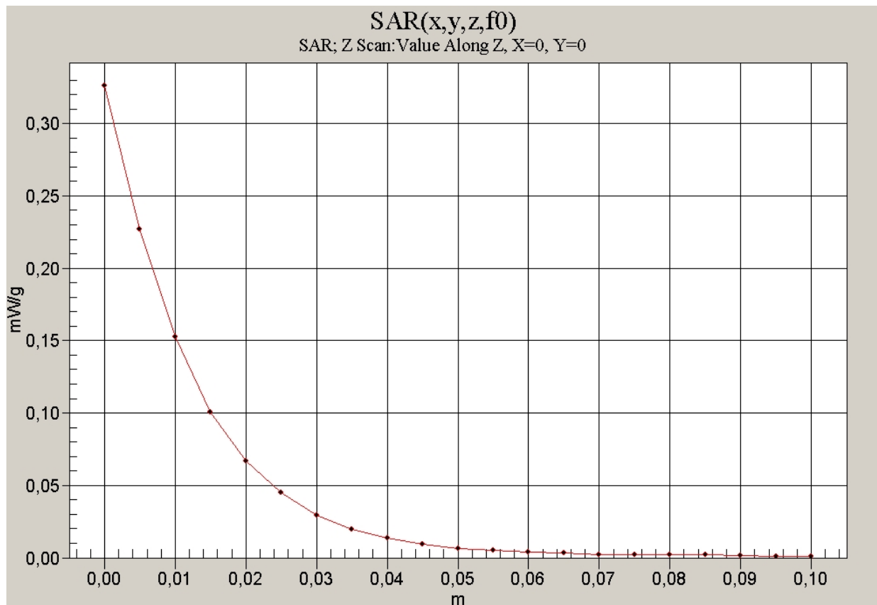
1900 MHz body
