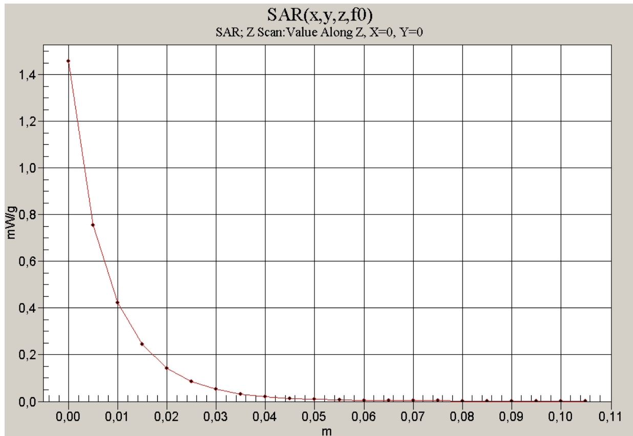
1900 MHz head
