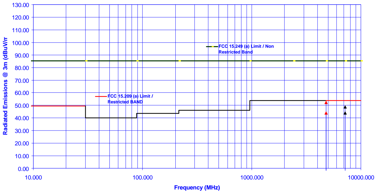
Transmitter Radiated Emissions Measurements at 3 Meter OFTS AeroComm Inc. 2.4 GHz HFSS OEM Transceiver Model PKLR2400 TRANSMIT Freq.: 2402 MHz
