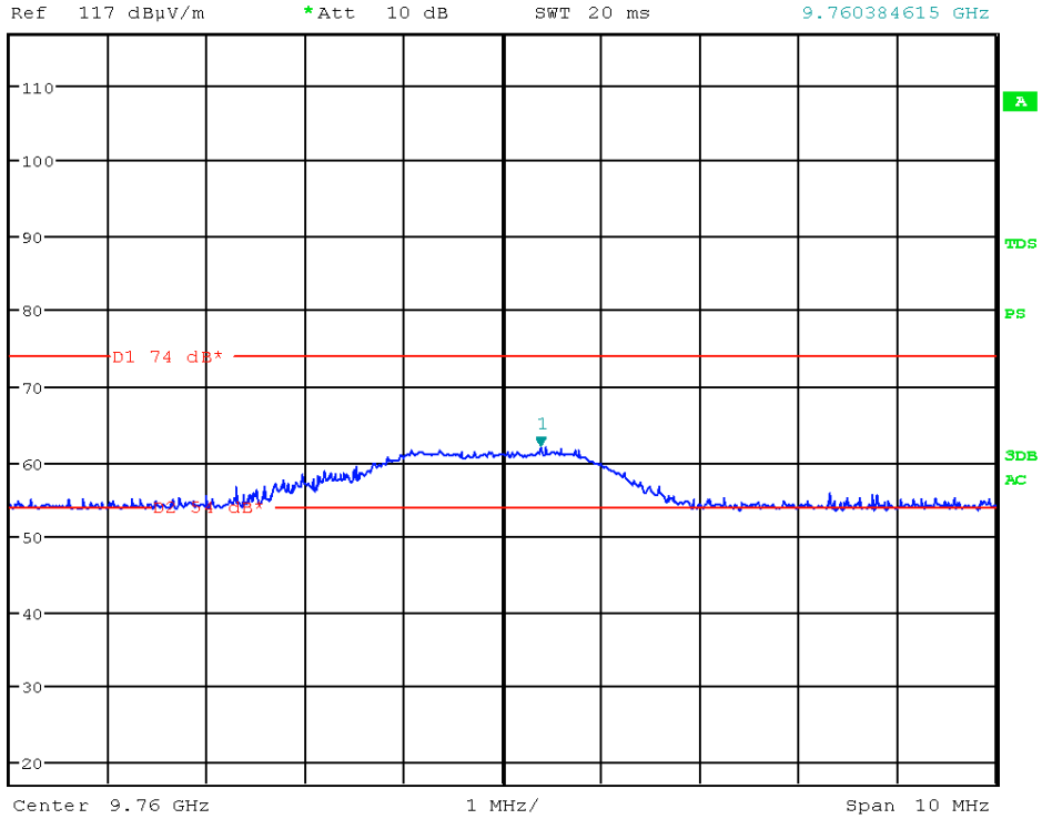
Picture 55: spurious emission, Channel mid - PK
