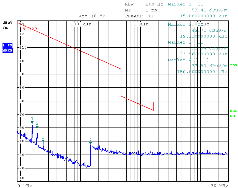
Picture 36: Radiated emission 9 kHz – 30MHz (Channel low)
