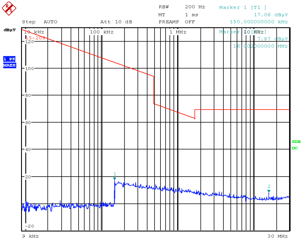
Picture 25: spurious emission, channel mid (9 kHz - 30 MHz)
