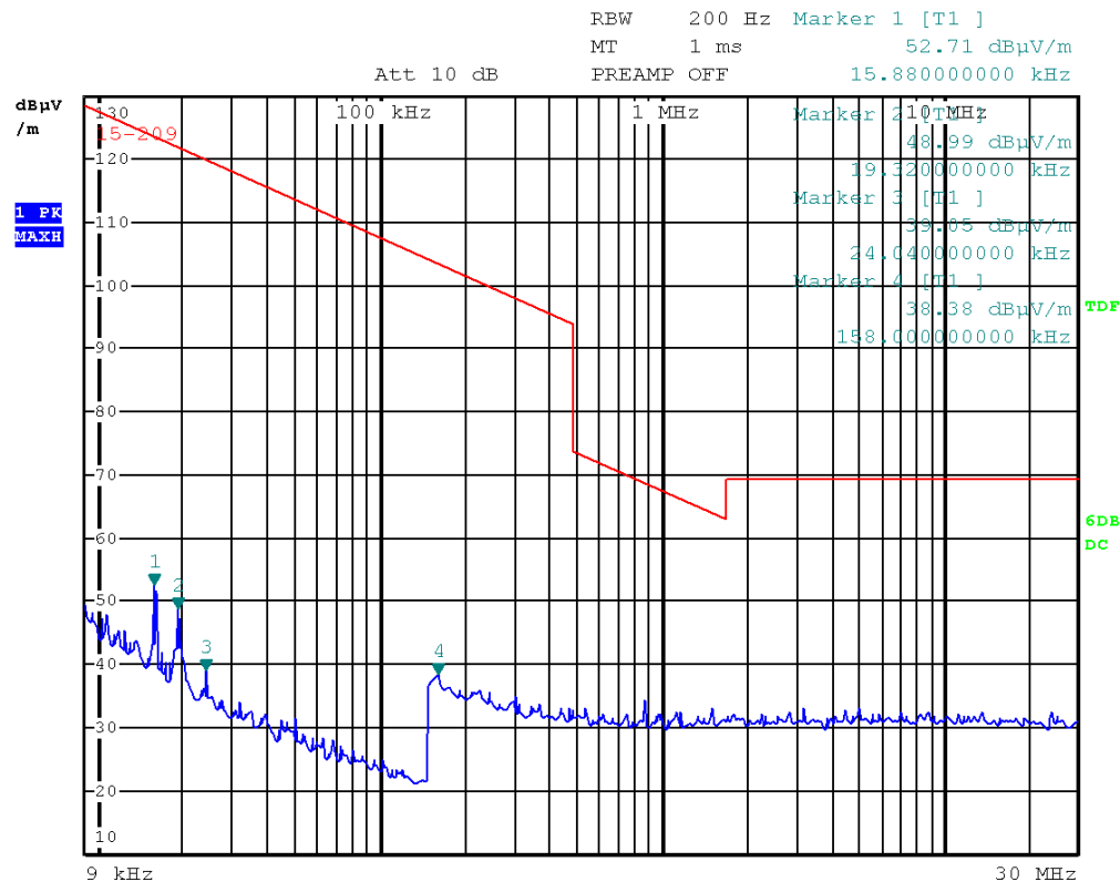
Picture 37: Radiated emission 9 kHz – 30MHz (Channel mid)
