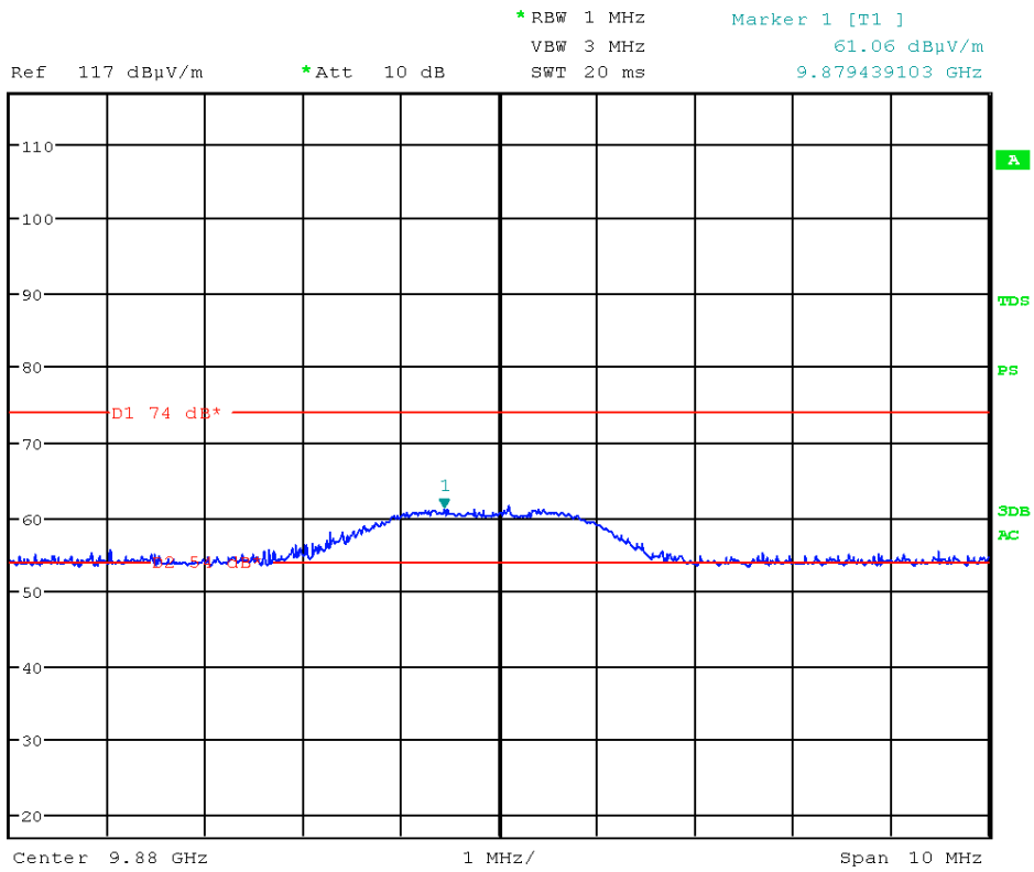
Picture 61: spurious emission, Channel mid - PK
