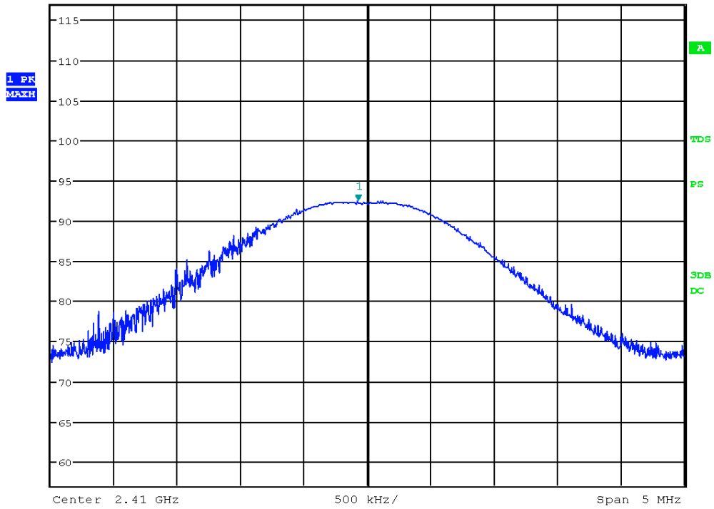
Picture 43: spurious emission, Channel low - PK
