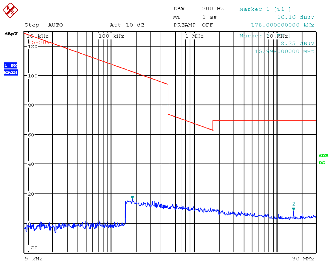
Picture 24: spurious emission, channel low (9 kHz - 30 MHz)
