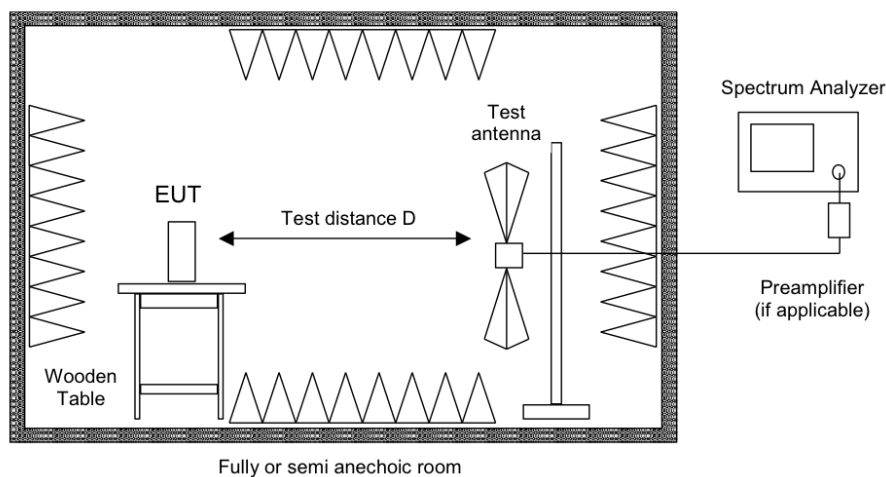
Picture 42: Test setup for radiated emission measurement (> 1 GHz)
