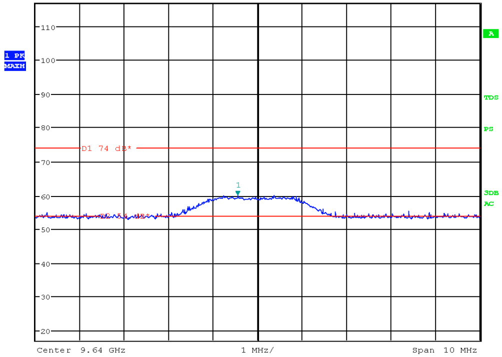
Picture 49: spurious emission, Channel low - PK
