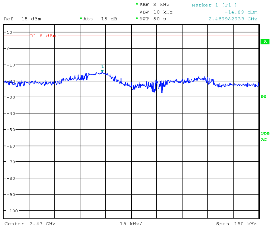
Picture 15: Power spectral density, channel high - zoom to maximum
