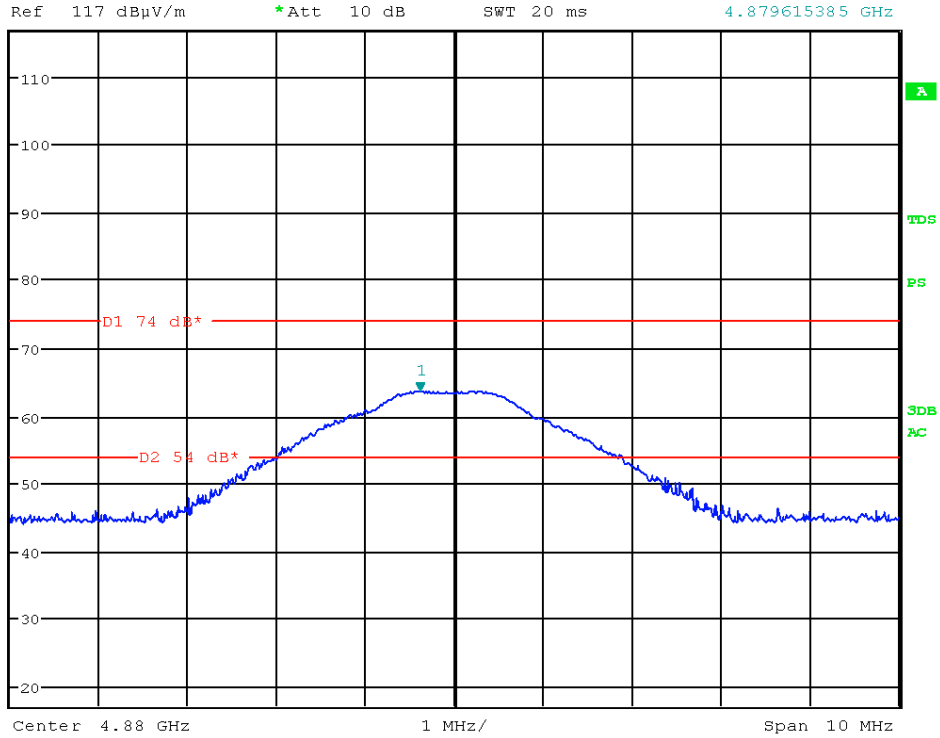
Picture 53: spurious emission, Channel mid - PK
