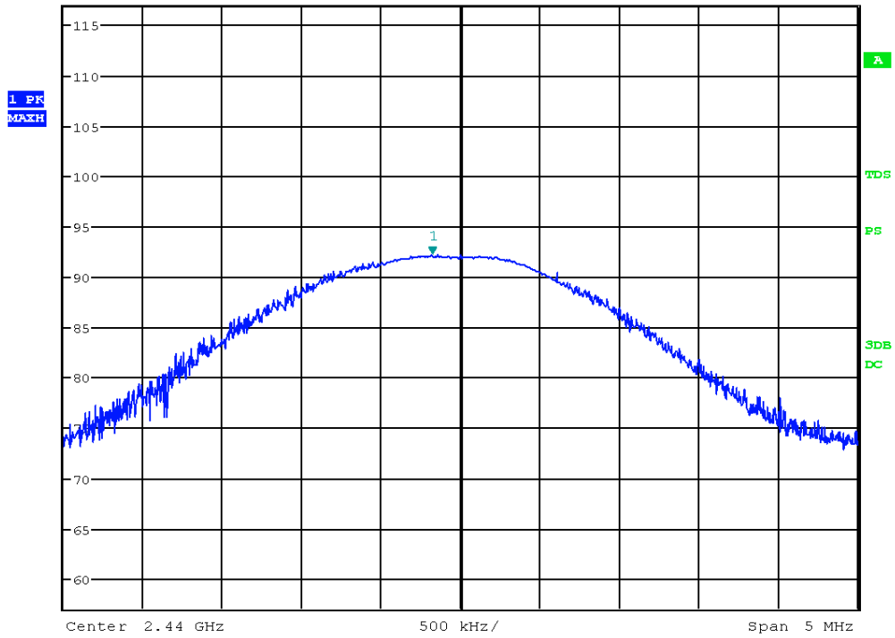
Picture 51: spurious emission, Channel mid - PK
