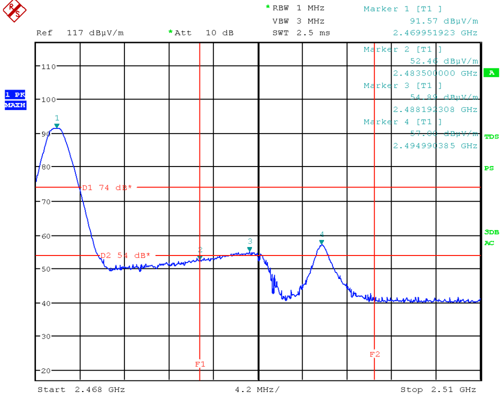
Picture 21: upper edge (PK) with channel high
