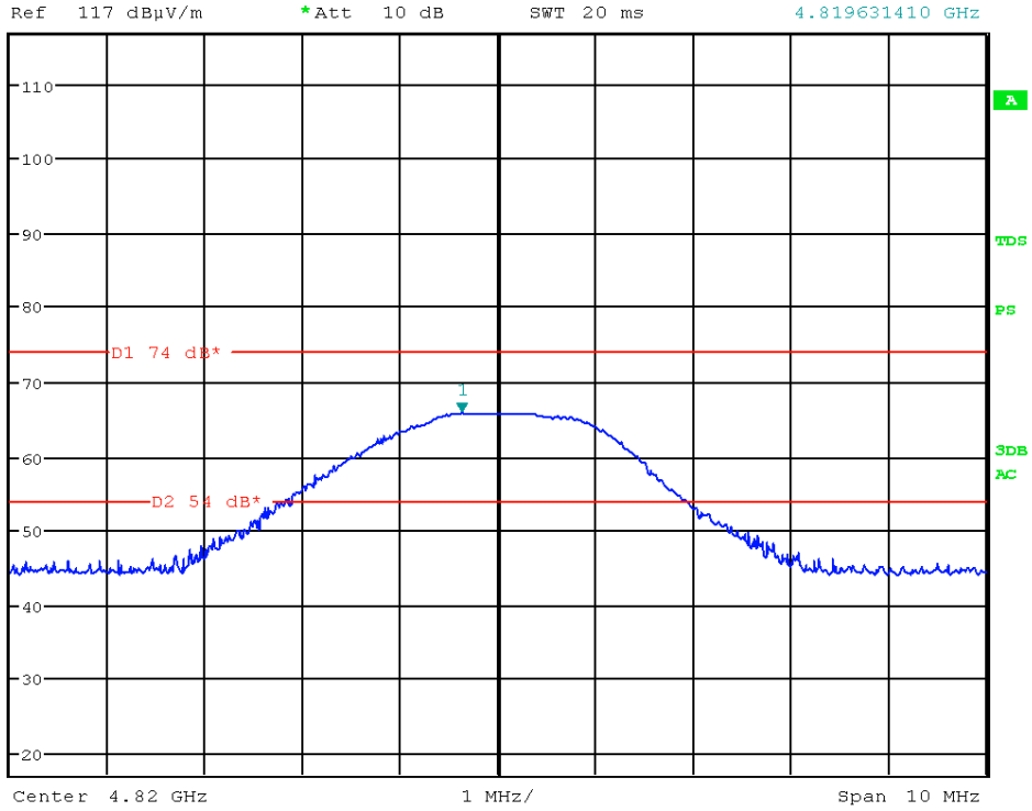
Picture 45: spurious emission, Channel low - PK
