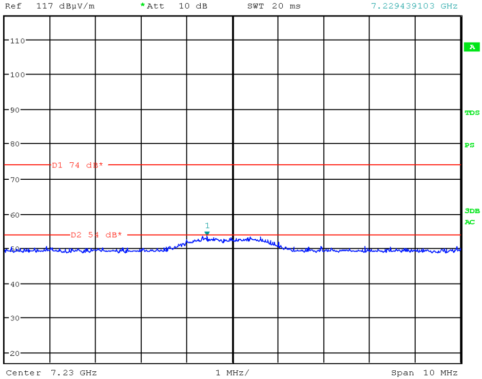
Picture 47: spurious emission, Channel low - PK
