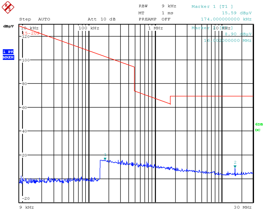
Picture 26: spurious emission, channel high (9 kHz - 30 MHz)
