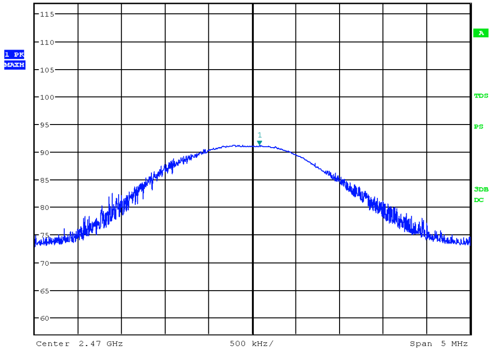
Picture 57: spurious emission, Channel high - PK
