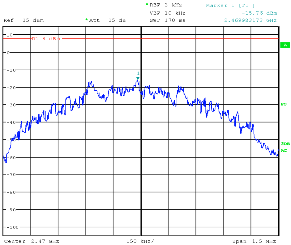
Picture 14: Power spectral density, channel high - complete carrier
