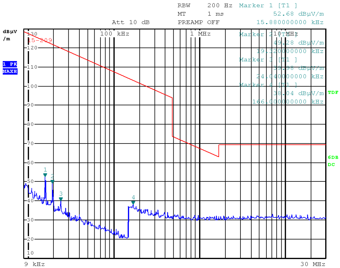
Picture 38: Radiated emission 9 kHz – 30MHz (Channel high)
