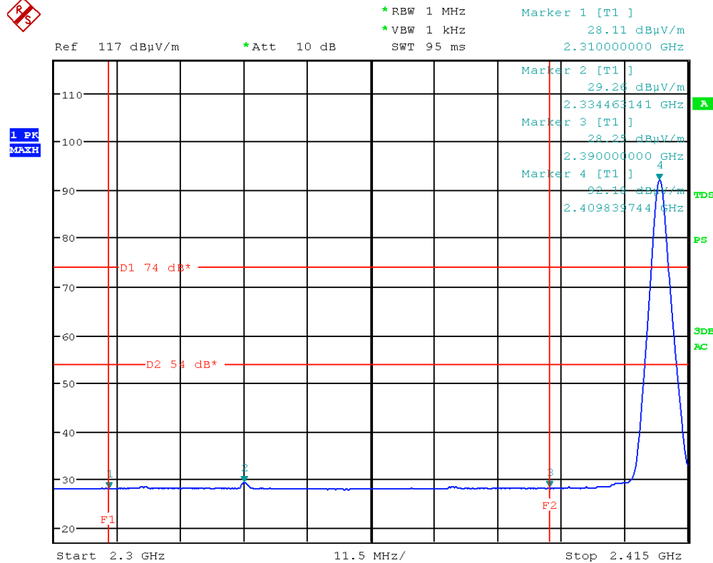
Picture 20: lower edge (AV) with channel low
