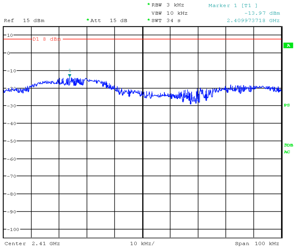
Picture 11: Power spectral density, channel low - zoom to maximum
