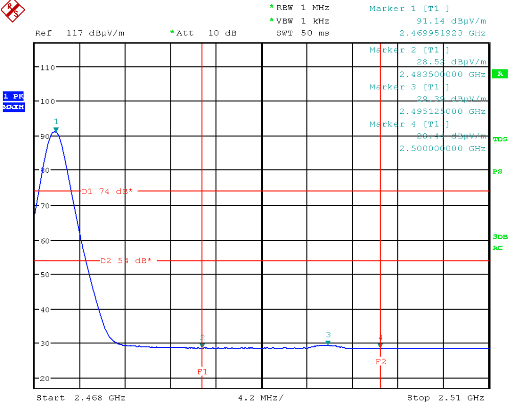
Picture 22: upper edge (AV) with channel high
