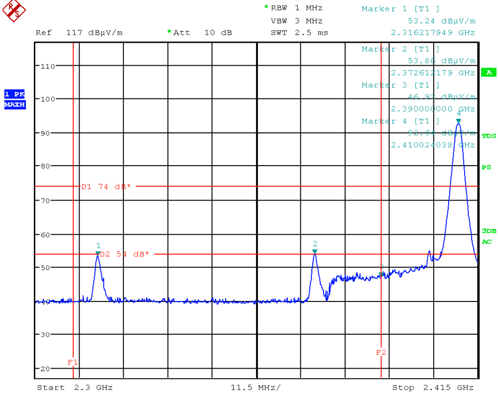
Picture 19: lower edge (PK) with channel low
