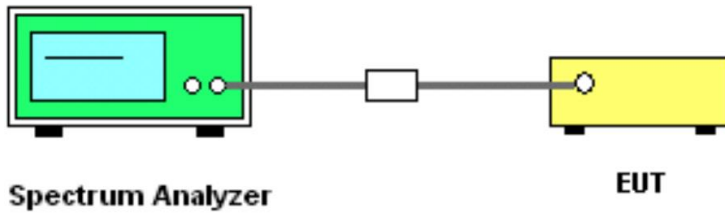
Picture 1: Test setup for 6 dB bandwidth measurement
