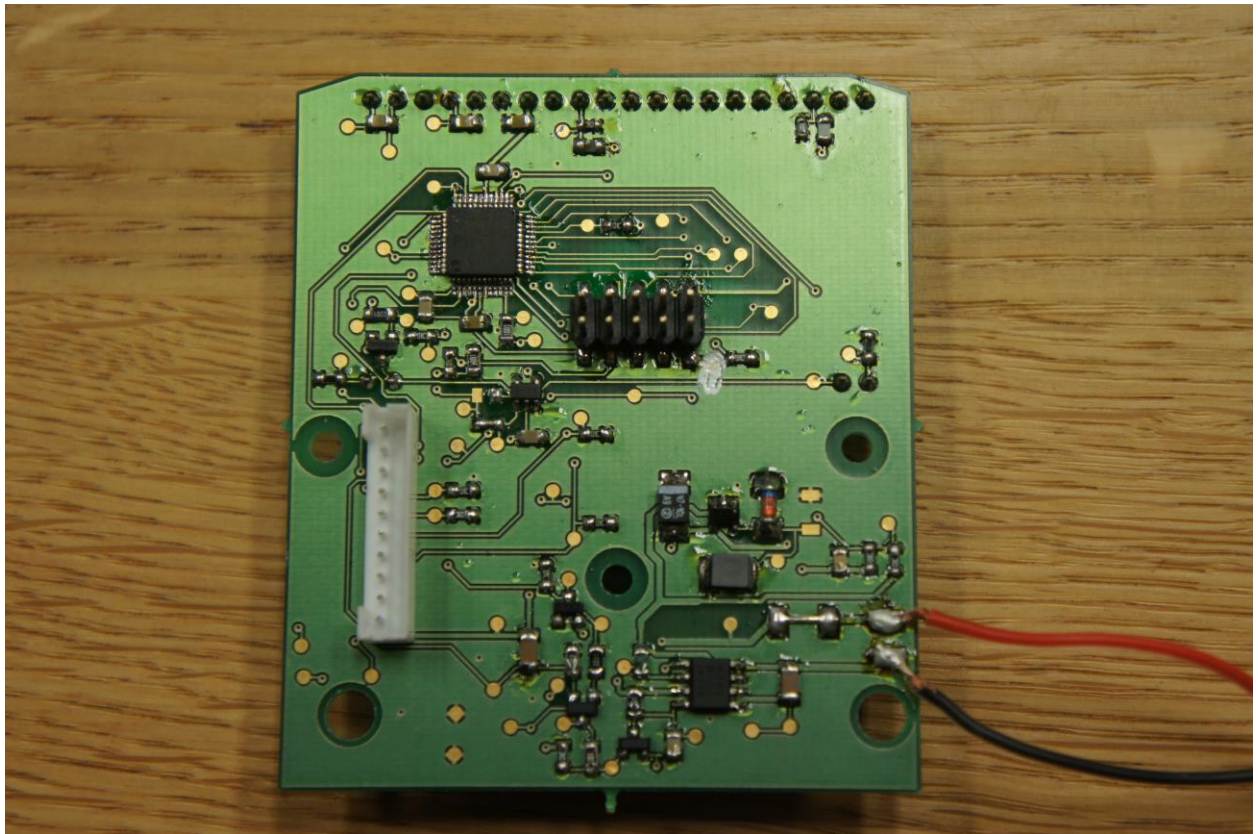
Picture 5: Remote PCB back side
