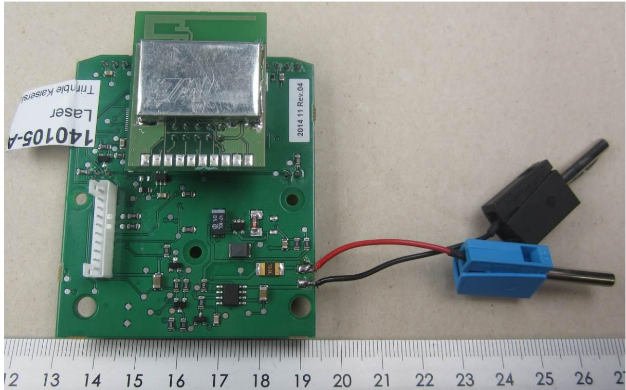
140852_06.JPG: Carrier Board + EUT – Bottom View
