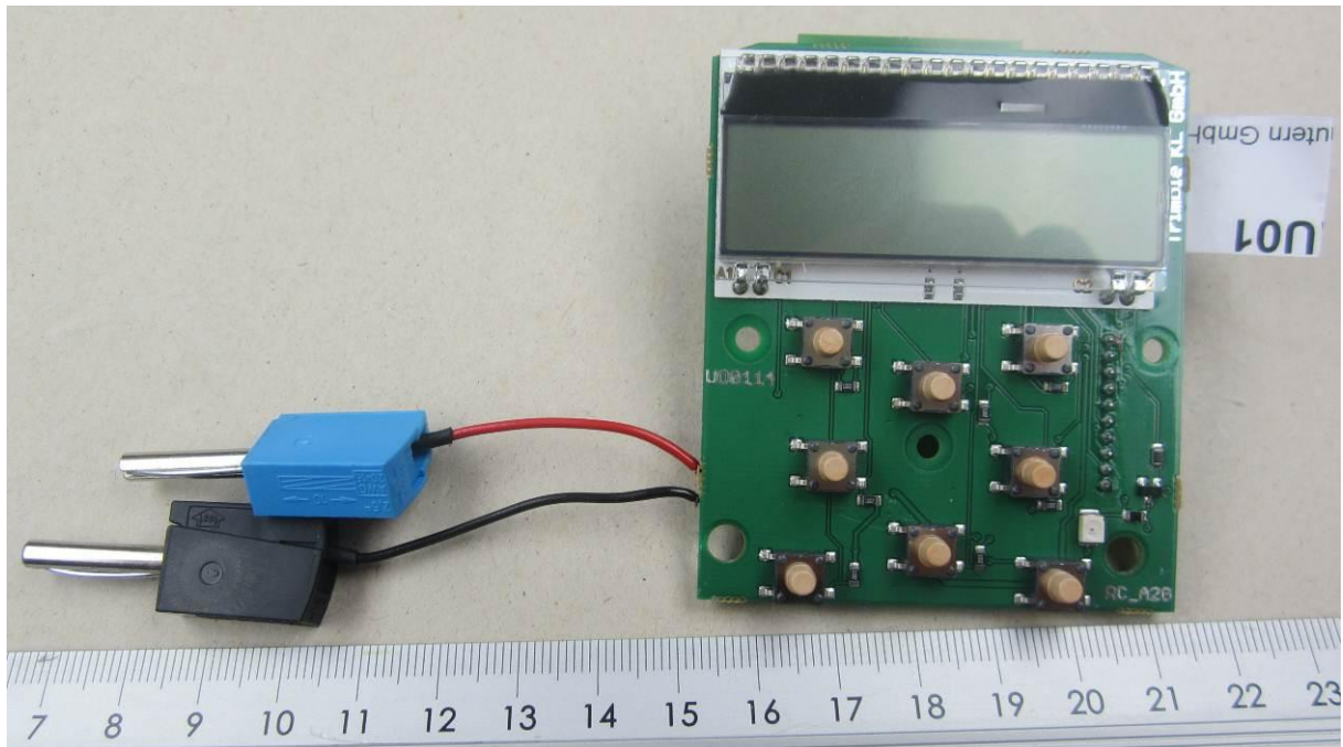
140852_05.jpg: Carrier Board + EUT – Top View
