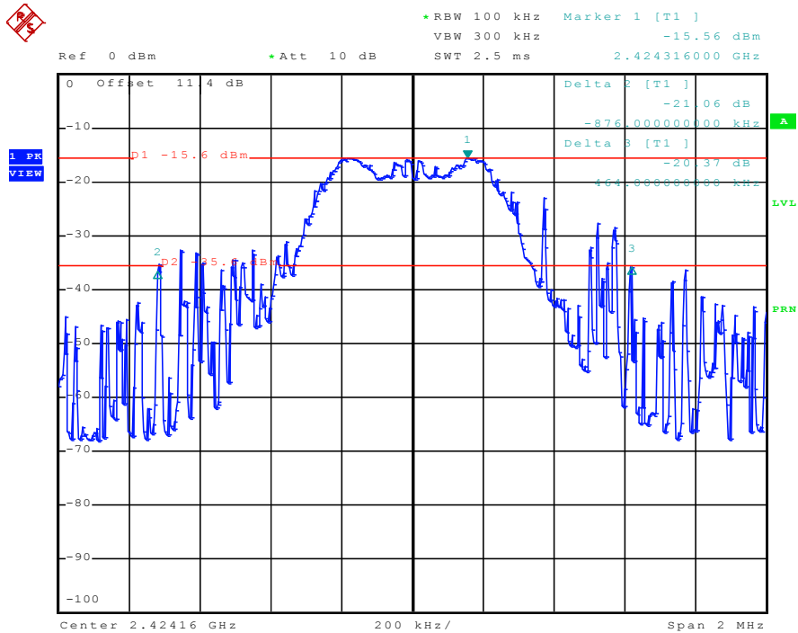
Plot 1b : mid channel 20 dB emission bandwidth
