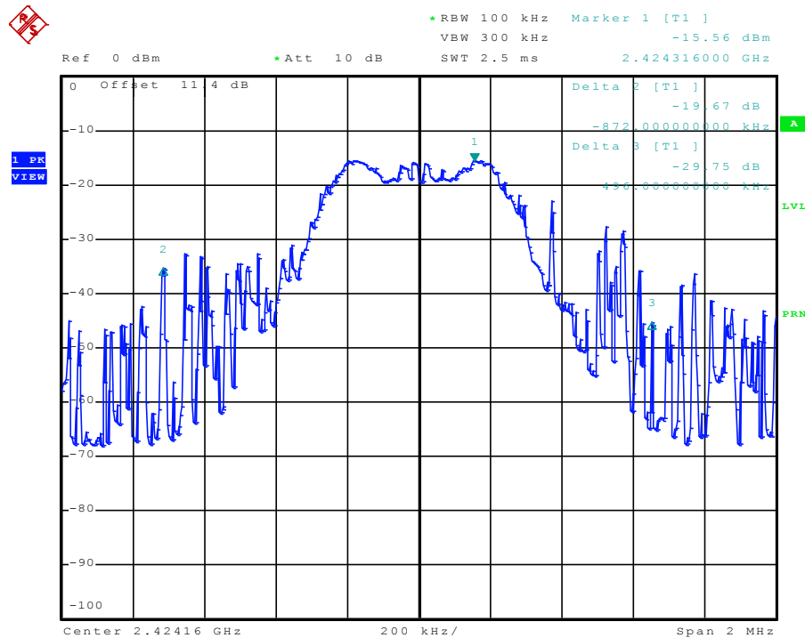
Plot 2b: mid channel 99% occupied bandwidth
