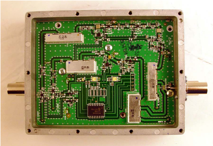
Board 1 - Bottom
