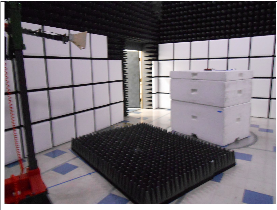
RF Radiated #2
