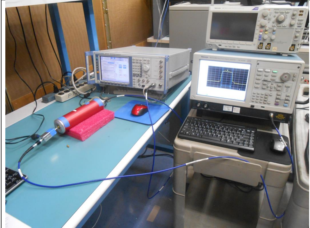
RF Conducted #2
