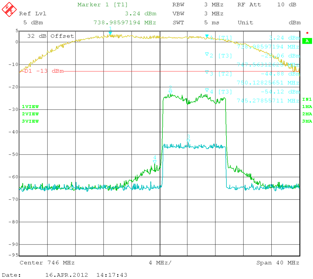
Figure 43: LTE – In vs. Out 751.00 MHz
