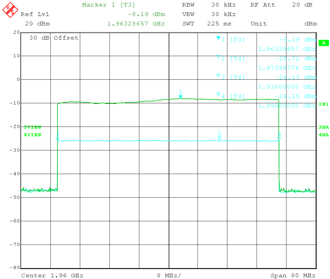
Figure 54. Frequency response (1930 – 1990) MHz band
