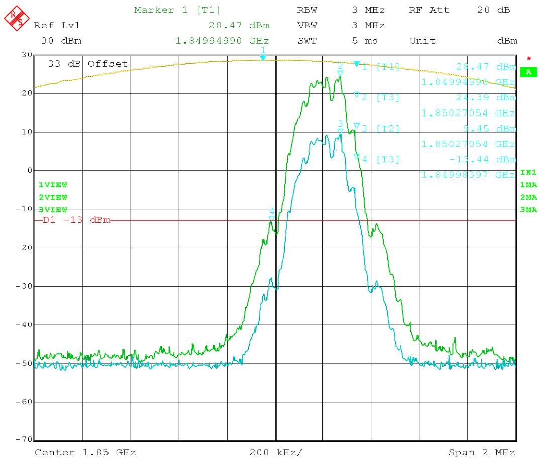
Figure 13: GSM – In vs. Out 1850.20MHz
