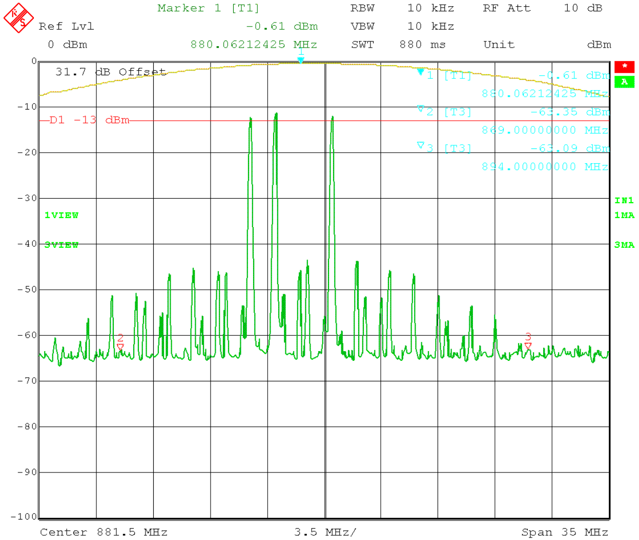
Figure 52: GSM 3 tones intermodulation - (869 – 894) MHz
