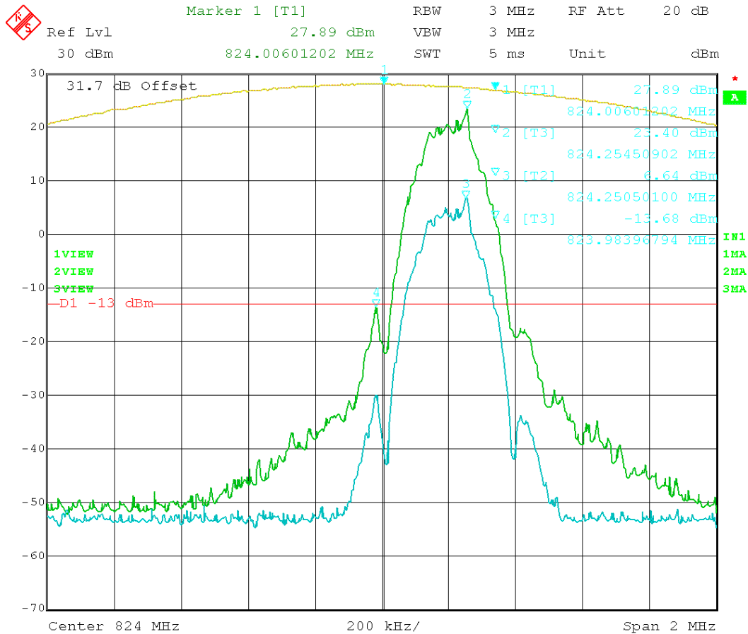
Figure 37: EDGE – In vs. Out 824.20 MHz
