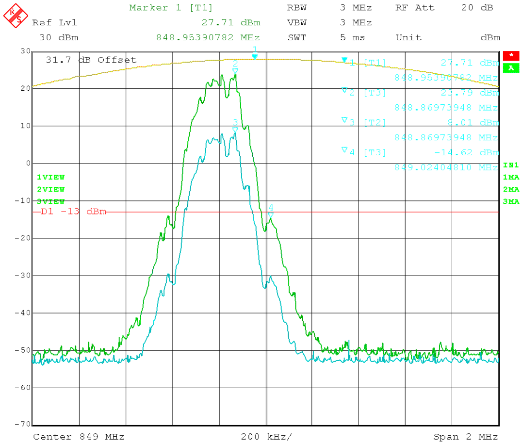
Figure 34: GSM – In vs. Out 848.8 MHz
