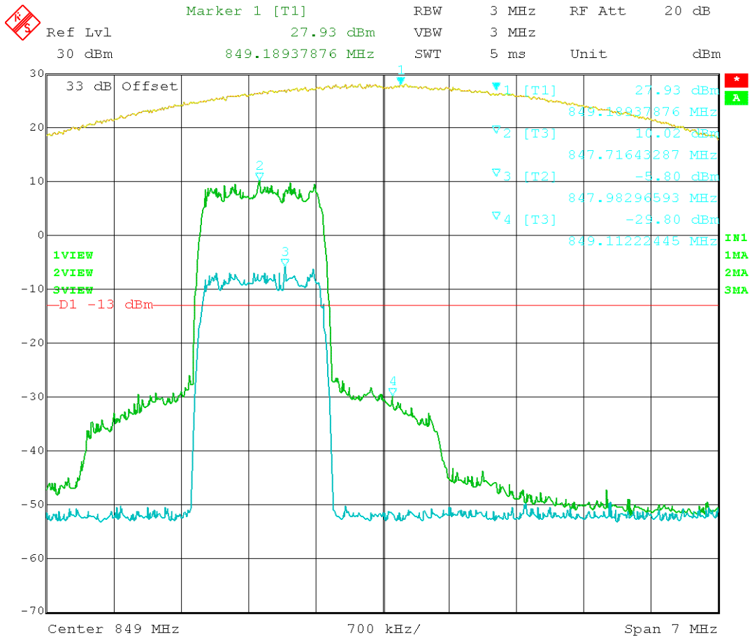
Figure 22: CDMA – In vs. Out 847.75 MHz
