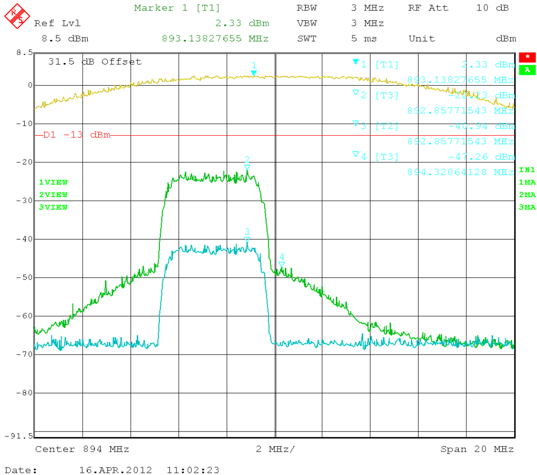
Figure 28: WCDMA – In vs. Out 893.50 MHz
