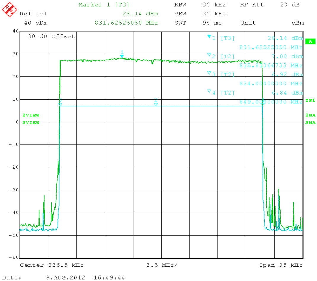
Figure 89. Frequency response (824 – 849) MHz band
