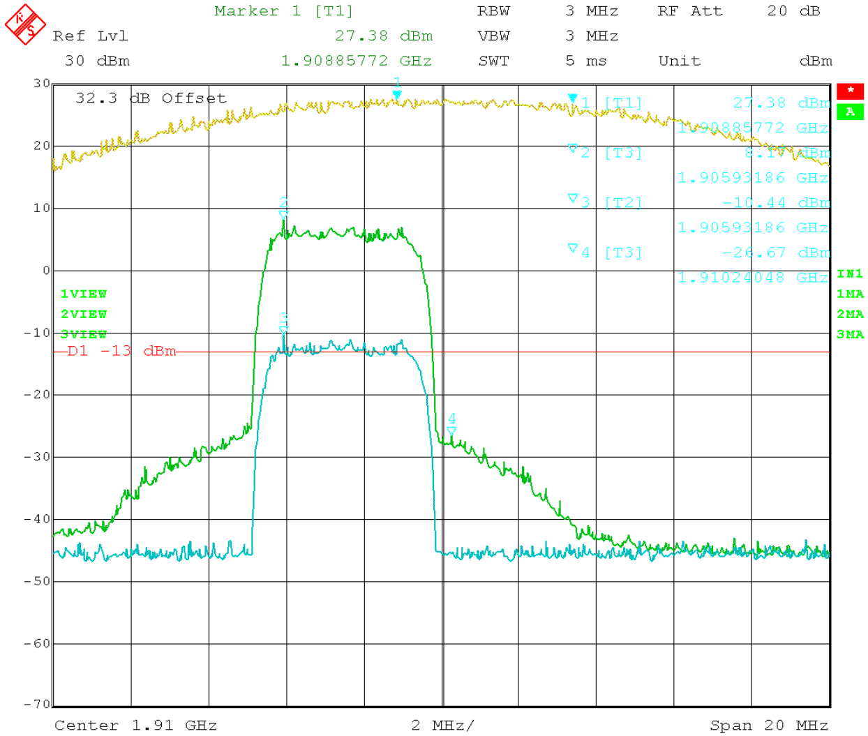
Figure 10: HSPA – In vs. Out 1907.50 MHz
