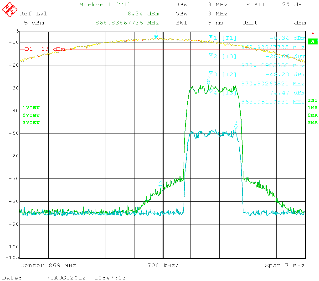
Figure 55: EVDO – In vs. Out 870.25 MHz
