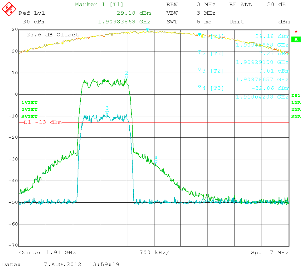
Figure 6: EVDO – In vs. Out 1908.75MHz
