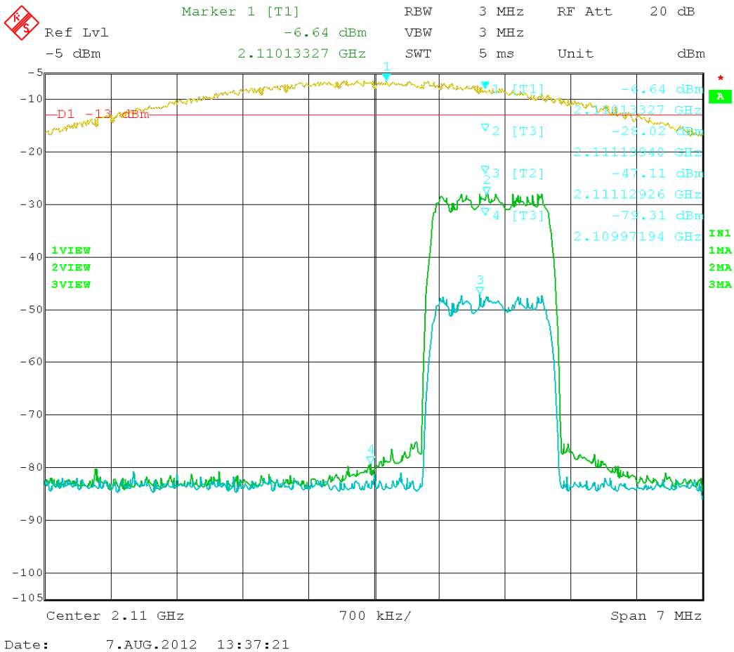
Figure 31: EVDO – In vs. Out 2111.25MHz
