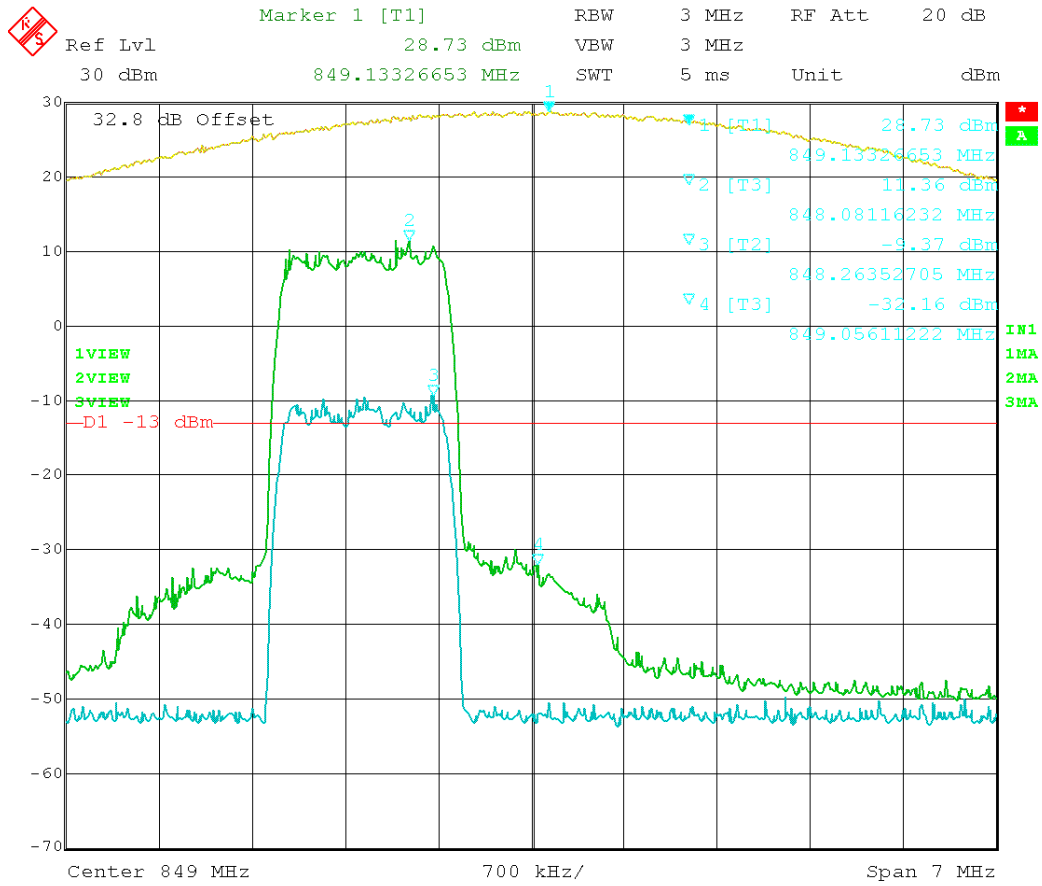
Figure 50: CDMA – In vs. Out 847.75 MHz
