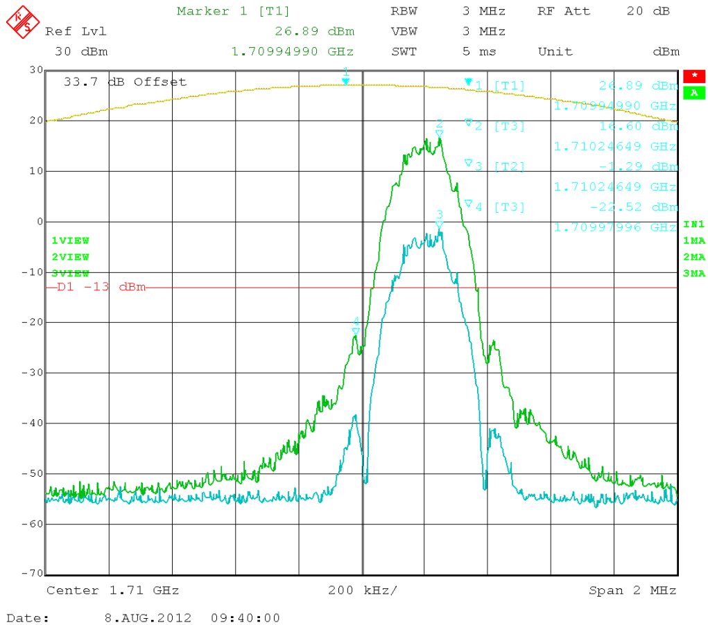
Figure 45: EDGE – In vs. Out 1710.20MHz
