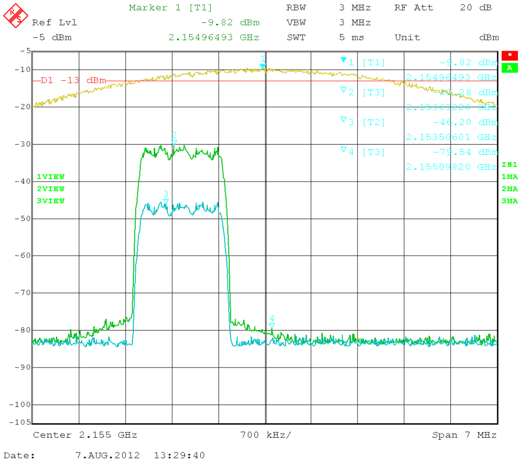
Figure 32: EVDO – In vs. Out 2153.75MHz
