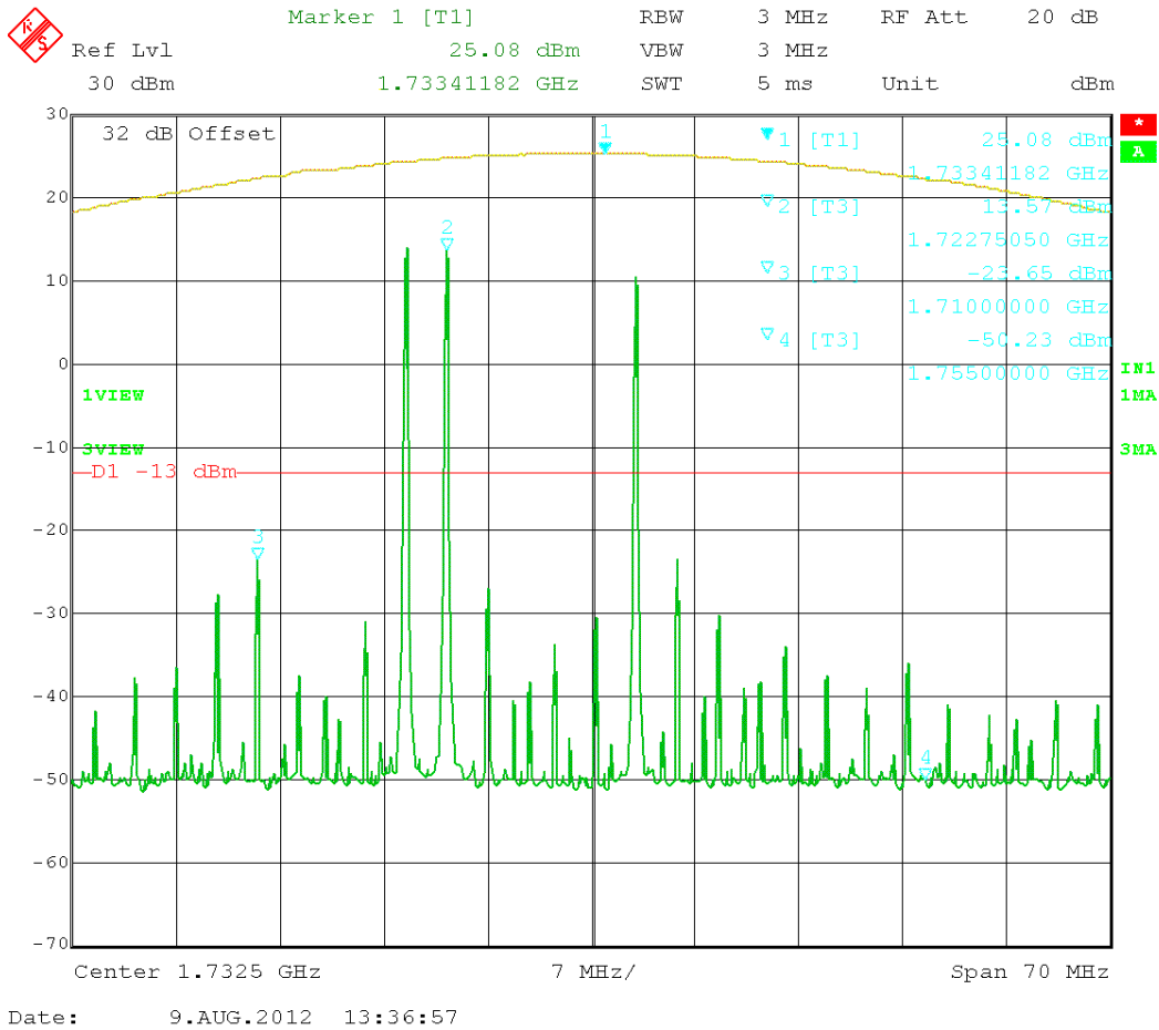
Figure 81: GSM 3 tones intermodulation - (1710 – 1755) MHz
