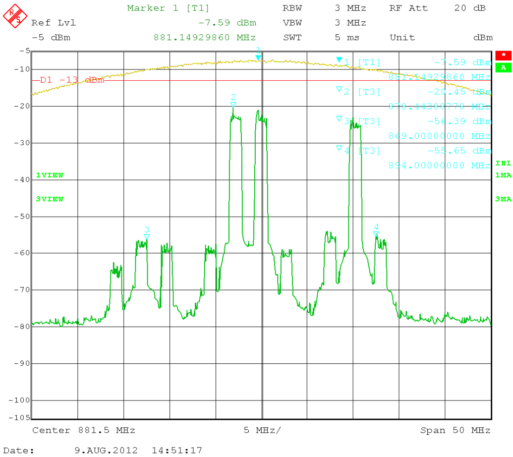
Figure 78: CDMA 3 tones intermodulation - (869 – 894) MHz.
