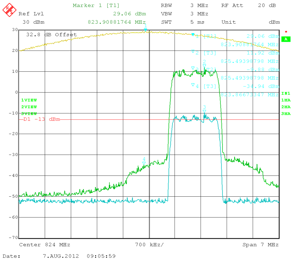
Figure 49: CDMA – In vs. Out 825.25MHz
