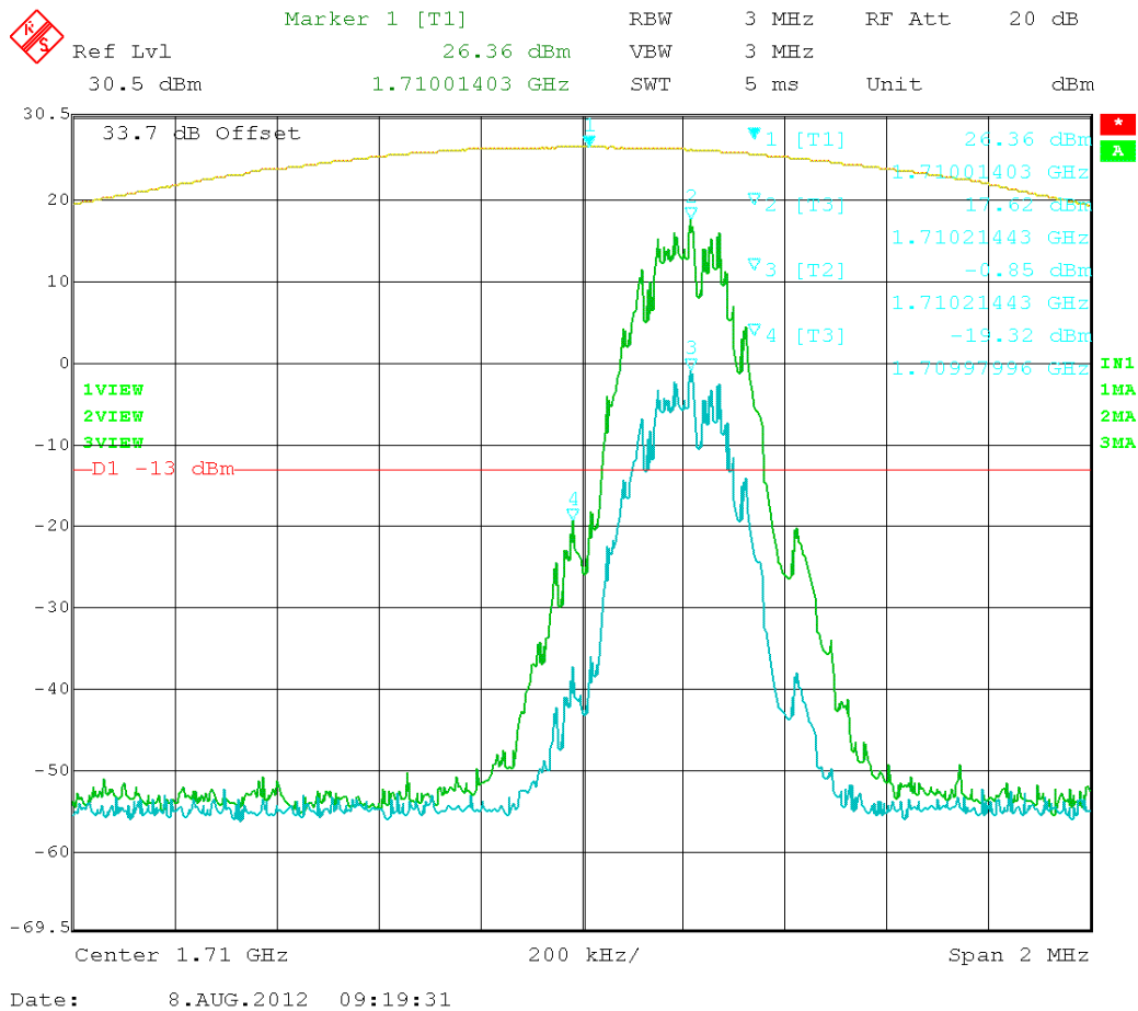
Figure 41: GSM – In vs. Out 1710.20MHz
