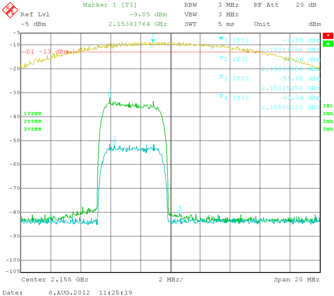
Figure 36: HSPA – In vs. Out 2152.50 MHz
