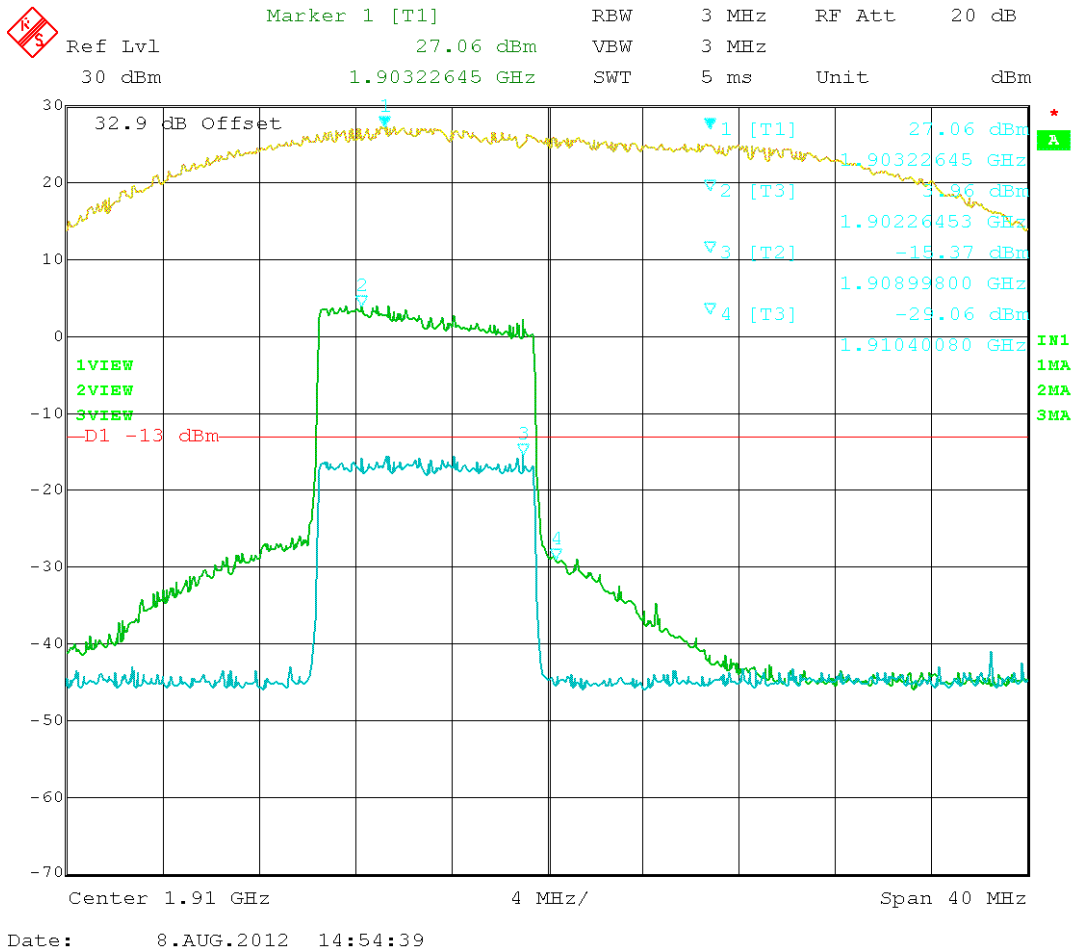
Figure 14: LTE – In vs. Out 1905.00MHz
