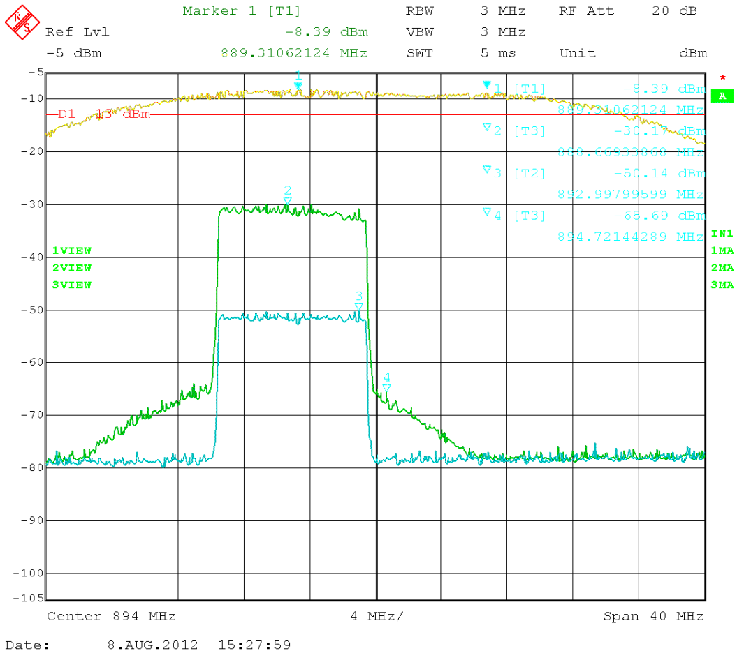
Figure 64: LTE – In vs. Out 889.00 MHz
