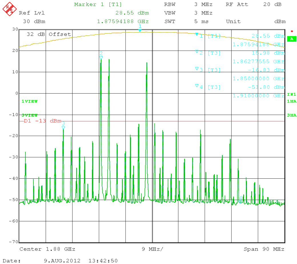
Figure 79: GSM 3 tones intermodulation - (1850 – 1910) MHz
