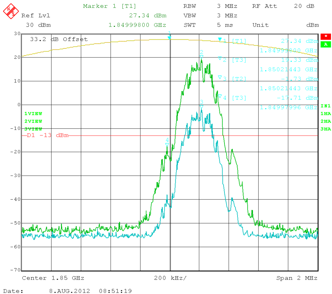
Figure 21: EDGE – In vs. Out 1850.20MHz
