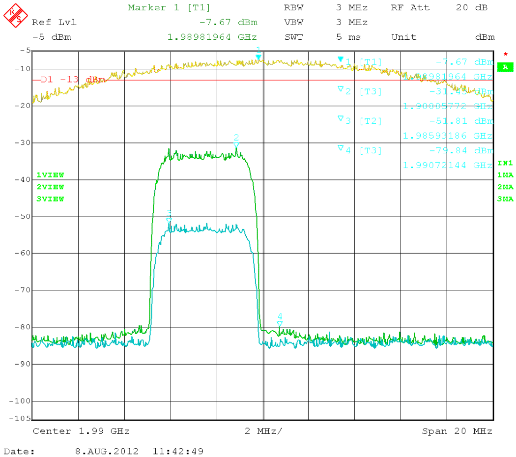
Figure 12: HSPA – In vs. Out 1987.50 MHz
