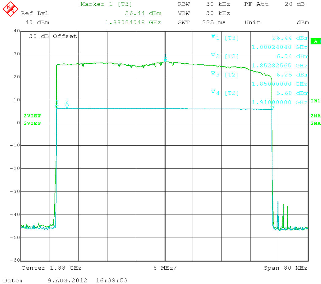
Figure 85. Frequency response (1850 – 1910) MHz band
