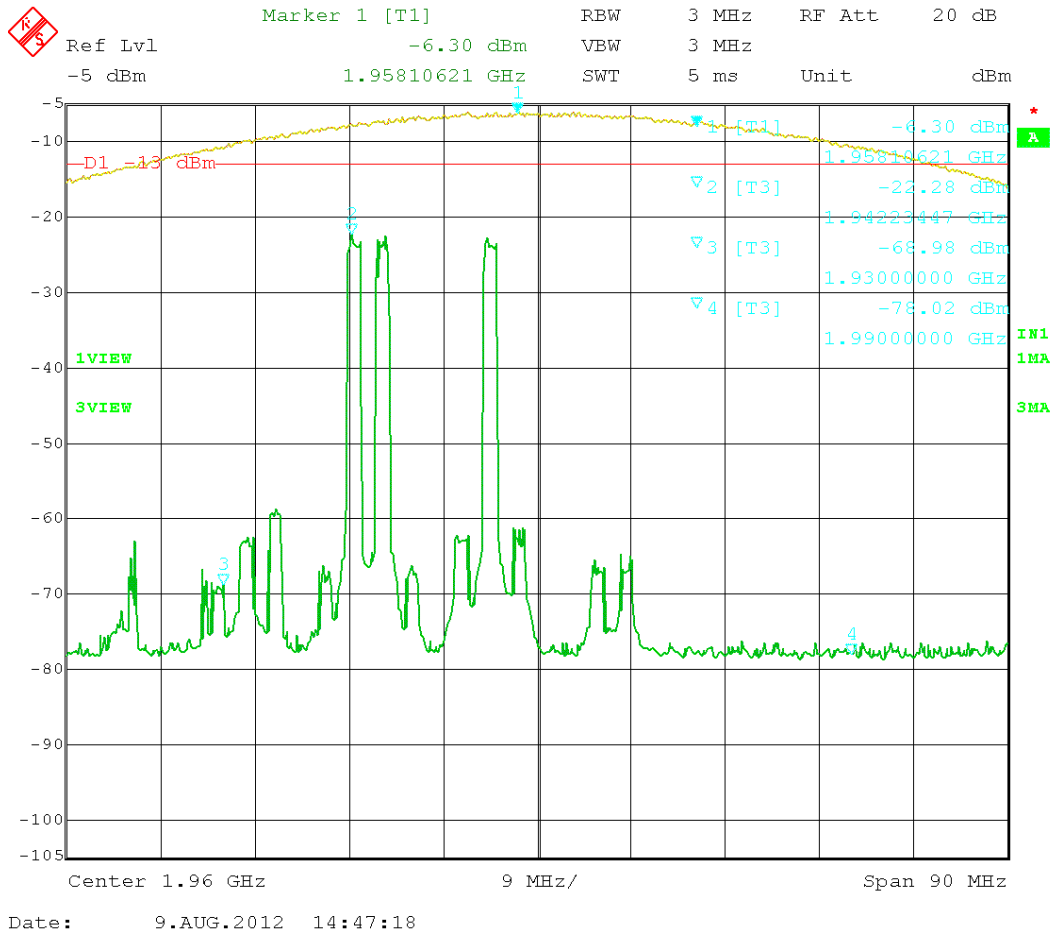
Figure 74: CDMA 3 tones intermodulation - (1930 – 1990) MHz.
