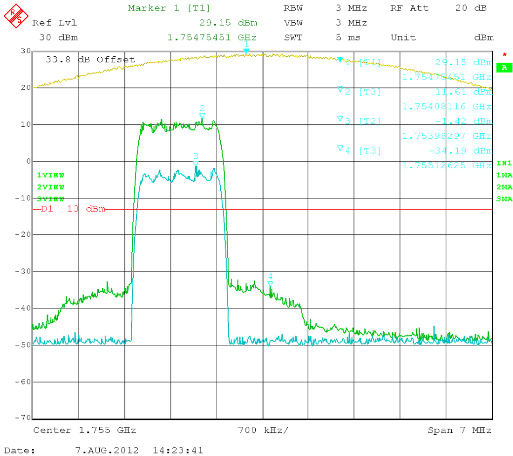
Figure 26: CDMA – In vs. Out 1.755 GHz
