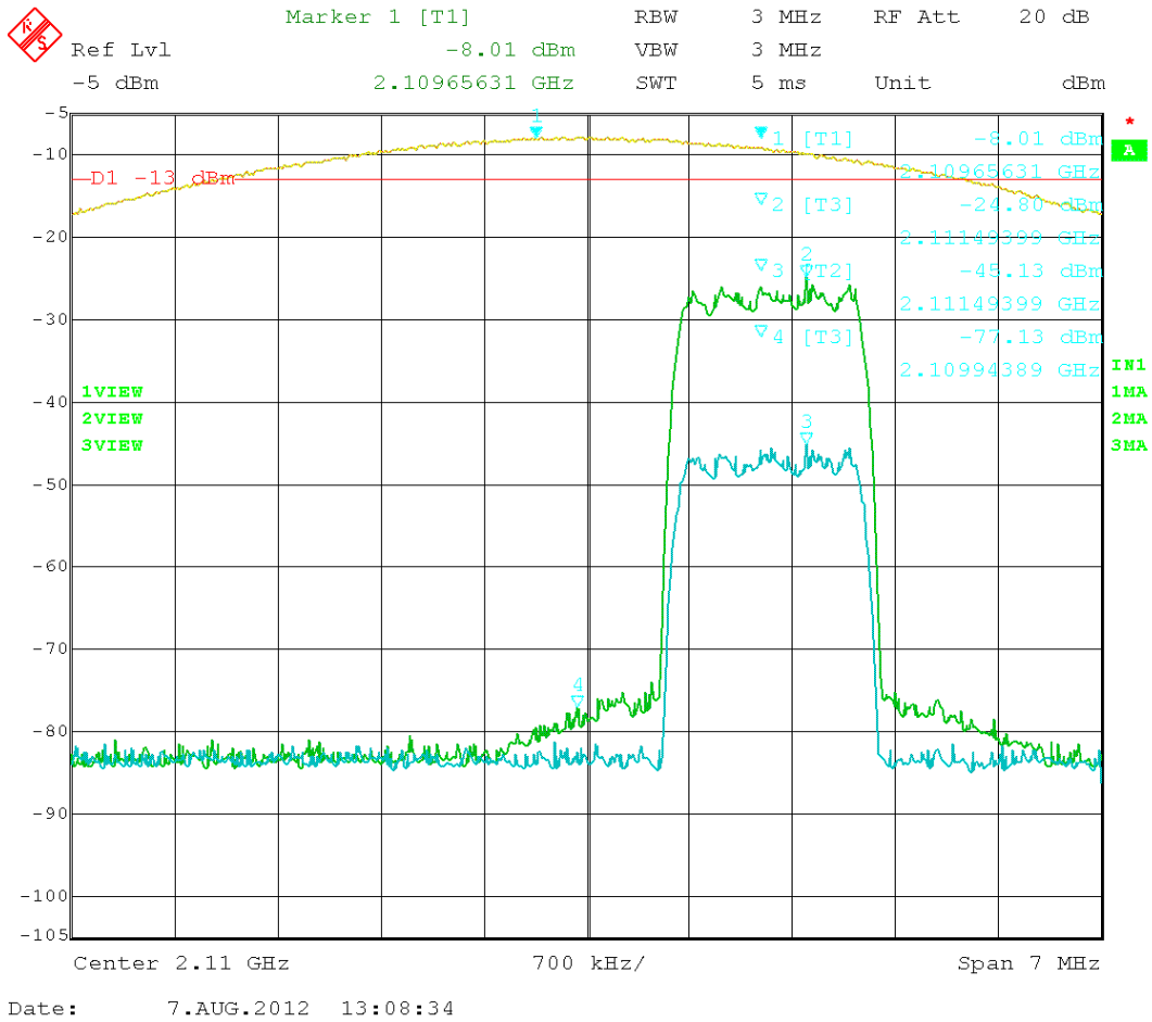
Figure 27: CDMA – In vs. Out 2111.25MHz
