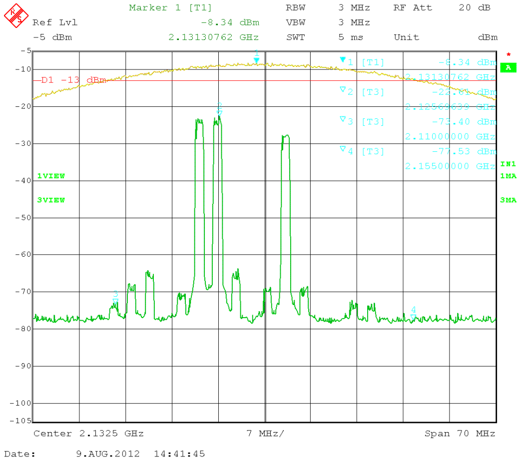
Figure 76: CDMA 3 tones intermodulation - (2110 – 2155) MHz.
