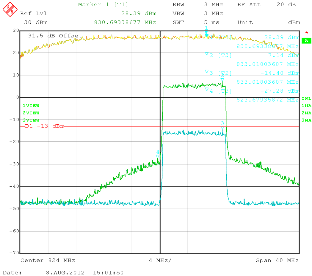
Figure 61: LTE – In vs. Out 829.00 MHz
