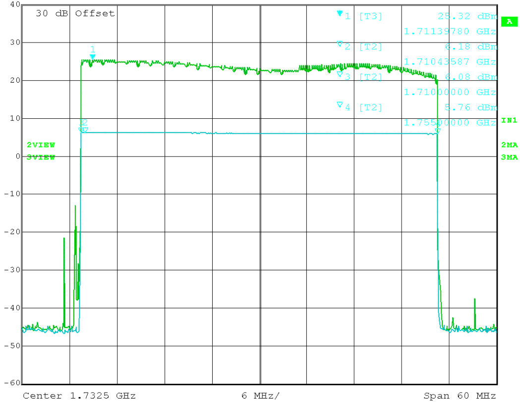
Figure 87. Frequency response (1710 – 1755) MHz band
