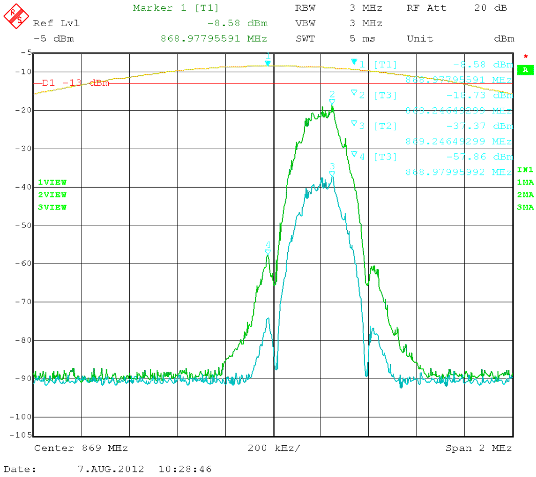
Figure 71: EDGE – In vs. Out 869.20 MHz
