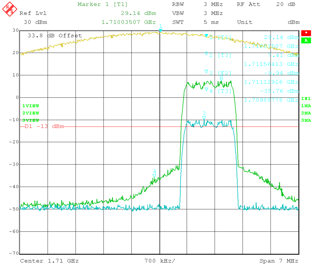
Figure 29: EVDO – In vs. Out 1711.25MHz
