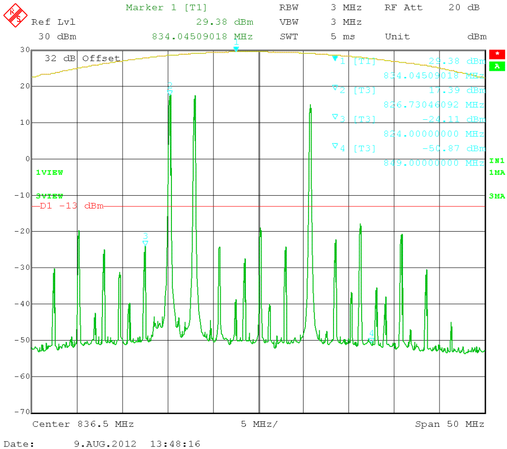
Figure 83: GSM 3 tones intermodulation - (824 – 849) MHz
