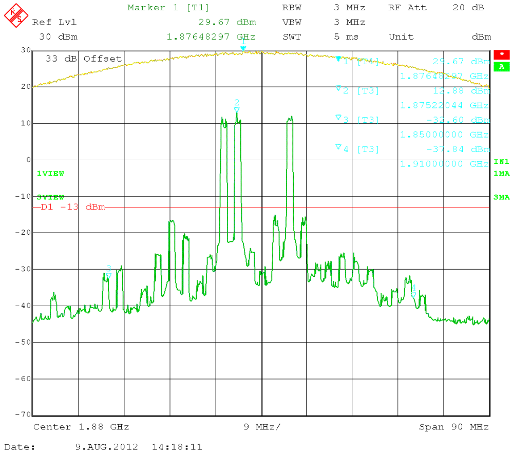
Figure 73: CDMA 3 tones intermodulation - (1850 – 1910) MHz.
