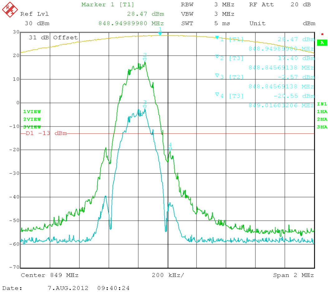
Figure 70: EDGE – In vs. Out 848.80 MHz
