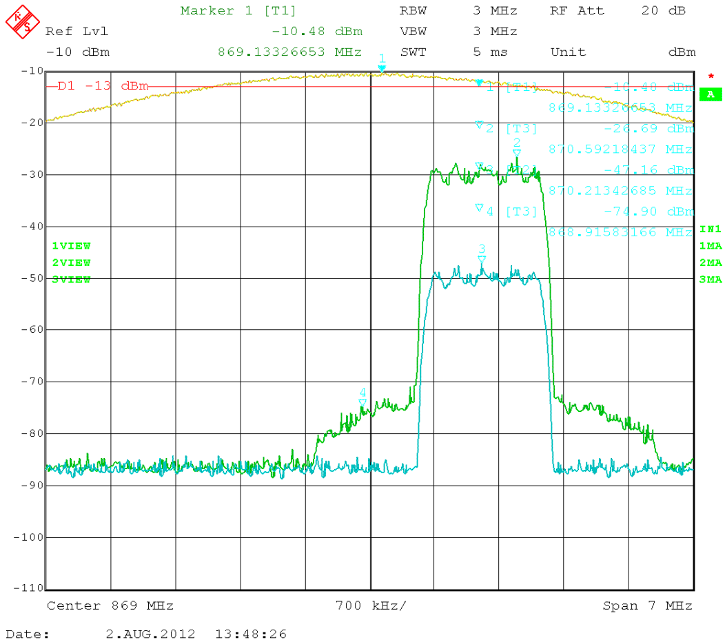
Figure 51: CDMA – In vs. Out 870.25 MHz
