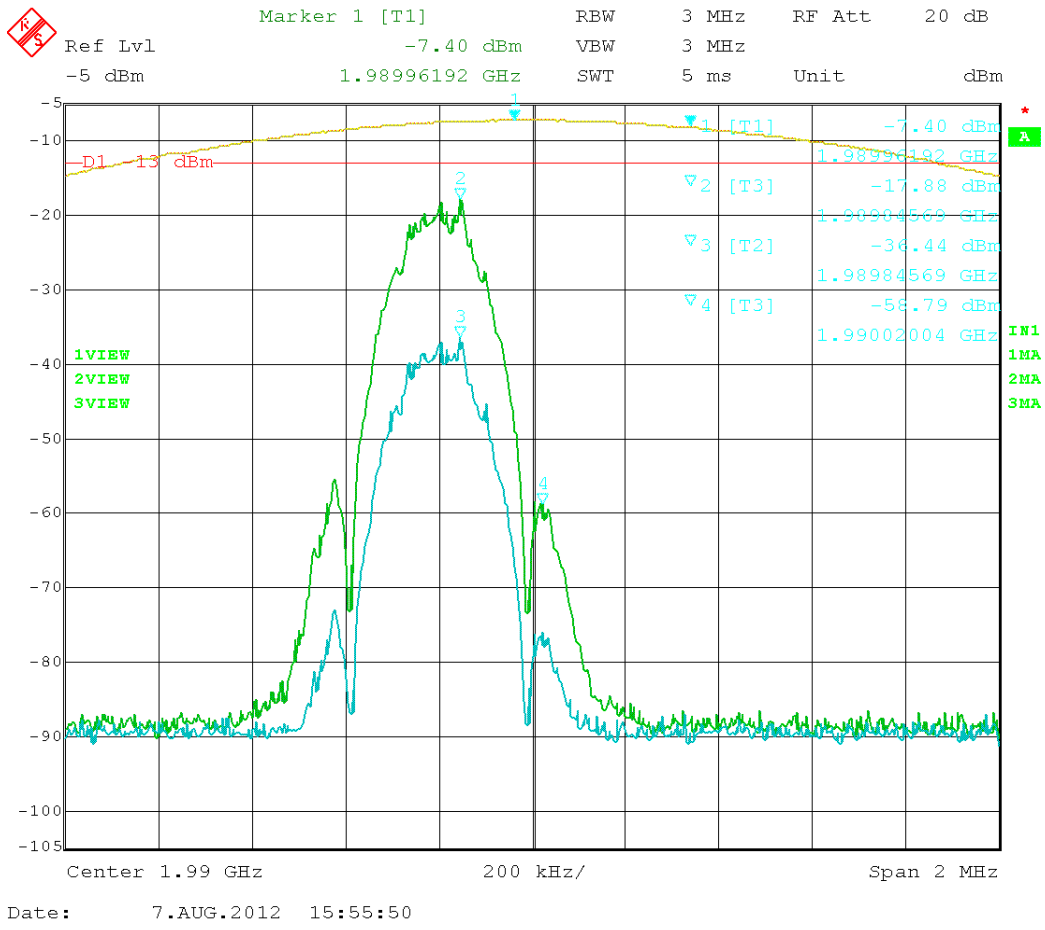
Figure 24: EDGE – In vs. Out 1989.80MHz
