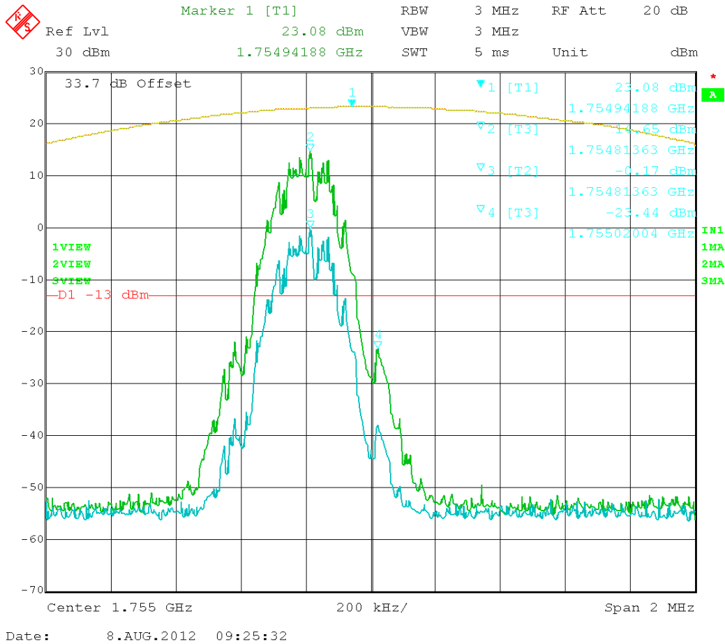
Figure 42: GSM – In vs. Out 1754.80MHz
