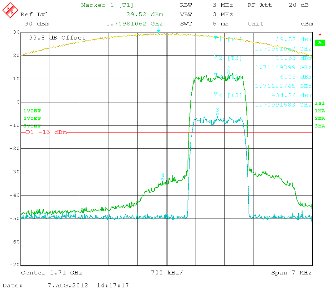
Figure 25: CDMA – In vs. Out 1711.25MHz
