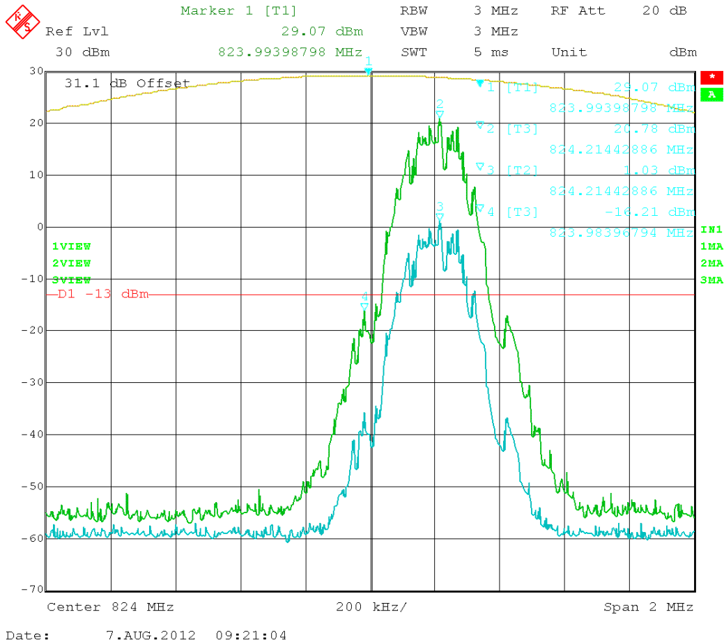
Figure 65: GSM – In vs. Out 824.2 MHz
