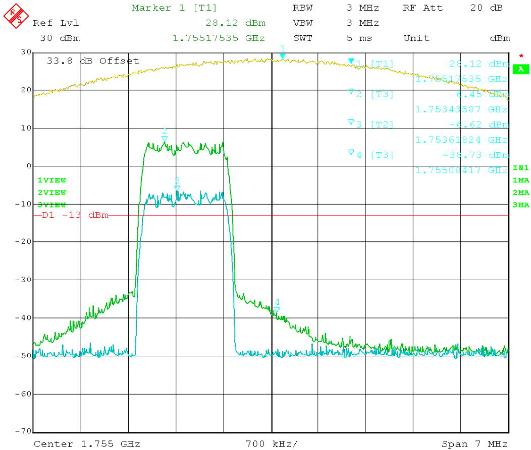
Figure 30: EVDO – In vs. Out 1753.75MHz
