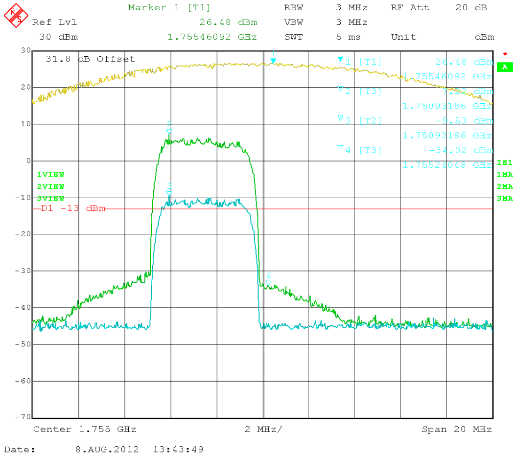
Figure 34: HSPA – In vs. Out 1752.50 MHz
