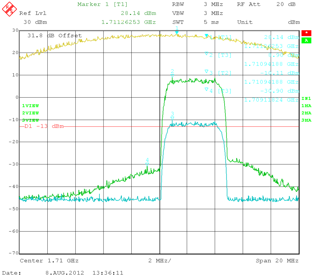
Figure 33: HSPA – In vs. Out 1712.50 MHz
