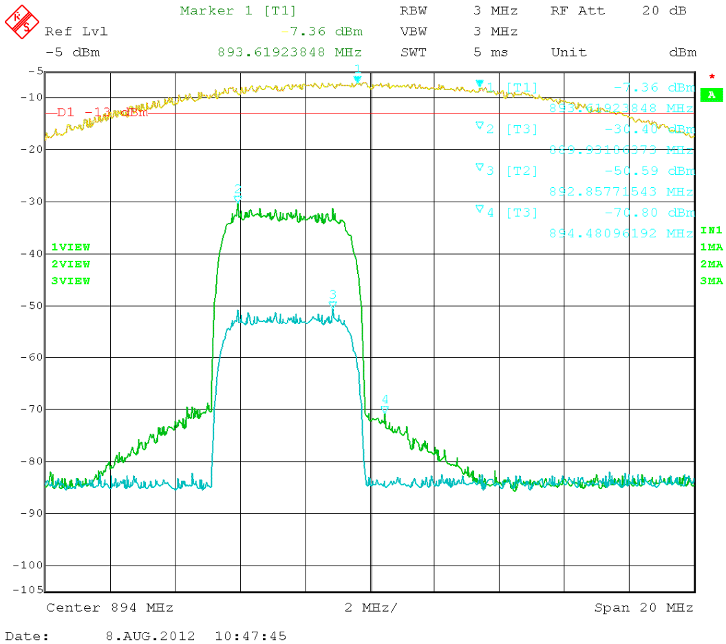
Figure 60: HSPA – In vs. Out 891.50 MHz
