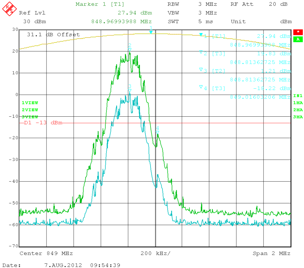
Figure 66: GSM – In vs. Out 848.8 MHz
