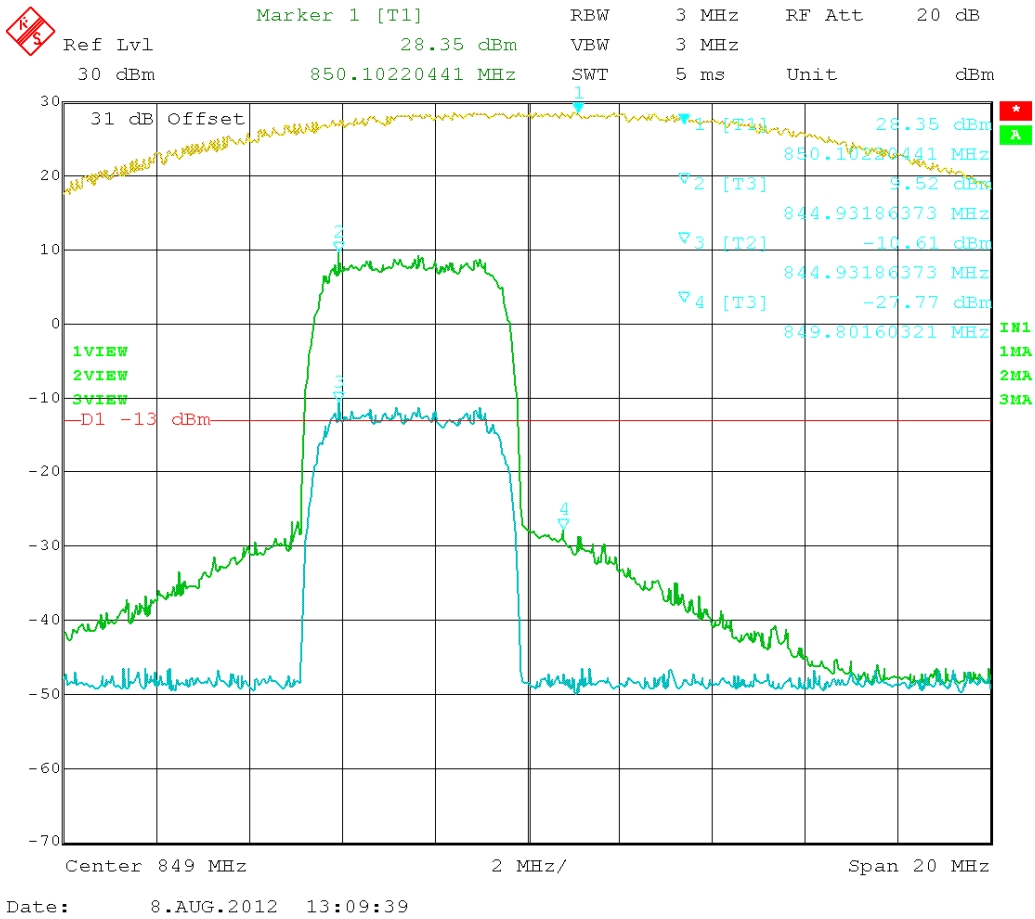
Figure 58: HSPA – In vs. Out 846.50 MHz
