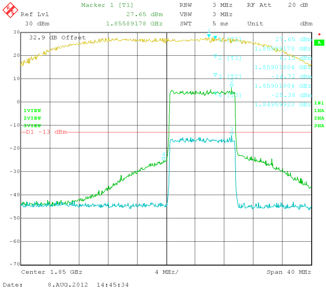
Figure 13: LTE – In vs. Out 1855.00MHz
