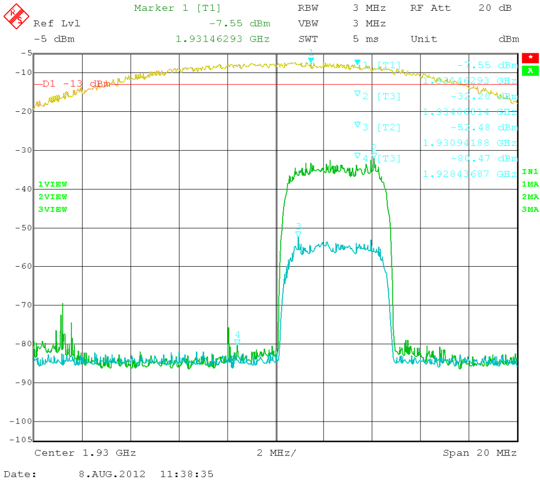
Figure 11: HSPA – In vs. Out 1932.50 MHz
