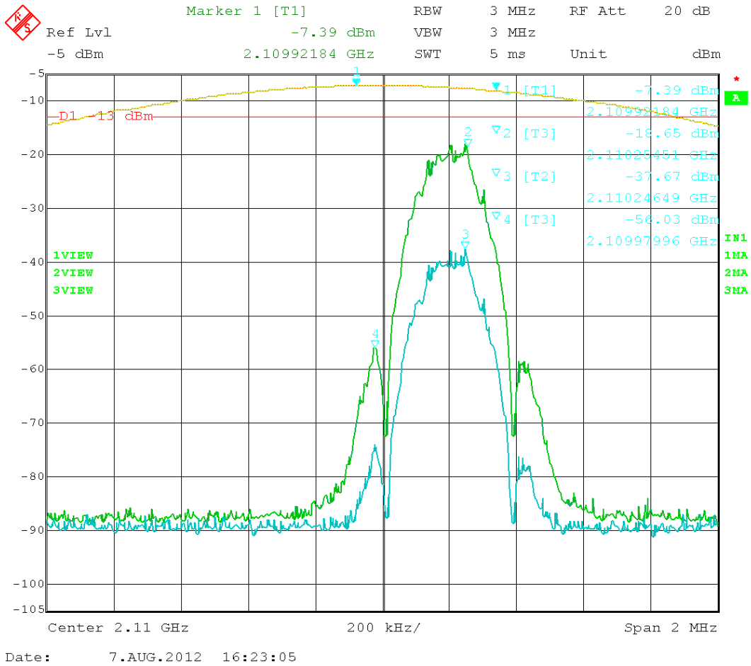
Figure 47: EDGE – In vs. Out 2110.20MHz
