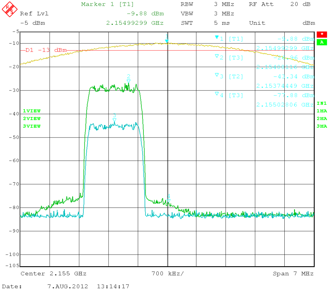
Figure 28: CDMA – In vs. Out 2153.75MHz
