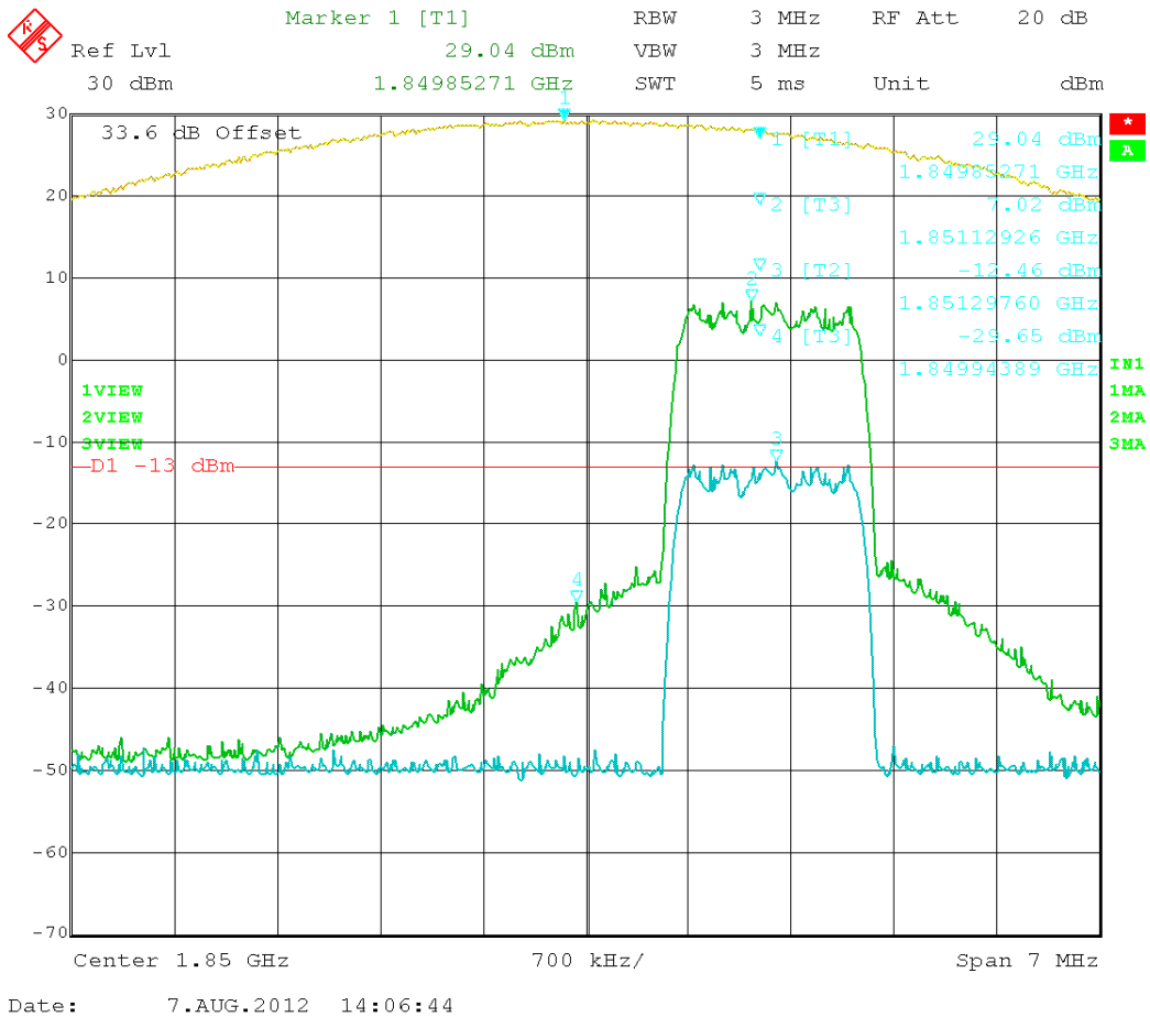
Figure 5: EVDO – In vs. Out 1851.25MHz
