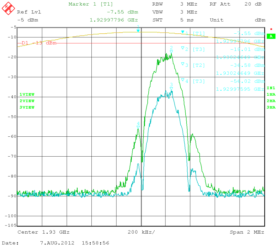
Figure 23: EDGE – In vs. Out 1930.20MHz
