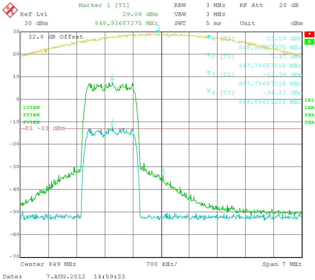
Figure 54: EVDO – In vs. Out 847.75 MHz
