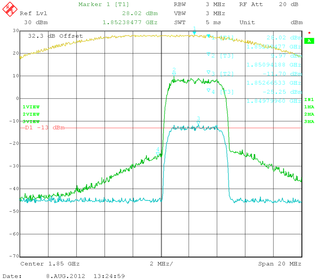
Figure 9: HSPA – In vs. Out 1852.50 MHz
