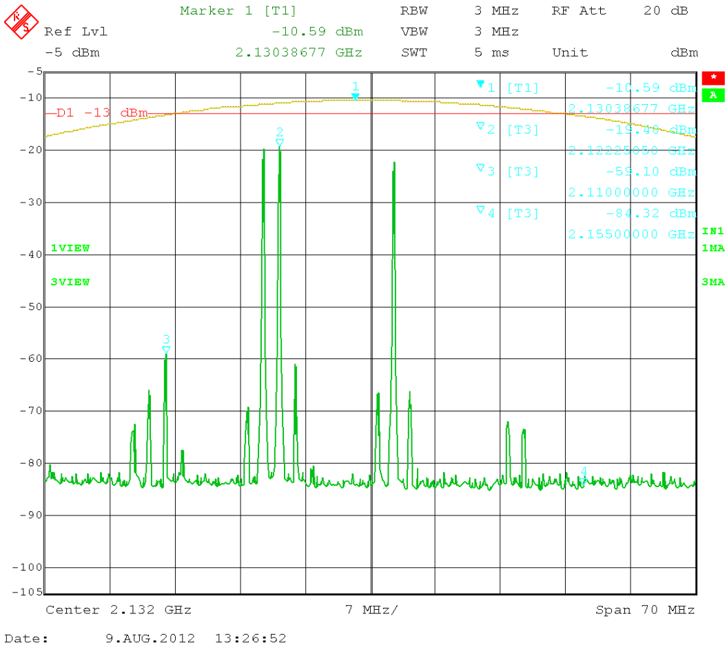
Figure 82: GSM 3 tones intermodulation - (2110 – 2155) MHz
