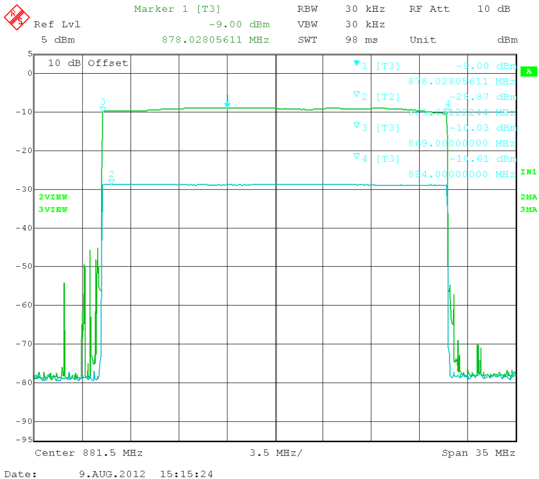
Figure 90. Frequency response (869 – 894) MHz band
