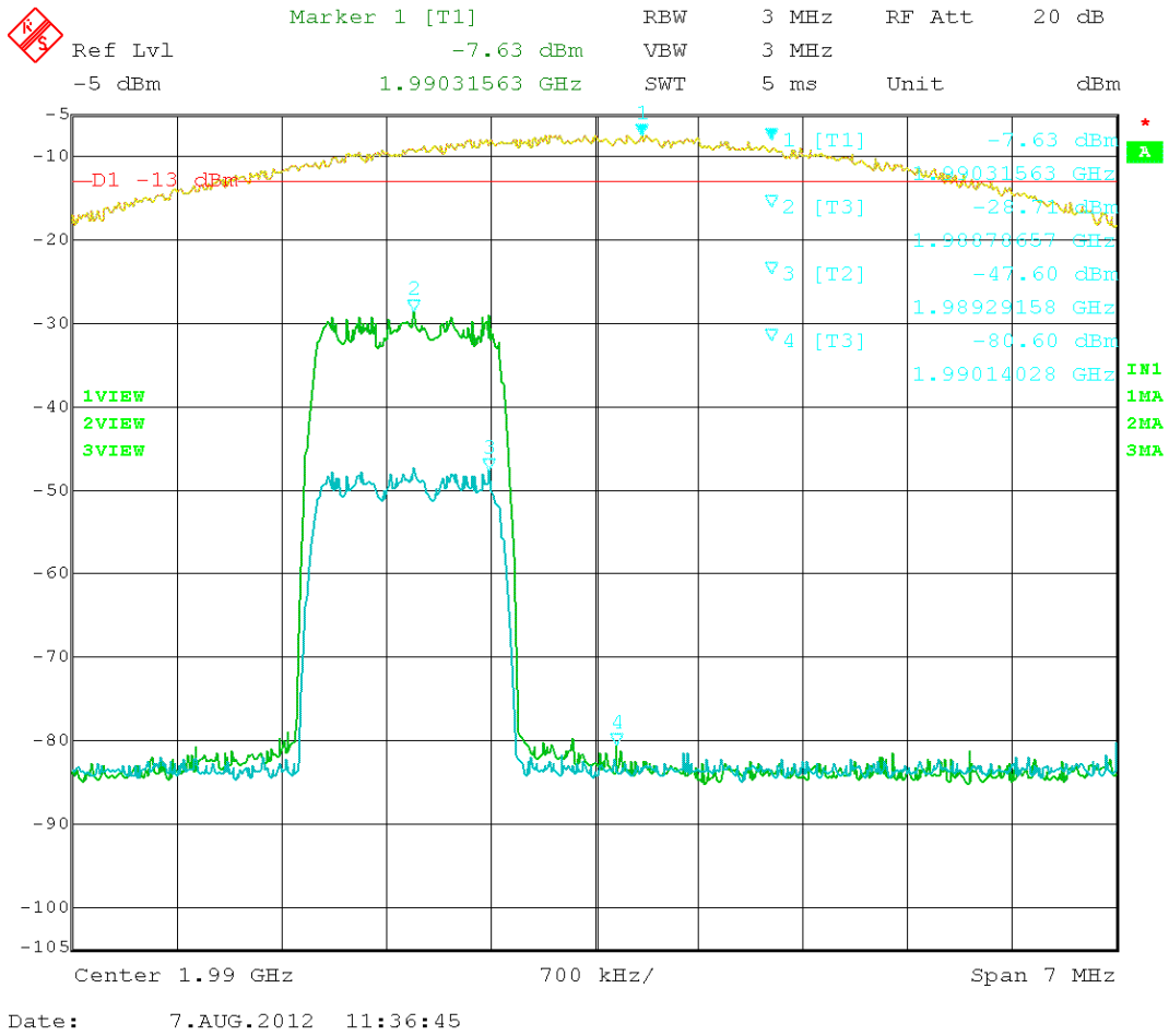
Figure 8: EVDO – In vs. Out 1988.75MHz
