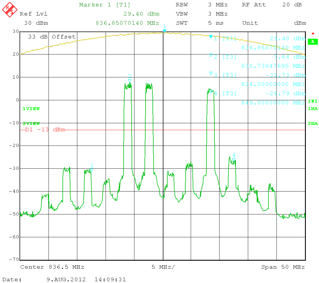
Figure 77: CDMA 3 tones intermodulation – (824 – 849) MHz.
