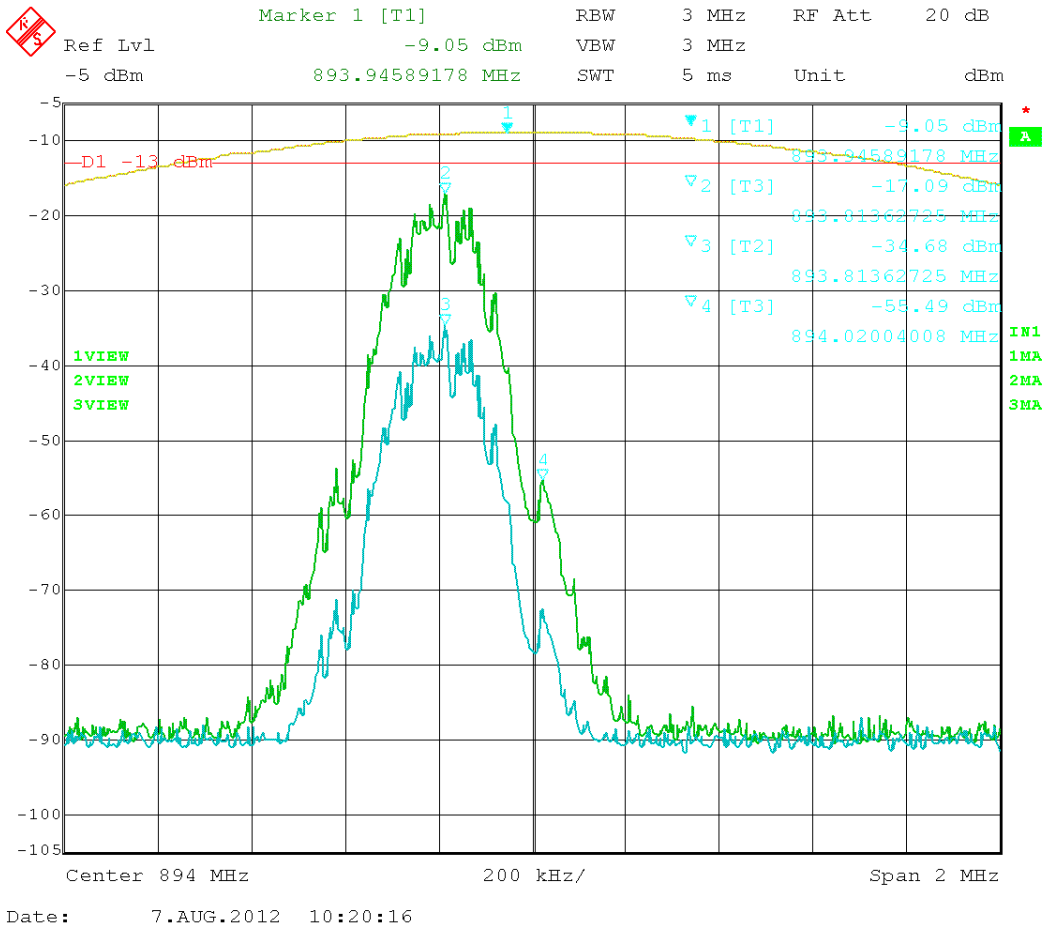
Figure 68: GSM – In vs. Out 893.8MHz
