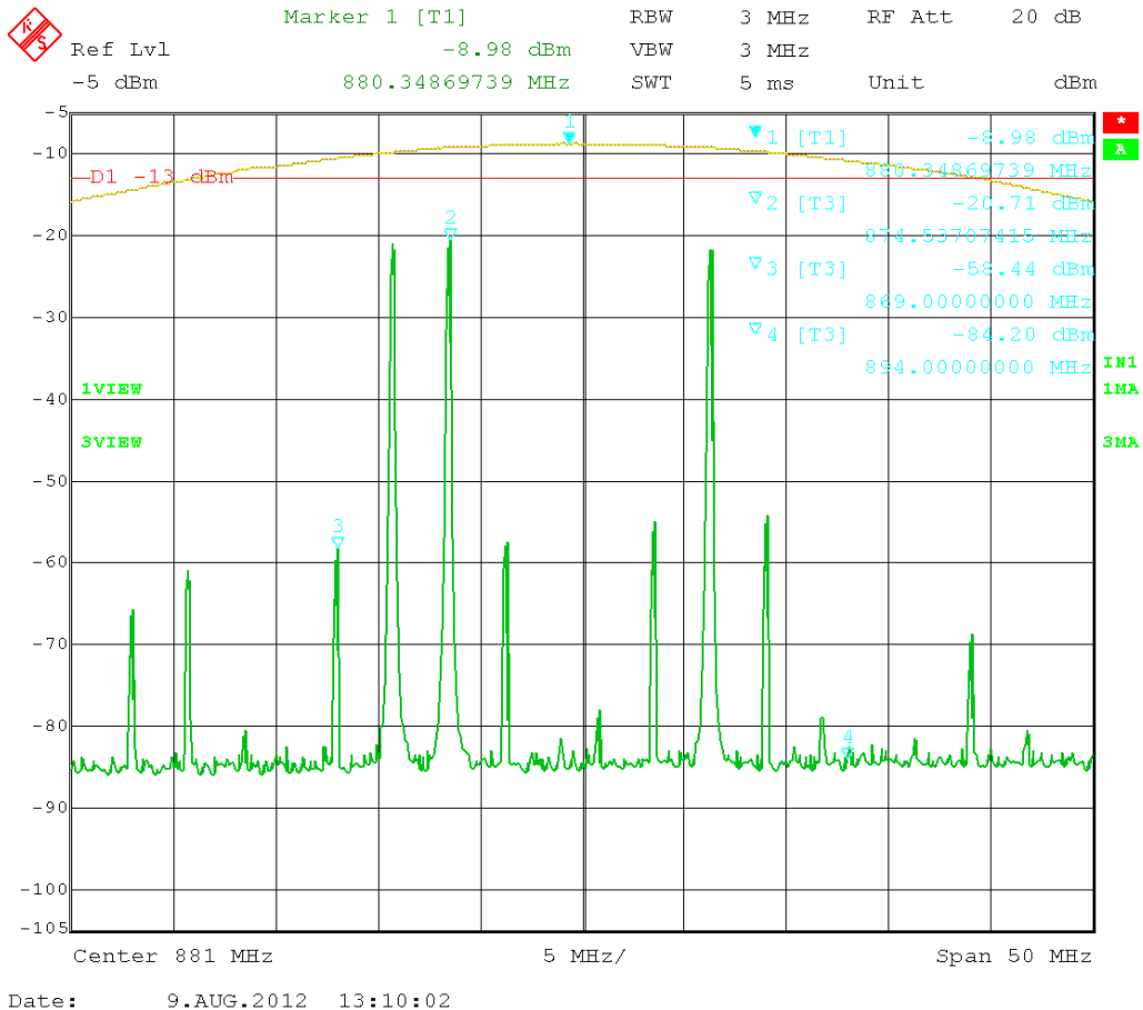
Figure 84: GSM 3 tones intermodulation - (869 – 894) MHz
