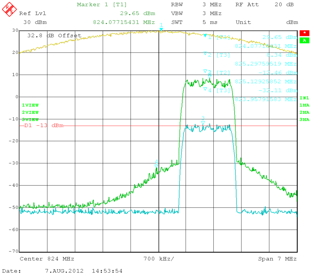
Figure 53: EVDO – In vs. Out 825.25 MHz
