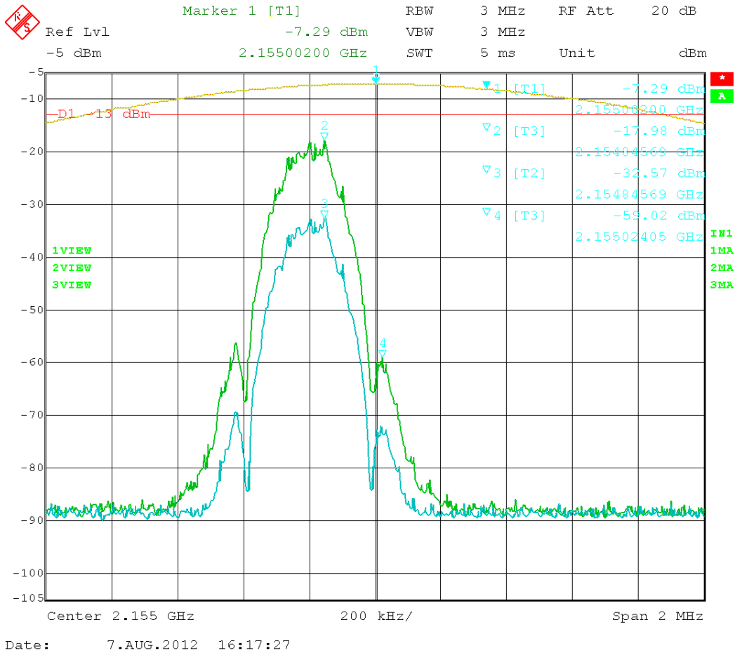
Figure 48: EDGE – In vs. Out 2154.80MHz
