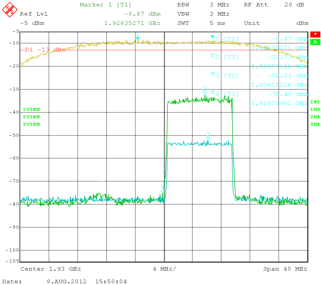
Figure 15: LTE – In vs. Out 1935.00MHz
