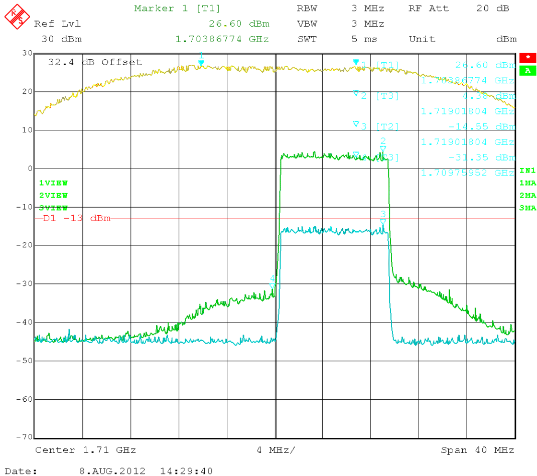
Figure 37: LTE – In vs. Out 1715.00MHz
