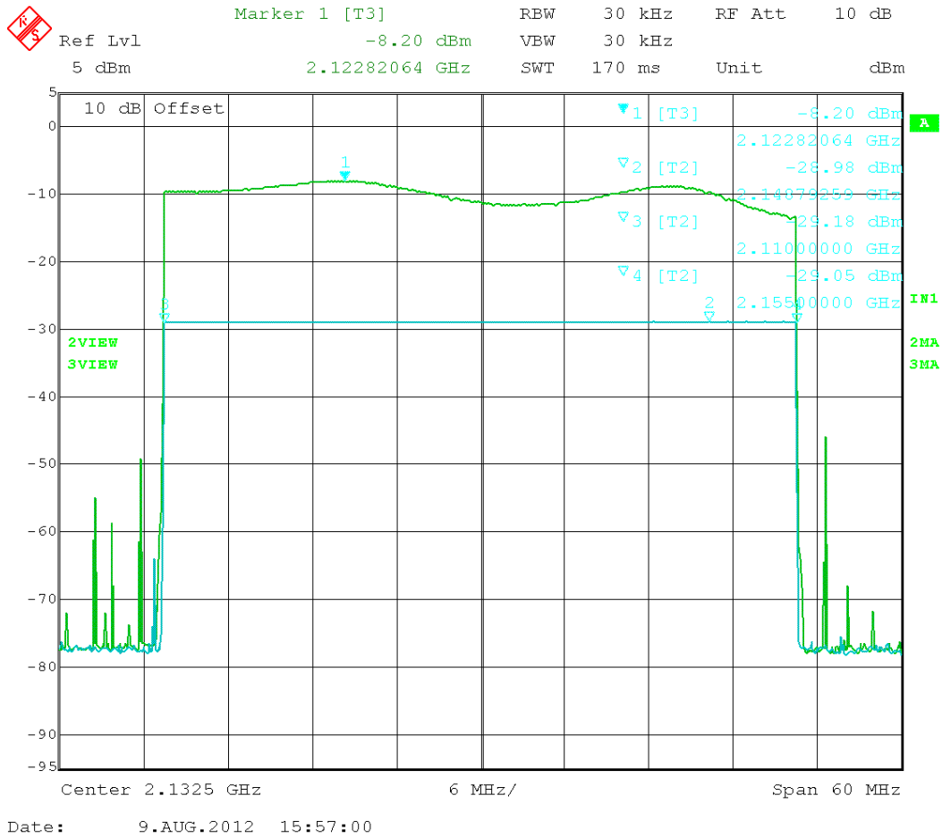
Figure 88. Frequency response (2110 – 2155) MHz band
