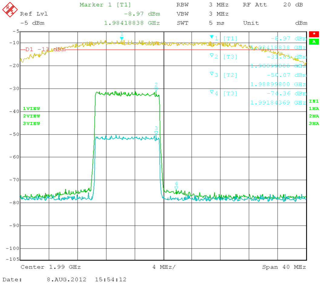
Figure 16: LTE – In vs. Out 1985.00MHz
