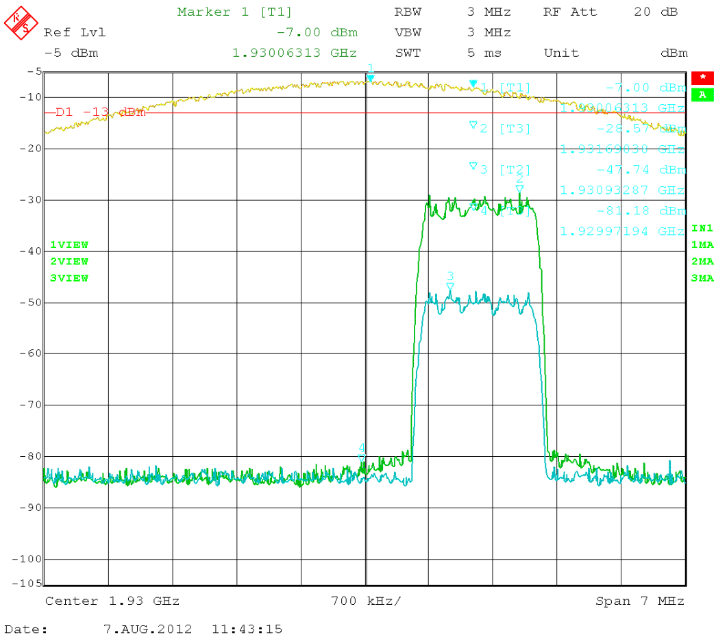
Figure 7: EVDO – In vs. Out 1931.25MHz
