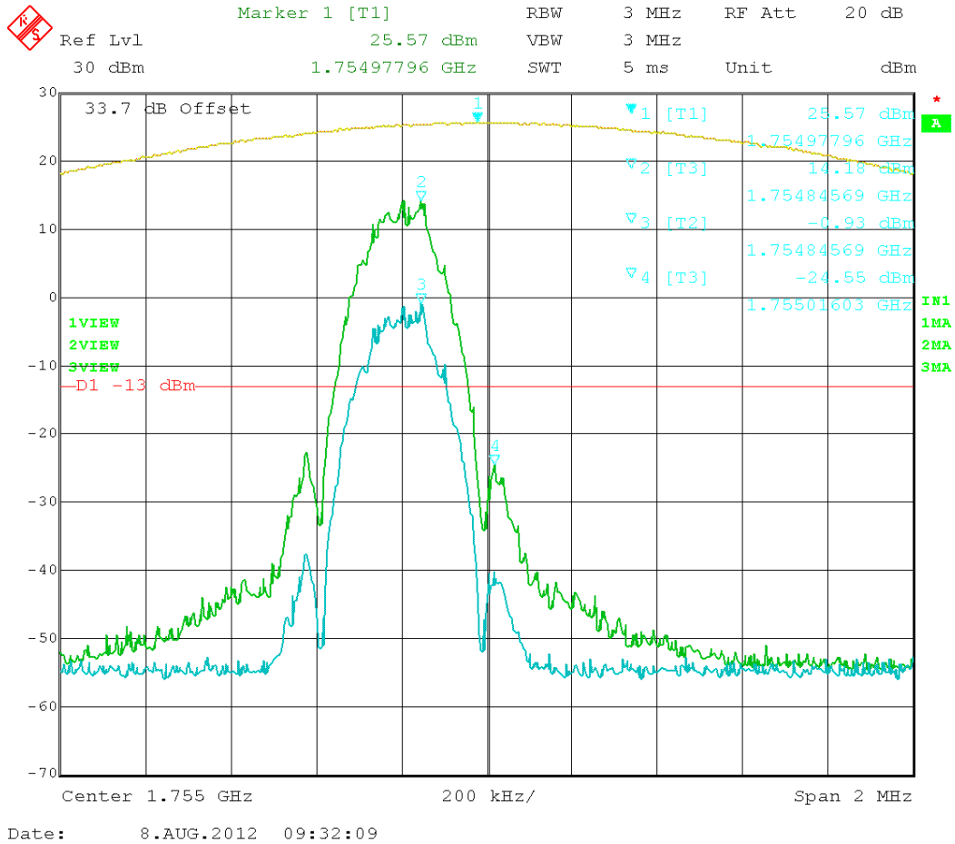
Figure 46: EDGE – In vs. Out 1.755 GHz
