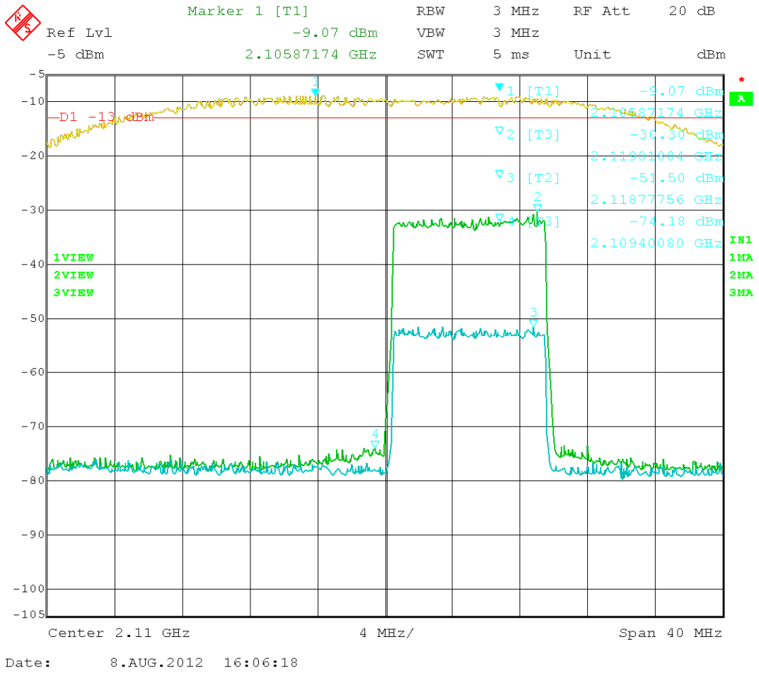
Figure 39: LTE – In vs. Out 2115.00MHz
