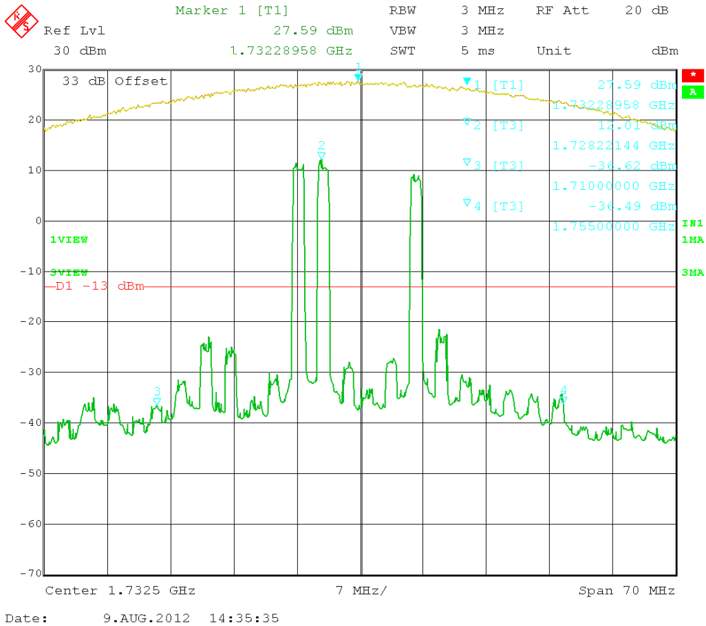
Figure 75: CDMA 3 tones intermodulation - (1710 – 1755) MHz.
