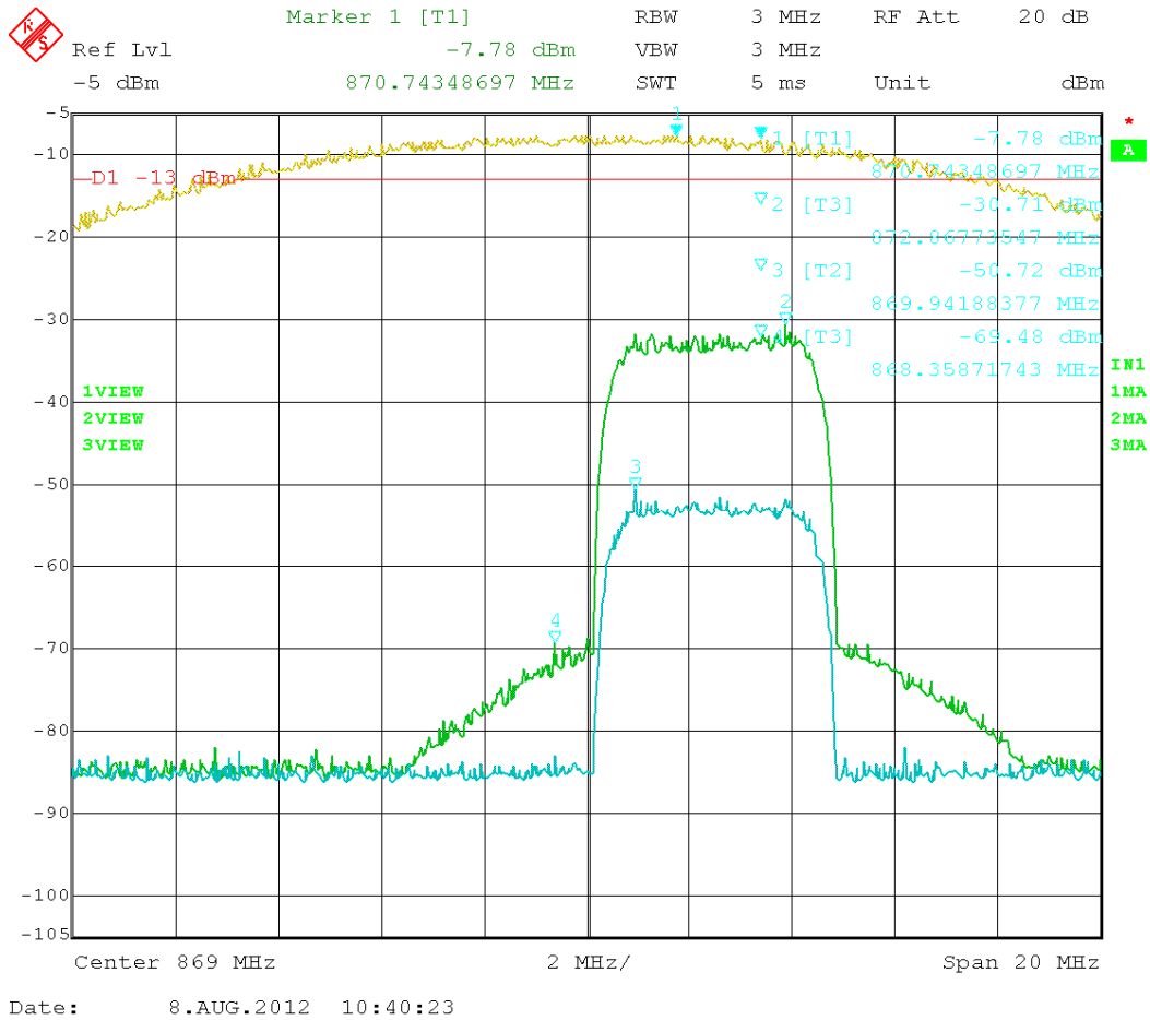
Figure 59: HSPA – In vs. Out 871.50 MHz
