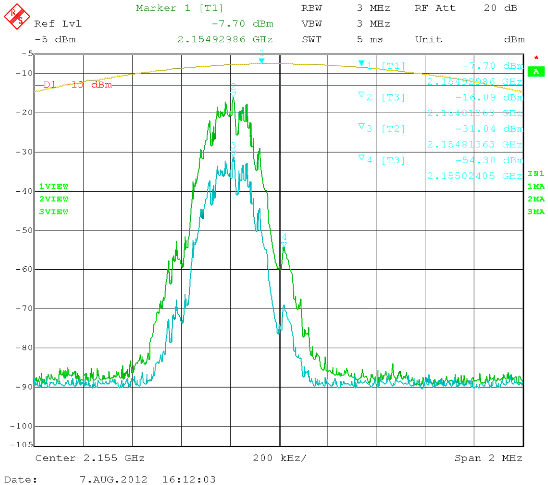
Figure 44: GSM – In vs. Out 2154.80MHz
