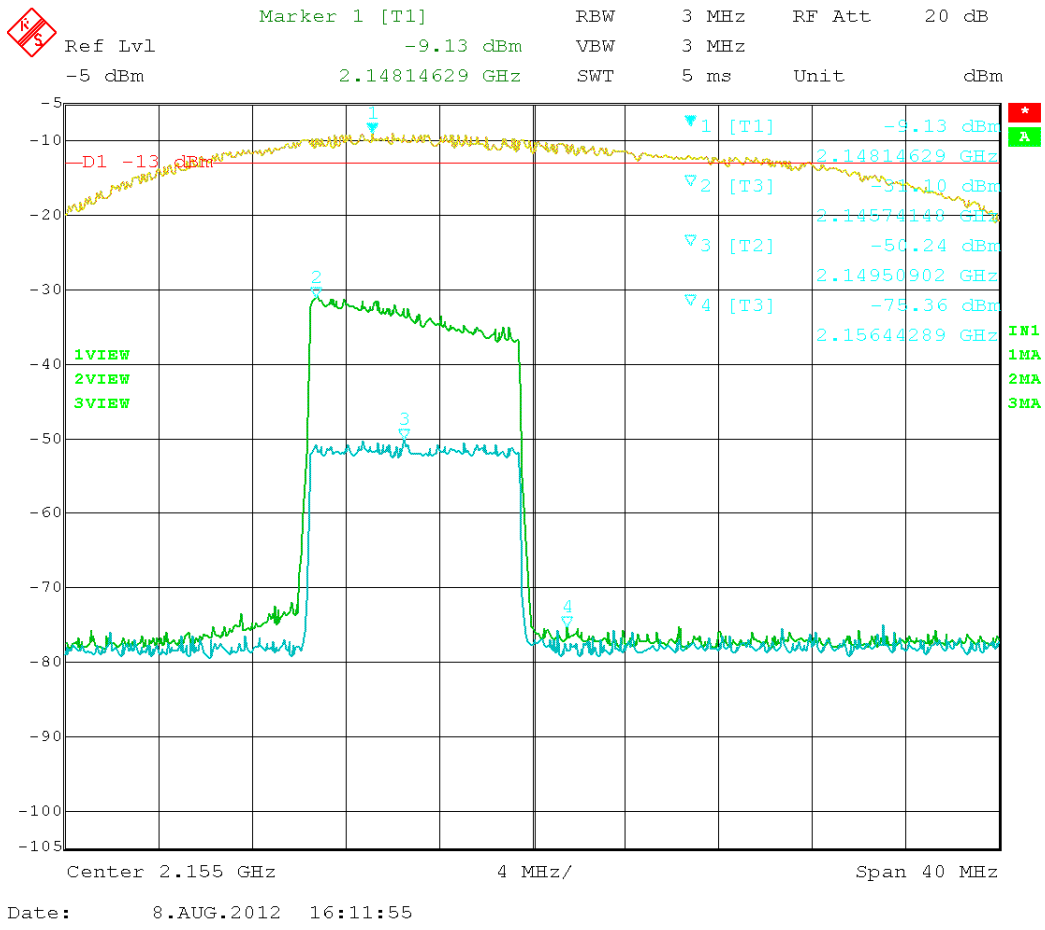
Figure 40: LTE – In vs. Out 2150.00MHz
