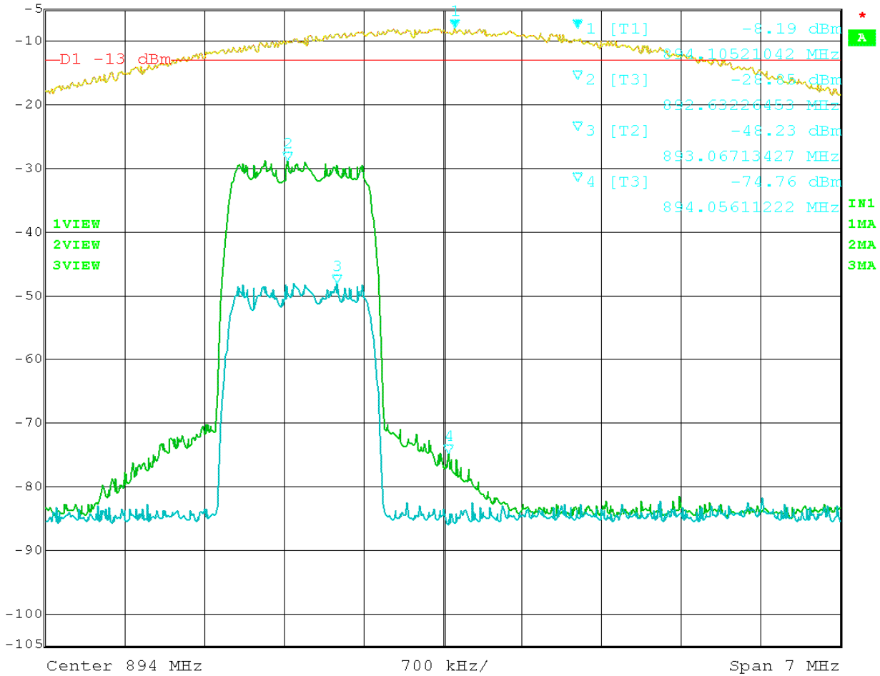
Figure 56: EVDO – In vs. Out 892.75 MHz
