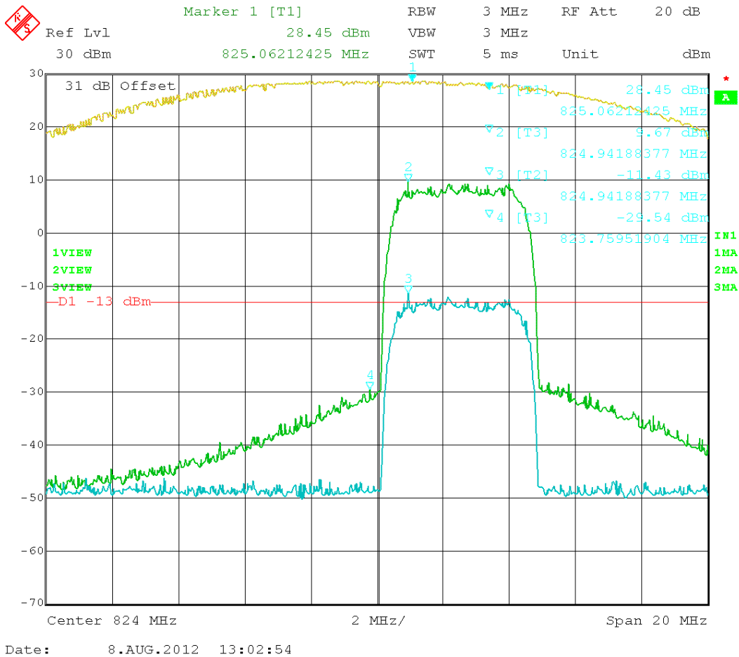
Figure 57: HSPA – In vs. Out 826.50 MHz
