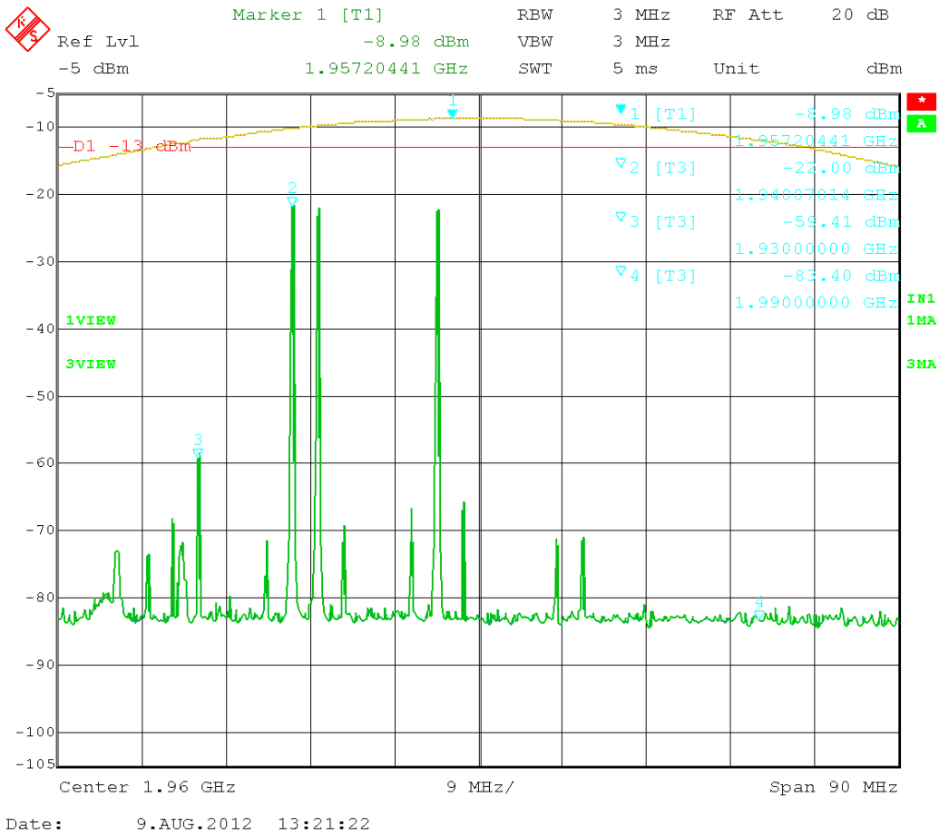
Figure 80: GSM 3 tones intermodulation - (1930 – 1990) MHz
