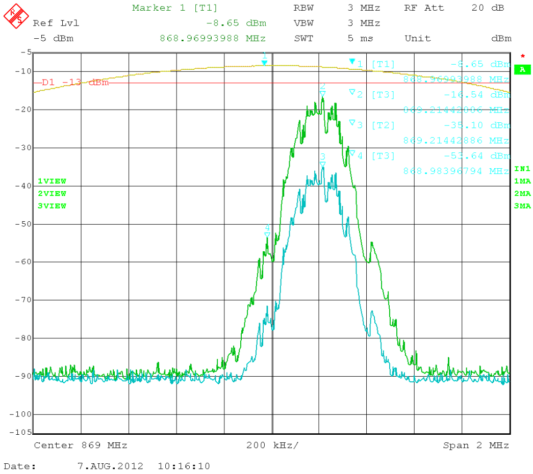
Figure 67: GSM – In vs. Out 869.2MHz
