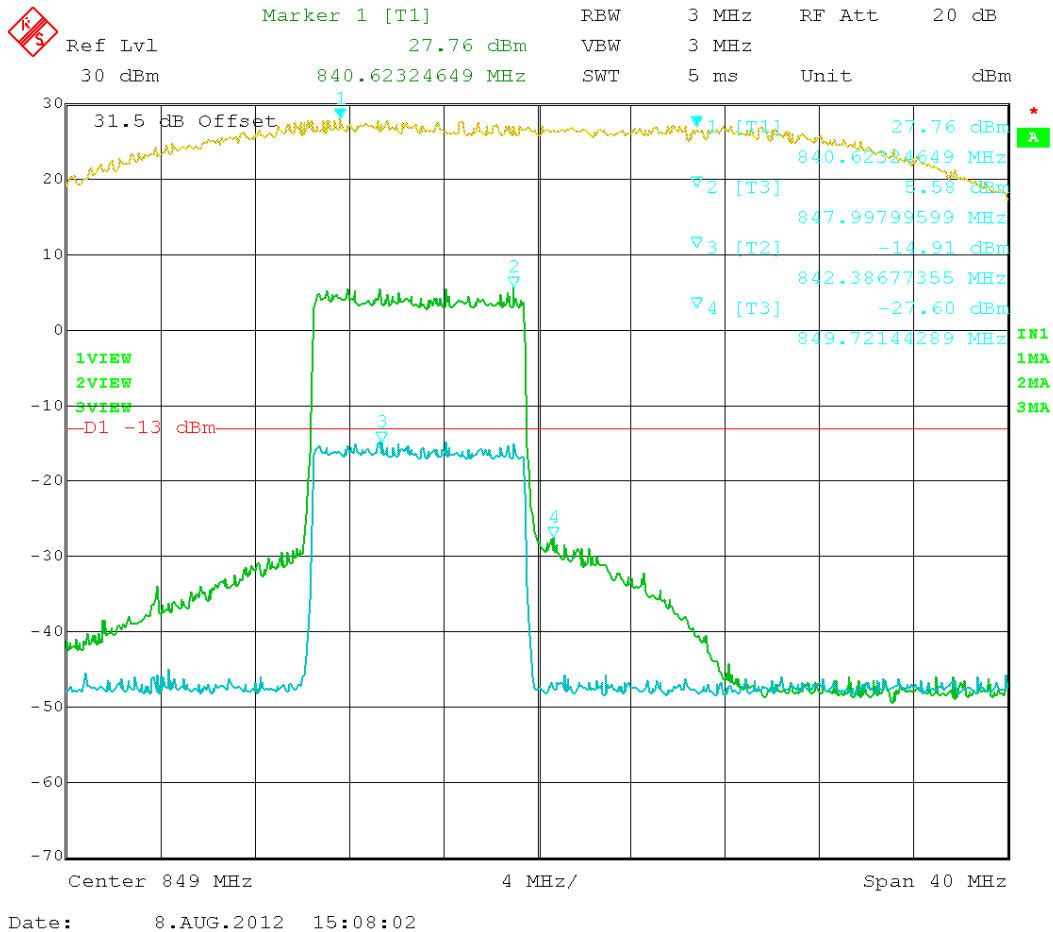
Figure 62: LTE – In vs. Out 844.00 MHz
