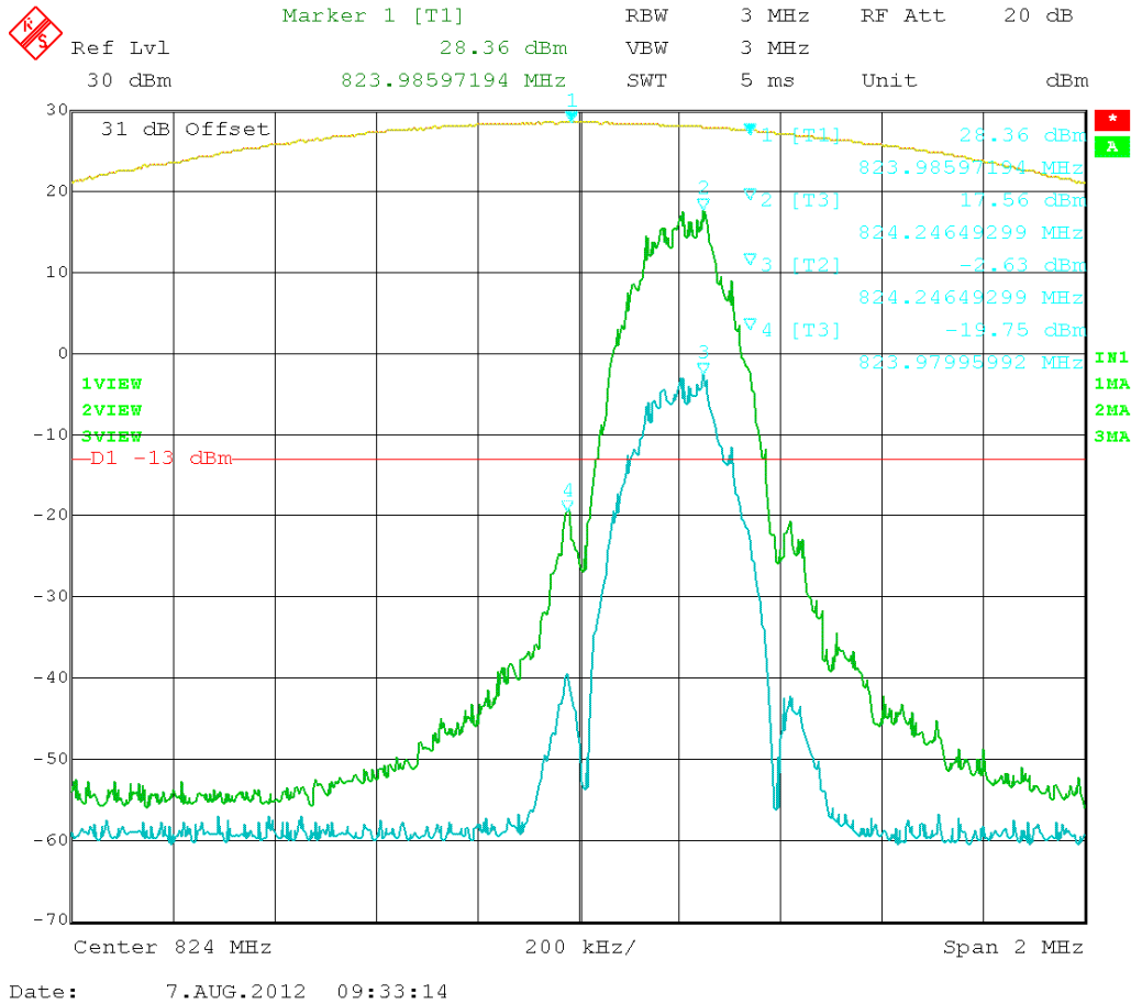
Figure 69: EDGE – In vs. Out 824.20 MHz
