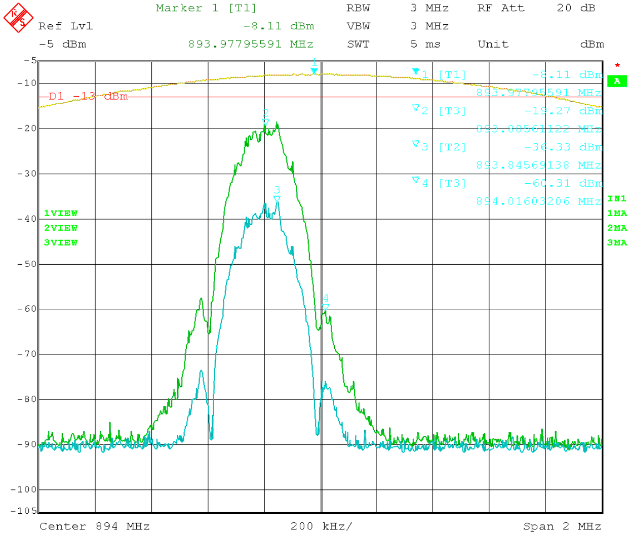
Figure 72: EDGE – In vs. Out 893.80 MHz
