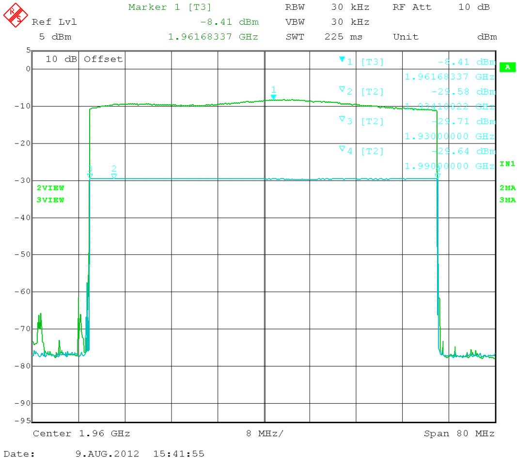
Figure 86. Frequency response (1930 – 1990) MHz band
