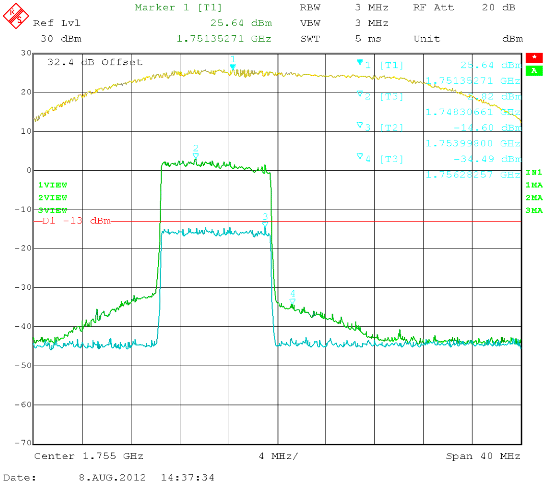
Figure 38: LTE – In vs. Out 1750.00MHz
