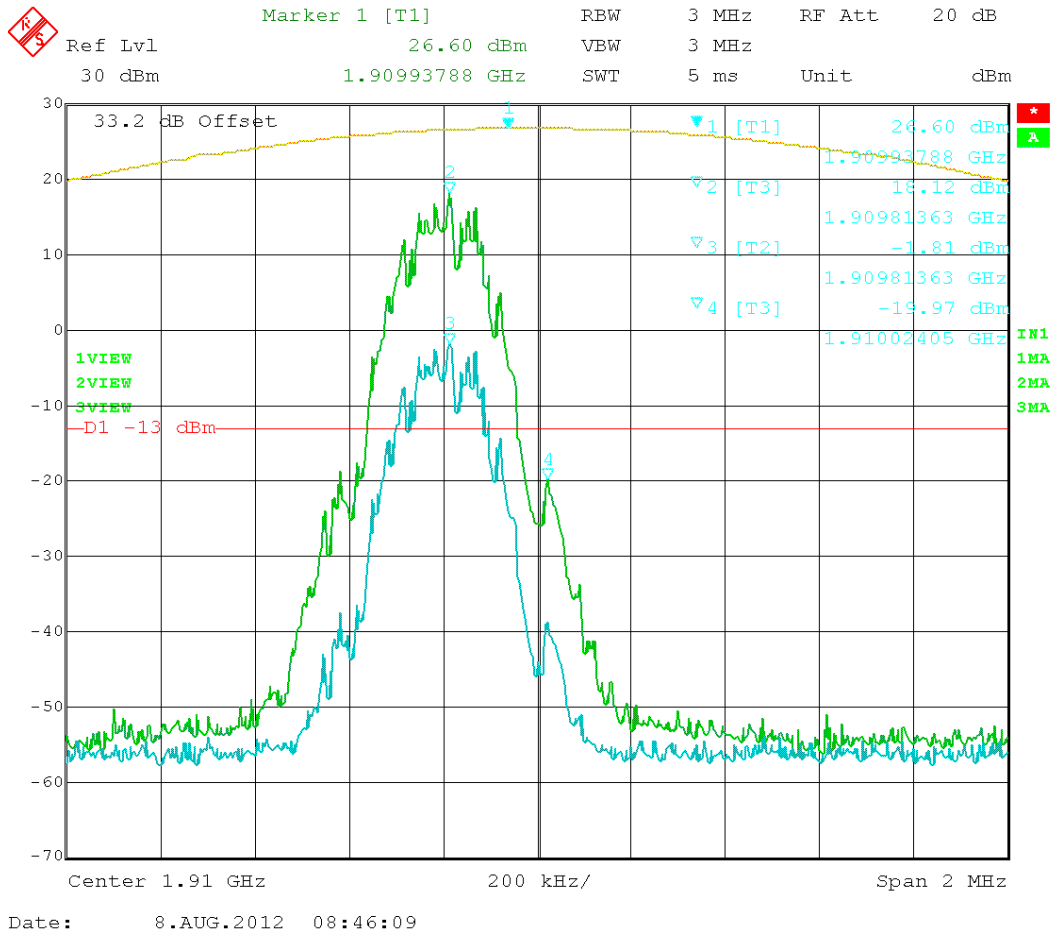
Figure 22: EDGE – In vs. Out 1909.80MHz
