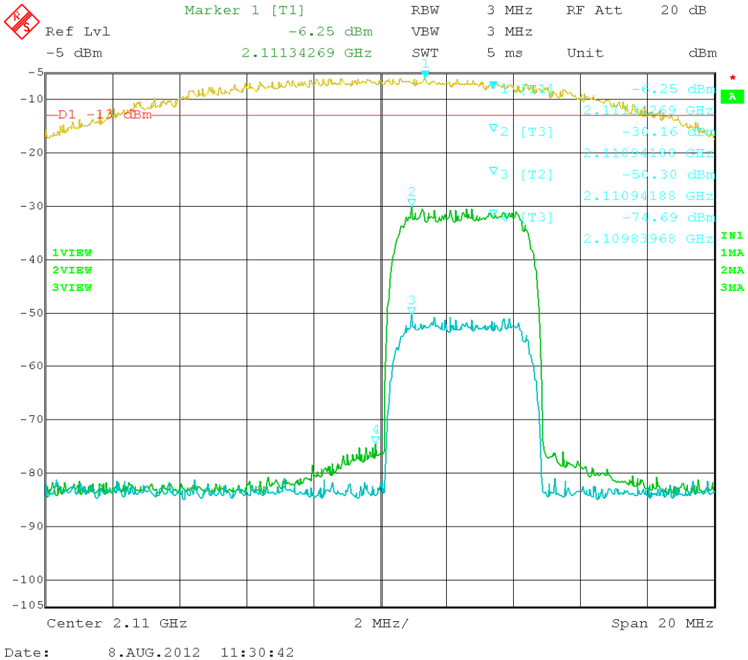
Figure 35: HSPA – In vs. Out 2112.50 MHz
