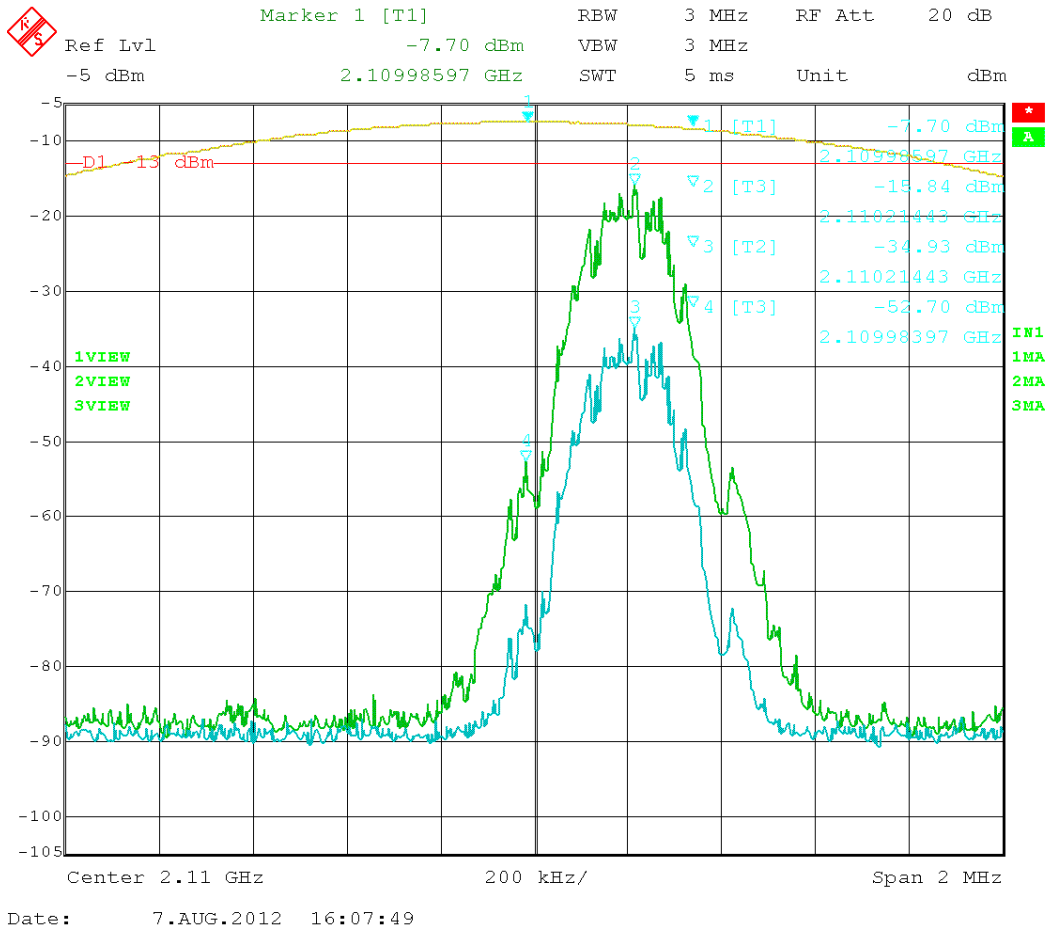
Figure 43: GSM – In vs. Out 2110.20MHz
