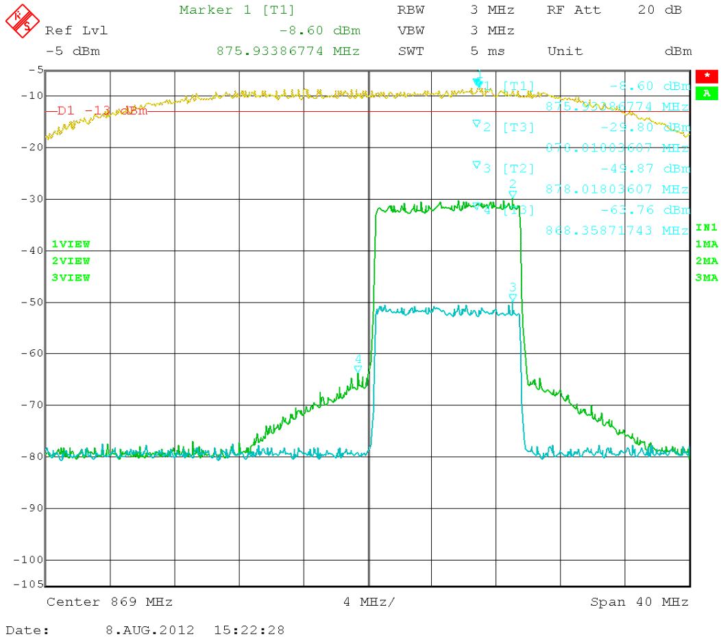
Figure 63: LTE – In vs. Out 874.00 MHz
