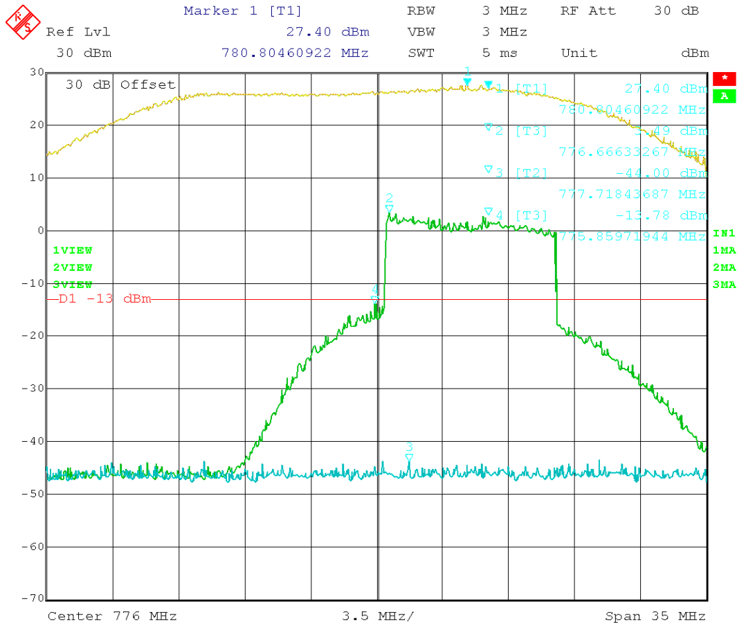
Figure 36: LTE – In vs. Out 781.0 MHz
