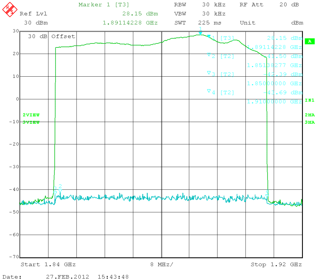
Figure 42. Frequency response (1850 – 1910) MHz band
