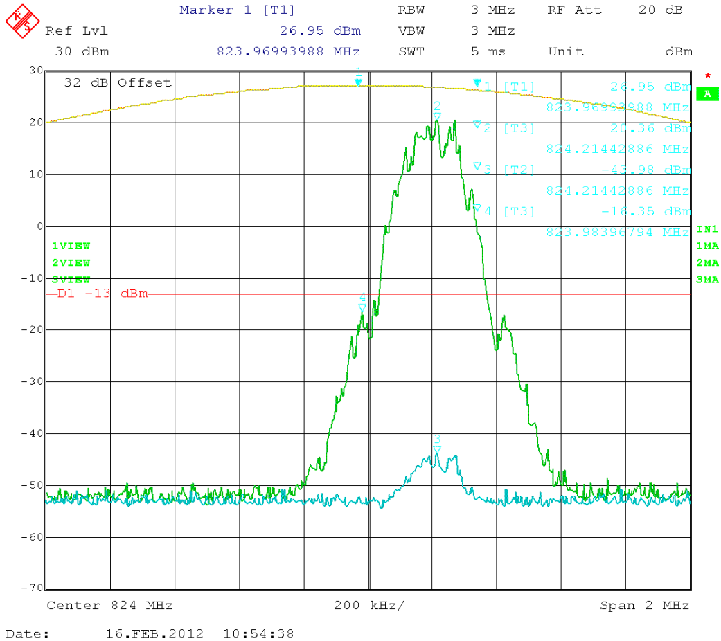
Figure 29: GSM – In vs. Out 824.2 MHz
