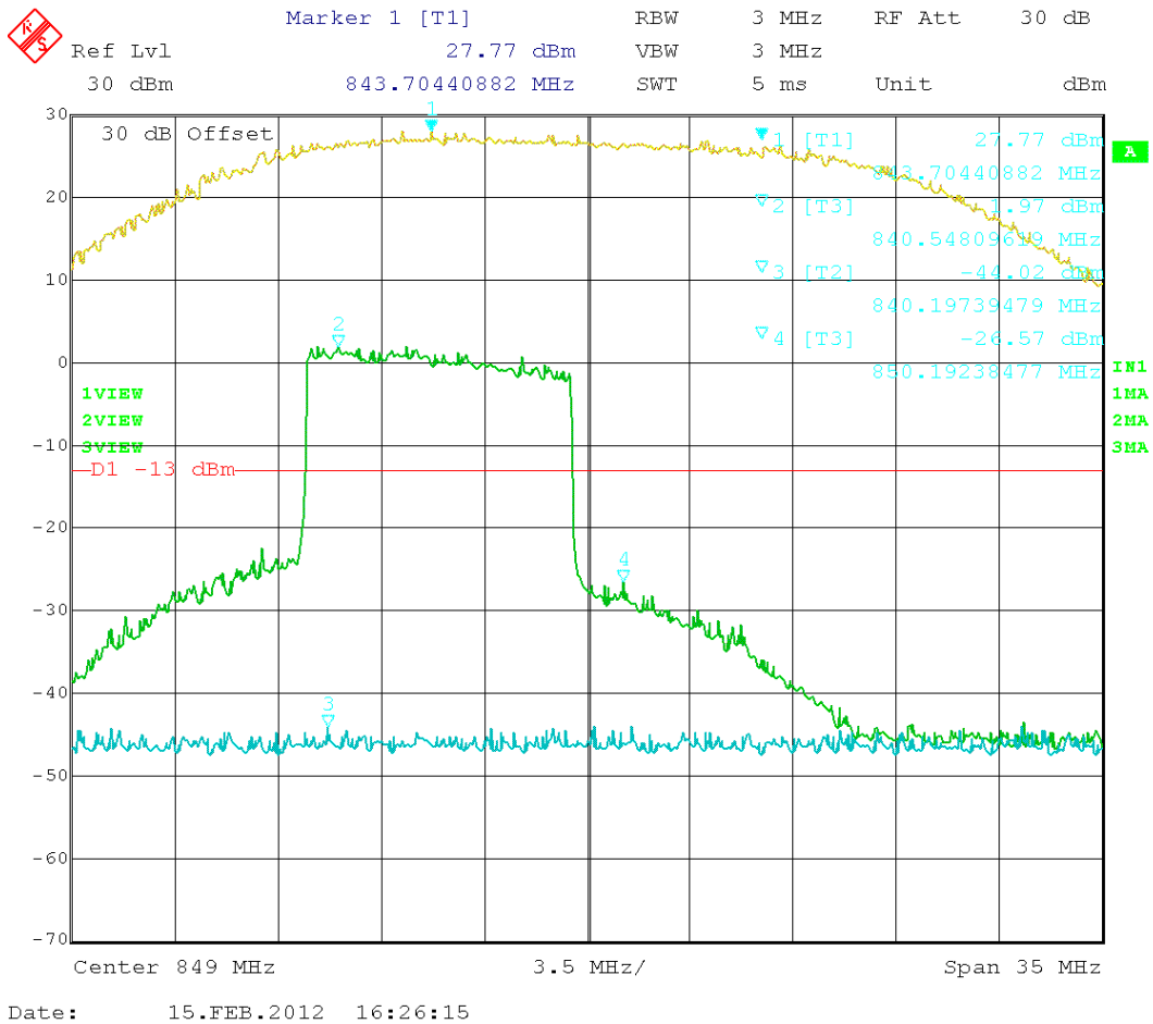
Figure 26: LTE – In vs. Out 844.00 MHz
