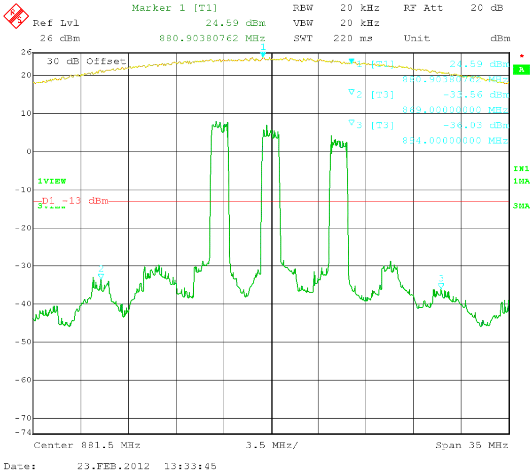
Figure 37: CDMA 3 tones intermodulation - (869 – 894) MHz.
