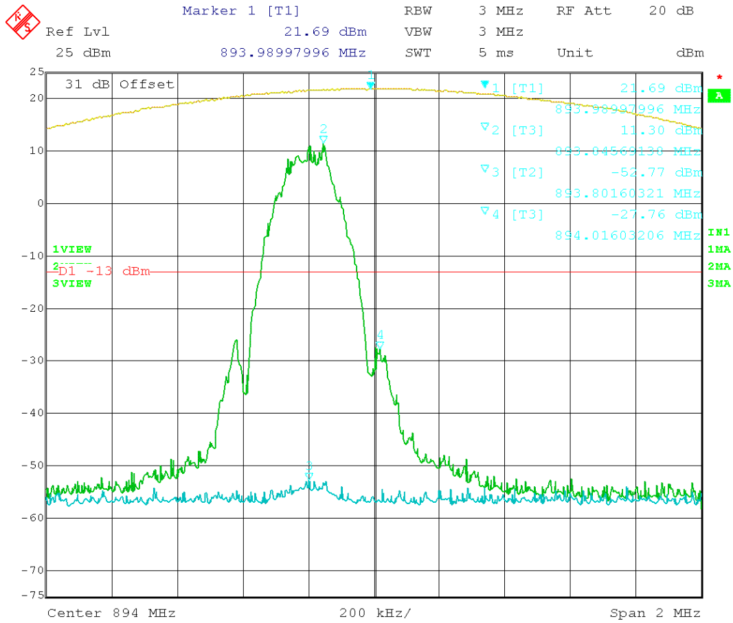
Figure 28: EDGE - In vs. Out 893.80 MHz
