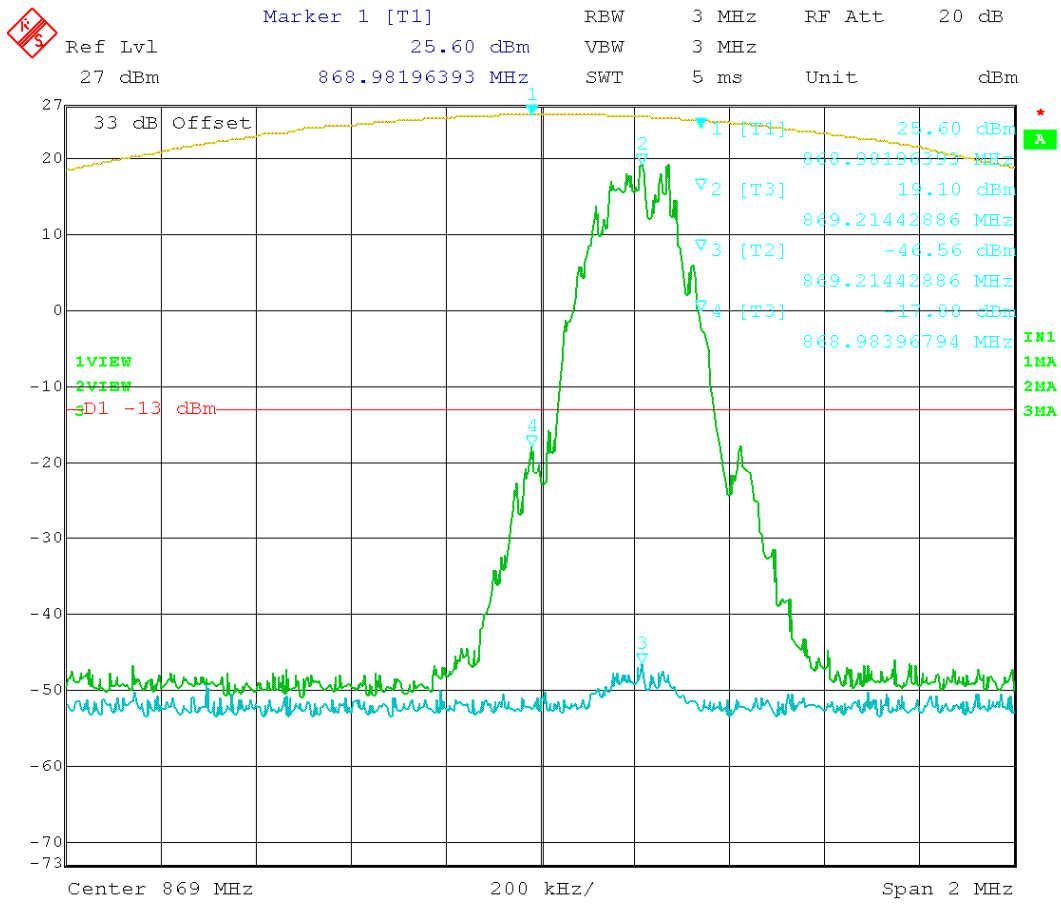
Figure 31: GSM – In vs. Out 869.2MHz
