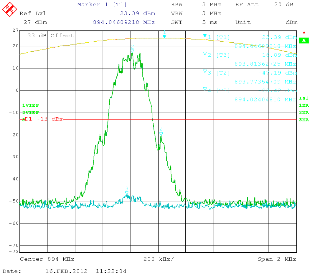
Figure 32: GSM – In vs. Out 893.8MHz
