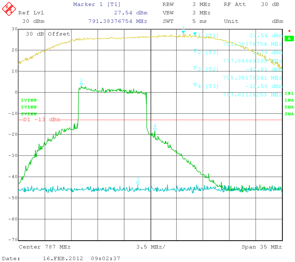
Figure 36: LTE – In vs. Out 782.0 MHz
