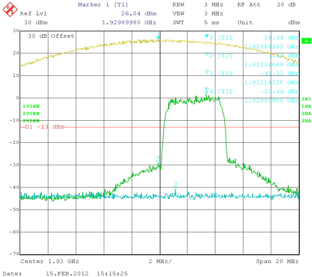
Figure 7: WCDMA – In vs. Out 1932.50 MHz
