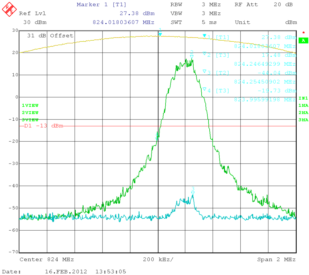
Figure 25: EDGE – In vs. Out 824.20 MHz
