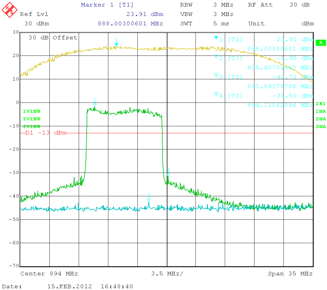
Figure 28: LTE – In vs. Out 889.00 MHz
