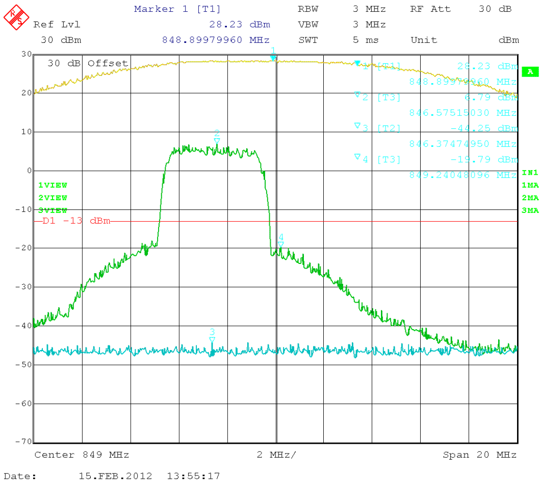
Figure 22: WCDMA – In vs. Out 846.50 MHz
