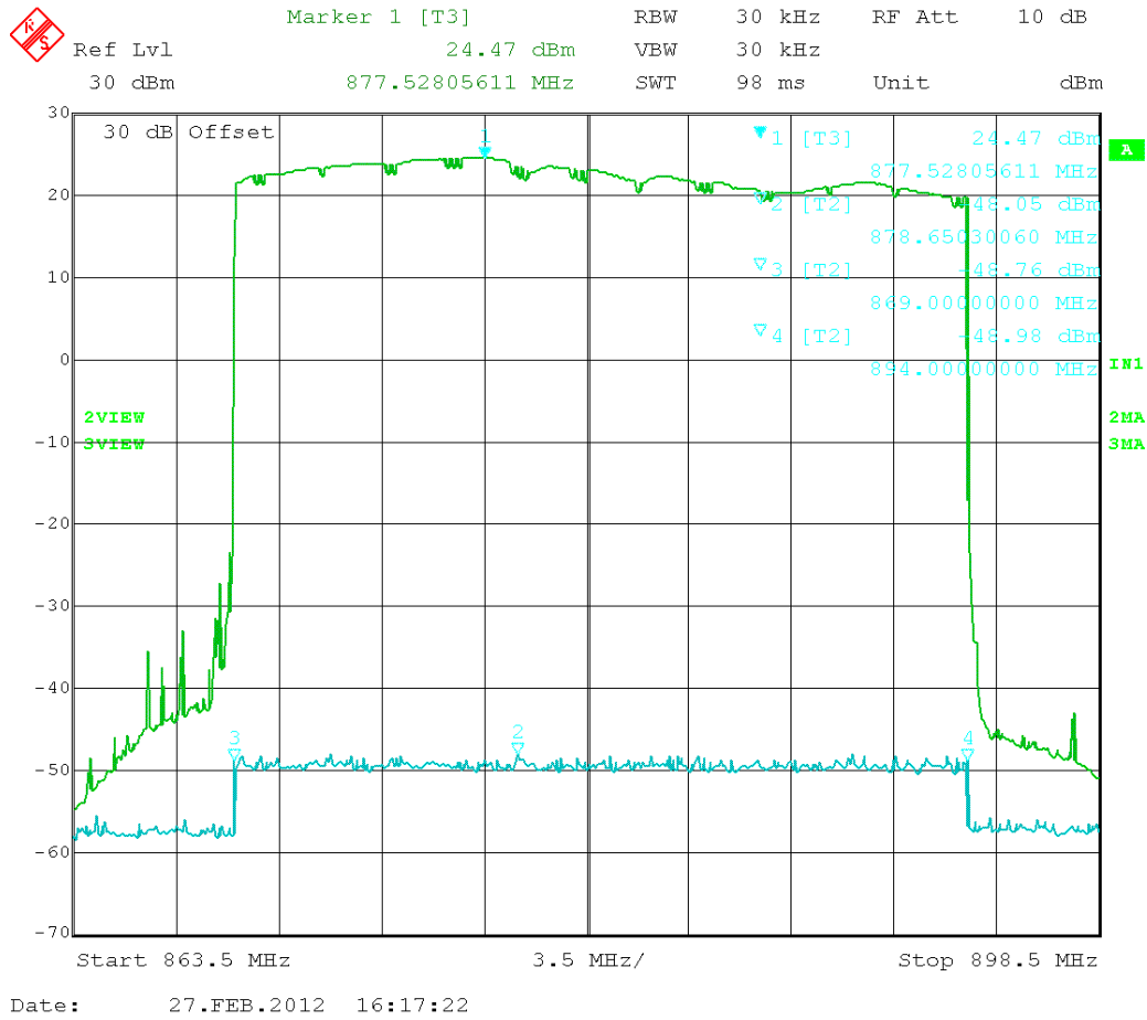
Figure 45. Frequency response (869 – 894) MHz band
