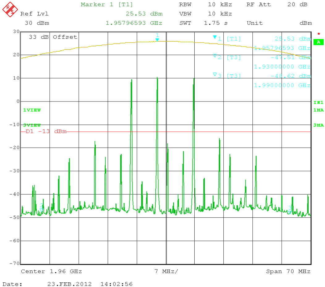
Figure 39: GSM 3 tones intermodulation - (1930 – 1990) MHz
