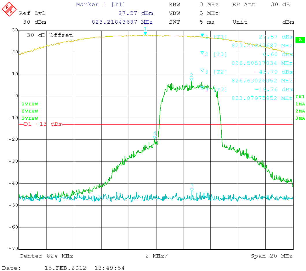
Figure 21: WCDMA – In vs. Out 826.50 MHz
