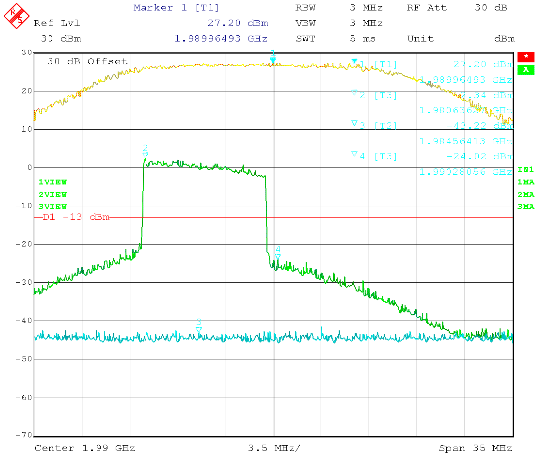
Figure 12: LTE – In vs. Out 1985.00 MHz
