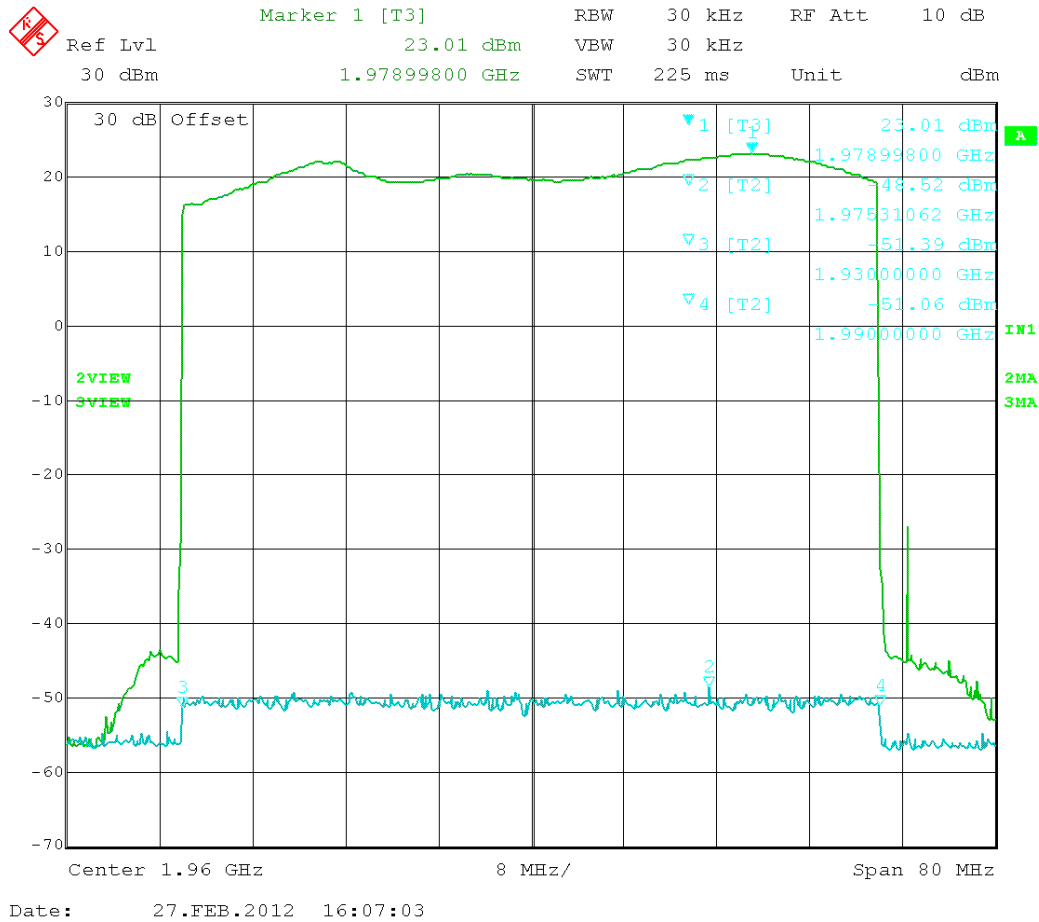
Figure 43. Frequency response (1930 – 1990) MHz band
