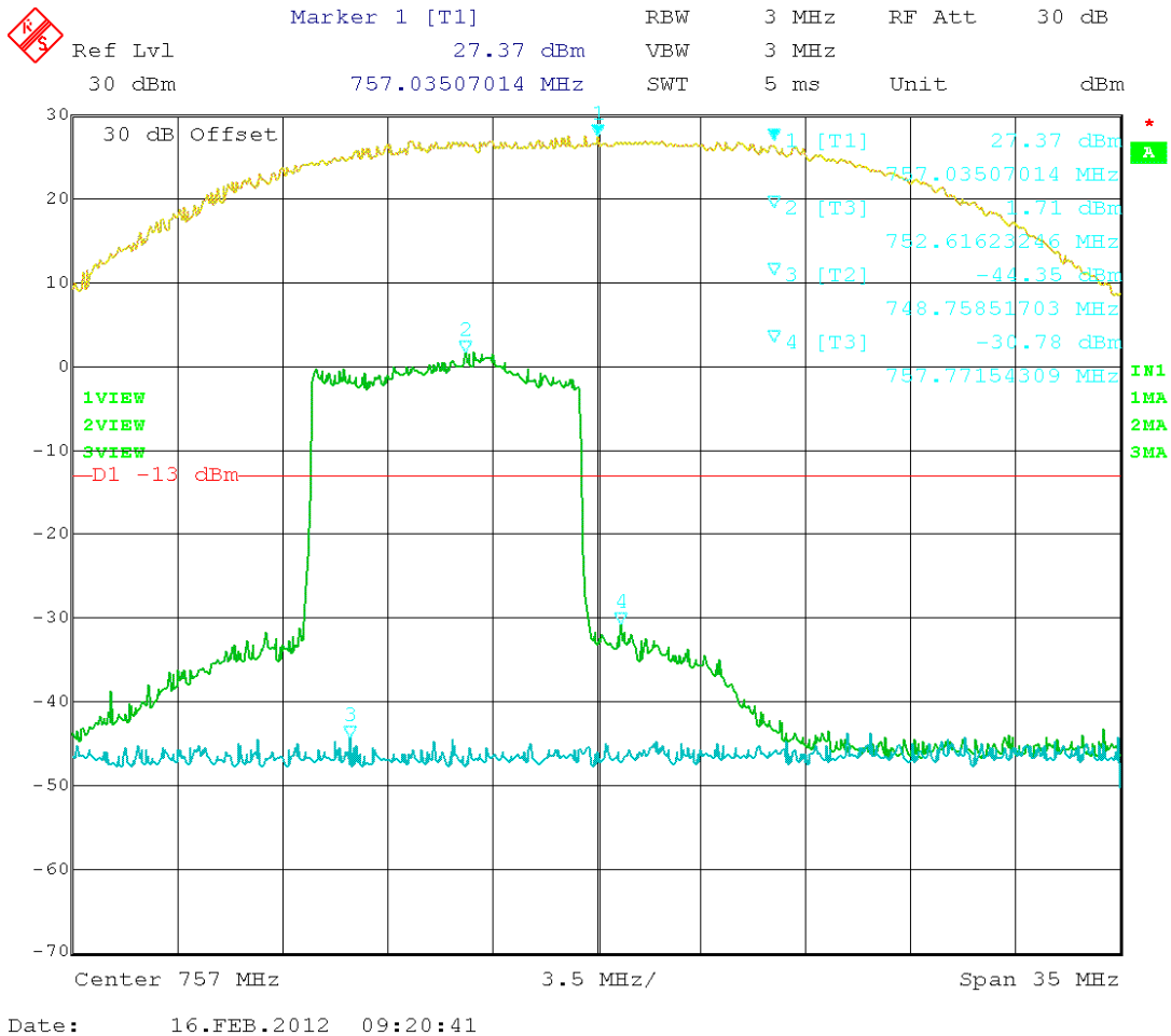
Figure 36: LTE – In vs. Out 752.0 MHz
