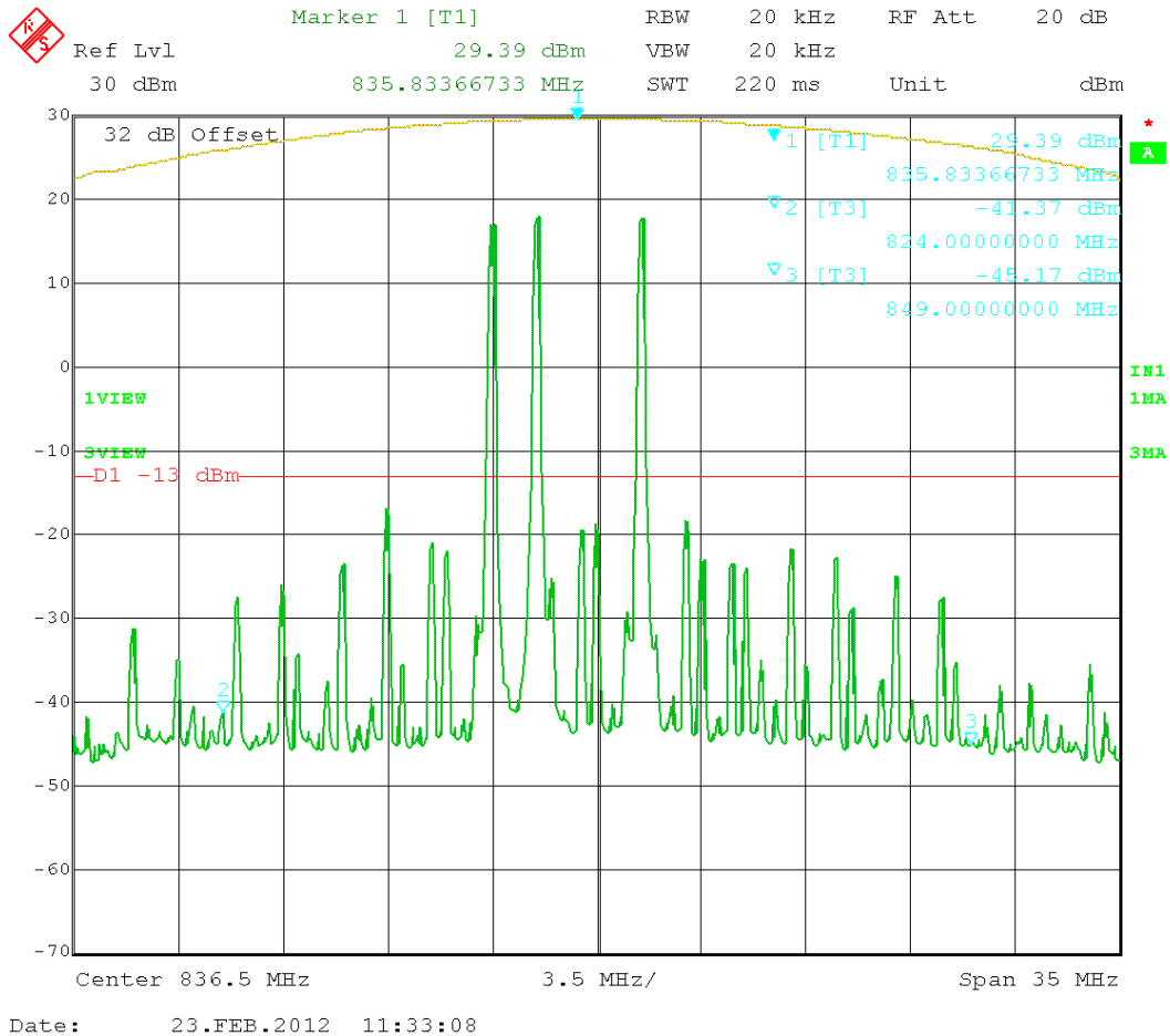
Figure 40: GSM 3 tones intermodulation - (824 – 849) MHz
