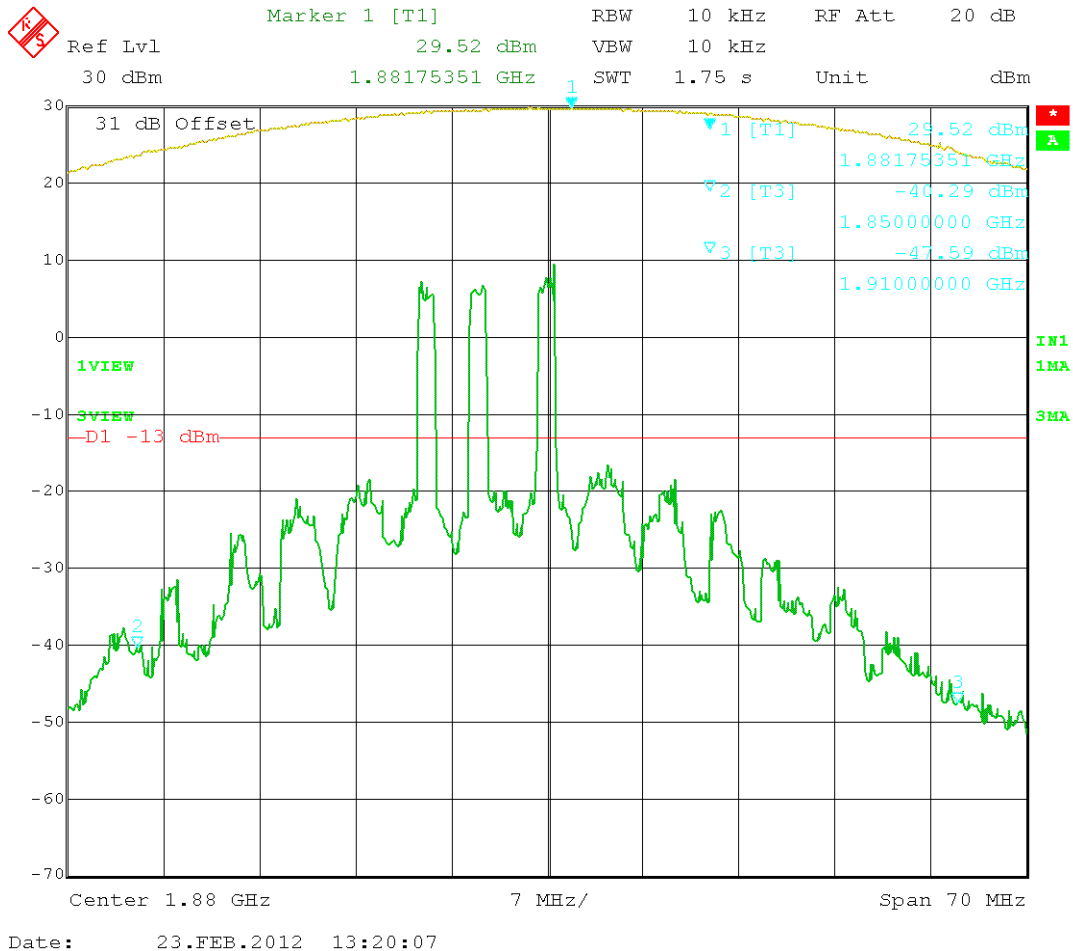
Figure 34: CDMA 3 tones intermodulation - (1850 – 1910) MHz.
