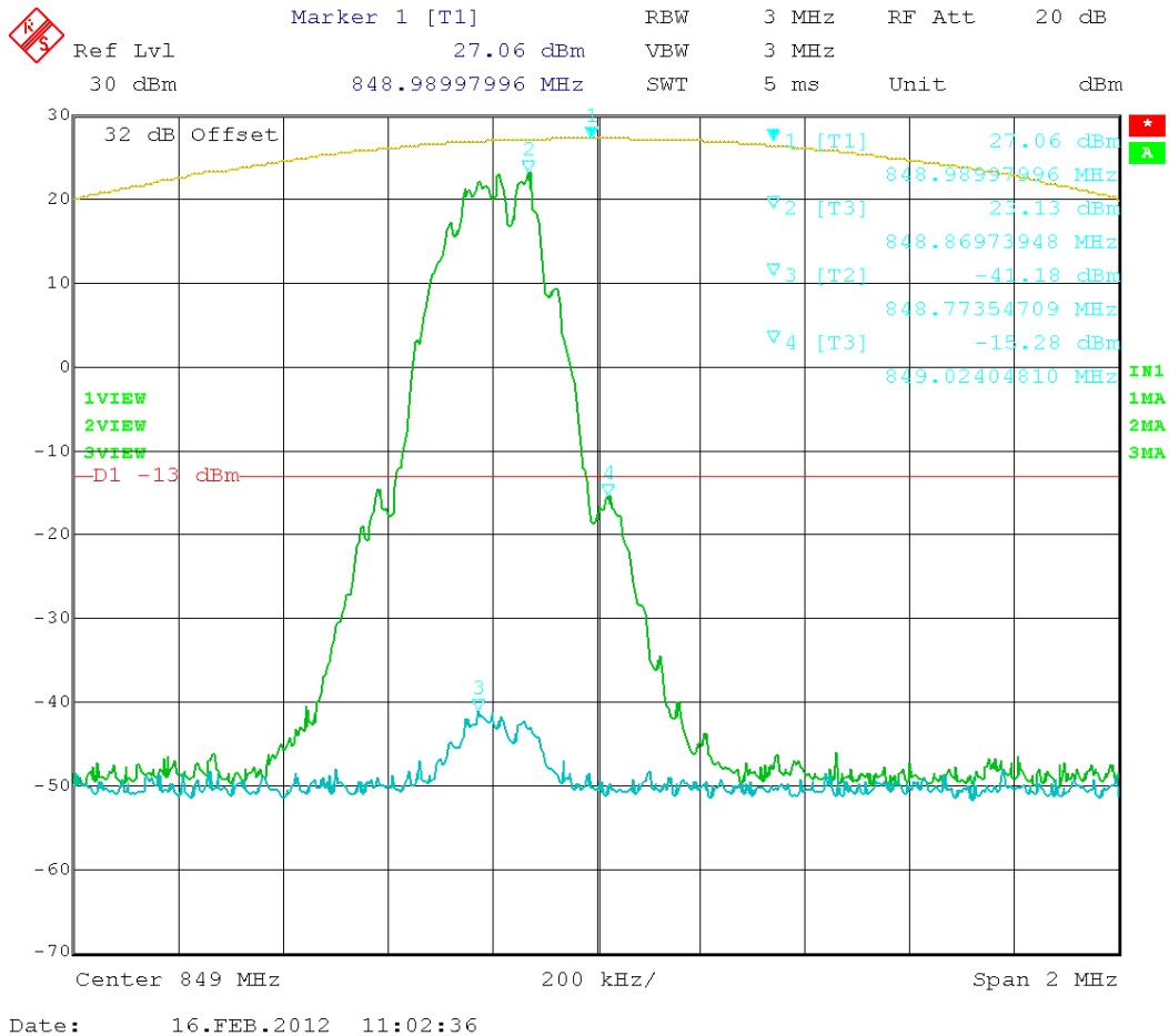
Figure 30: GSM – In vs. Out 848.8 MHz
