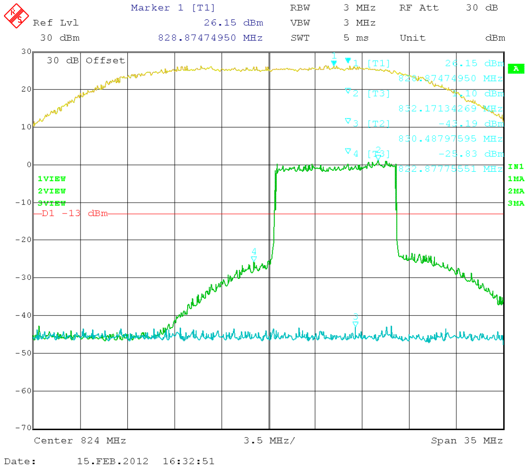
Figure 25: LTE – In vs. Out 829.00 MHz
