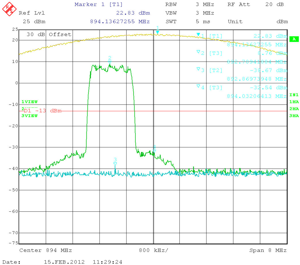
Figure 20: CDMA – In vs. Out 892.75 MHz
