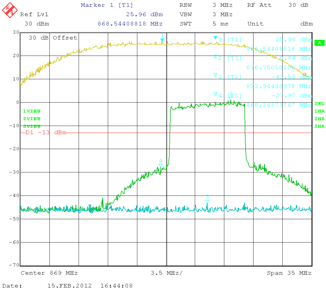
Figure 27: LTE – In vs. Out 874.00 MHz
