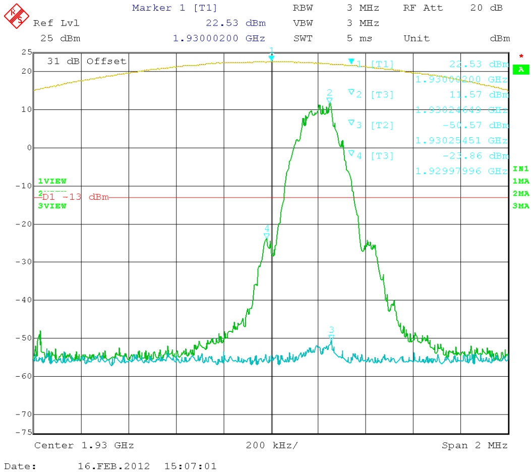
Figure 11: EDGE – In vs. Out 1930.20MHz
