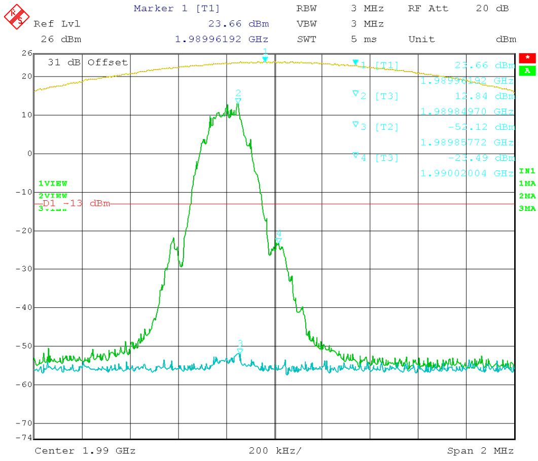
Figure 12: EDGE – In vs. Out 1989.80MHz
