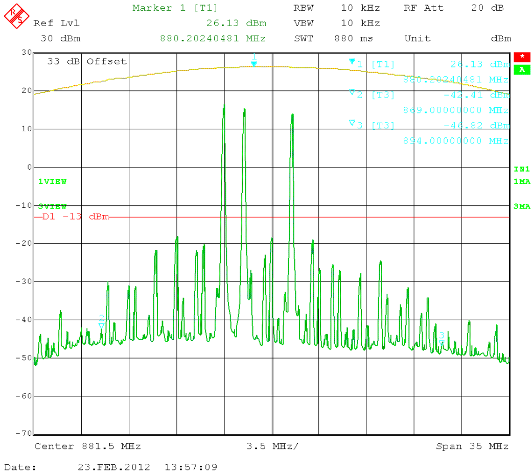
Figure 41: GSM 3 tones intermodulation - (869 – 894) MHz
