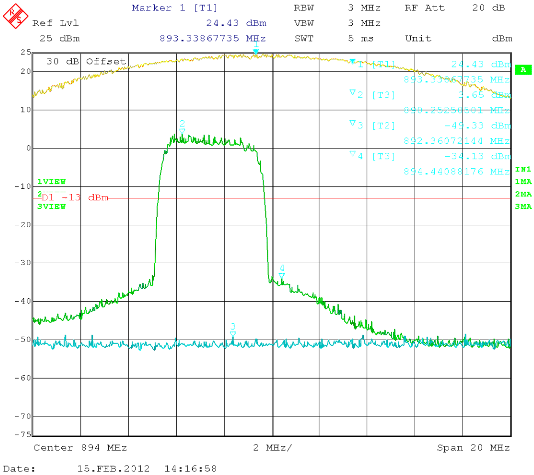
Figure 24: WCDMA – In vs. Out 893.50 MHz
