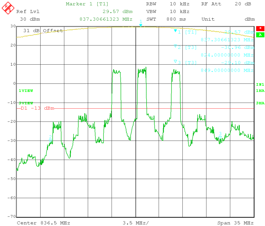
Figure 36: CDMA 3 tones intermodulation – (824 – 849) MHz.
