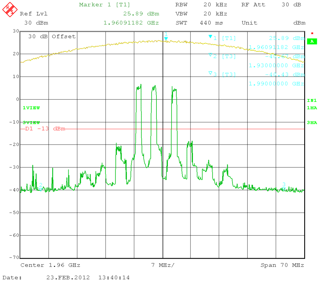
Figure 35: CDMA 3 tones intermodulation - (1930 – 1990) MHz.
