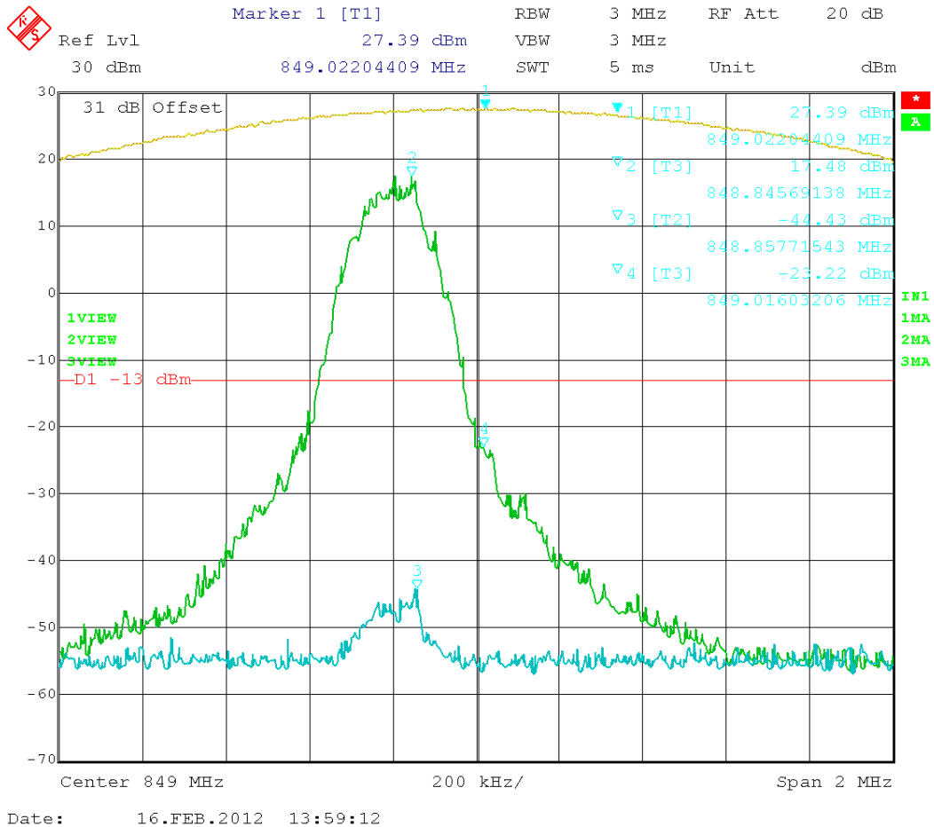
Figure 26: EDGE – In vs. Out 848.80 MHz
