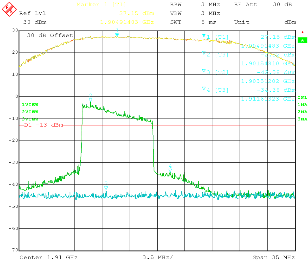
Figure 10: LTE – In vs. Out 1905.00 MHz
