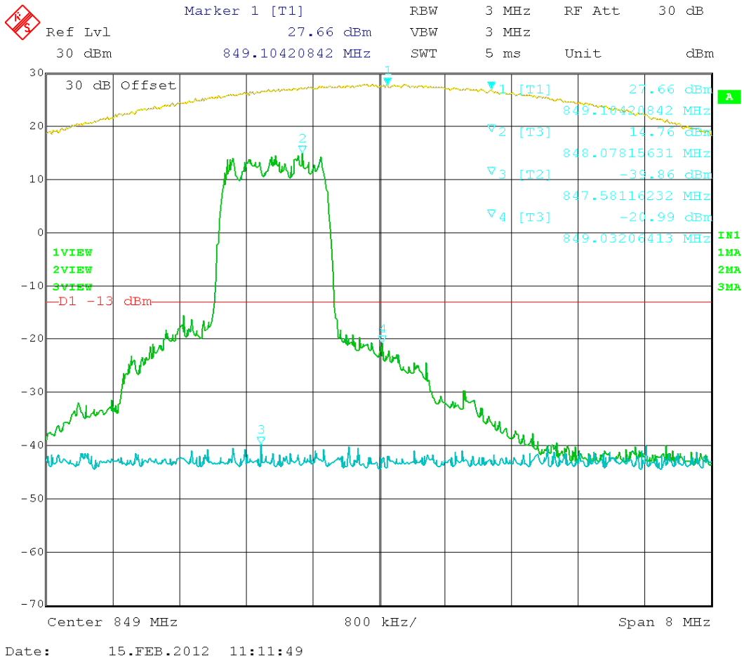
Figure 18: CDMA – In vs. Out 847.75 MHz
