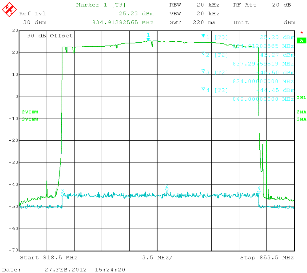
Figure 44. Frequency response (824 – 849) MHz band
