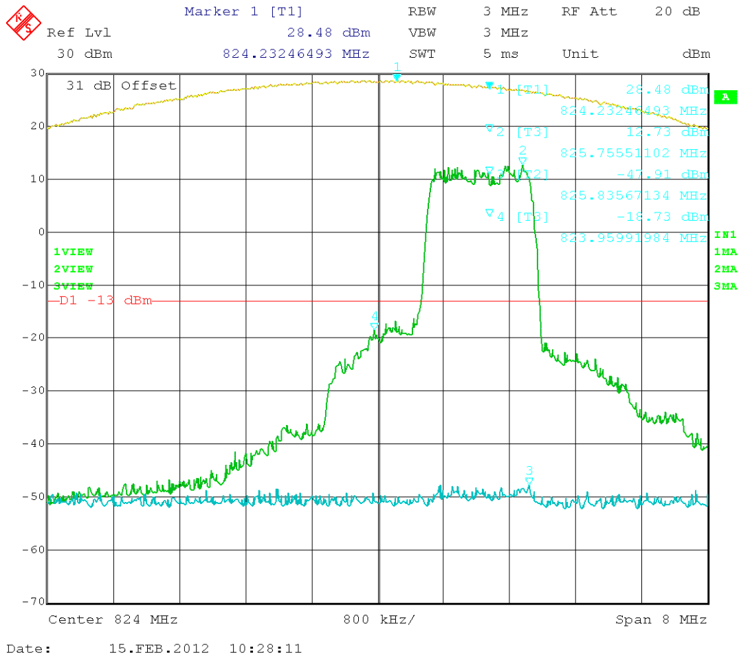
Figure 17: CDMA – In vs. Out 825.25MHz
