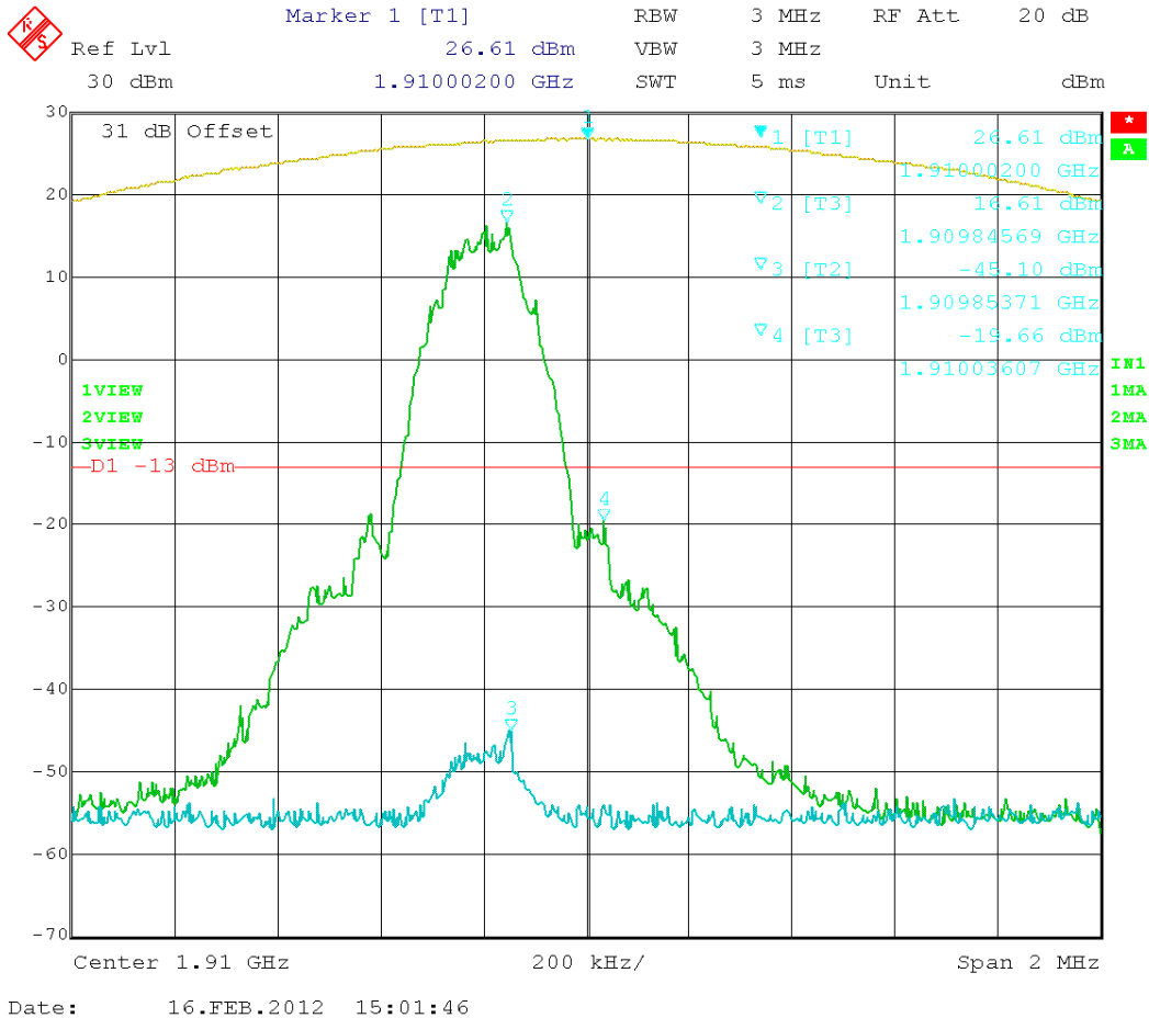
Figure 10: EDGE – In vs. Out 1909.80MHz
