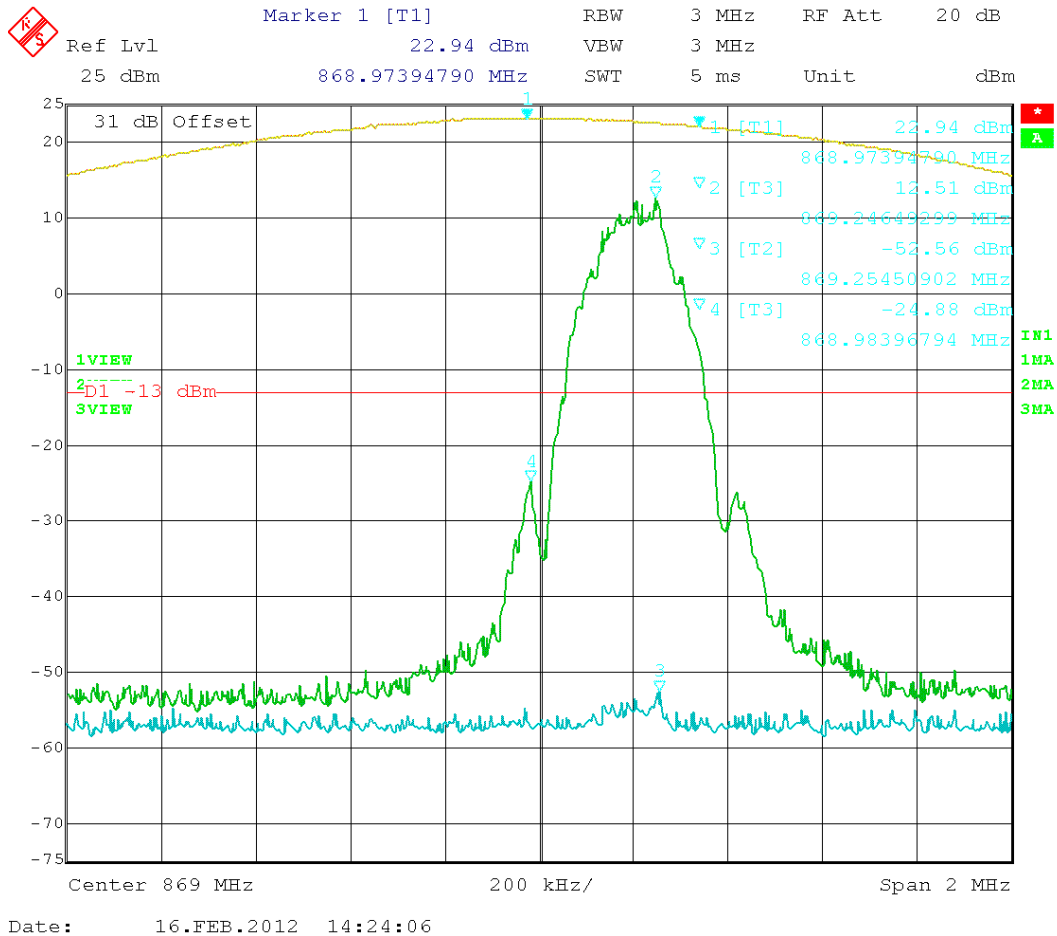
Figure 27: EDGE – In vs. Out 869.20 MHz
