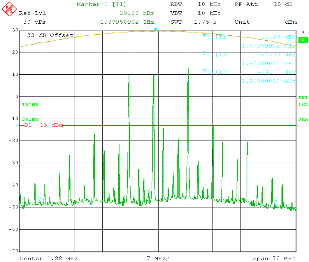
Figure 38: GSM 3 tones intermodulation - (1850 – 1910) MHz
