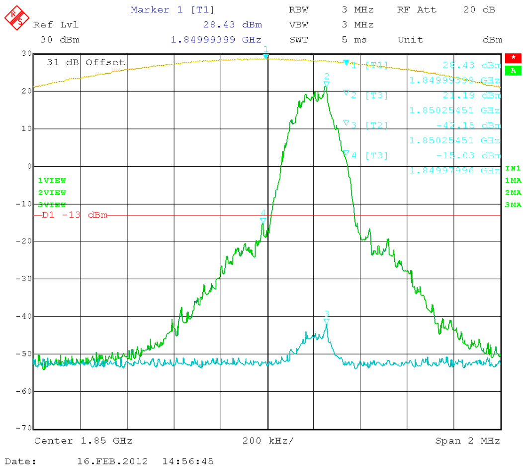
Figure 9: EDGE – In vs. Out 1850.20MHz
