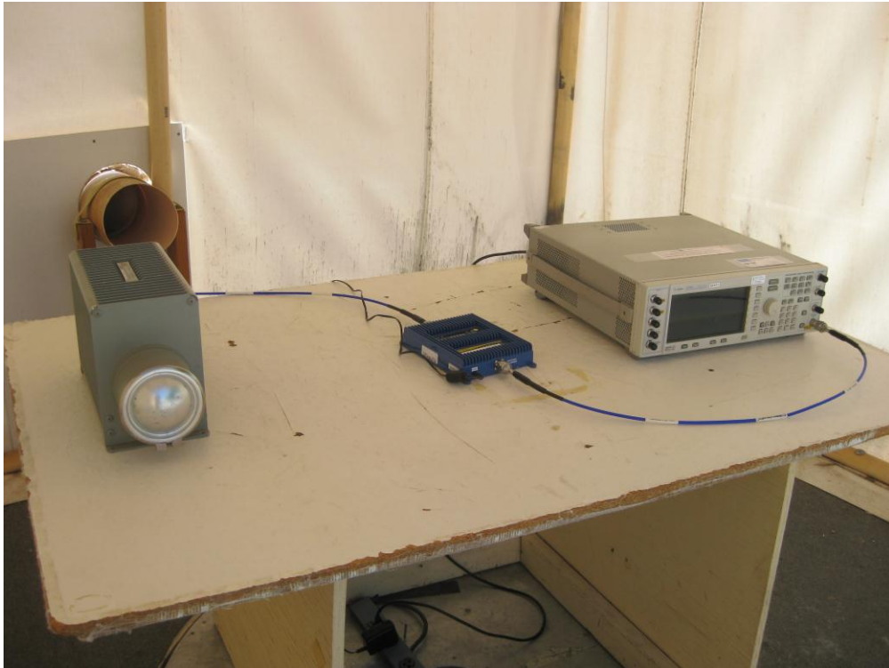
RF Radiated
