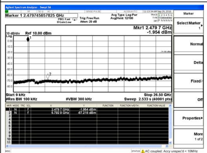
BLE-High channel
