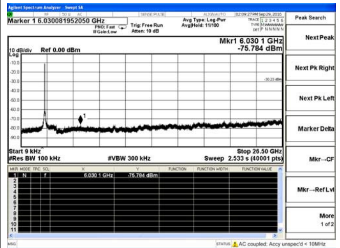
802.11g-Low channel
