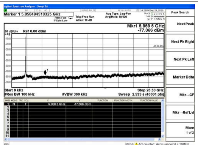
802.11b-High channel
