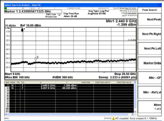
BLE-Middle channel
