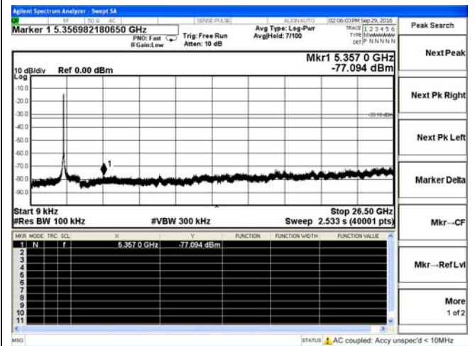
802.11n-HT40-Low channel
