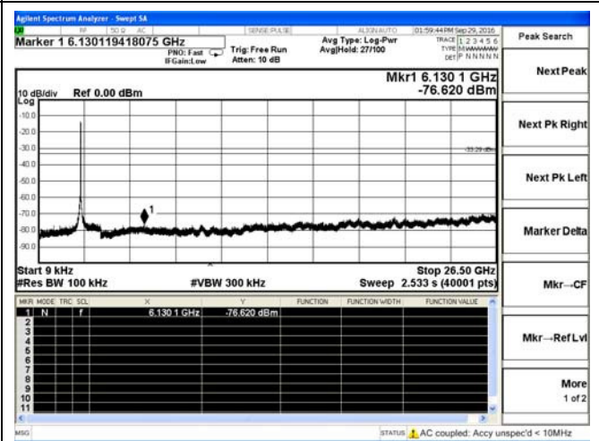
802.11n-HT40-High channel
