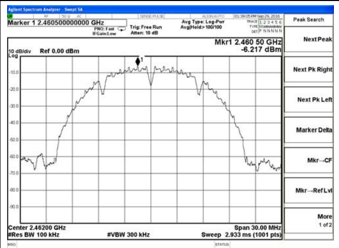
802.11b-High Channel
