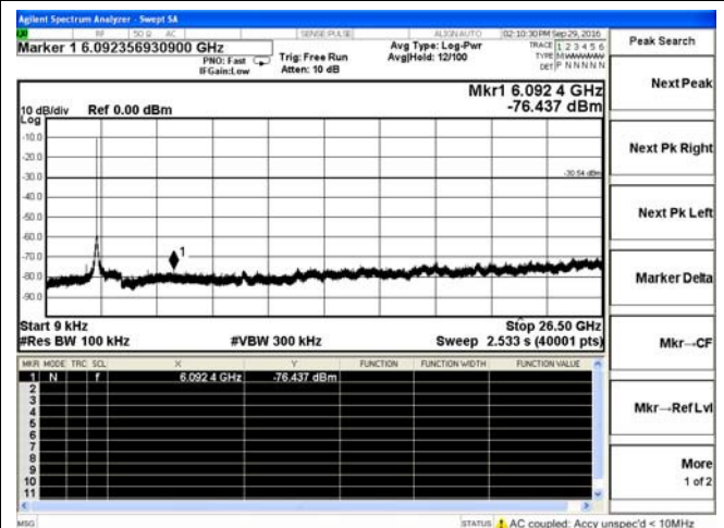
802.11g-Middle channel
