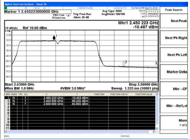
802.11n-HT40-High channel(Average)
