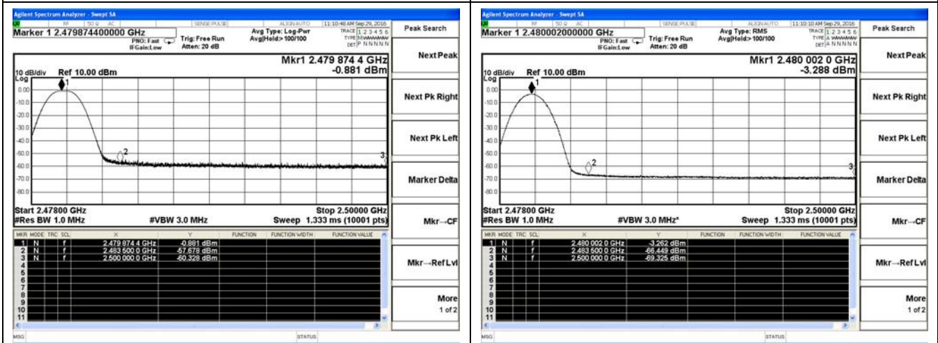
BLE-High channel(Peak)
