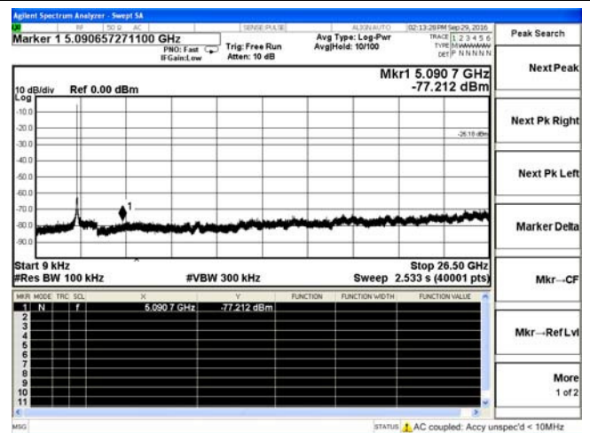
802.11b-Middle channel
