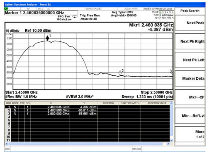
802.11b-High channel(Average)
