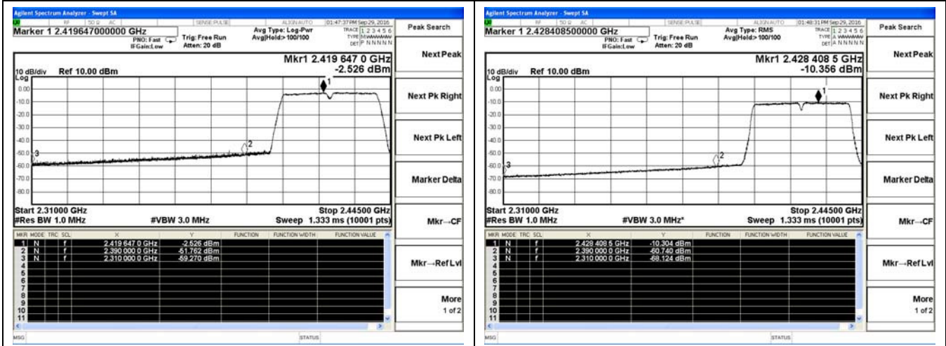
802.11n-HT40-Low channel(Peak)
