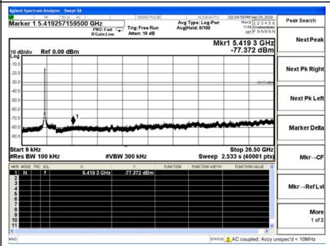
802.11n-HT40-Middle channel
