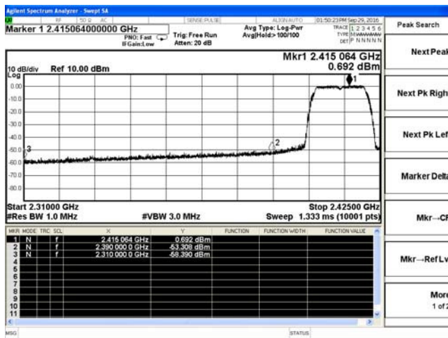
802.11g-Low channel(Peak)
