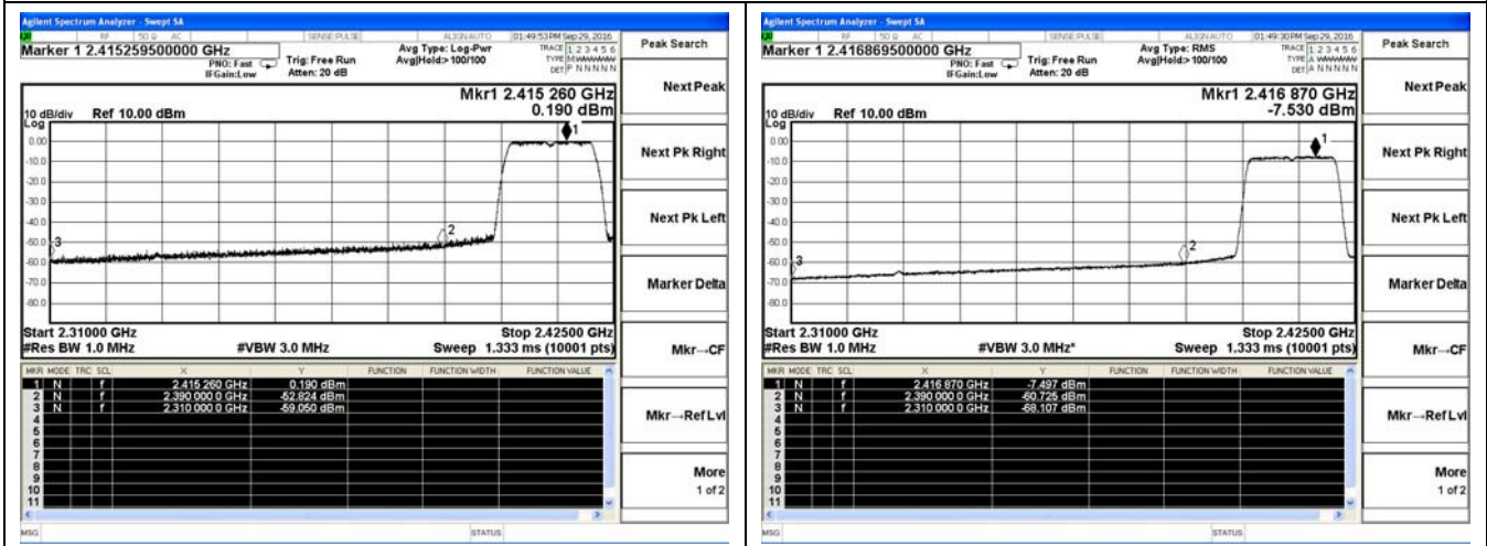
802.11n-HT20-Low channel(Peak)
