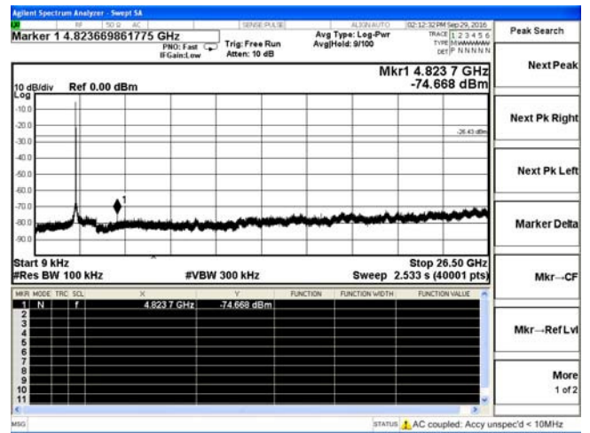
802.11b-Low channel
