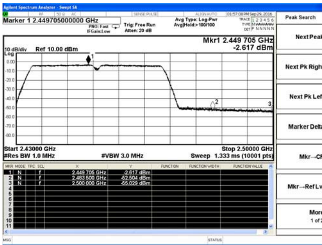
802.11n-HT40-High channel(Peak)
