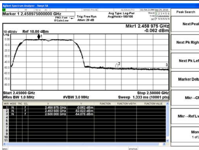
802.11g-High channel(Peak)
