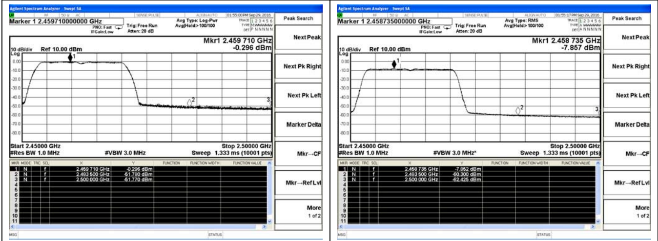
802.11n-HT20-High channel(Peak)
