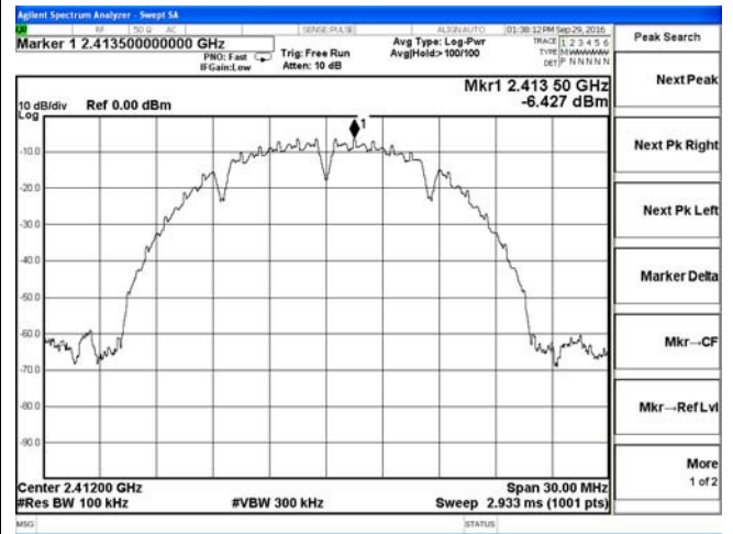
802.11b-Low Channel
