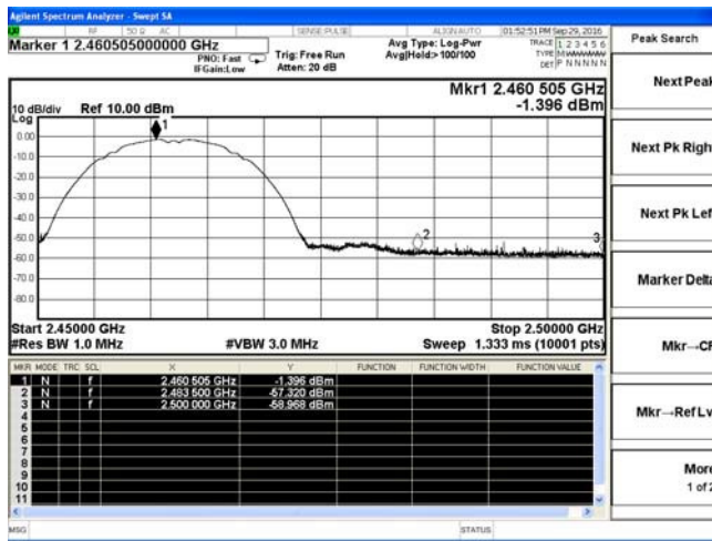
802.11b-High channel(Peak)
