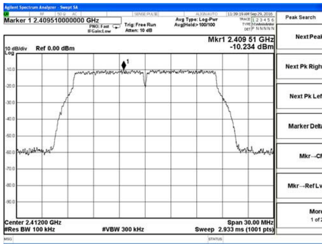
802.11g-Low Channel
