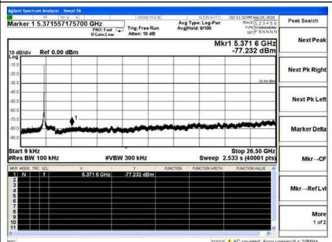
802.11g-High channel
