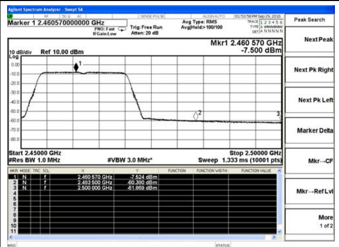
802.11g-High channel(Average)
