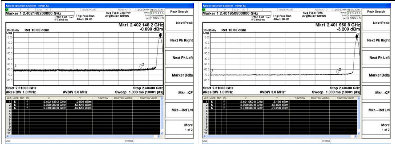
BLE-Low channel(Peak)
