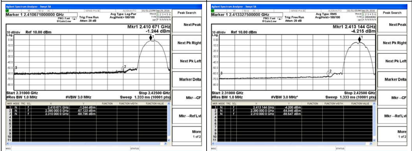
802.11b-Low channel(Peak)
