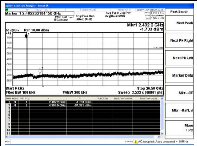
BLE-Low channel
