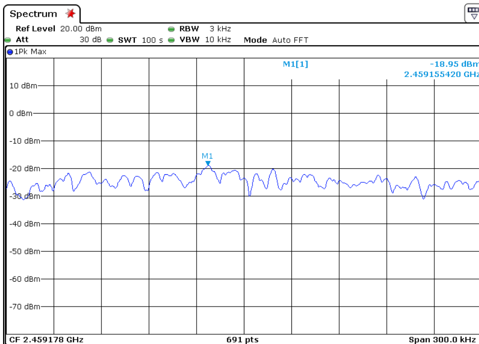
Channel 11: 2.462GHz:
