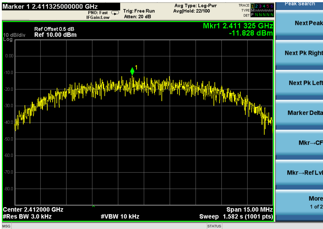
802.11b power density
