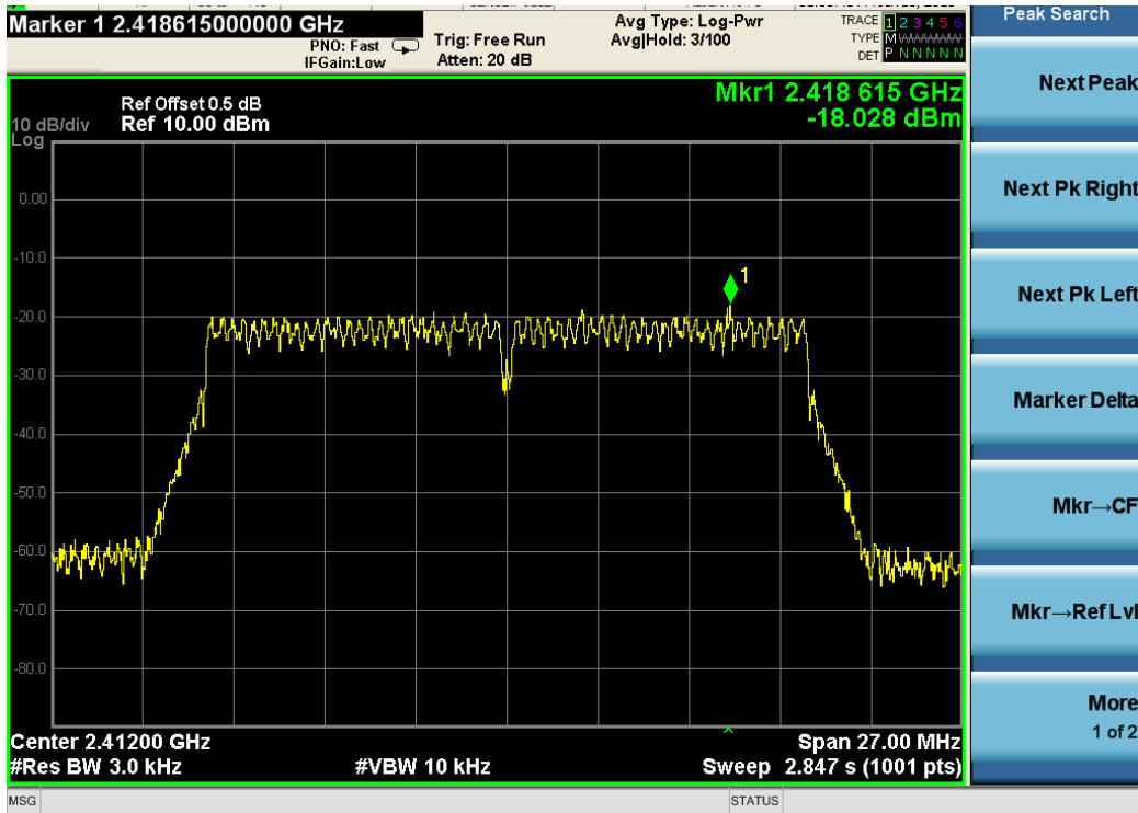
80.11n HT20 power density
