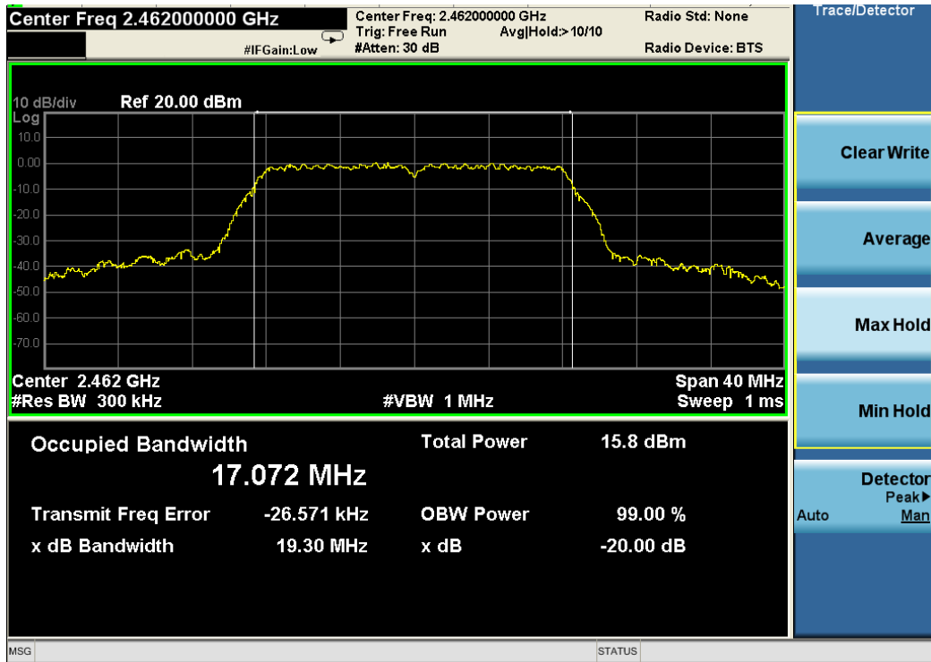
802.11n HT20 channel, 20dB bandwidth
