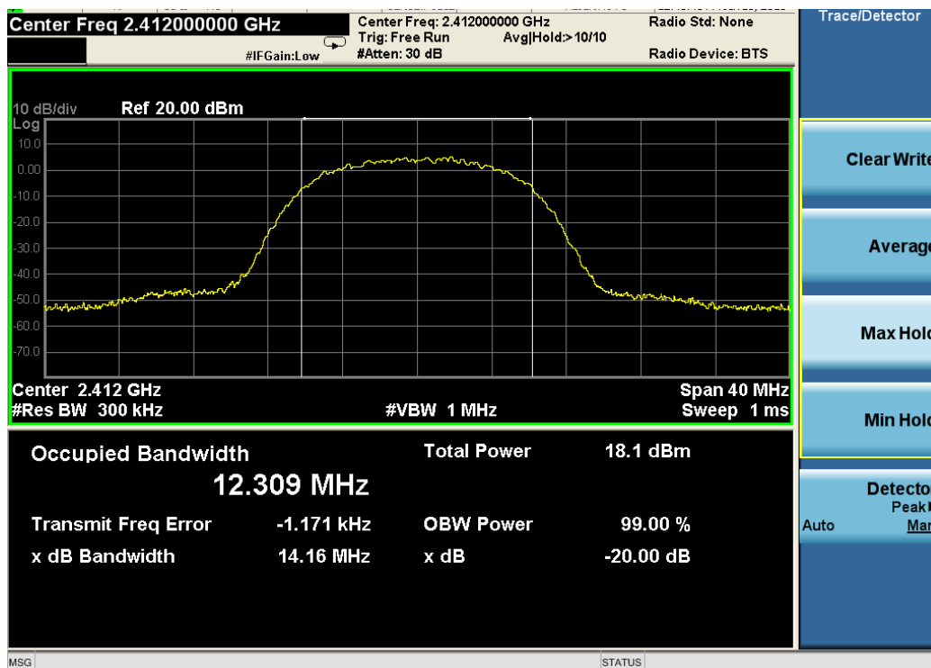
802.11b channel, 20dB bandwidth
