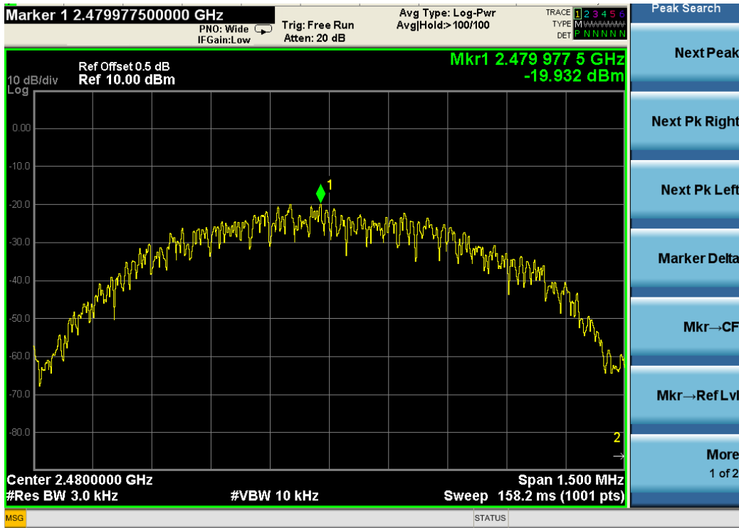
802.11b power density
