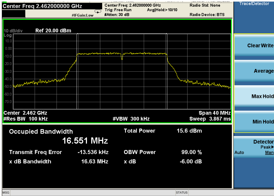
802.11n HT20 channel, 6dB bandwidth
