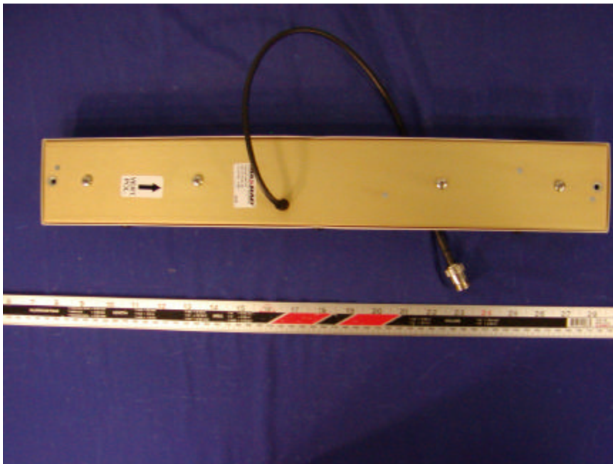
Antenna 2: WISP 24014-90PTNF 14dBi 90 Degree, Sector Panel Bottom View
