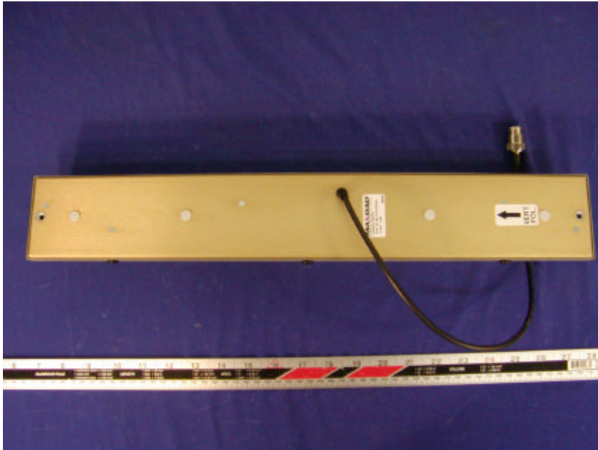
Antenna 1: WISP 24013-120PTNF 13dBi 120 degree, Sector Panel Bottom View
