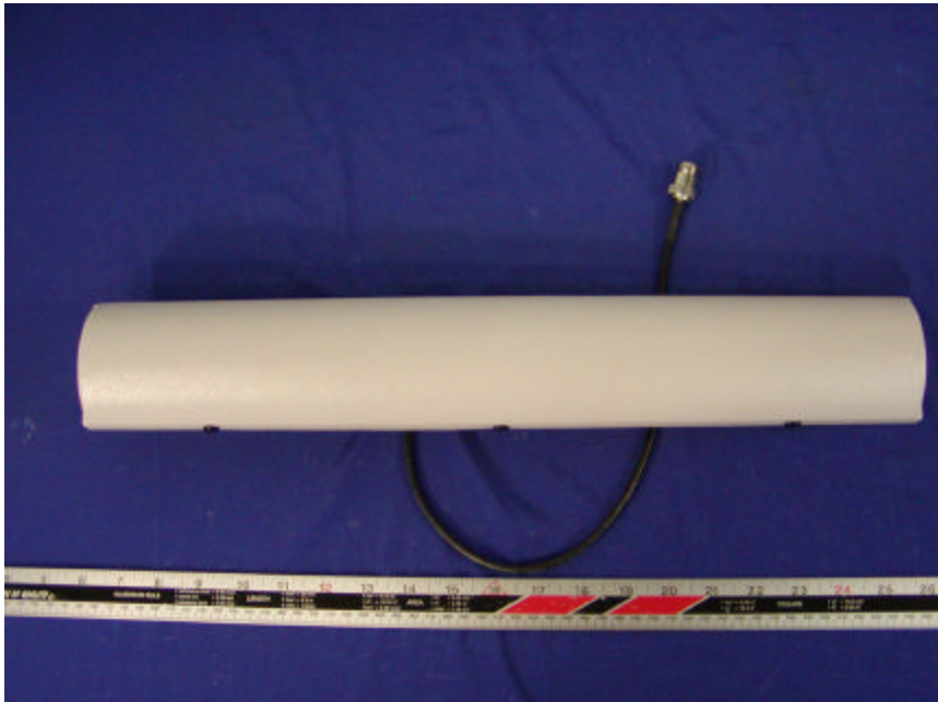
Antenna 2: WISP 24014-90PTNF 14dBi 90 Degree, Sector Panel Top View
